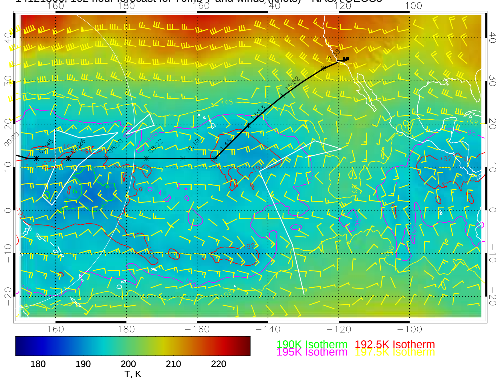
14121306, 102 hour forecast for 70mb T and winds (knots)-- NASA GEOS5
