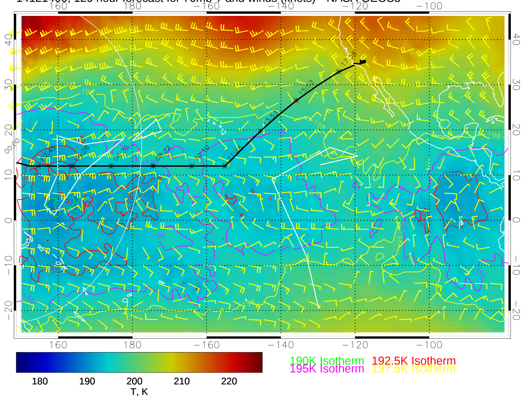
14121400, 120 hour forecast for 70mb T and winds (knots)-- NASA GEOS5
