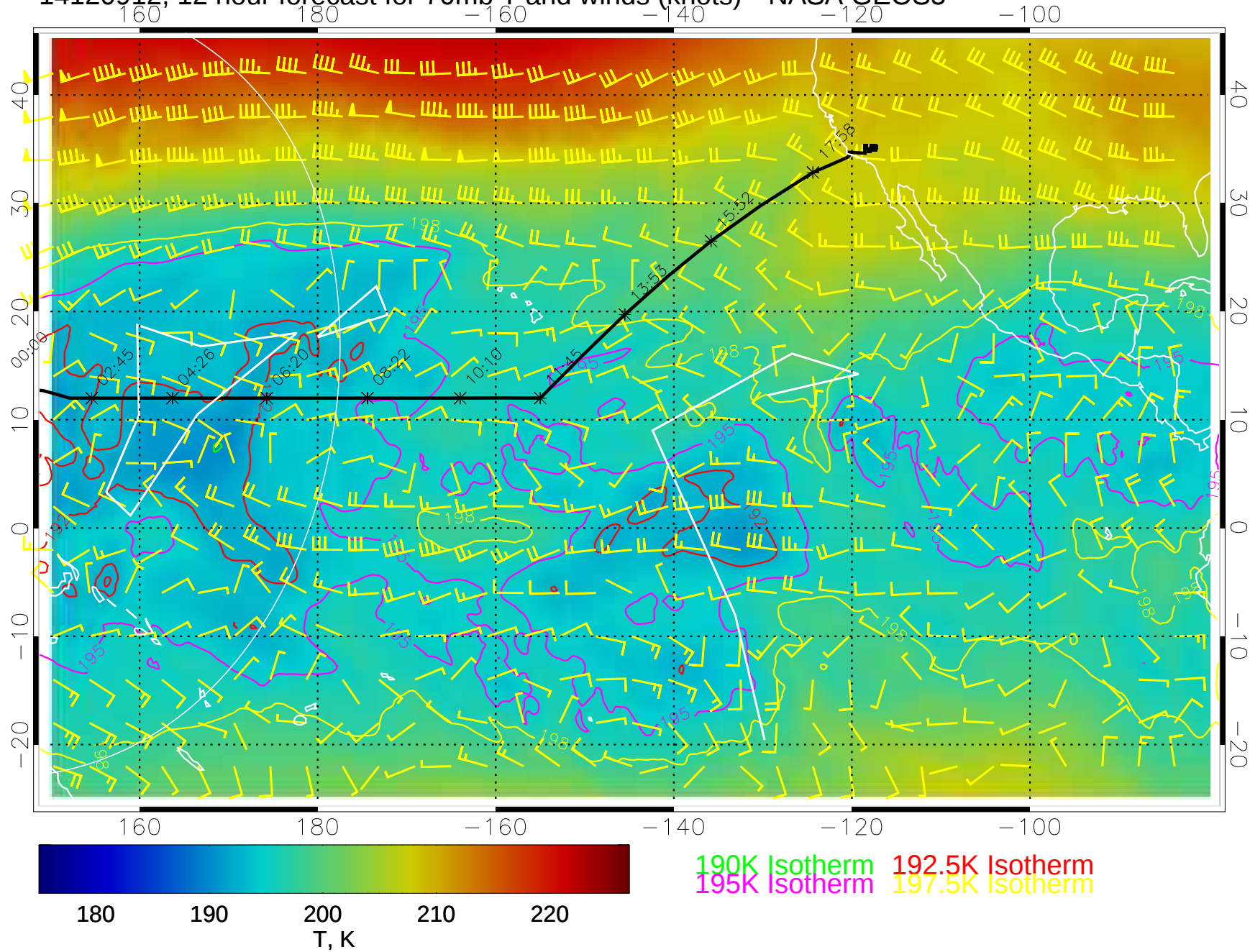
14120912, 12 hour forecast for 70mb T and winds (knots)-- NASA GEOS5
