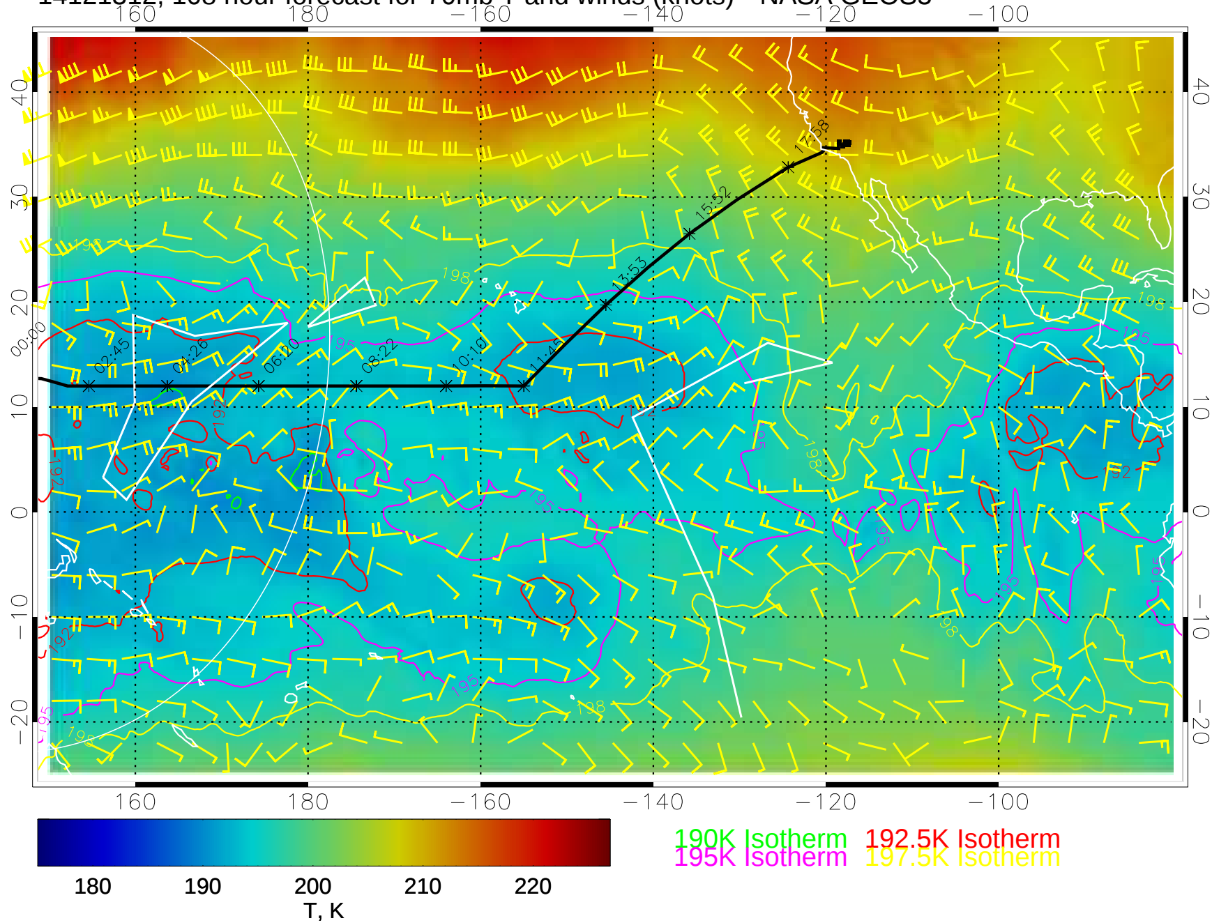
14121312, 108 hour forecast for 70mb T and winds (knots)-- NASA GEOS5
