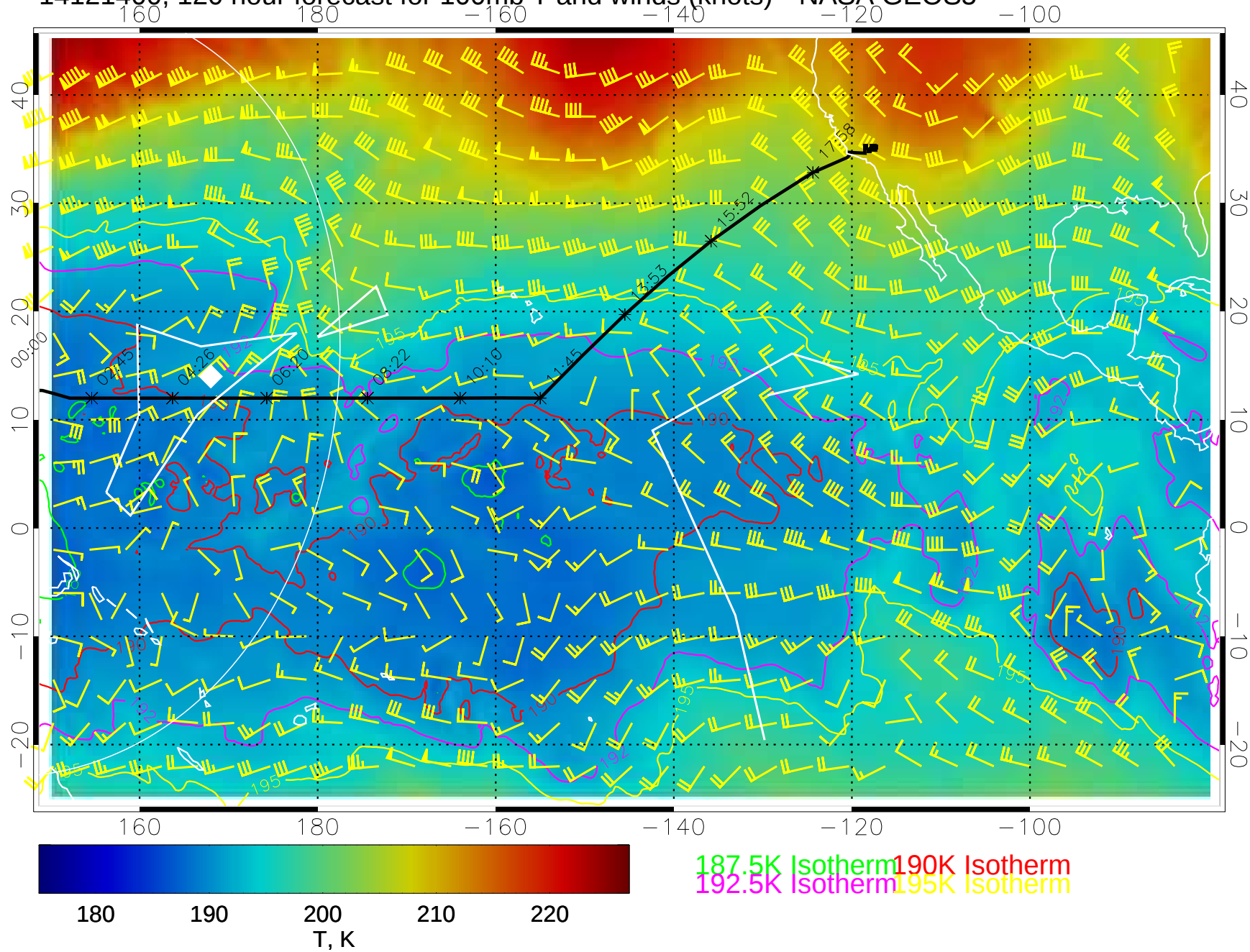
14121400, 120 hour forecast for 100mb T and winds (knots)-- NASA GEOS5
