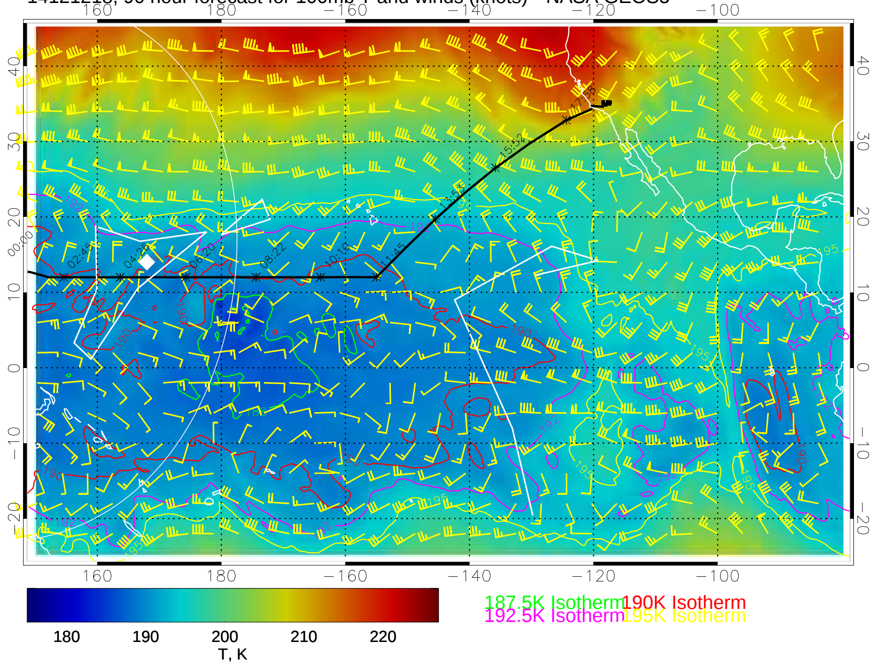
14121218, 90 hour forecast for 100mb T and winds (knots)-- NASA GEOS5
