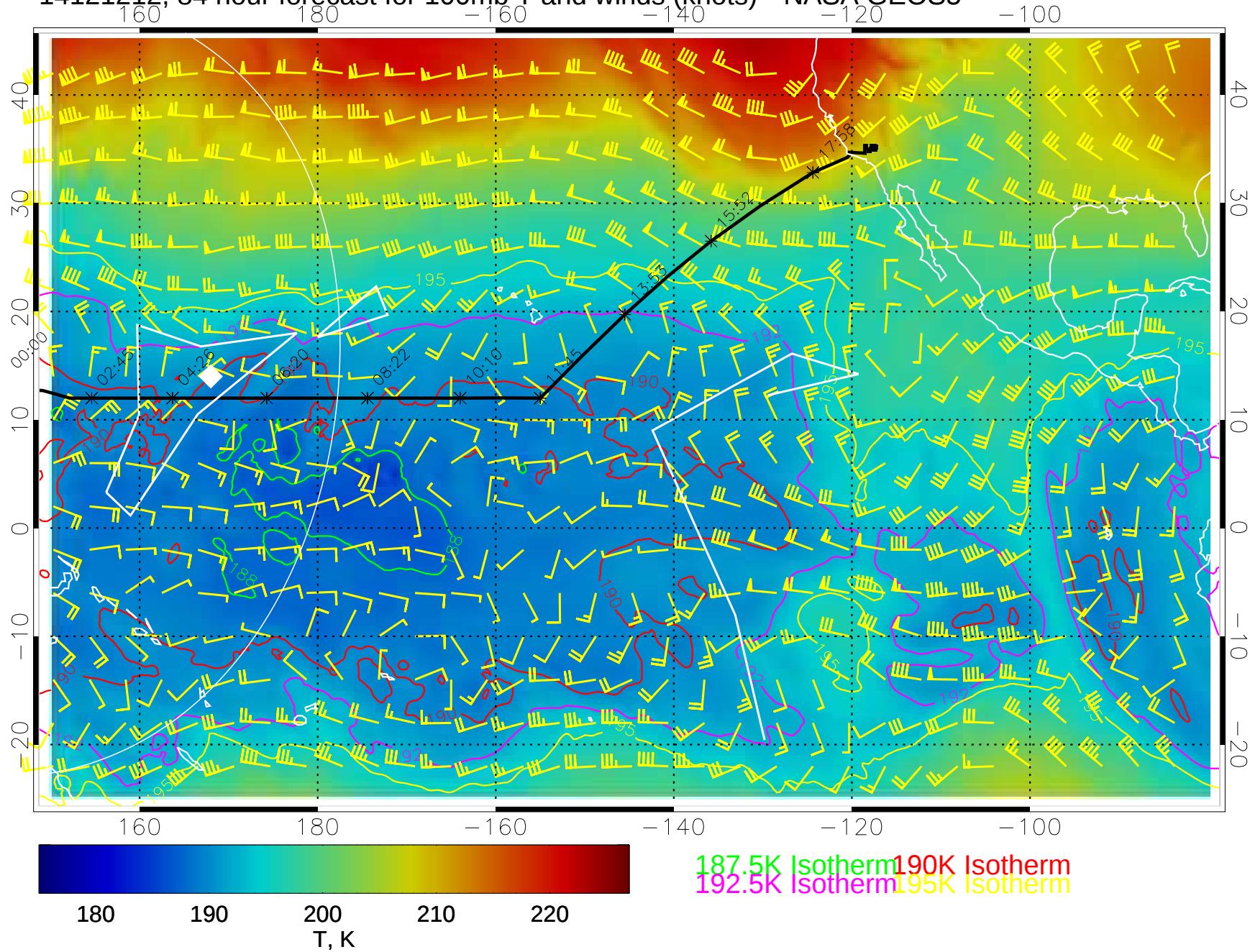
14121212, 84 hour forecast for 100mb T and winds (knots)-- NASA GEOS5
