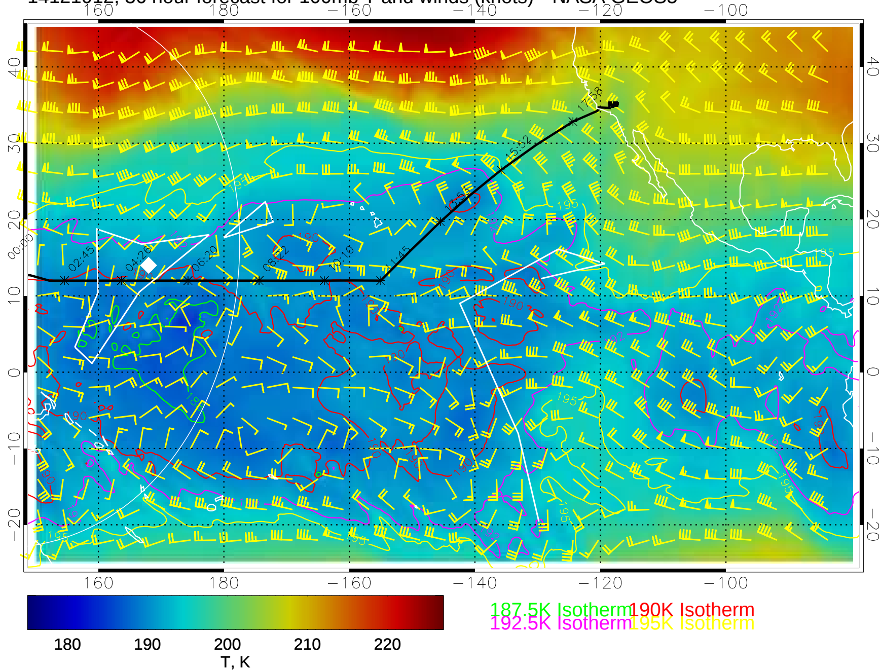
14121012, 36 hour forecast for 100mb T and winds (knots)-- NASA GEOS5
