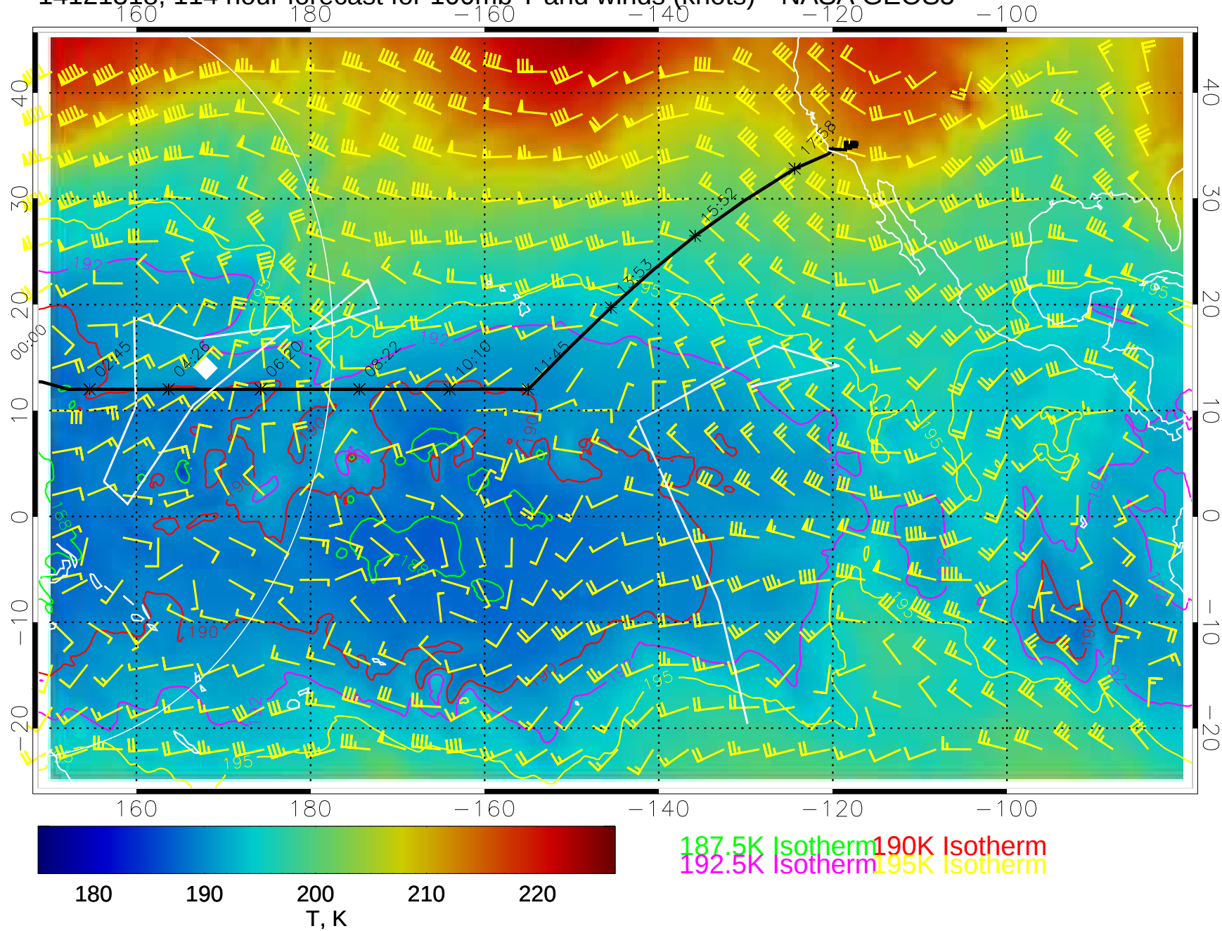
14121318, 114 hour forecast for 100mb T and winds (knots)-- NASA GEOS5
