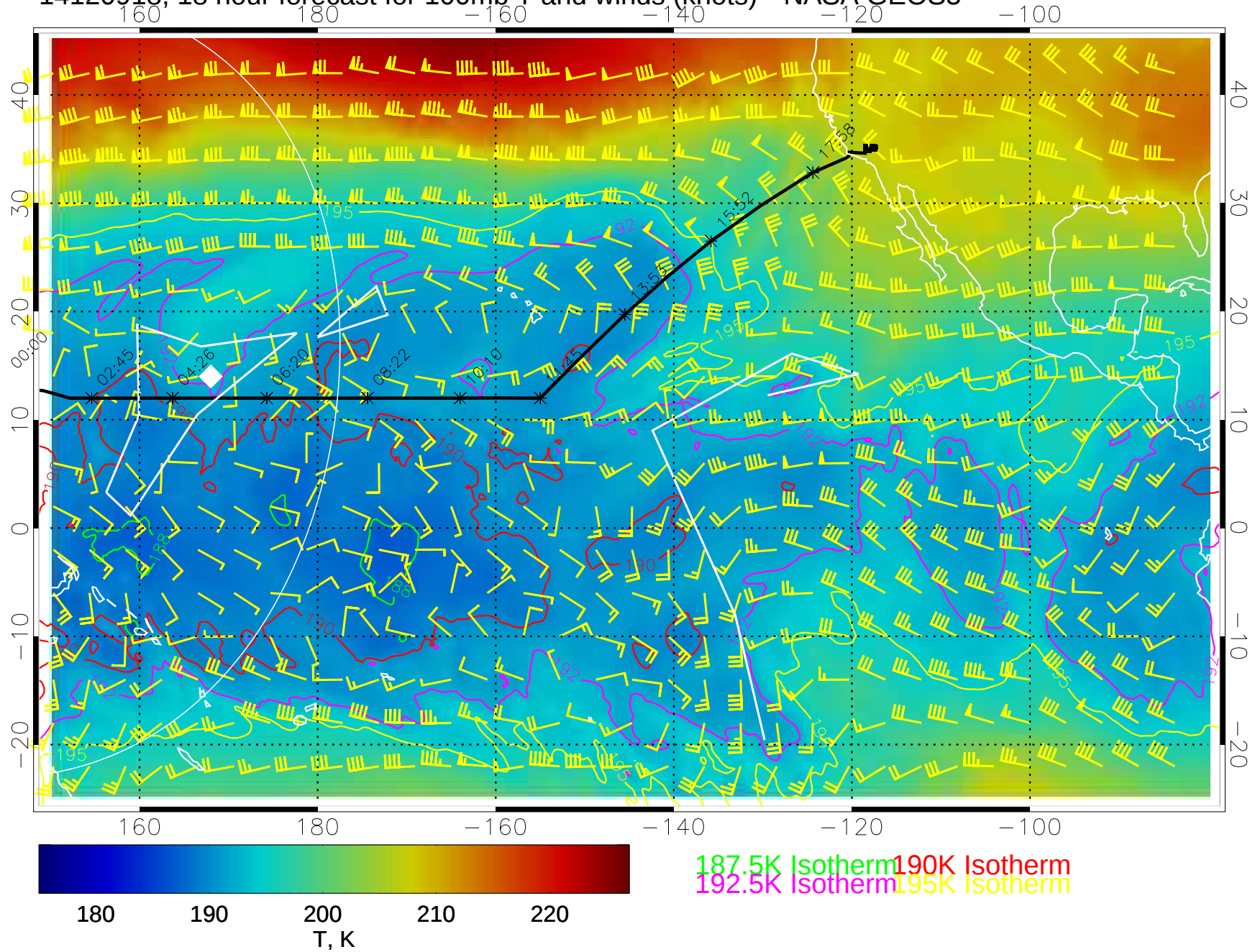
14120918, 18 hour forecast for 100mb T and winds (knots)-- NASA GEOS5
