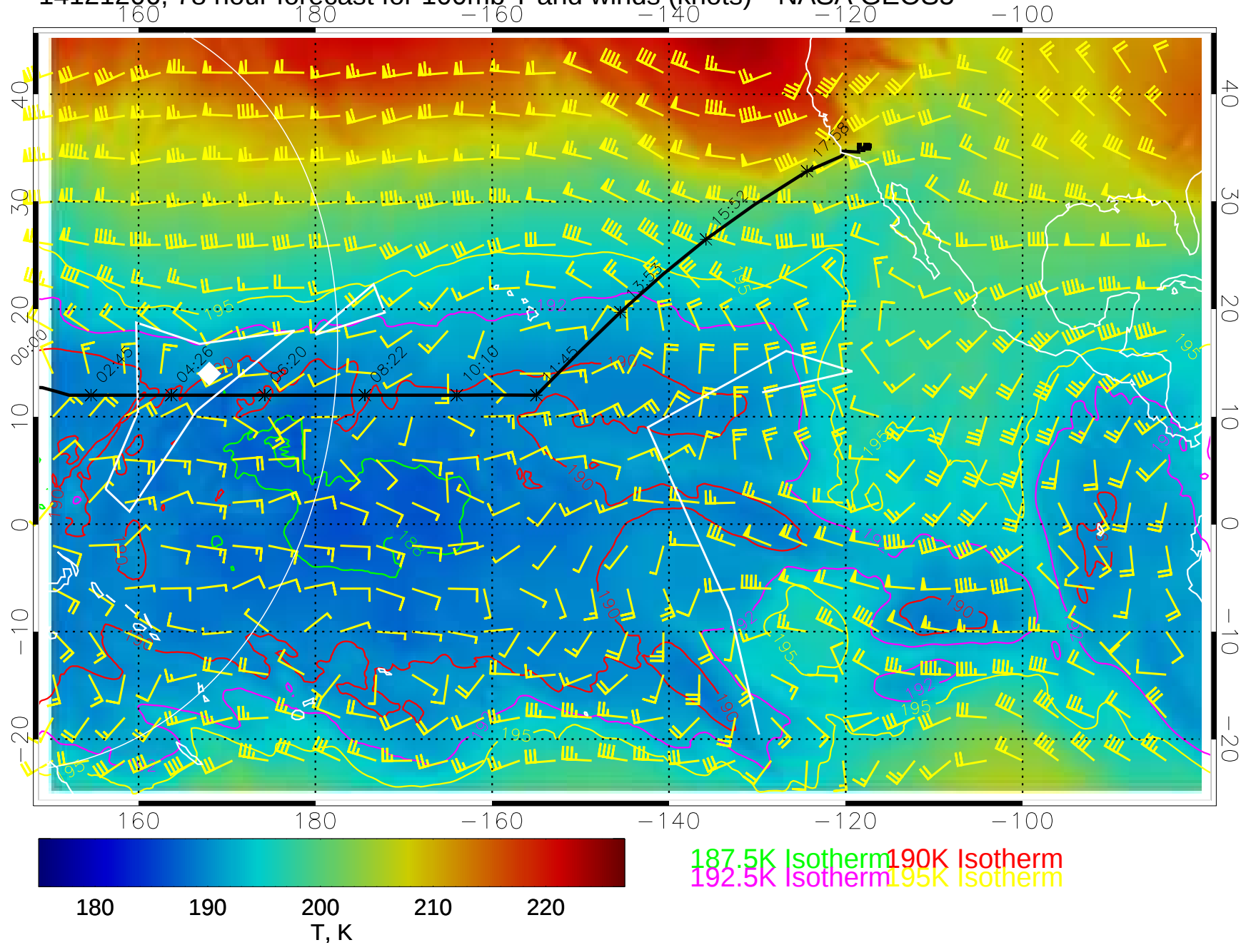
14121206, 78 hour forecast for 100mb T and winds (knots)-- NASA GEOS5
