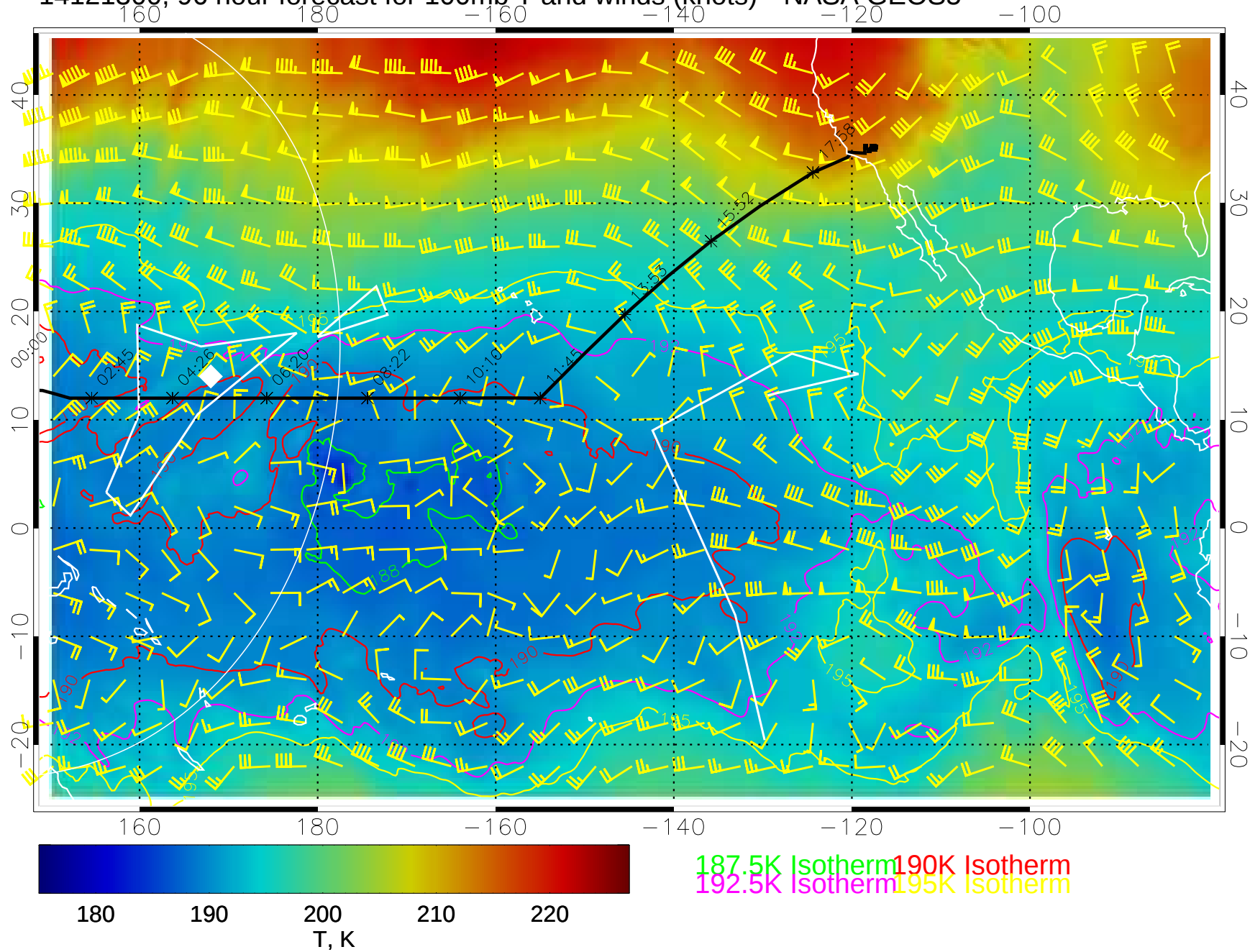
14121300, 96 hour forecast for 100mb T and winds (knots)-- NASA GEOS5
