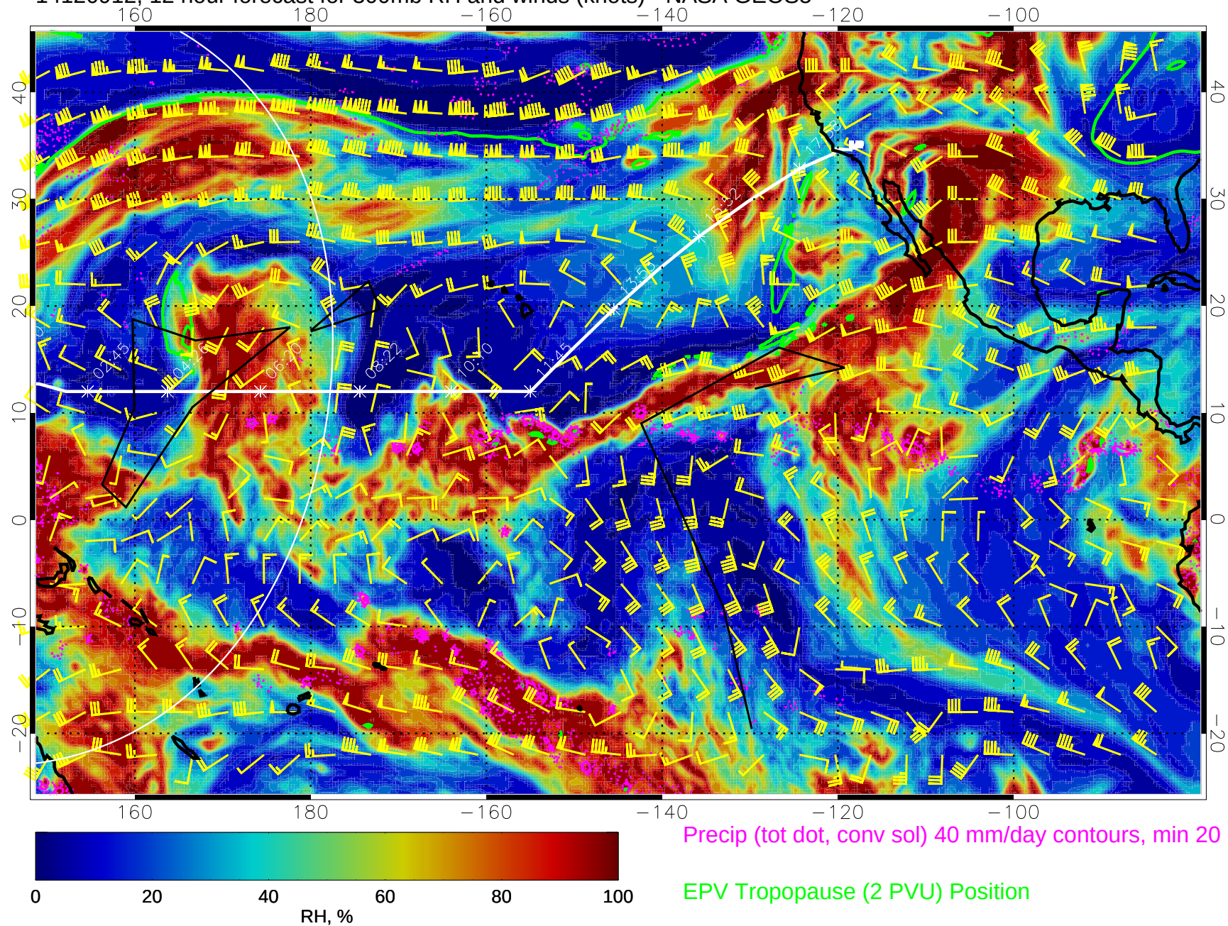
14120912, 12 hour forecast for 300mb RH and winds (knots) - NASA GEOS5
