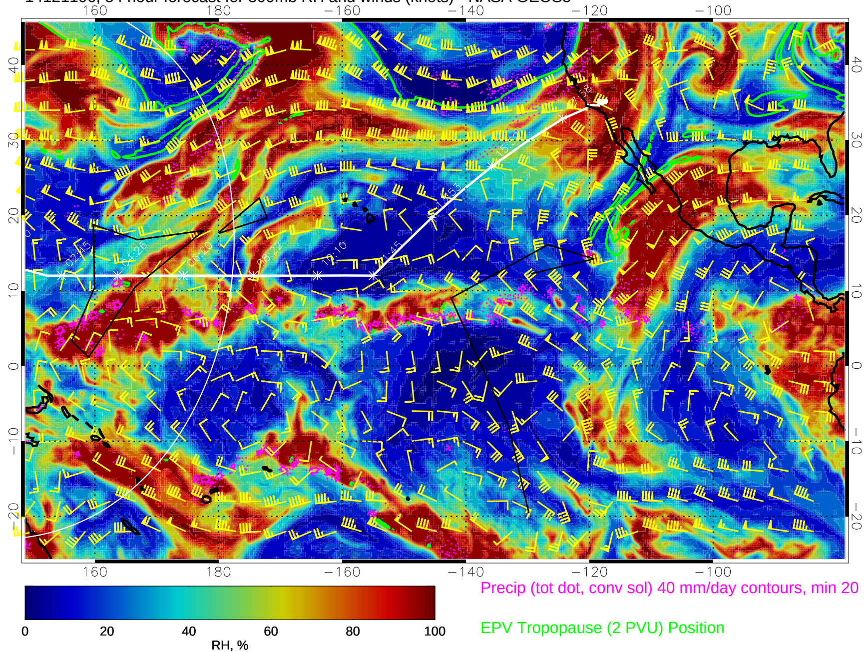
14121106, 54 hour forecast for 300mb RH and winds (knots) - NASA GEOS5
