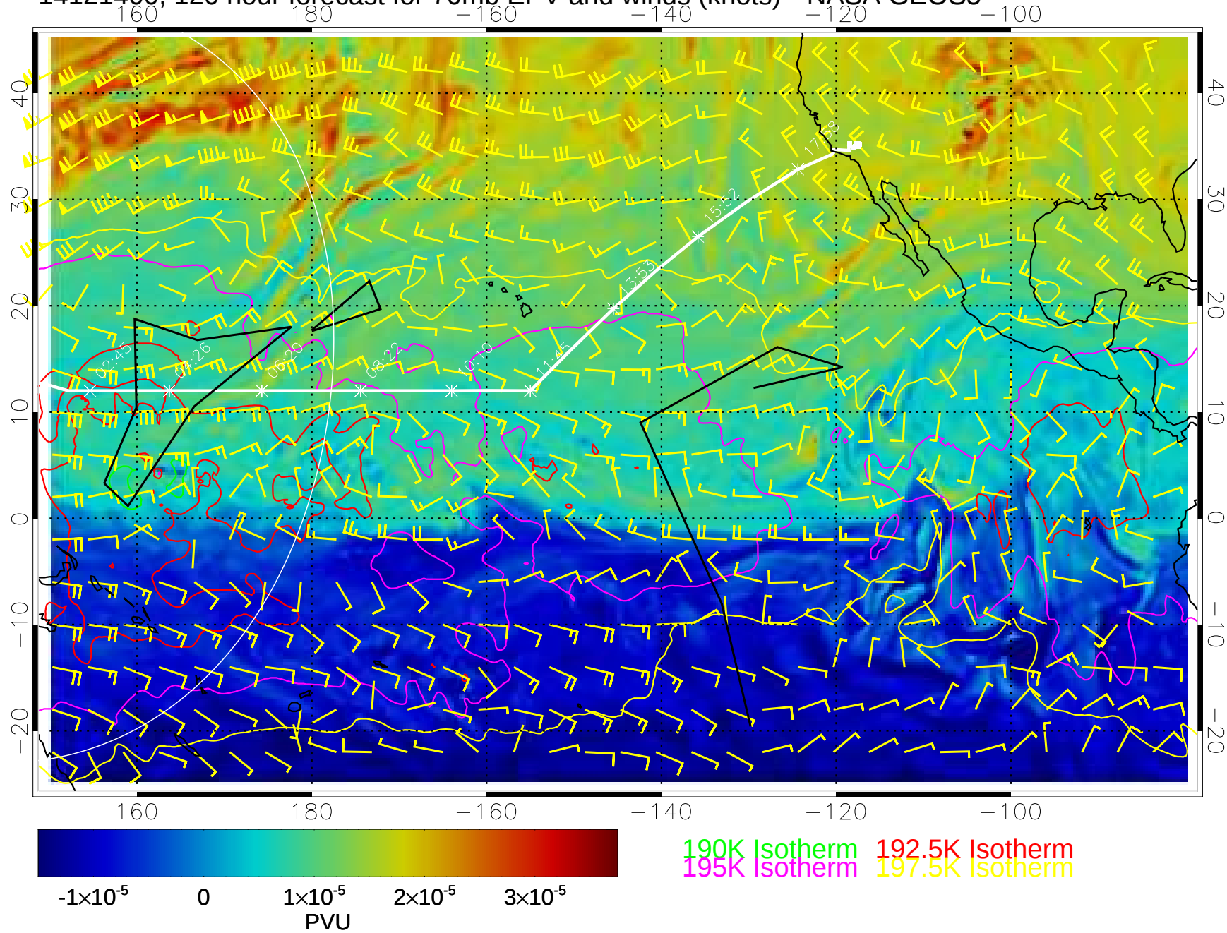
14121400, 120 hour forecast for 70mb EPV and winds (knots)-- NASA GEOS5
