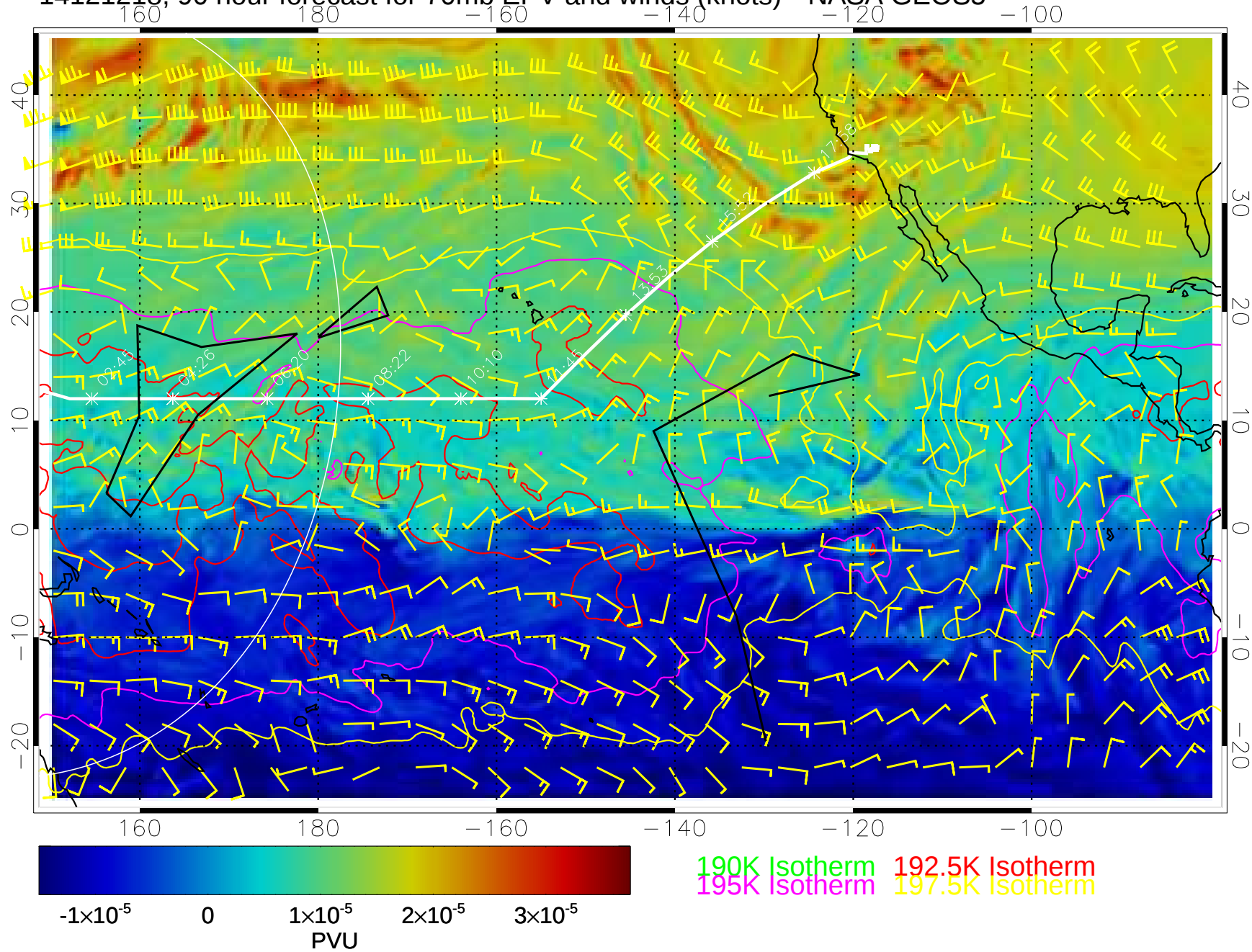
14121218, 90 hour forecast for 70mb EPV and winds (knots)-- NASA GEOS5
