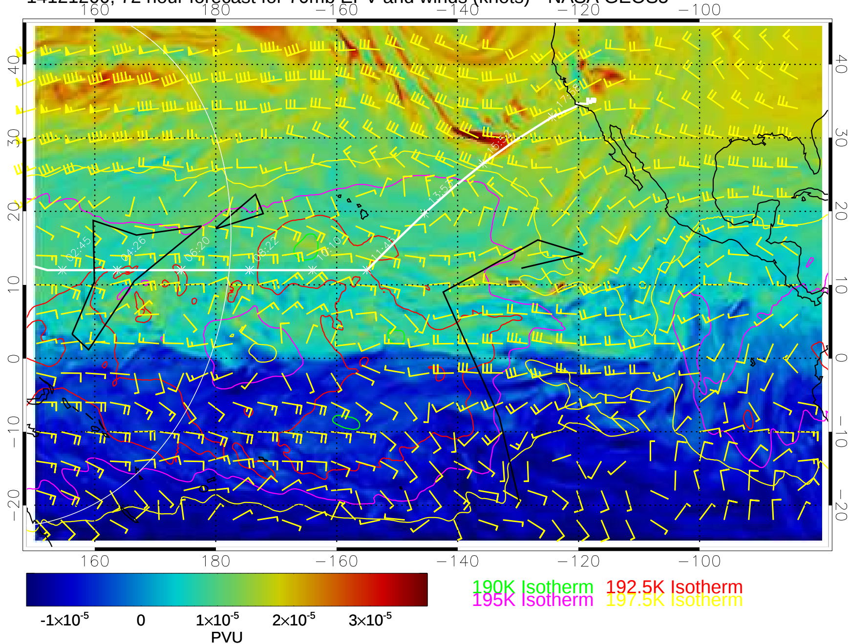
14121200, 72 hour forecast for 70mb EPV and winds (knots)-- NASA GEOS5
