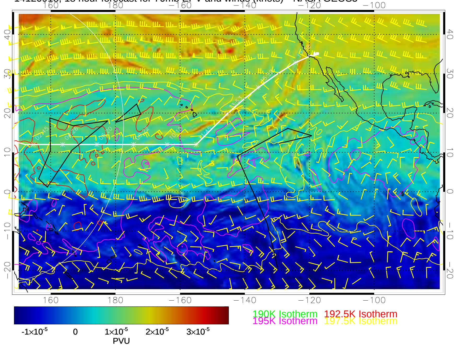
14120918, 18 hour forecast for 70mb EPV and winds (knots)-- NASA GEOS5
