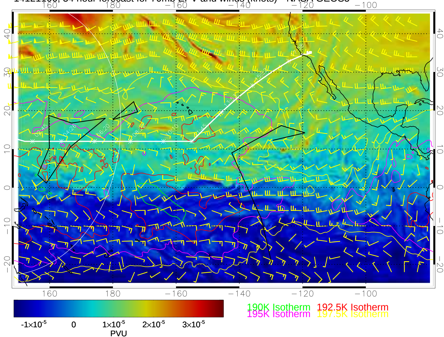
14121106, 54 hour forecast for 70mb EPV and winds (knots)-- NASA GEOS5
