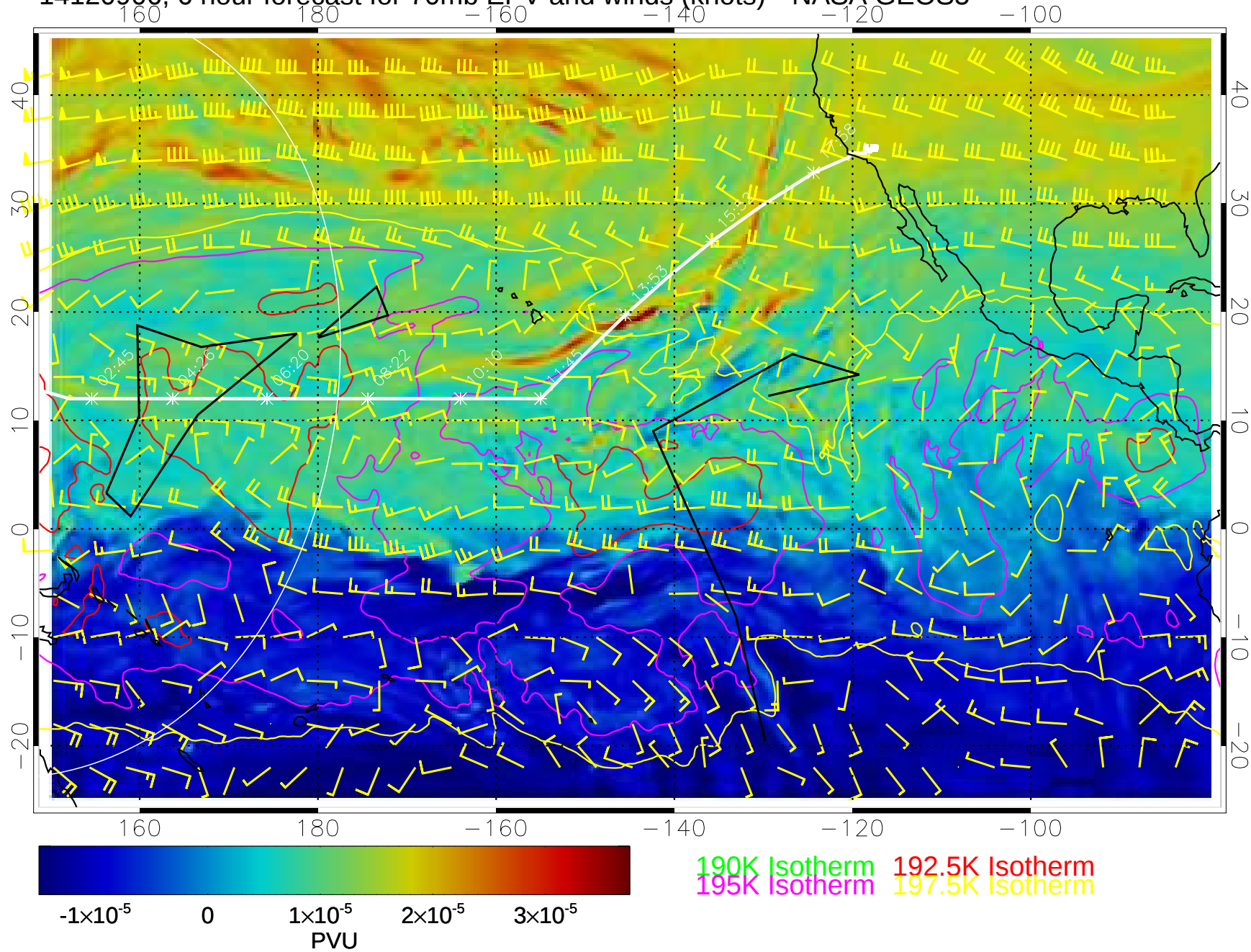
14120906, 6 hour forecast for 70mb EPV and winds (knots)-- NASA GEOS5
