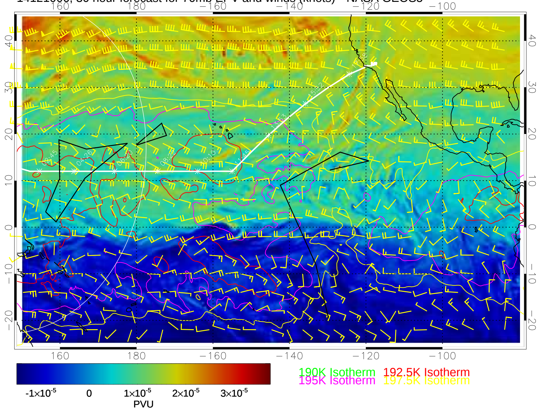
14121006, 30 hour forecast for 70mb EPV and winds (knots)-- NASA GEOS5
