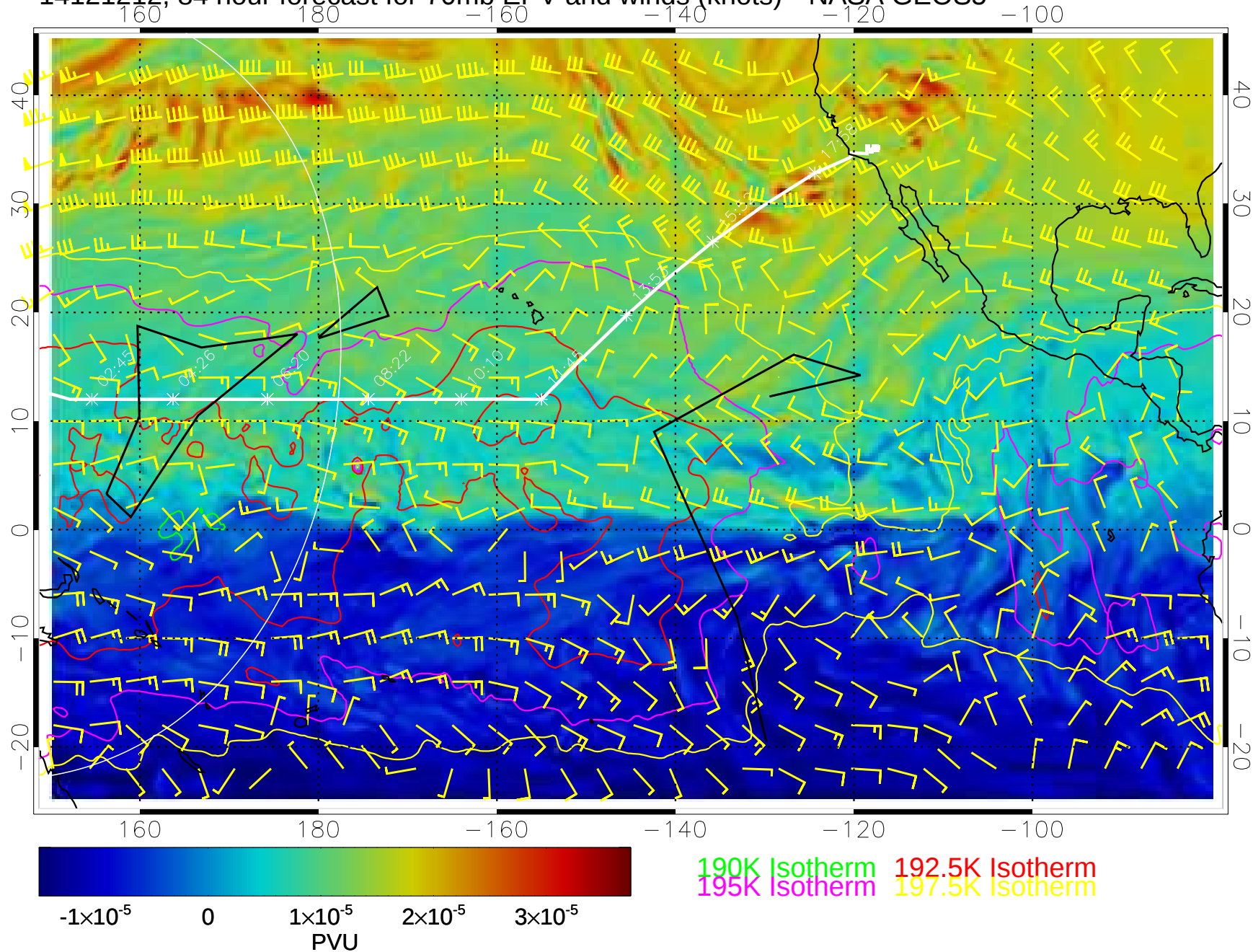
14121212, 84 hour forecast for 70mb EPV and winds (knots)-- NASA GEOS5
