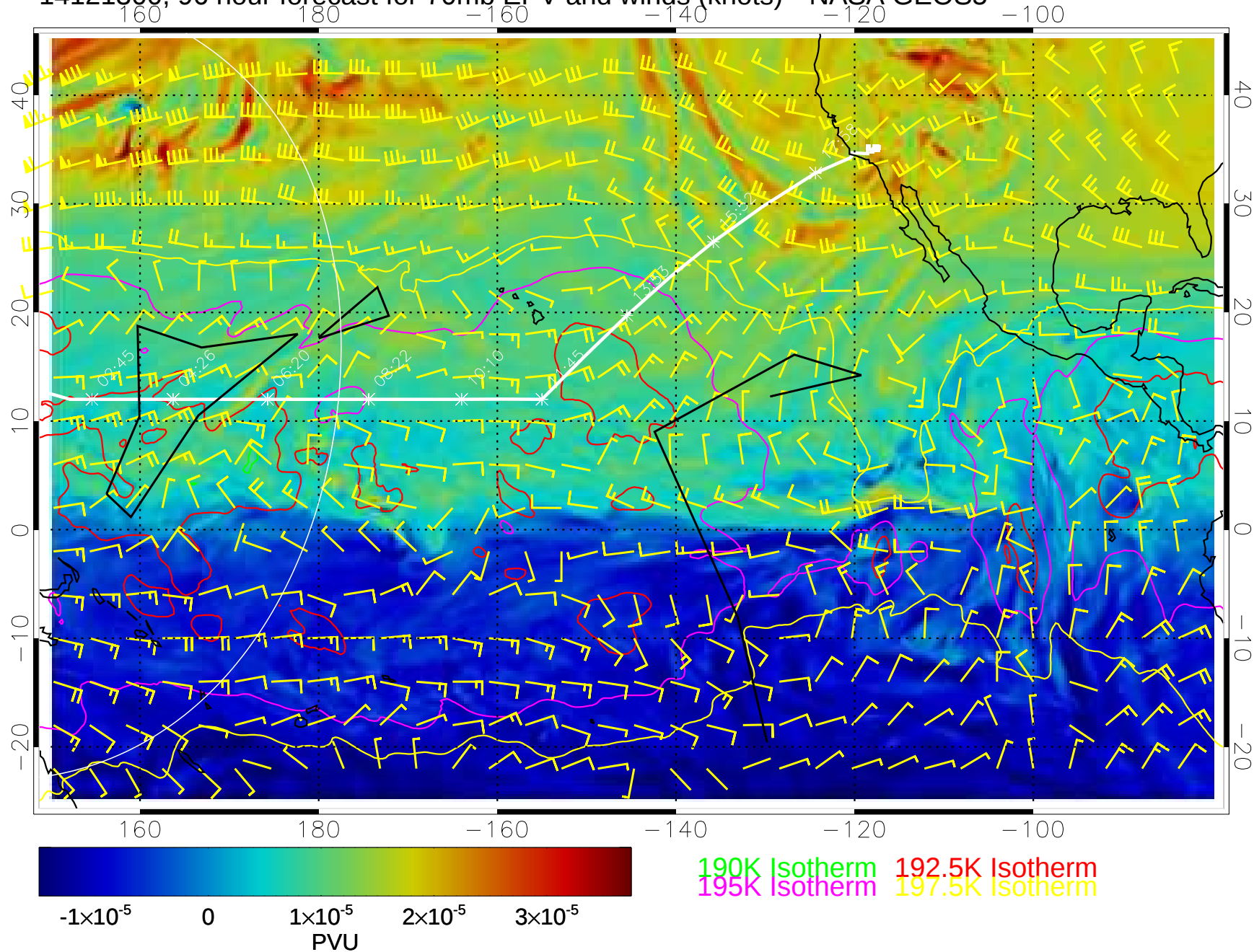
14121300, 96 hour forecast for 70mb EPV and winds (knots)-- NASA GEOS5
