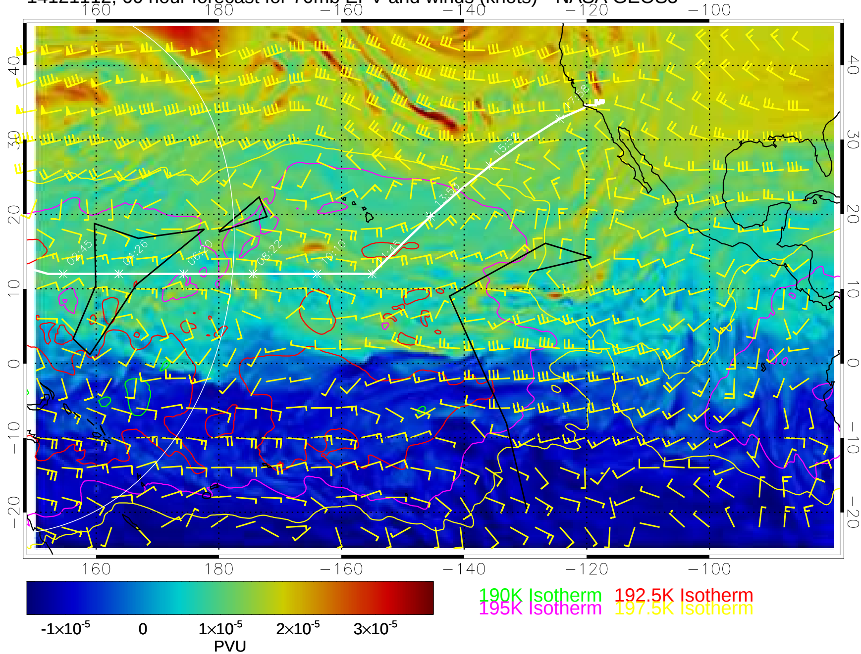
14121112, 60 hour forecast for 70mb EPV and winds (knots)-- NASA GEOS5
