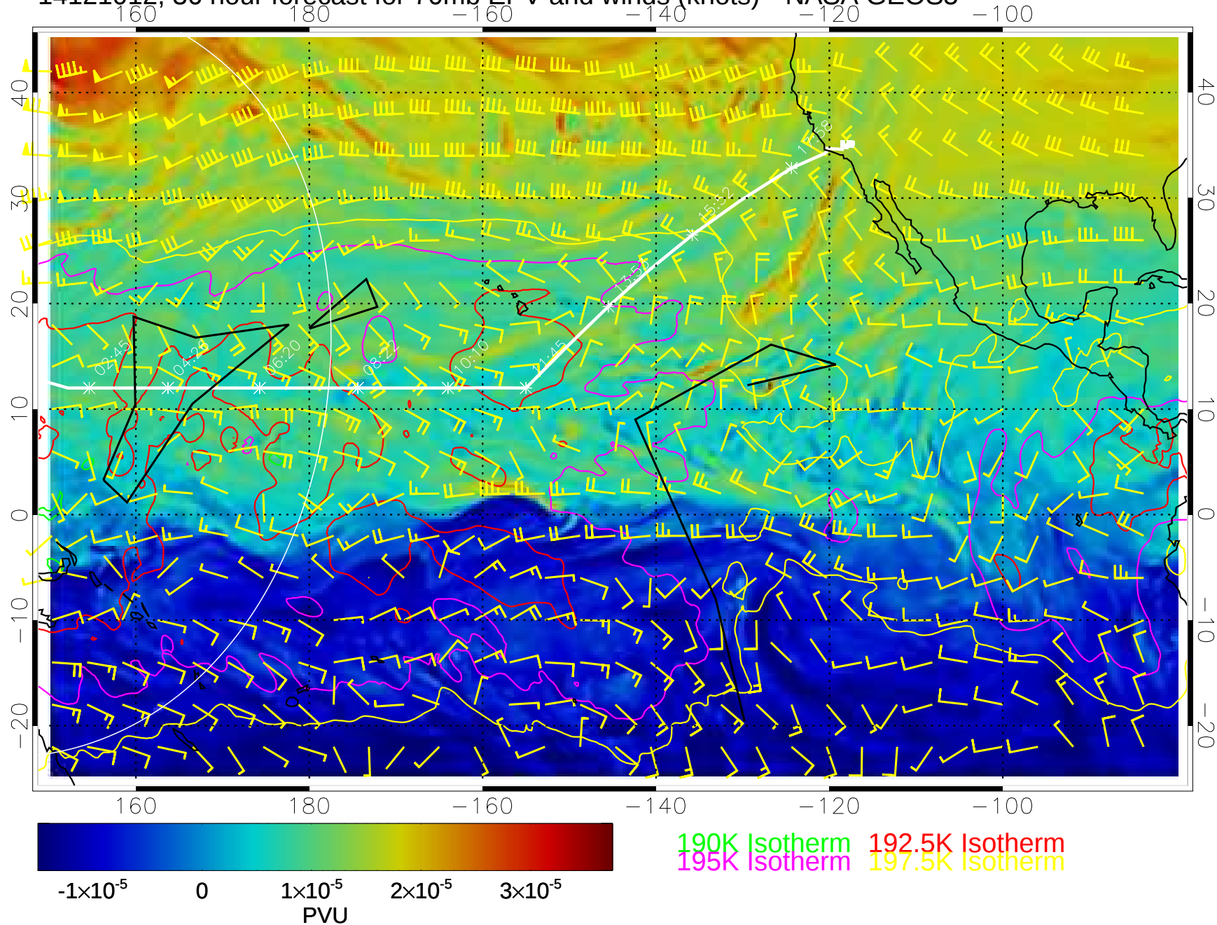
14121012, 36 hour forecast for 70mb EPV and winds (knots)-- NASA GEOS5
