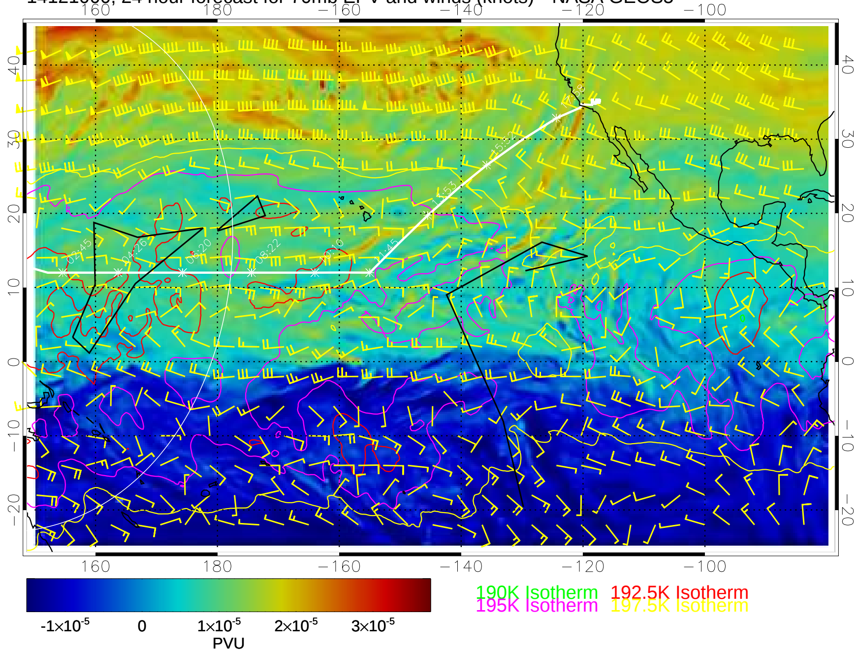
14121000, 24 hour forecast for 70mb EPV and winds (knots)-- NASA GEOS5
