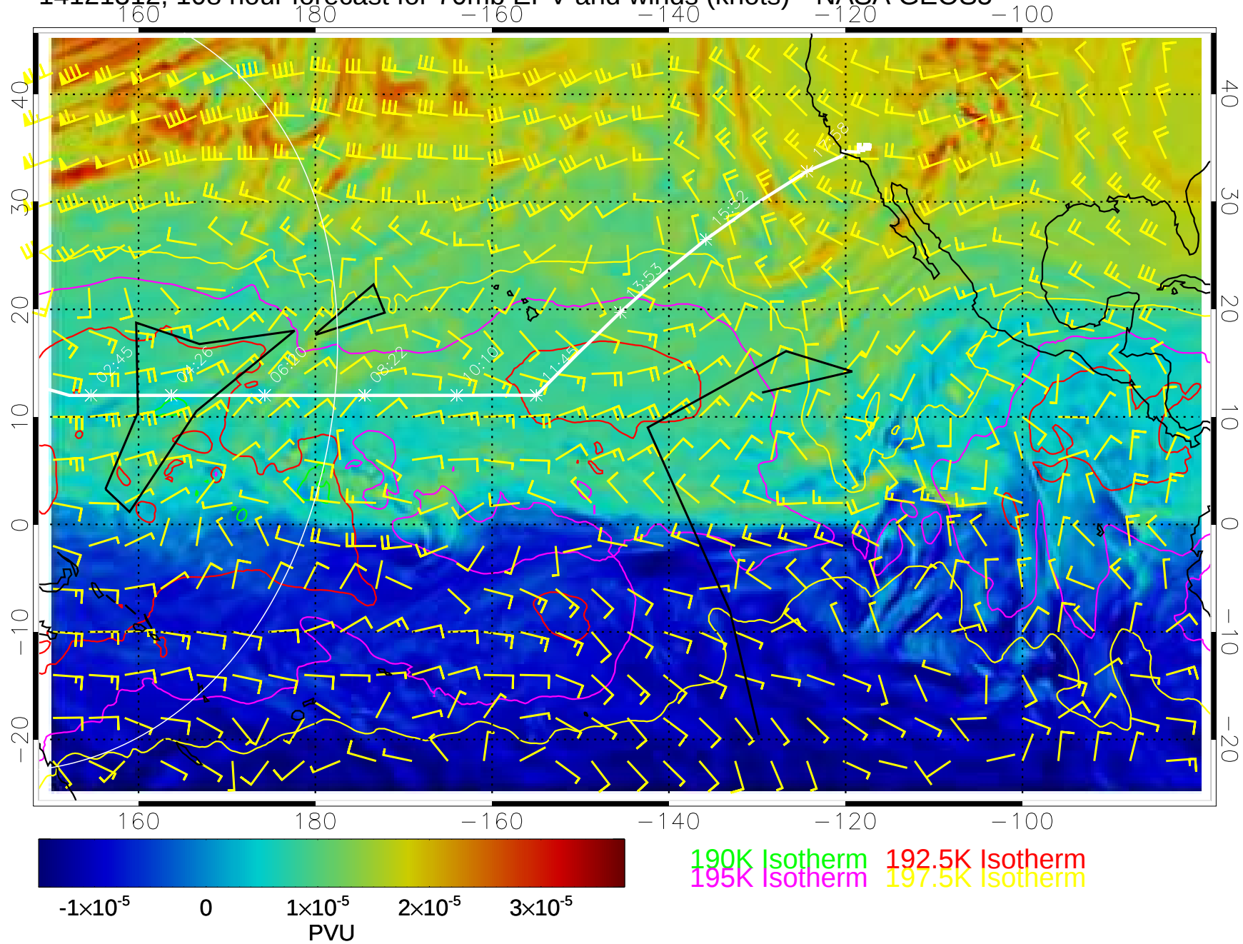
14121312, 108 hour forecast for 70mb EPV and winds (knots)-- NASA GEOS5
