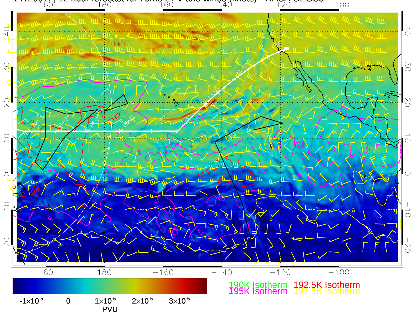
14120912, 12 hour forecast for 70mb EPV and winds (knots)-- NASA GEOS5
