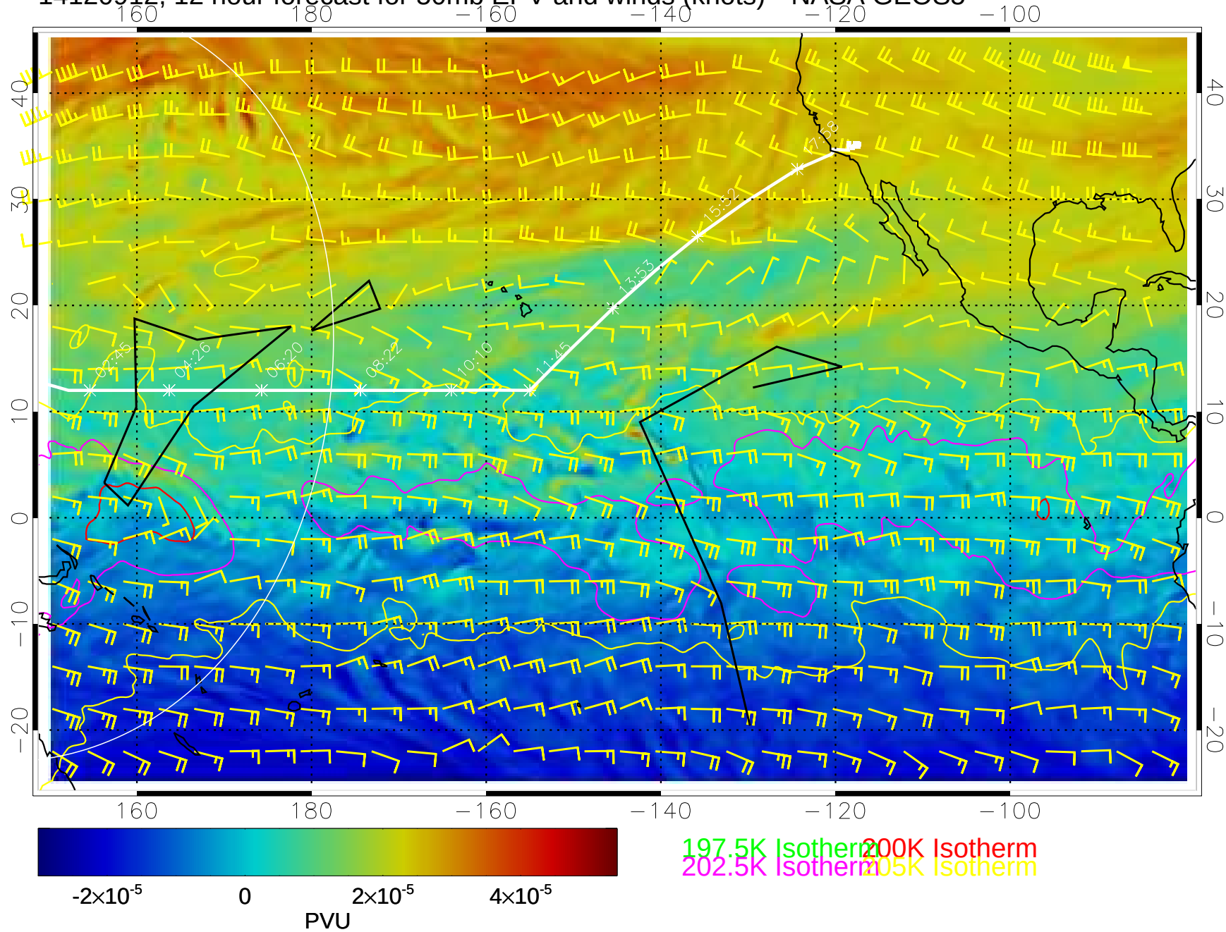
14120912, 12 hour forecast for 50mb EPV and winds (knots)-- NASA GEOS5
