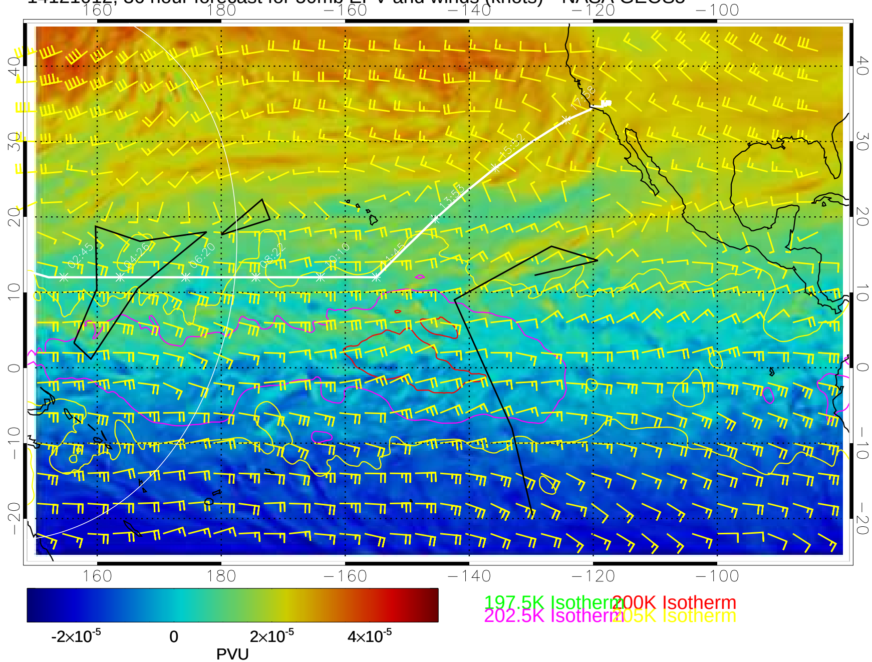
14121012, 36 hour forecast for 50mb EPV and winds (knots)-- NASA GEOS5
