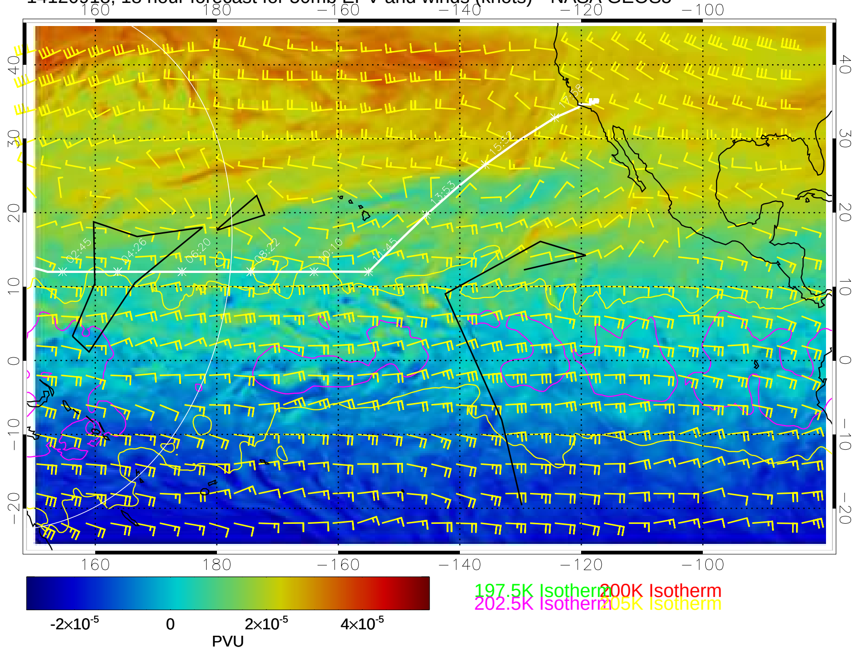
14120918, 18 hour forecast for 50mb EPV and winds (knots)-- NASA GEOS5
