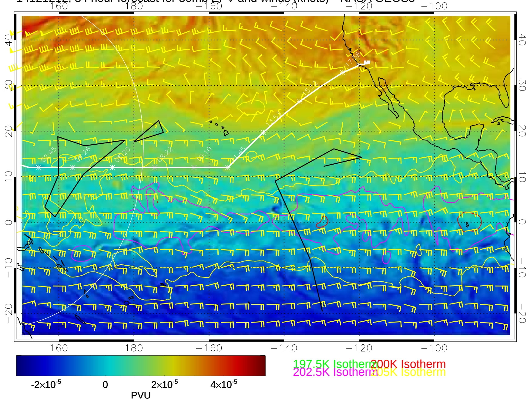
14121212, 84 hour forecast for 50mb EPV and winds (knots)-- NASA GEOS5
