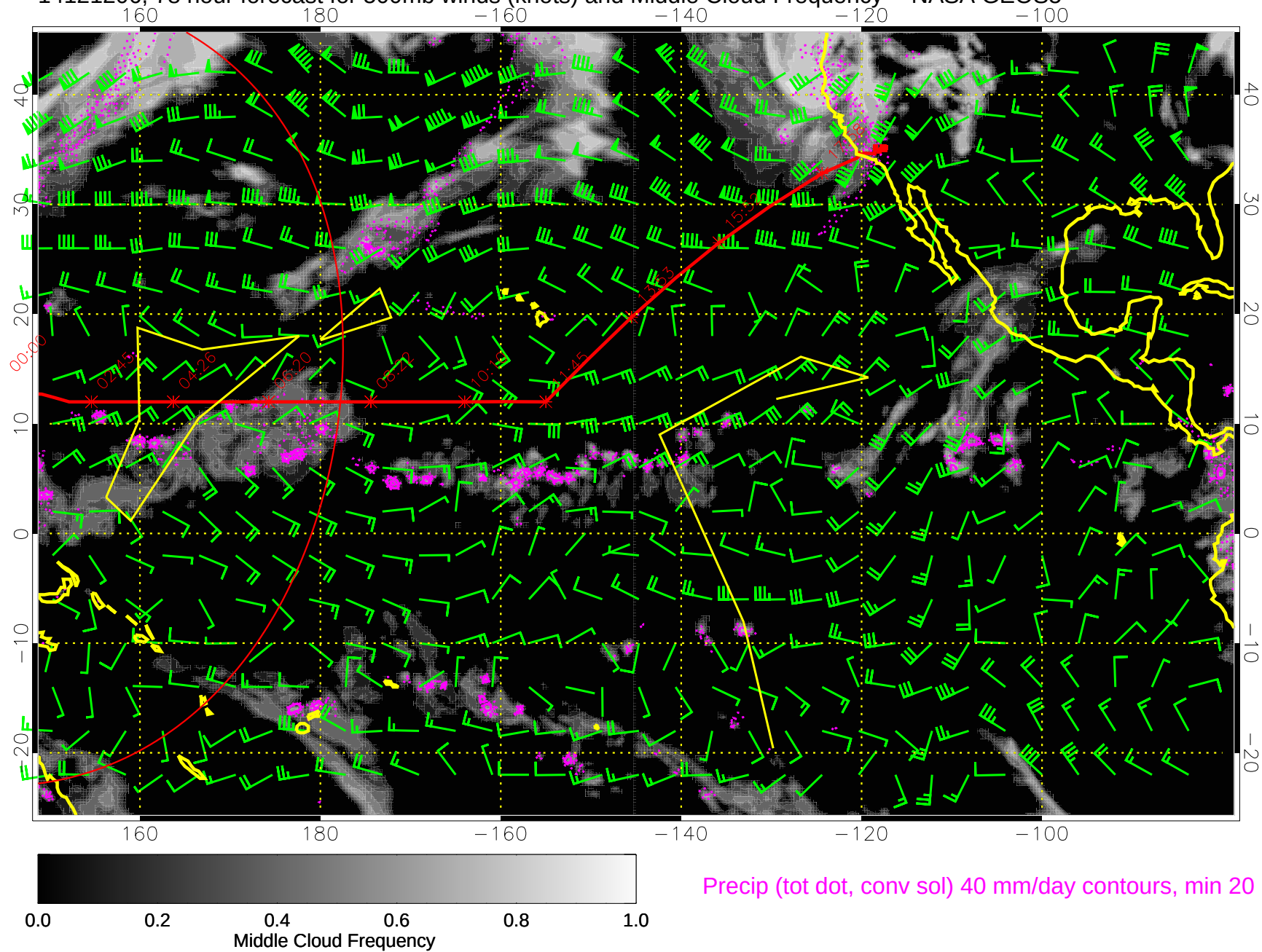
14121206, 78 hour forecast for 500mb winds (knots) and Middle Cloud Frequency -- NASA GEOS5
