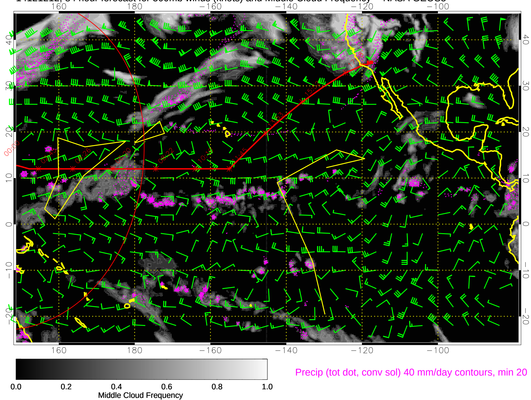
14121212, 84 hour forecast for 500mb winds (knots) and Middle Cloud Frequency -- NASA GEOS5
