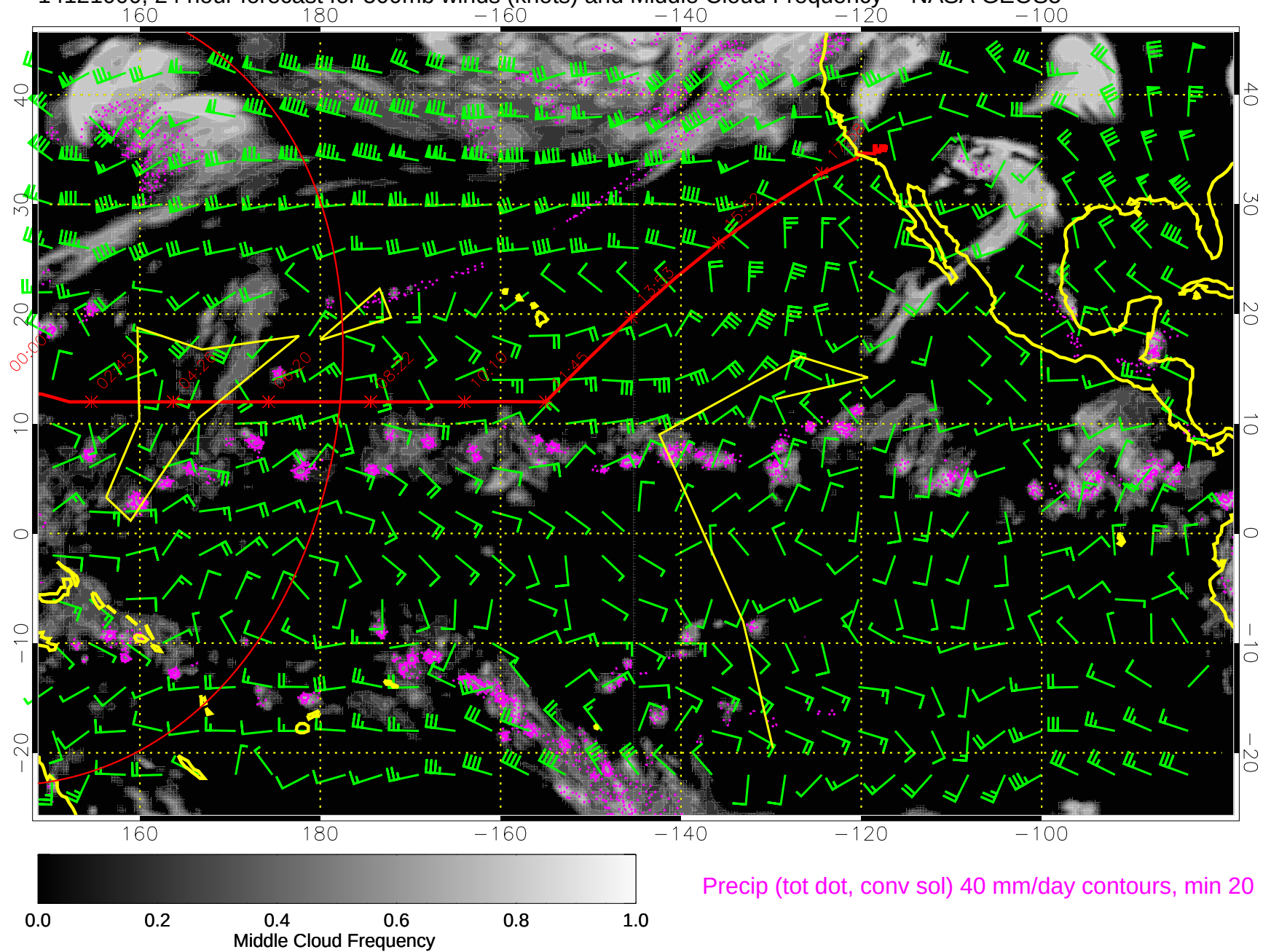
14121000, 24 hour forecast for 500mb winds (knots) and Middle Cloud Frequency -- NASA GEOS5
