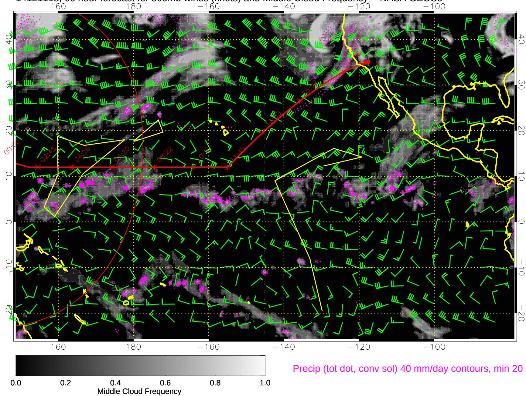
14121118, 66 hour forecast for 500mb winds (knots) and Middle Cloud Frequency -- NASA GEOS5
