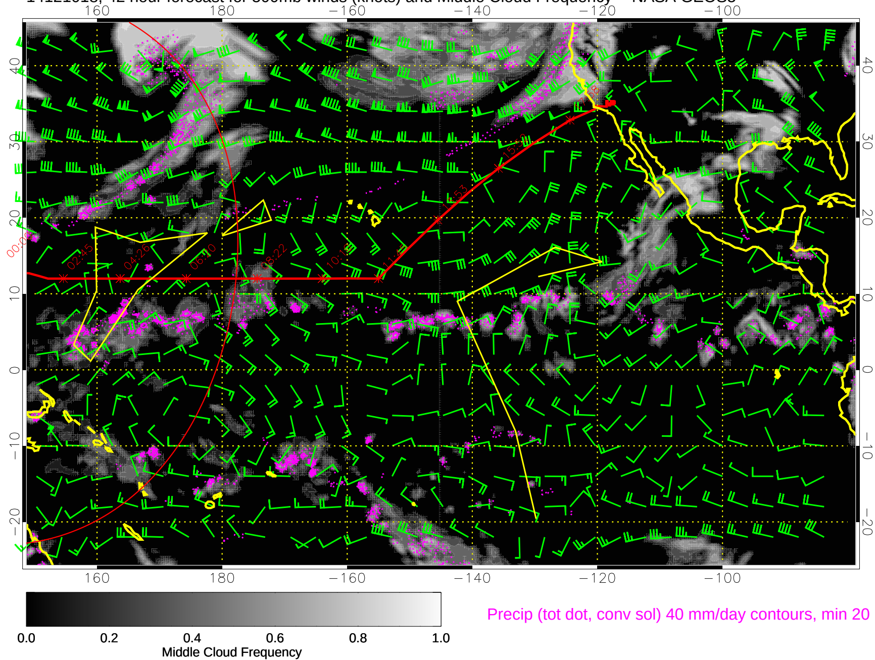
14121018, 42 hour forecast for 500mb winds (knots) and Middle Cloud Frequency -- NASA GEOS5
