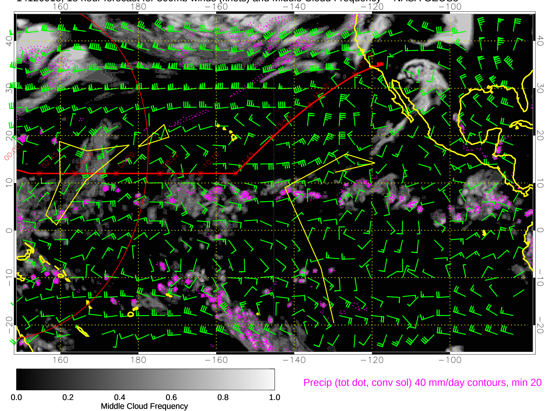
14120918, 18 hour forecast for 500mb winds (knots) and Middle Cloud Frequency -- NASA GEOS5
