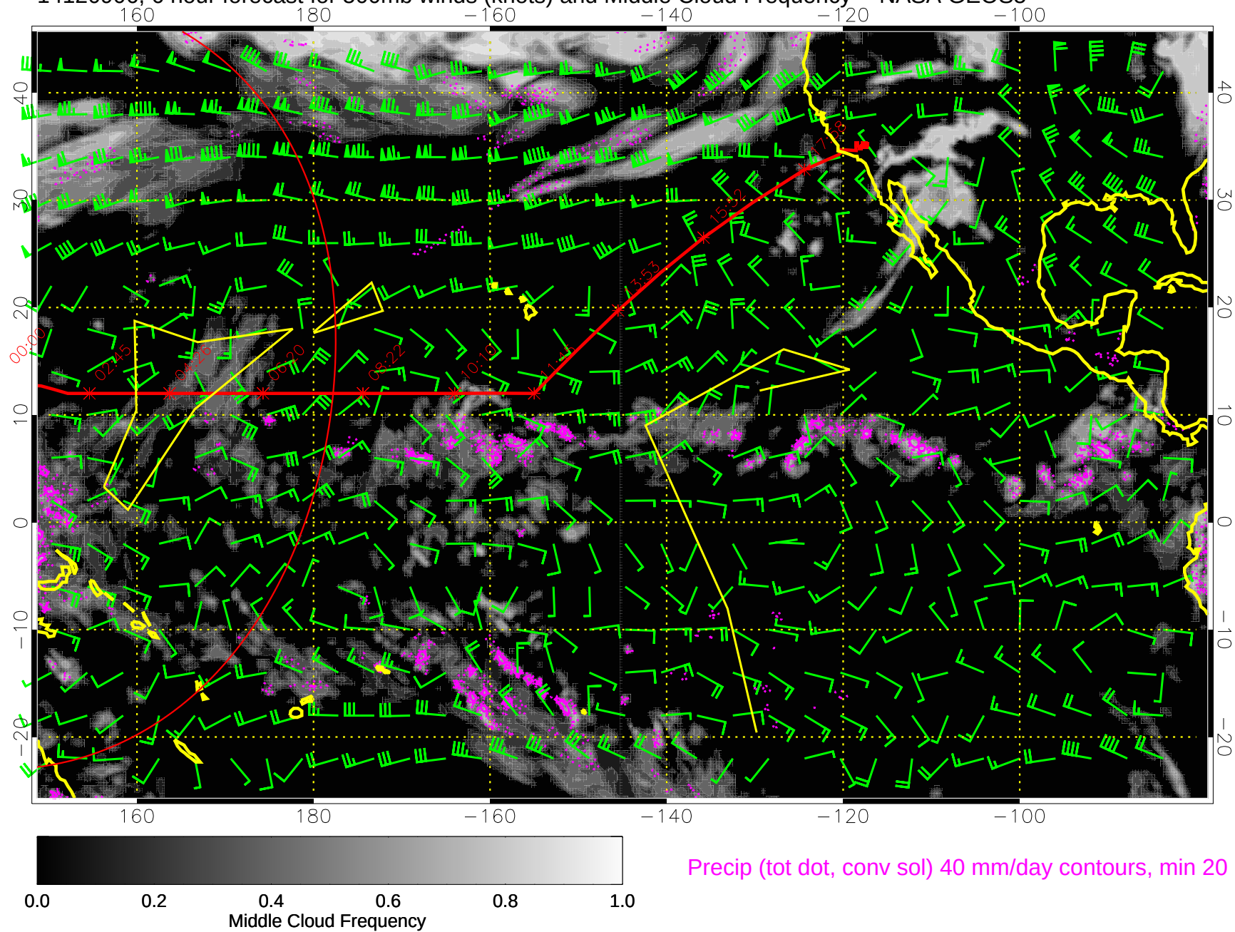
14120906, 6 hour forecast for 500mb winds (knots) and Middle Cloud Frequency -- NASA GEOS5
