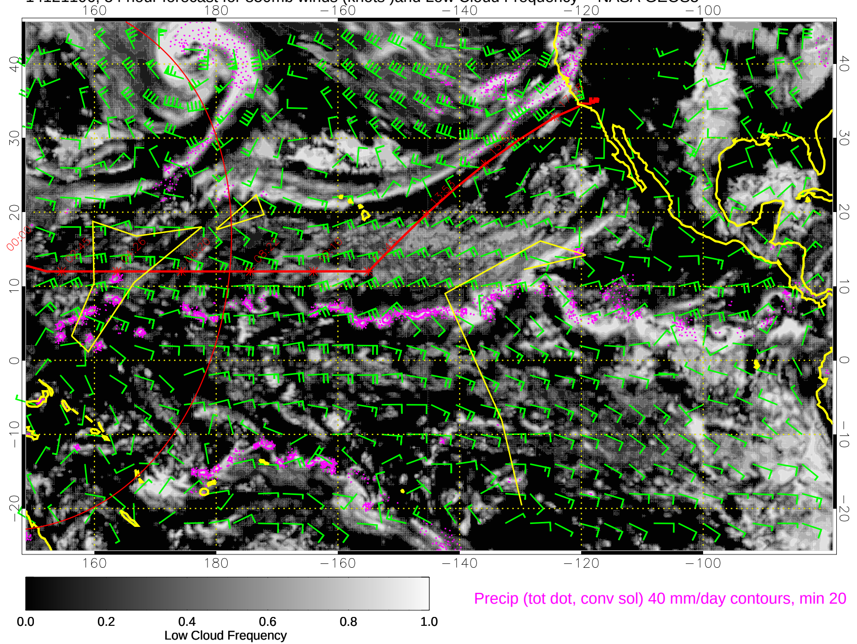
14121106, 54 hour forecast for 850mb winds (knots) and Low Cloud Frequency -- NASA GEOS5
