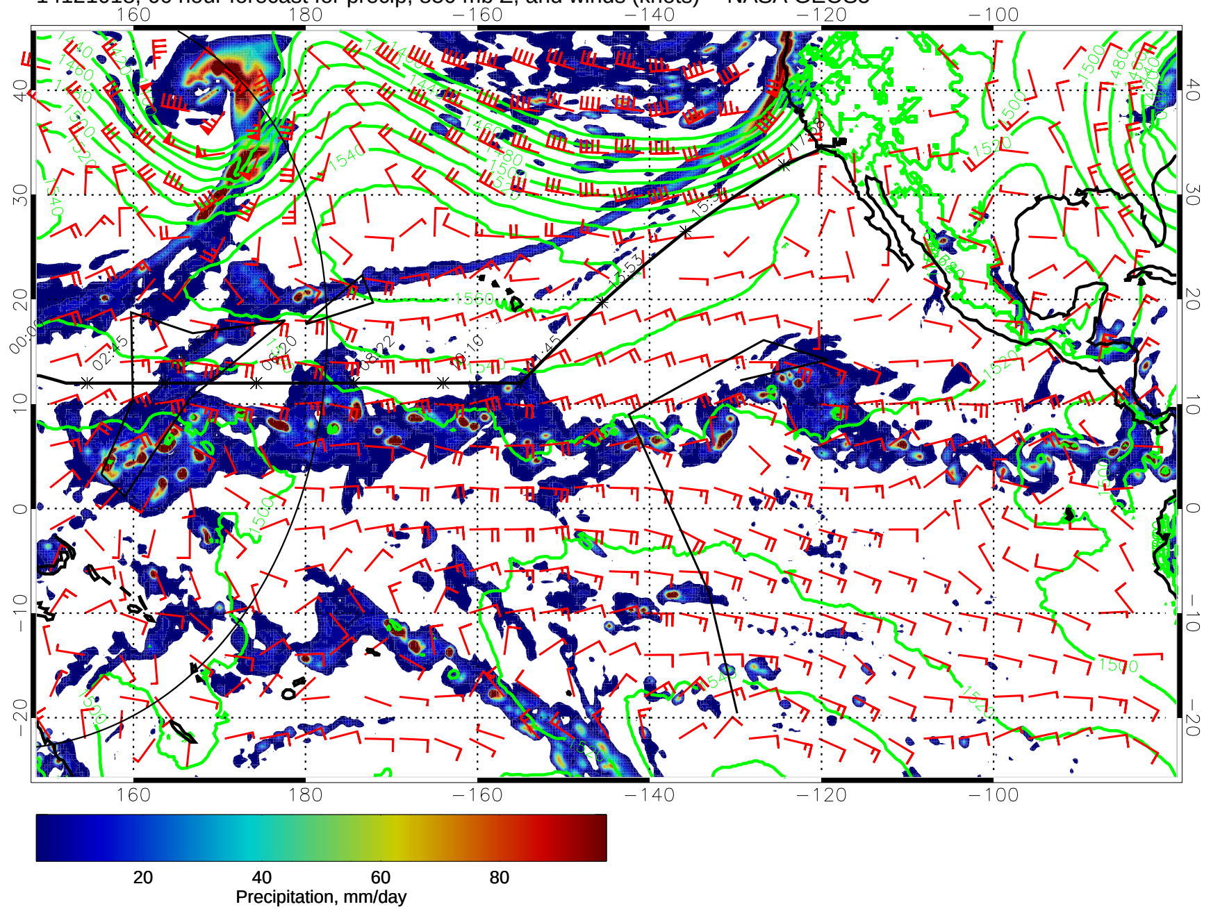
14121018, 66 hour forecast for precip, 850 mb Z, and winds (knots) -- NASA GEOS5
