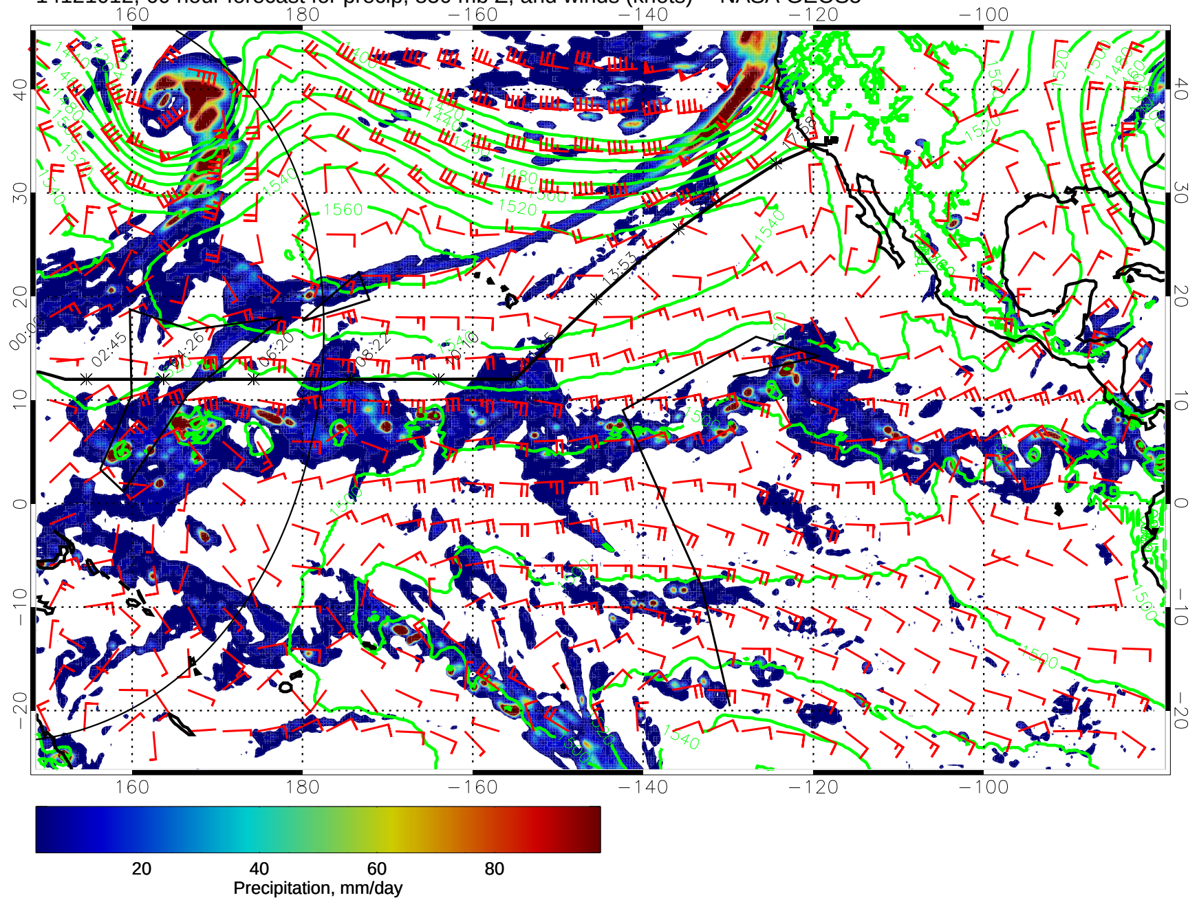
14121012, 60 hour forecast for precip, 850 mb Z, and winds (knots) -- NASA GEOS5
