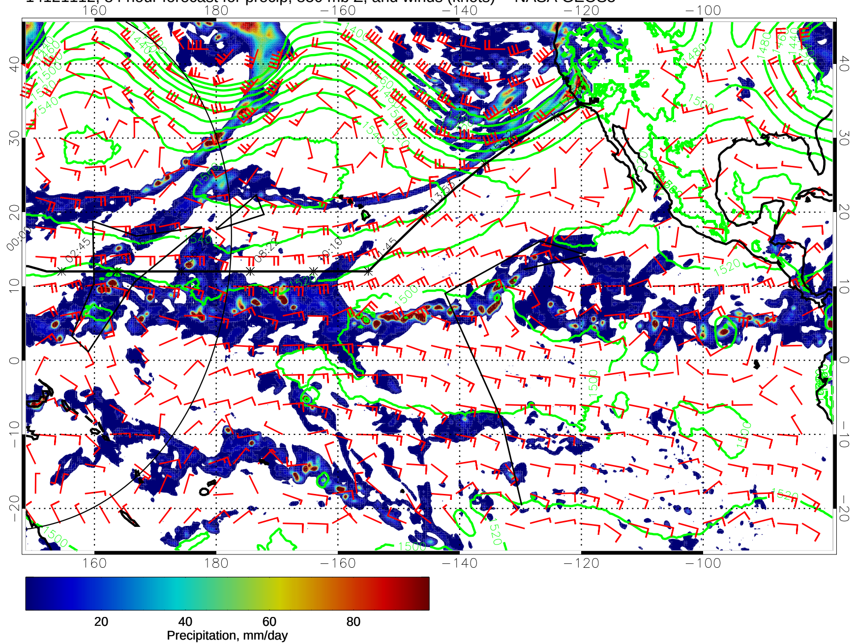
14121112, 84 hour forecast for precip, 850 mb Z, and winds (knots) -- NASA GEOS5
