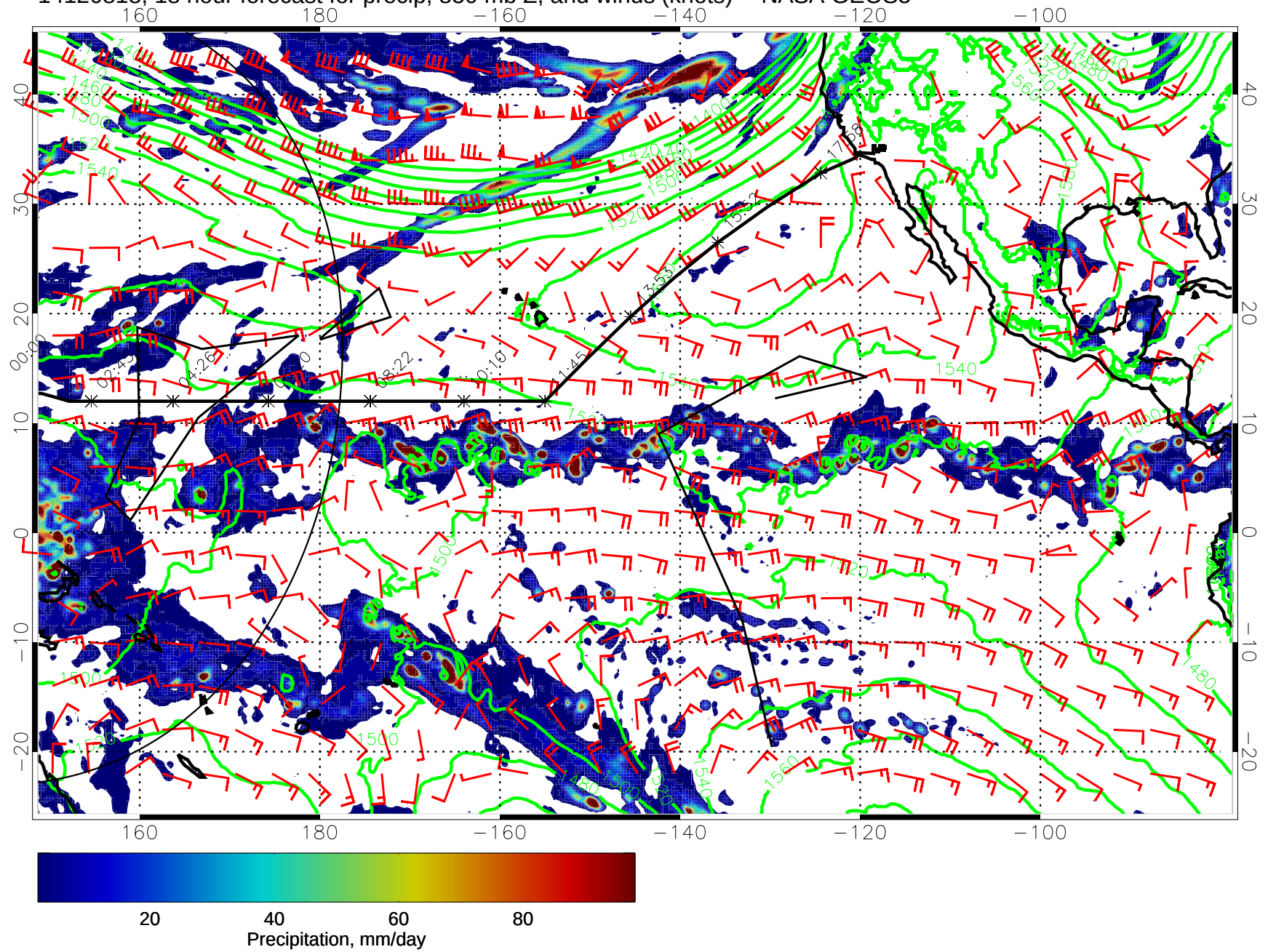
14120818, 18 hour forecast for precip, 850 mb Z, and winds (knots) -- NASA GEOS5
