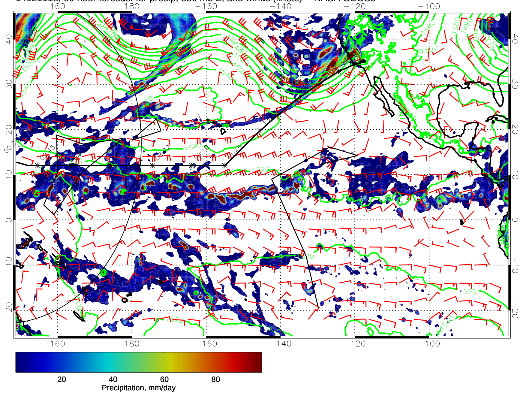
14121118, 90 hour forecast for precip, 850 mb Z, and winds (knots) -- NASA GEOS5
