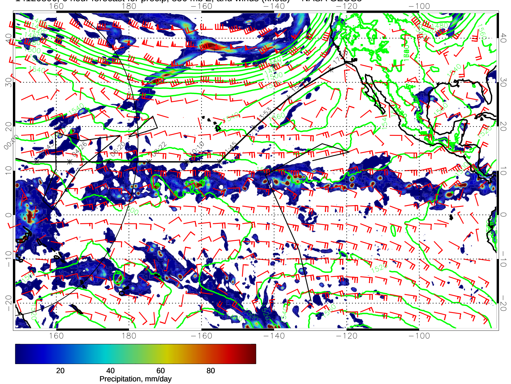
14120806, 6 hour forecast for precip, 850 mb Z, and winds (knots) -- NASA GEOS5
