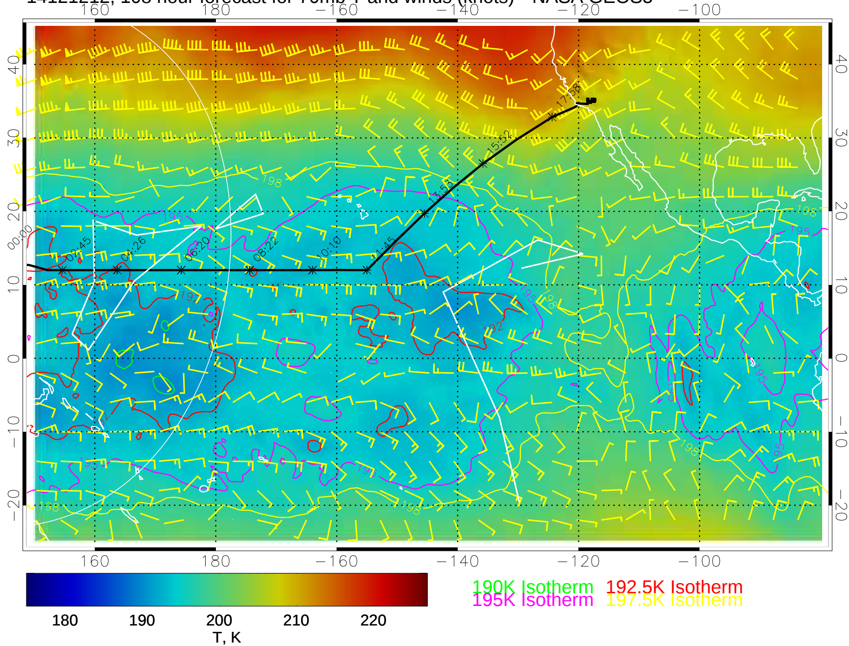
14121212, 108 hour forecast for 70mb T and winds (knots)-- NASA GEOS5
