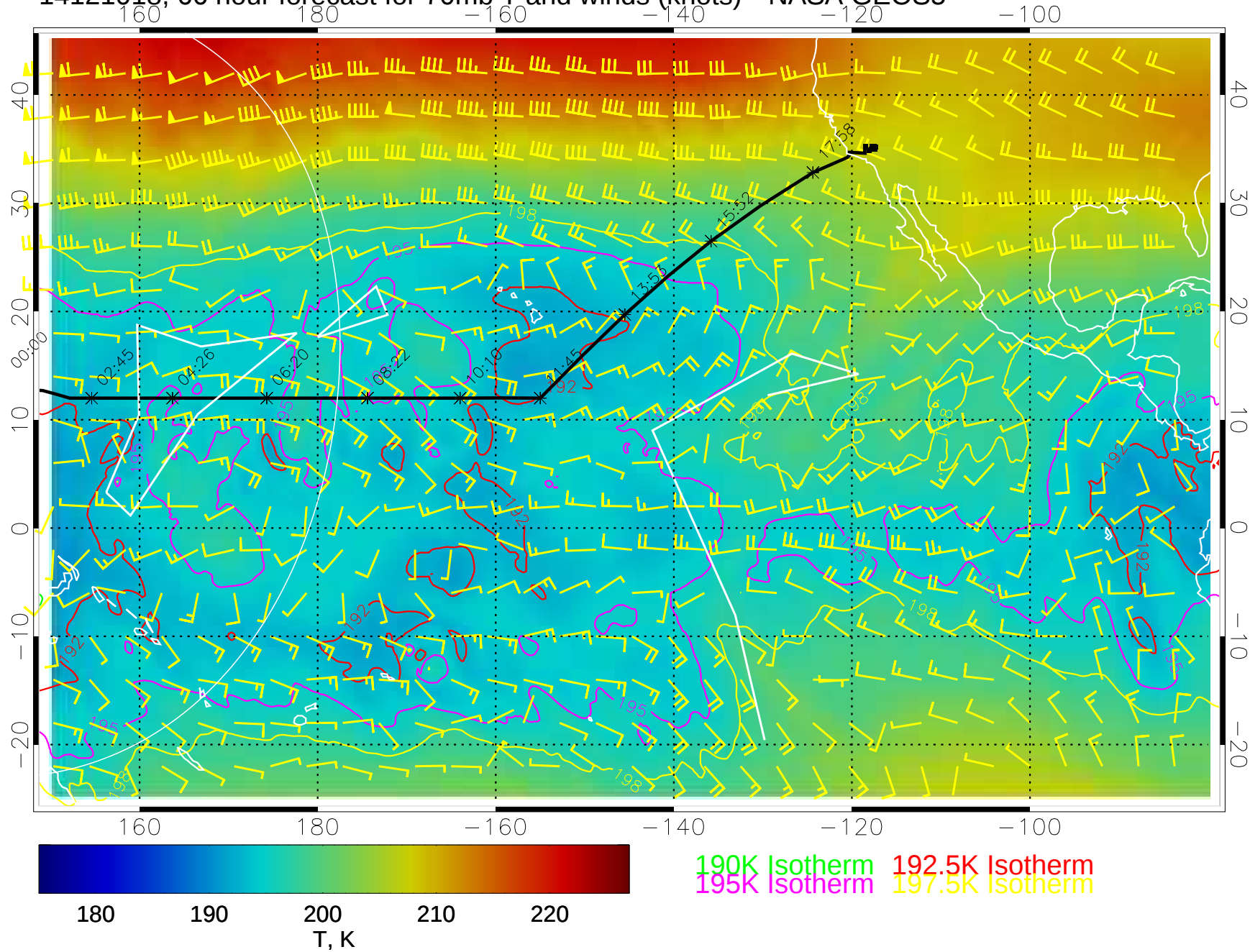
14121018, 66 hour forecast for 70mb T and winds (knots)-- NASA GEOS5
