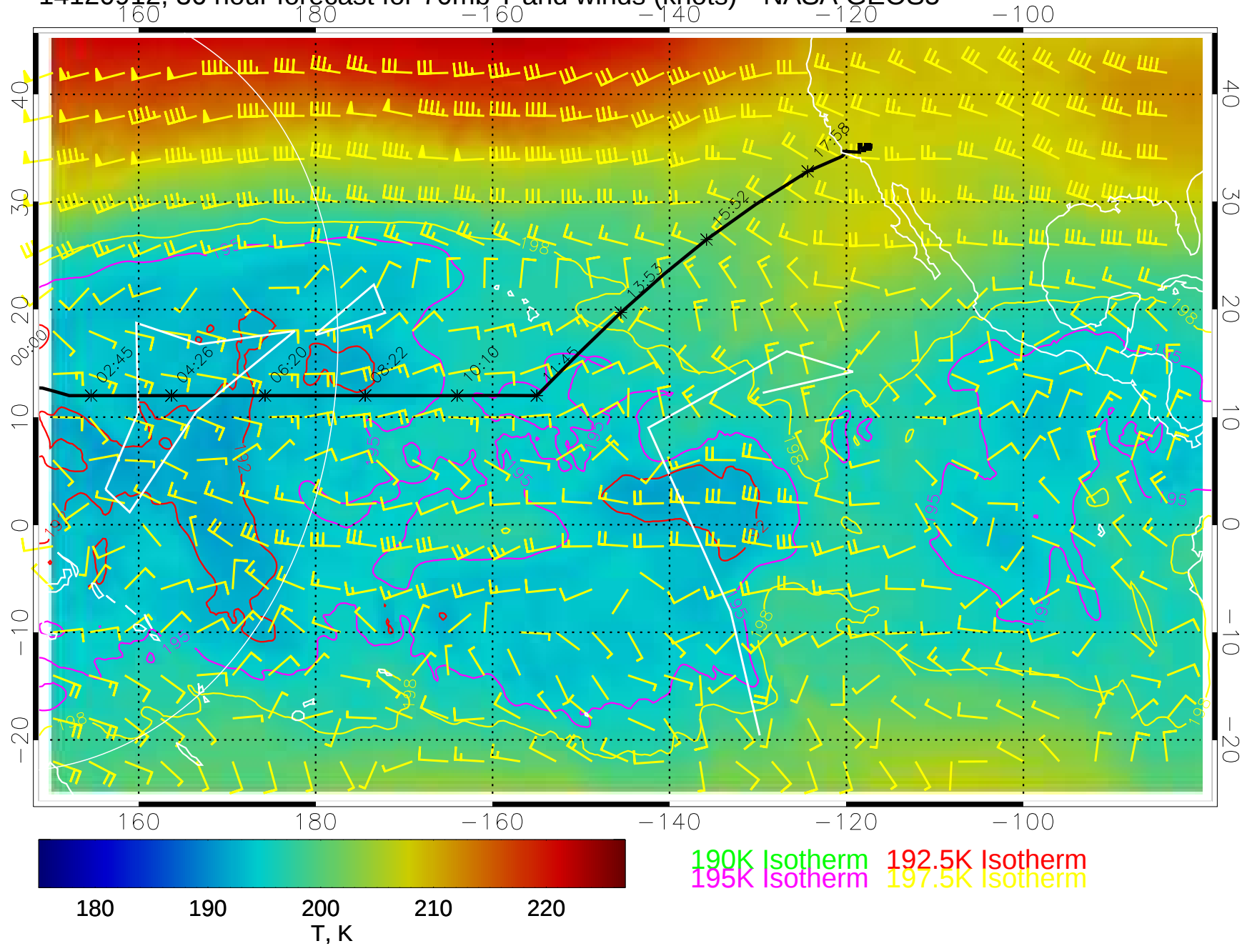
14120912, 36 hour forecast for 70mb T and winds (knots)-- NASA GEOS5
