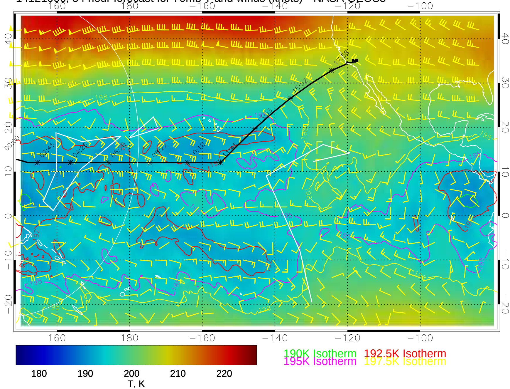
14121006, 54 hour forecast for 70mb T and winds (knots)-- NASA GEOS5
