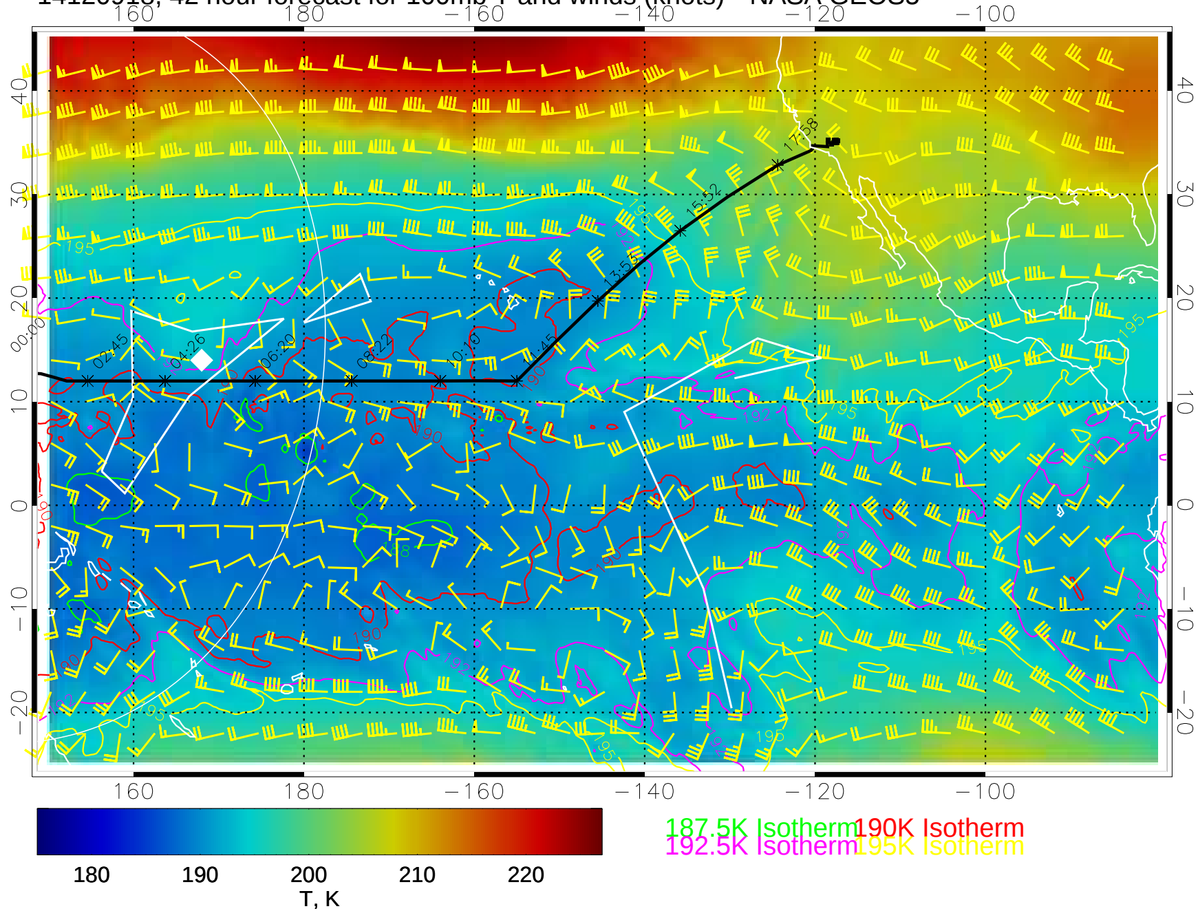
14120918, 42 hour forecast for 100mb T and winds (knots)-- NASA GEOS5
