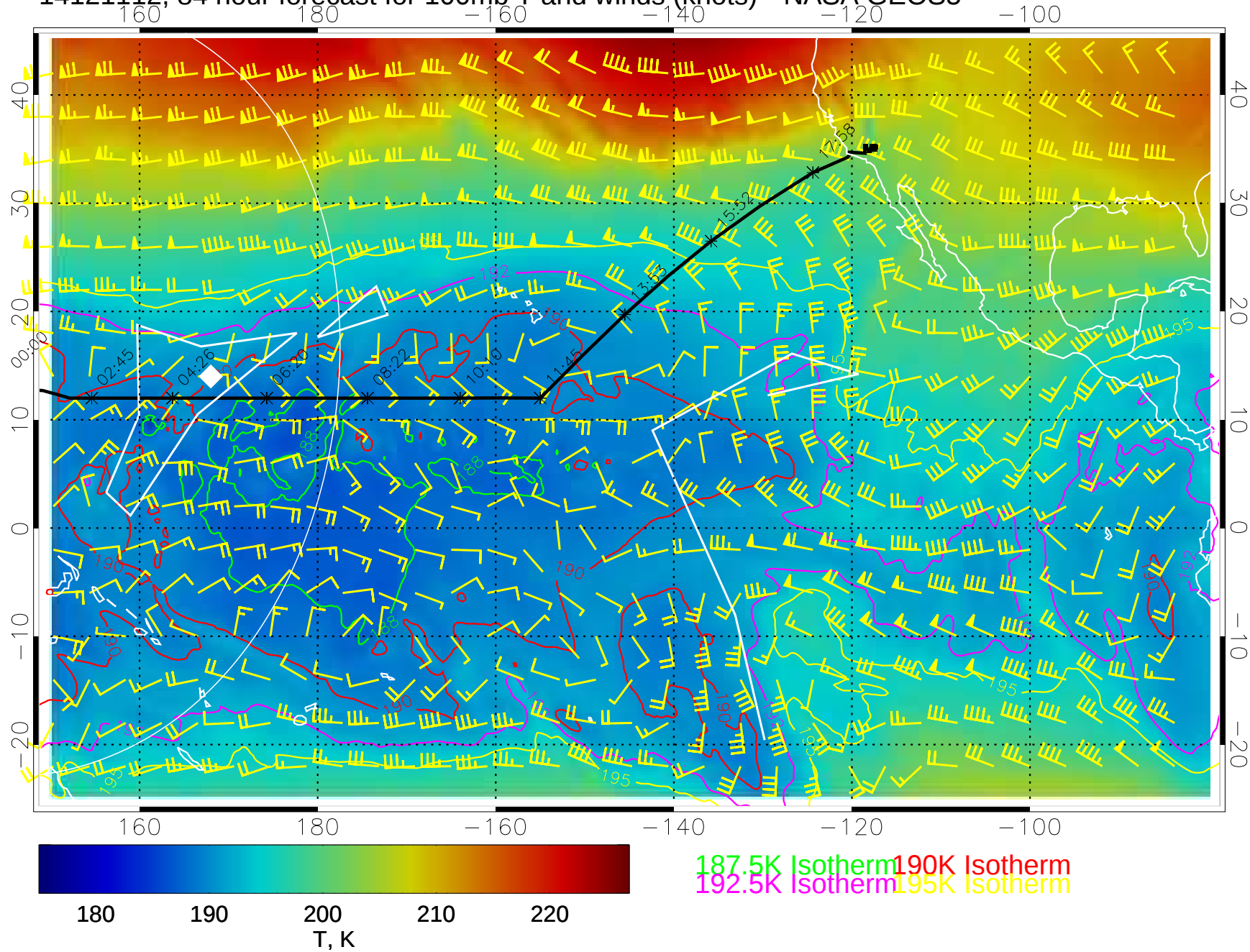
14121112, 84 hour forecast for 100mb T and winds (knots)-- NASA GEOS5
