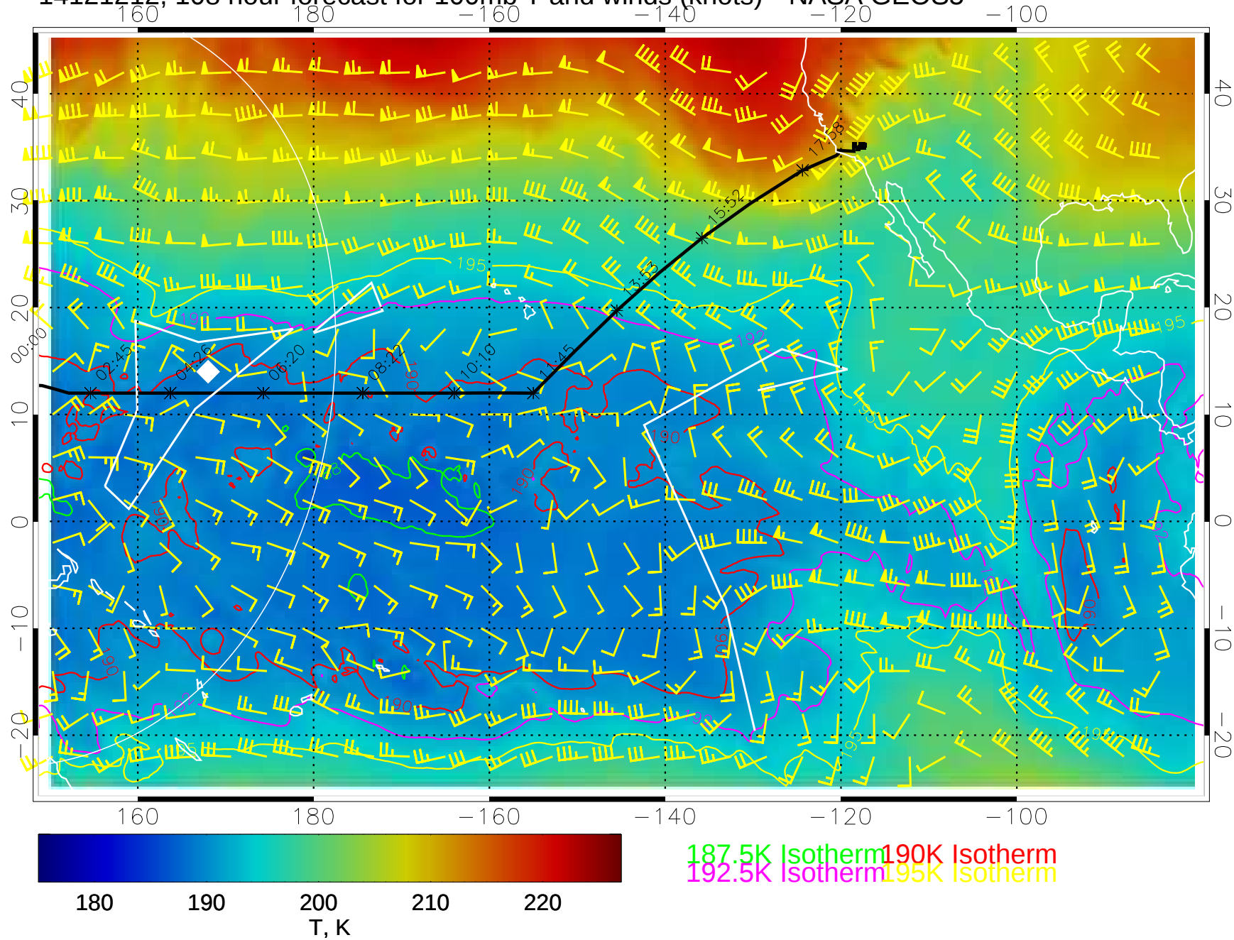
14121212, 108 hour forecast for 100mb T and winds (knots)-- NASA GEOS5
