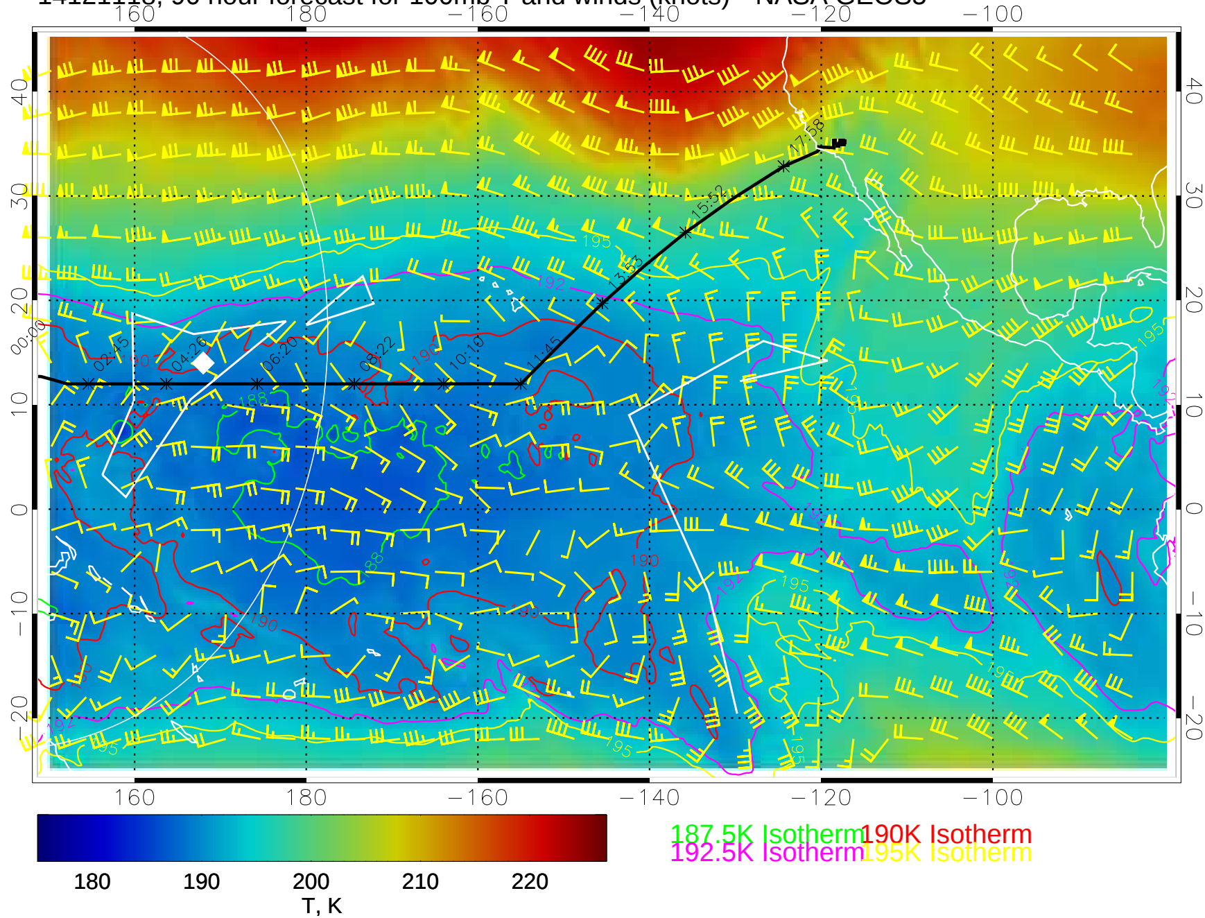
14121118, 90 hour forecast for 100mb T and winds (knots)-- NASA GEOS5
