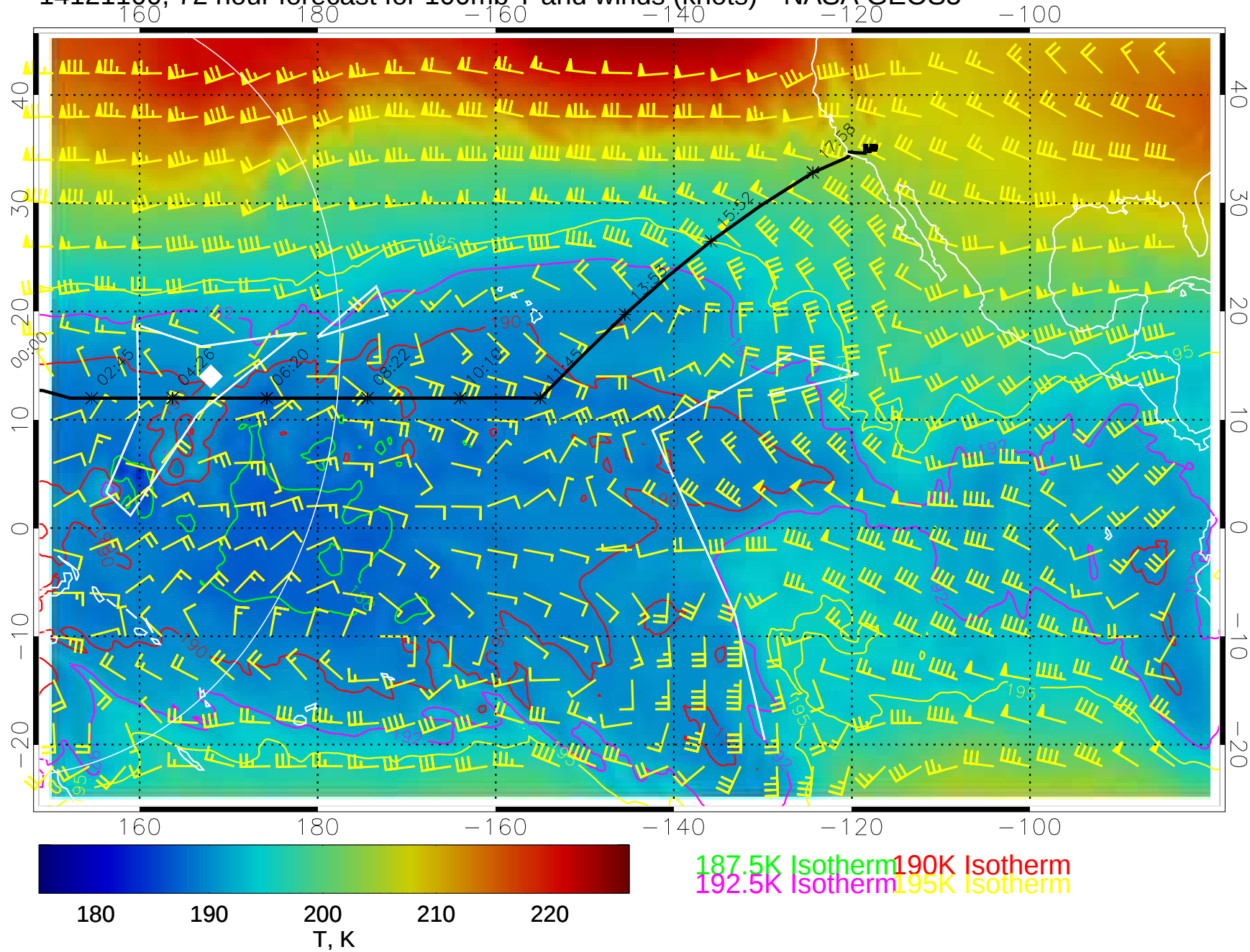
14121100, 72 hour forecast for 100mb T and winds (knots)-- NASA GEOS5
