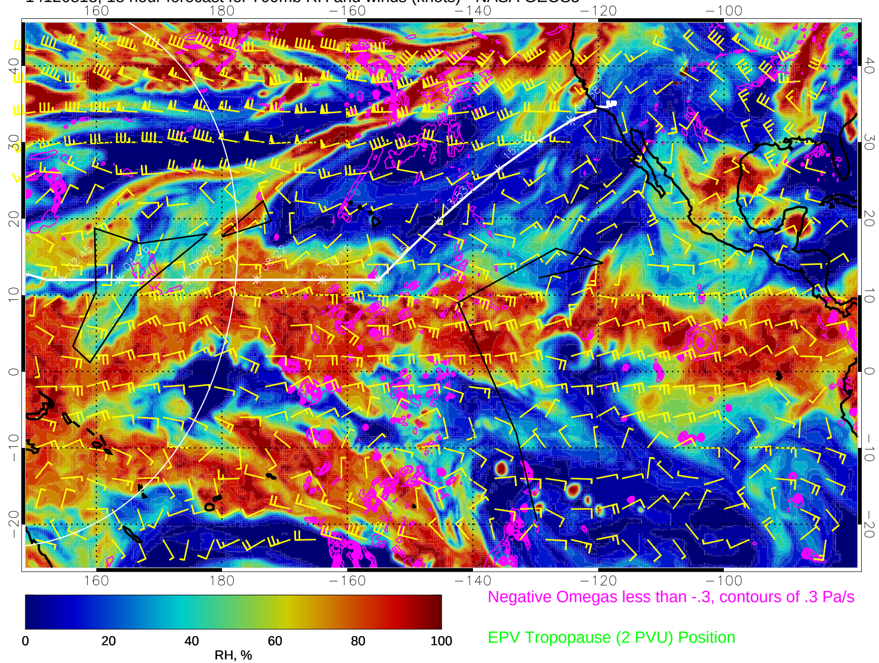
14120818, 18 hour forecast for 700mb RH and winds (knots) - NASA GEOS5
