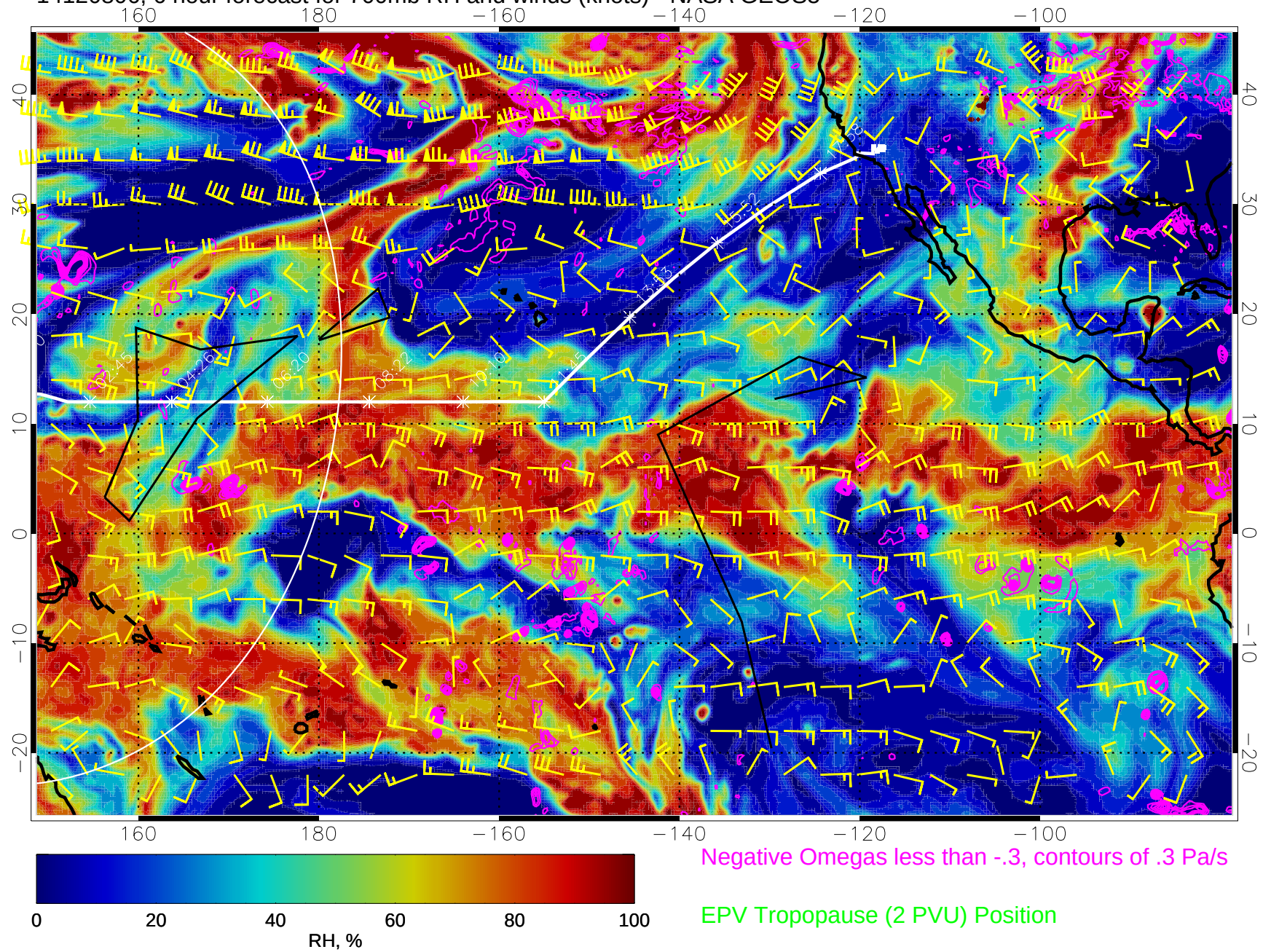
14120806, 6 hour forecast for 700mb RH and winds (knots) - NASA GEOS5
