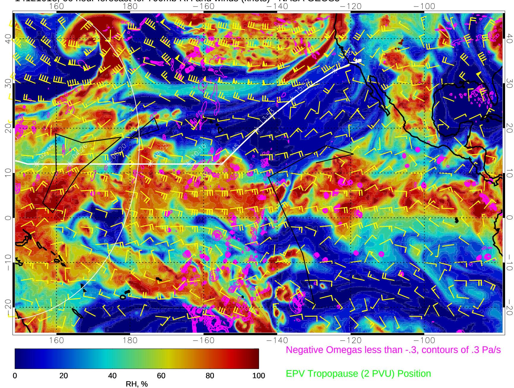
14121018, 66 hour forecast for 700mb RH and winds (knots) - NASA GEOS5
