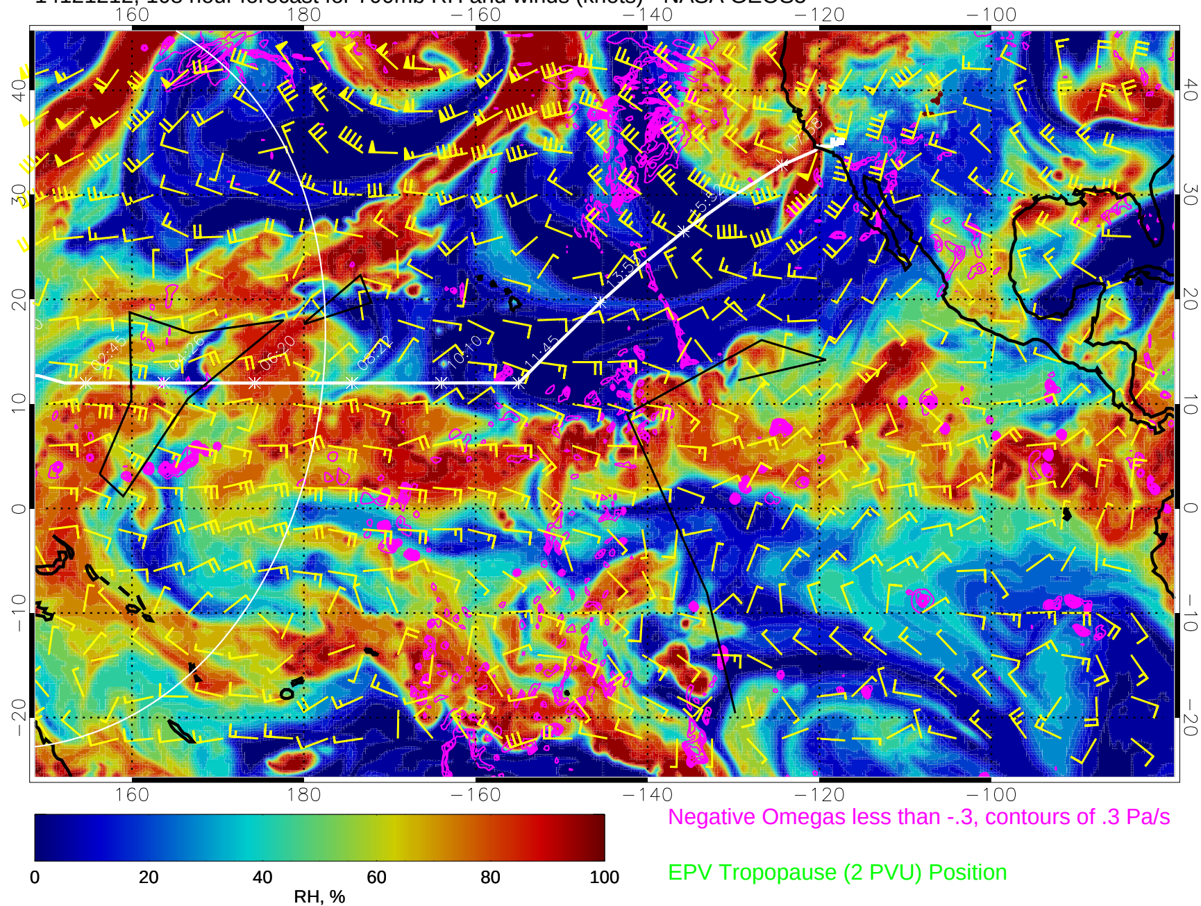
14121212, 108 hour forecast for 700mb RH and winds (knots) - NASA GEOS5
