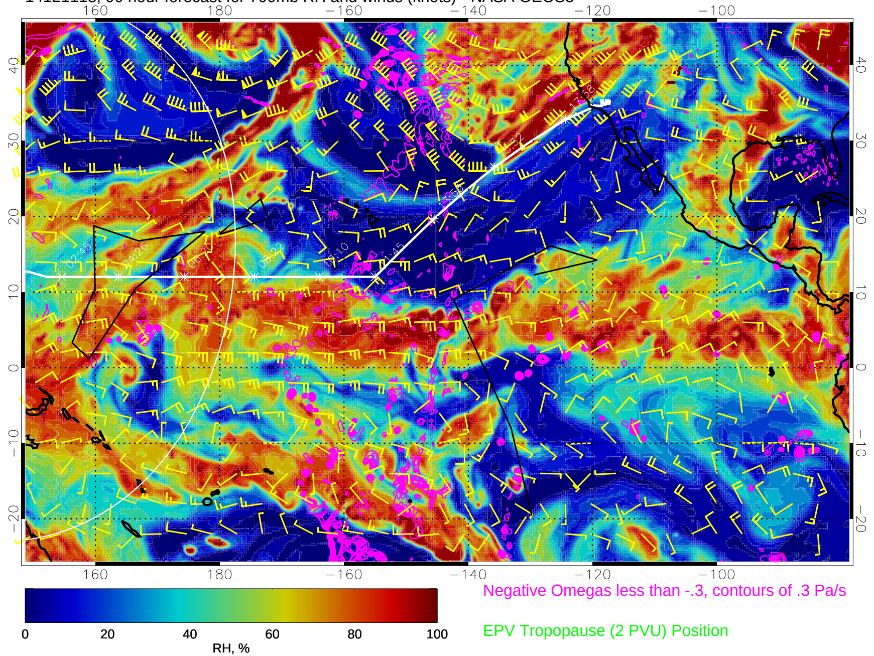
14121118, 90 hour forecast for 700mb RH and winds (knots) - NASA GEOS5
