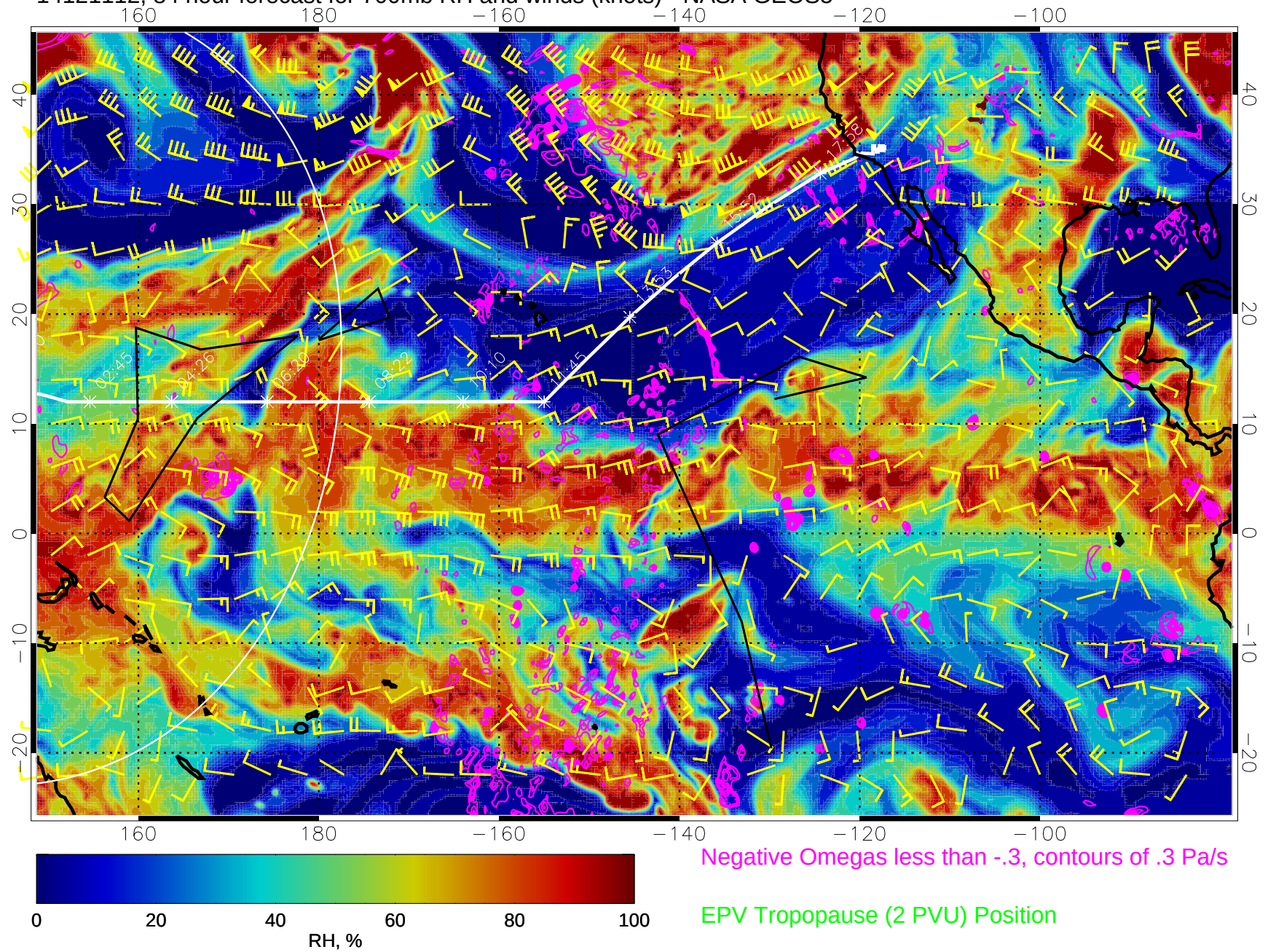
14121112, 84 hour forecast for 700mb RH and winds (knots) - NASA GEOS5
