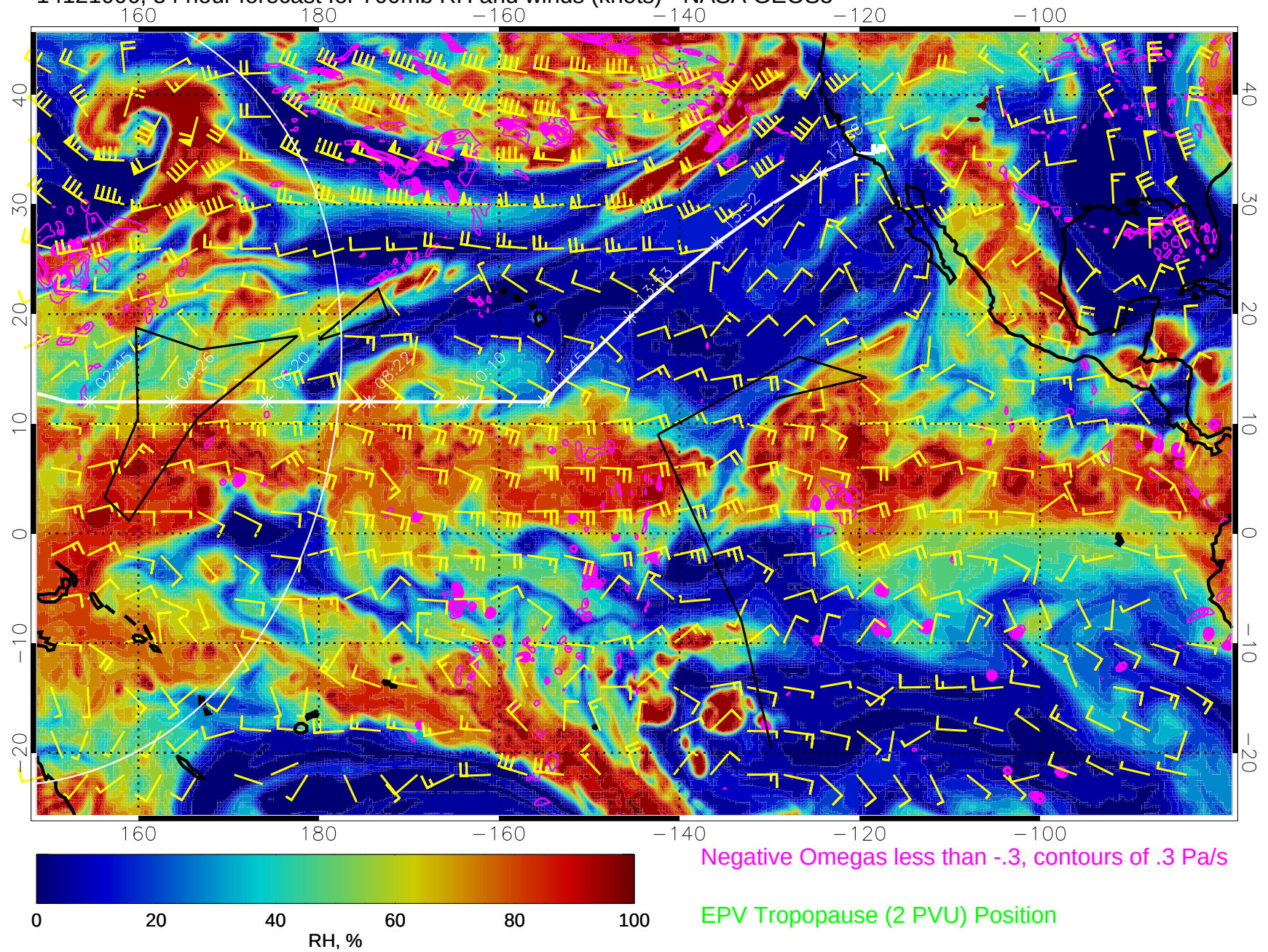
14121006, 54 hour forecast for 700mb RH and winds (knots) - NASA GEOS5
