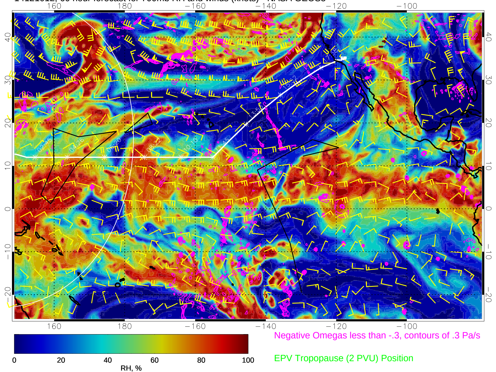
14121012, 60 hour forecast for 700mb RH and winds (knots) - NASA GEOS5
