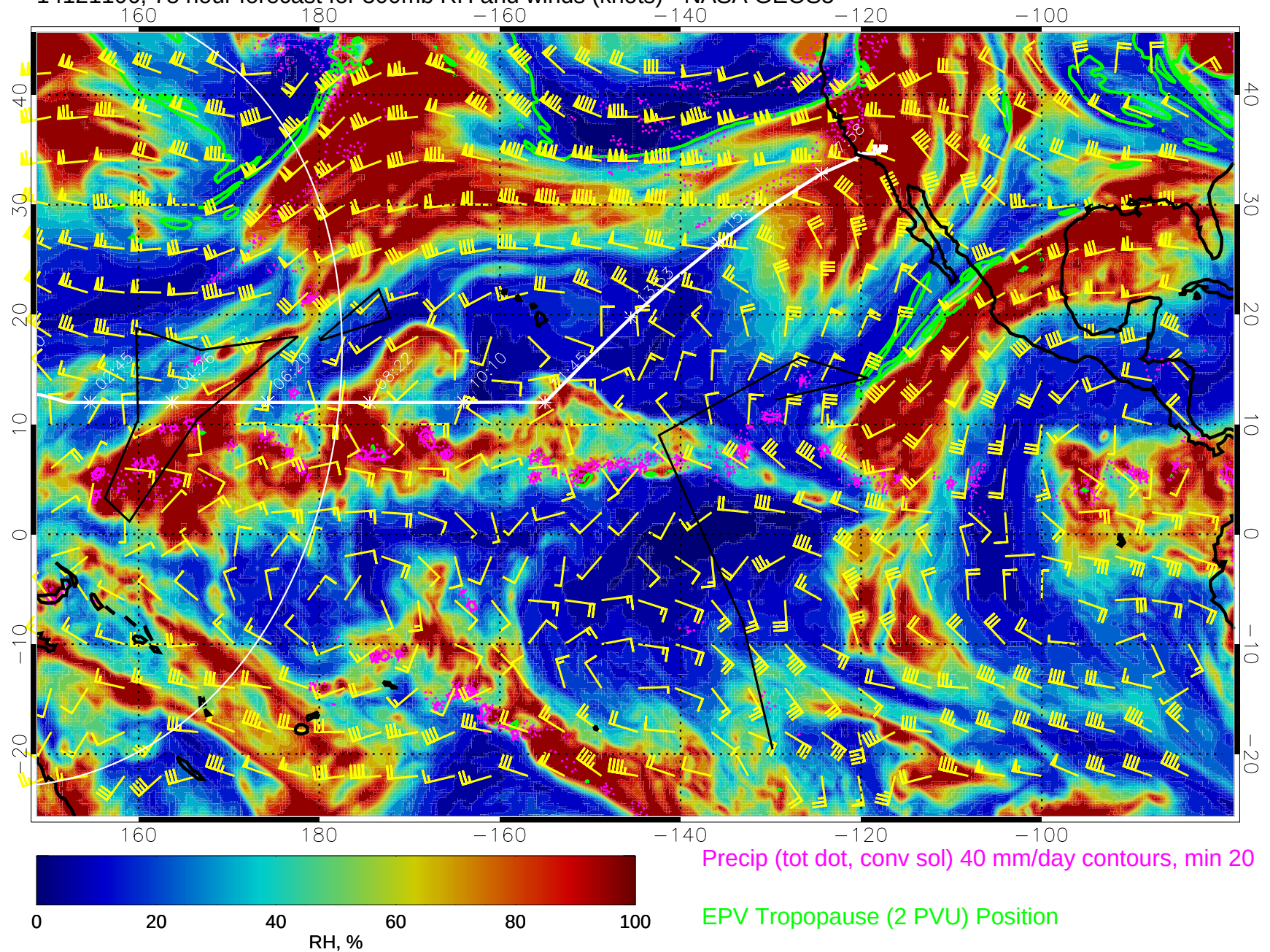
14121106, 78 hour forecast for 300mb RH and winds (knots) - NASA GEOS5
