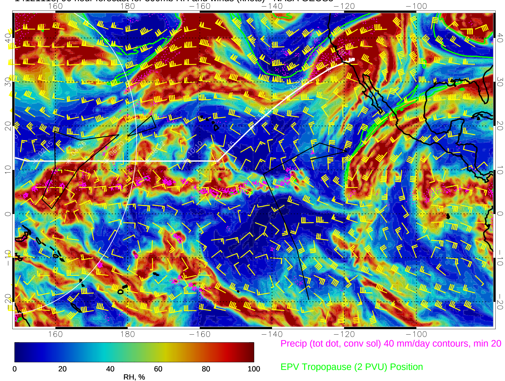
14121118, 90 hour forecast for 300mb RH and winds (knots) - NASA GEOS5
