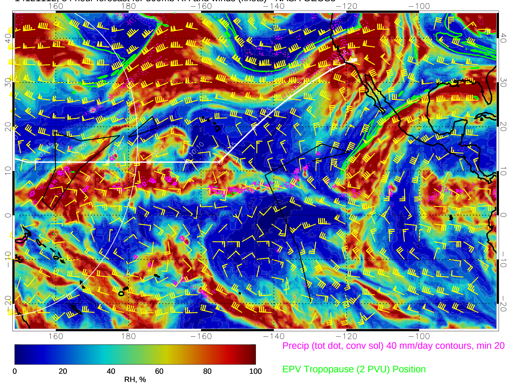
14121112, 84 hour forecast for 300mb RH and winds (knots) - NASA GEOS5
