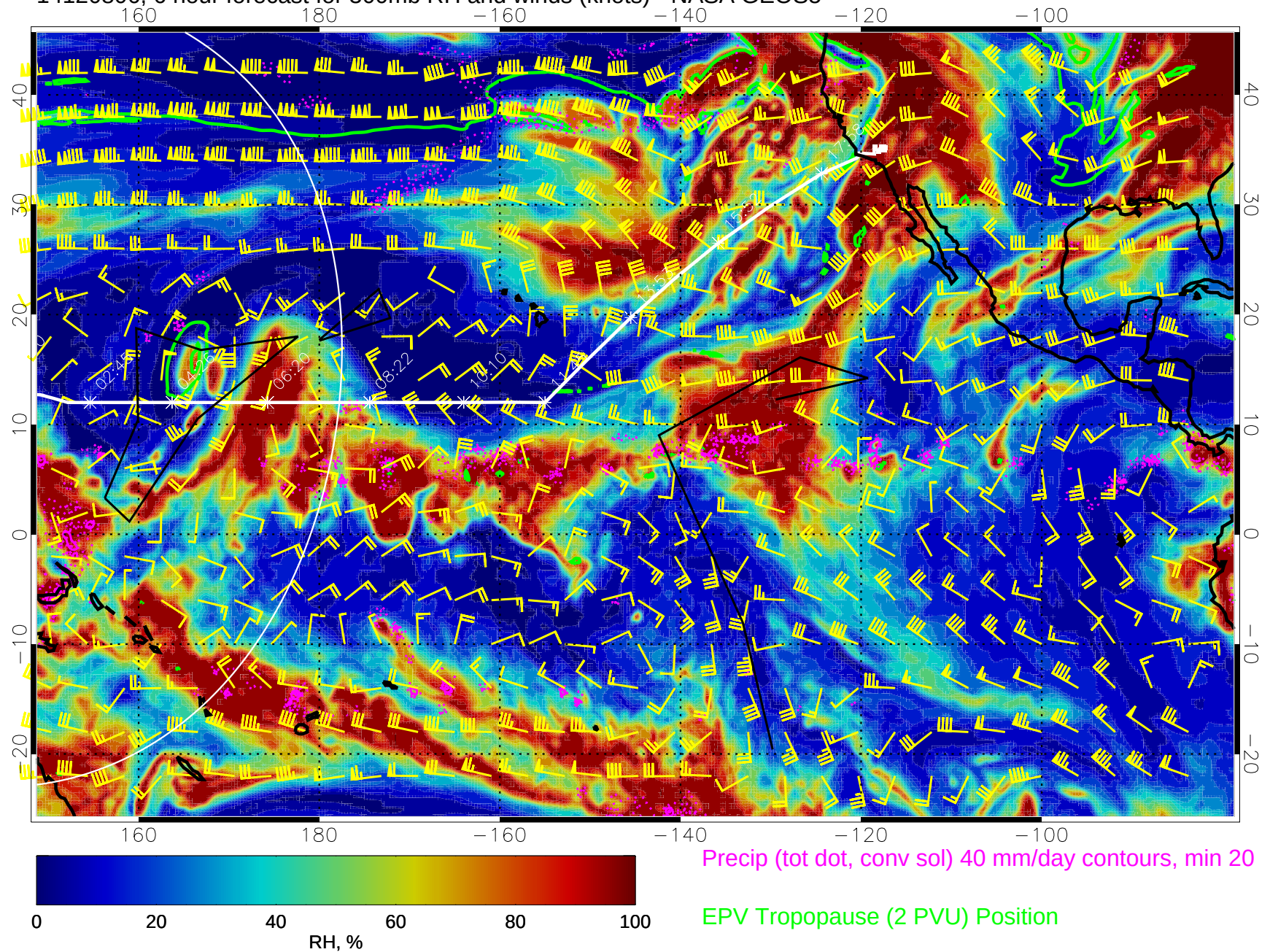
14120806, 6 hour forecast for 300mb RH and winds (knots) - NASA GEOS5
