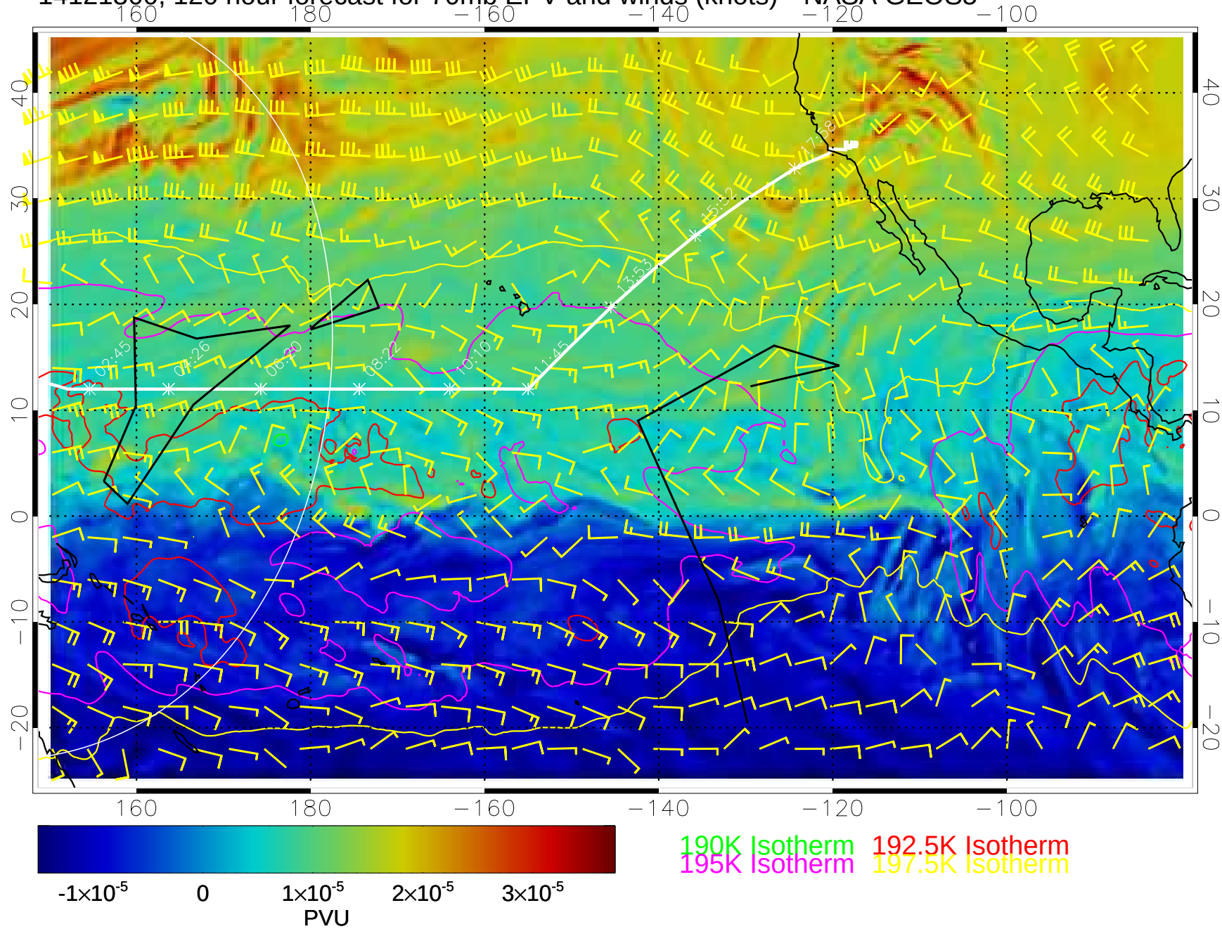
14121300, 120 hour forecast for 70mb EPV and winds (knots)-- NASA GEOS5
