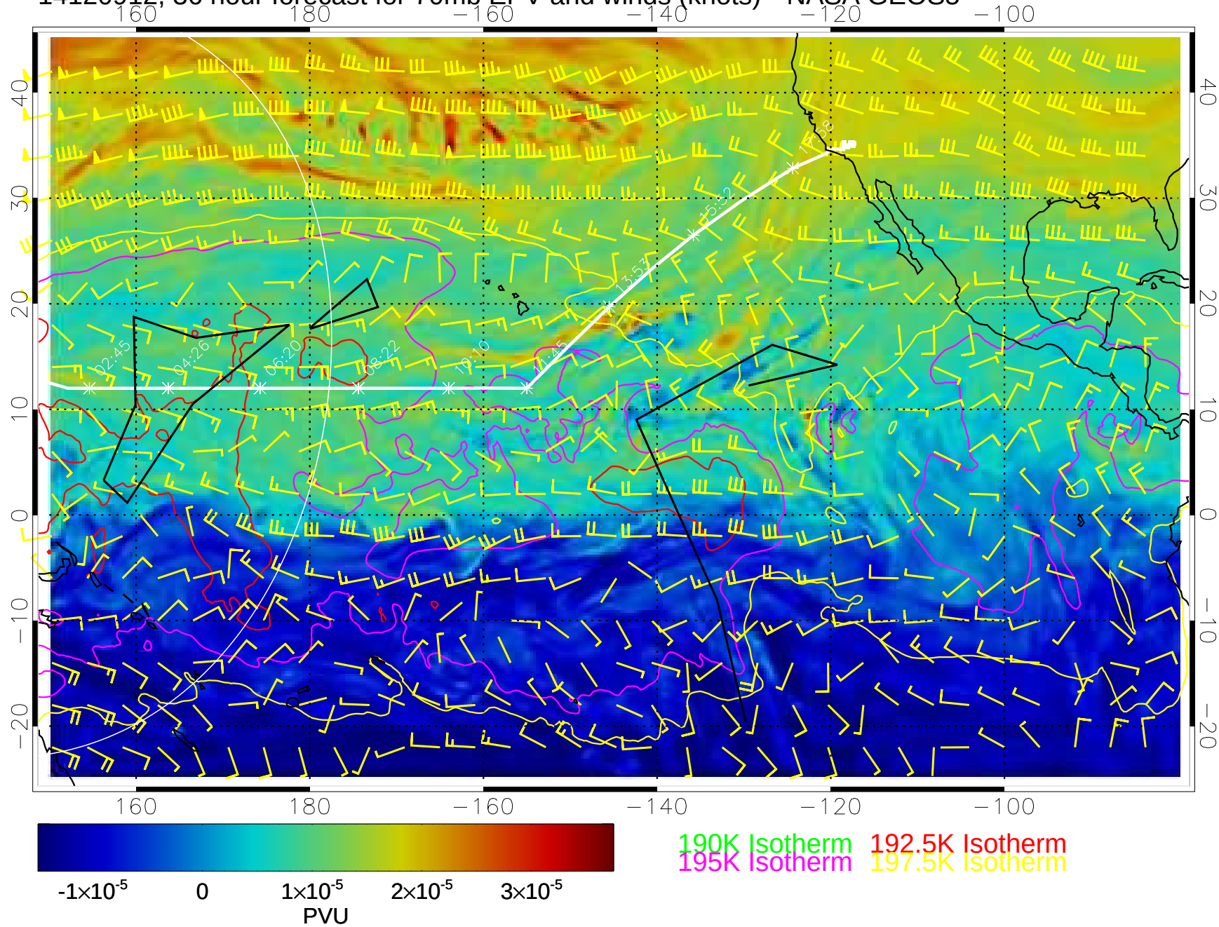
14120912, 36 hour forecast for 70mb EPV and winds (knots)-- NASA GEOS5
