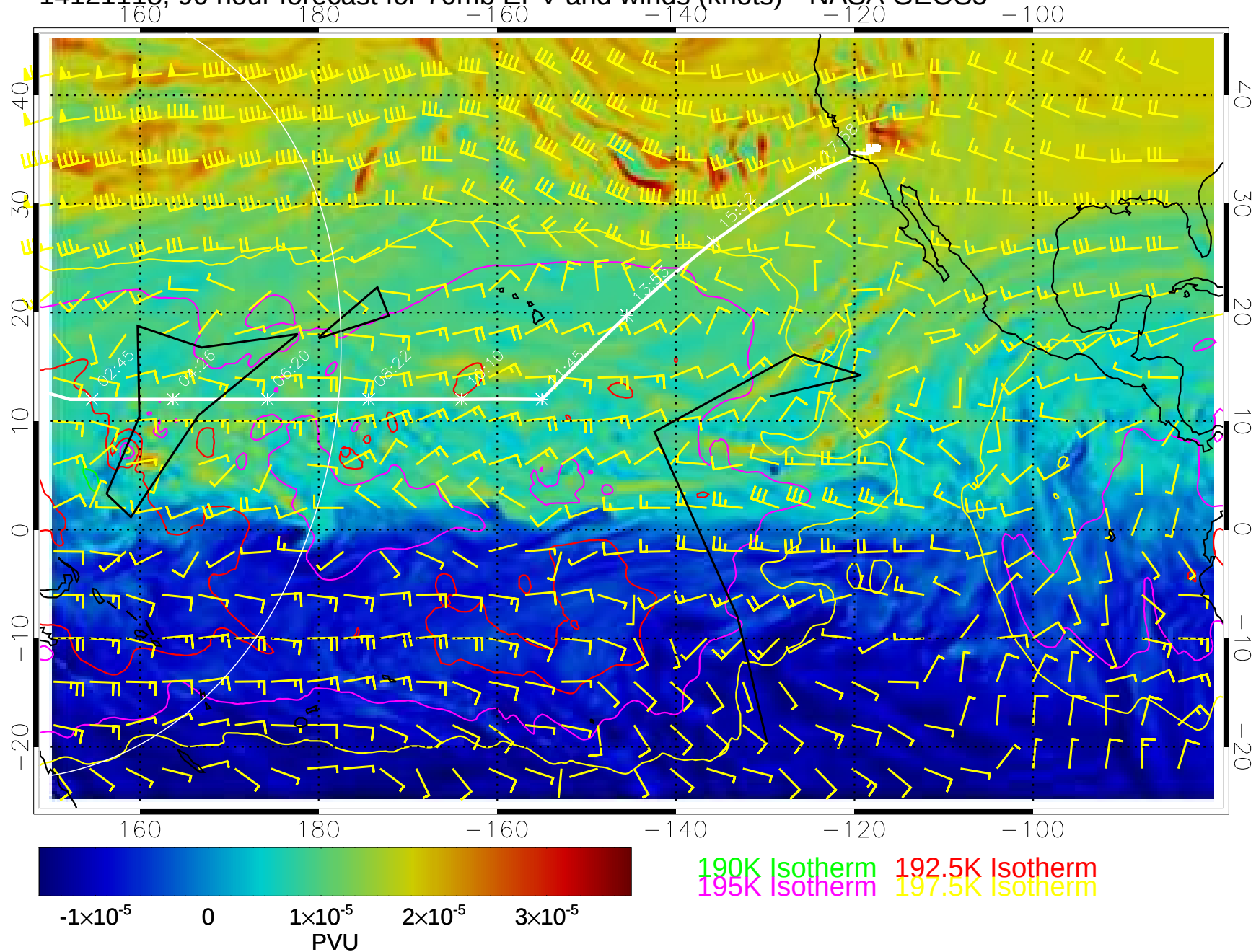
14121118, 90 hour forecast for 70mb EPV and winds (knots)-- NASA GEOS5
