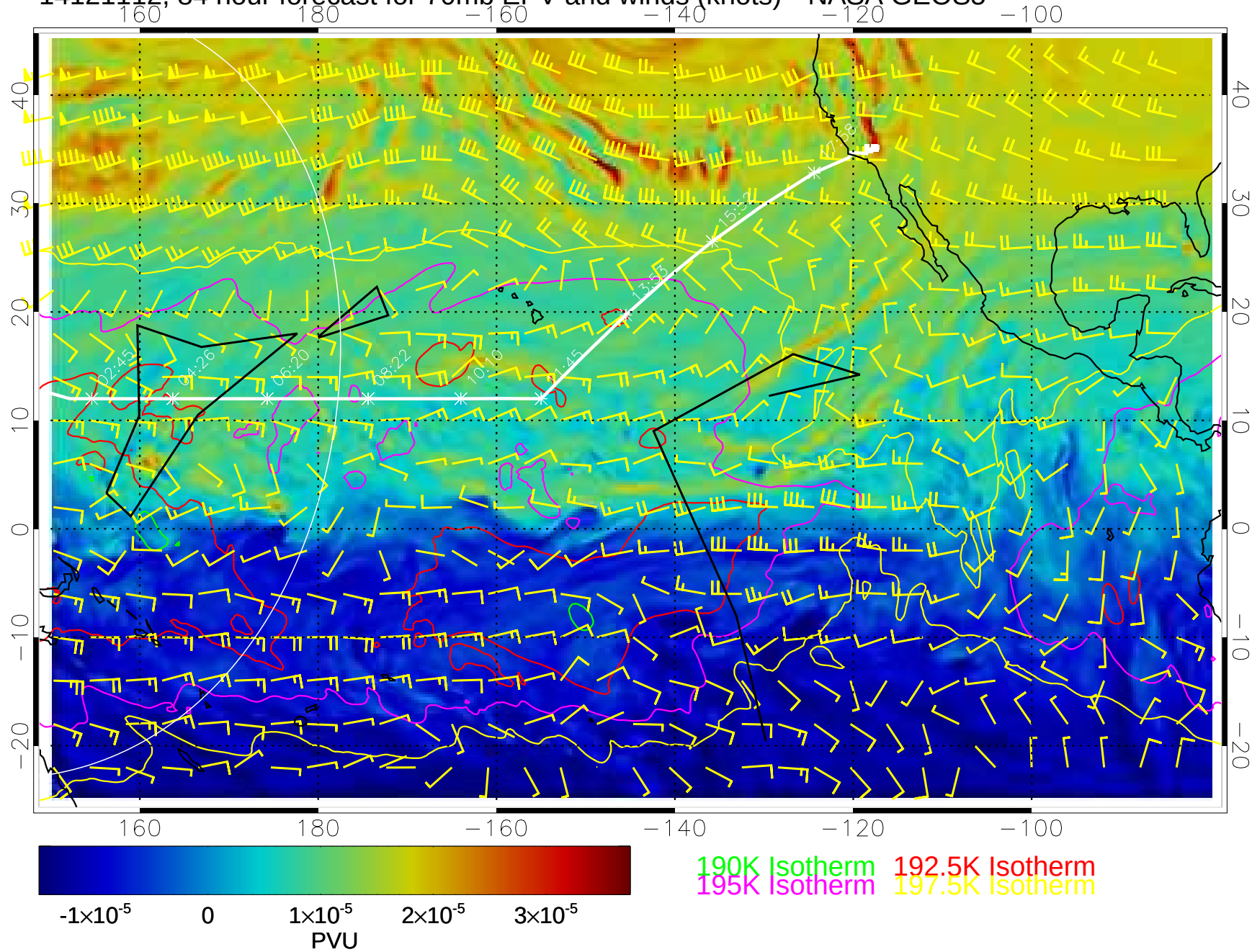
14121112, 84 hour forecast for 70mb EPV and winds (knots)-- NASA GEOS5
