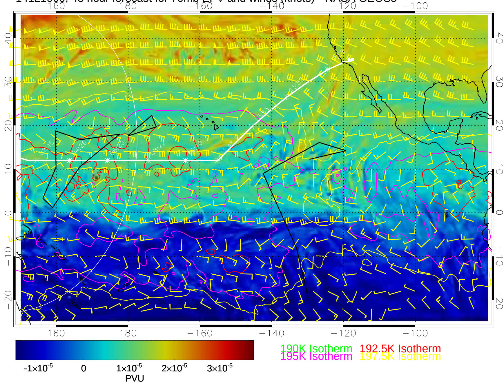
14121000, 48 hour forecast for 70mb EPV and winds (knots)-- NASA GEOS5
