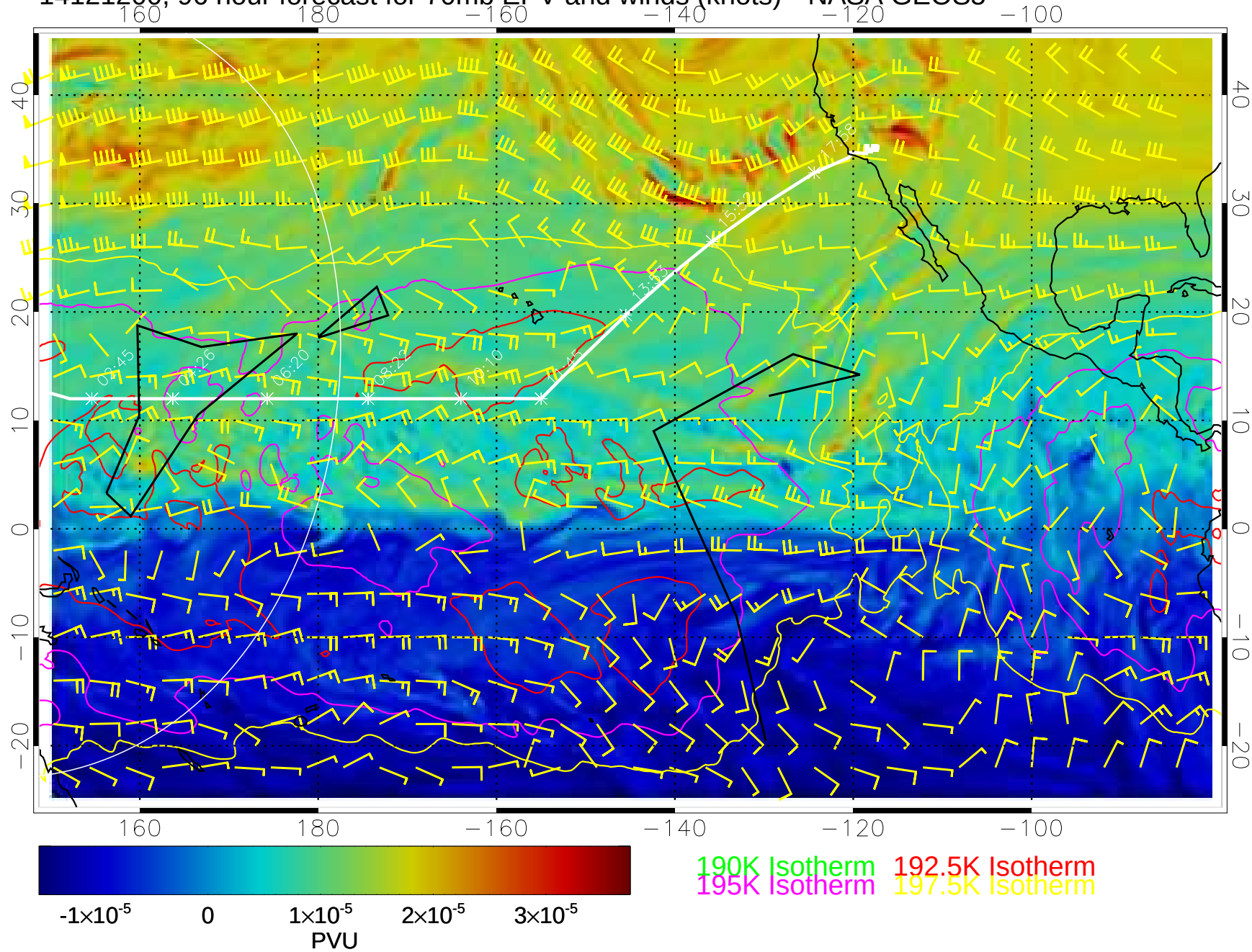
14121200, 96 hour forecast for 70mb EPV and winds (knots)-- NASA GEOS5
