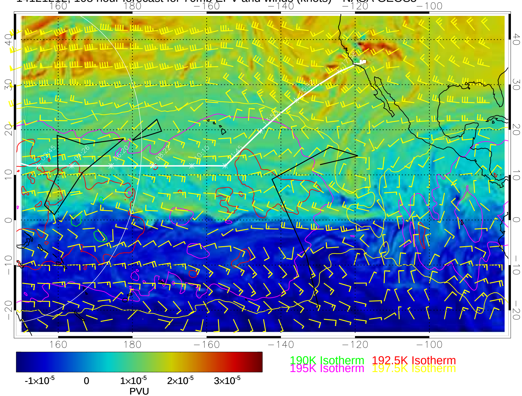
14121212, 108 hour forecast for 70mb EPV and winds (knots)-- NASA GEOS5
