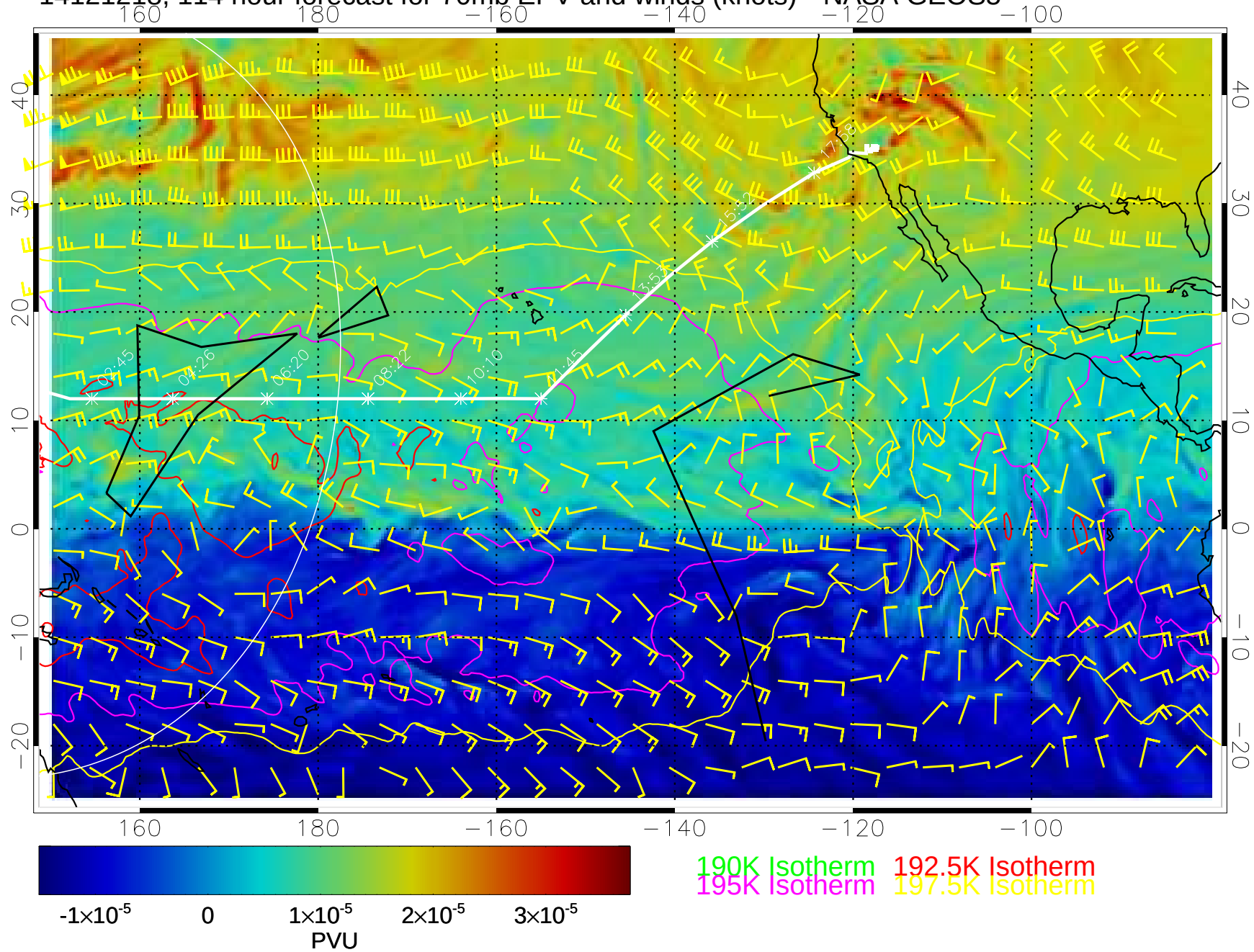
14121218, 114 hour forecast for 70mb EPV and winds (knots)-- NASA GEOS5
