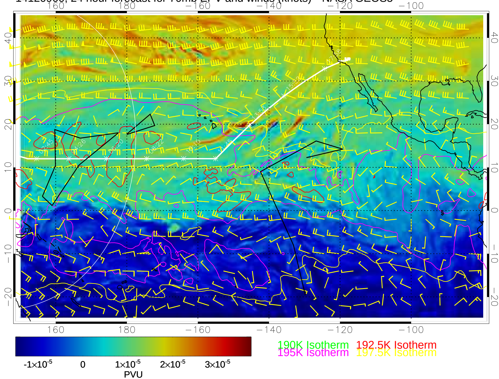
14120900, 24 hour forecast for 70mb EPV and winds (knots)-- NASA GEOS5
