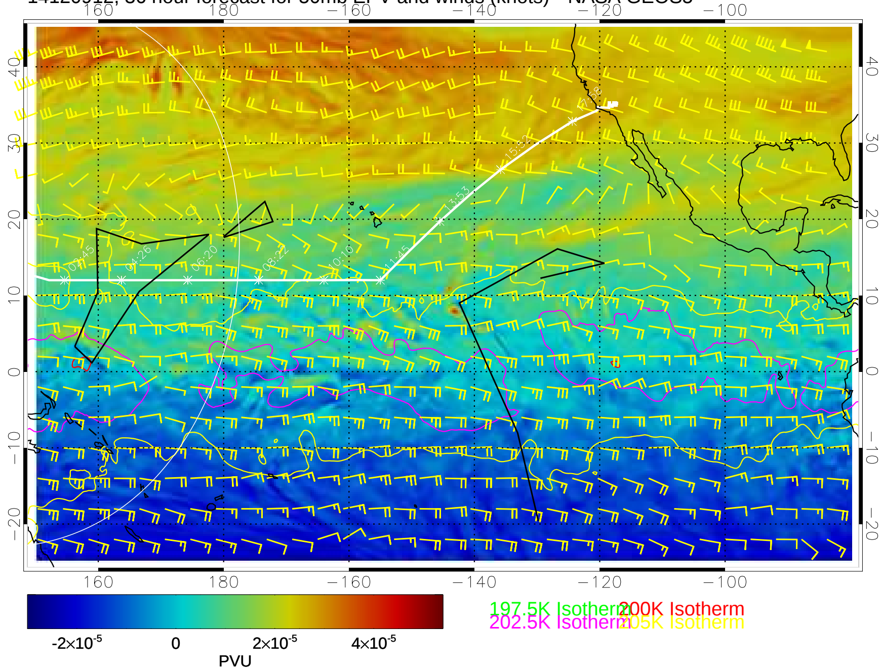
14120912, 36 hour forecast for 50mb EPV and winds (knots)-- NASA GEOS5
