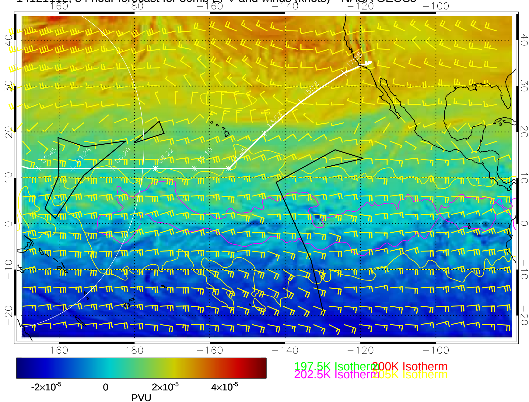
14121112, 84 hour forecast for 50mb EPV and winds (knots)-- NASA GEOS5
