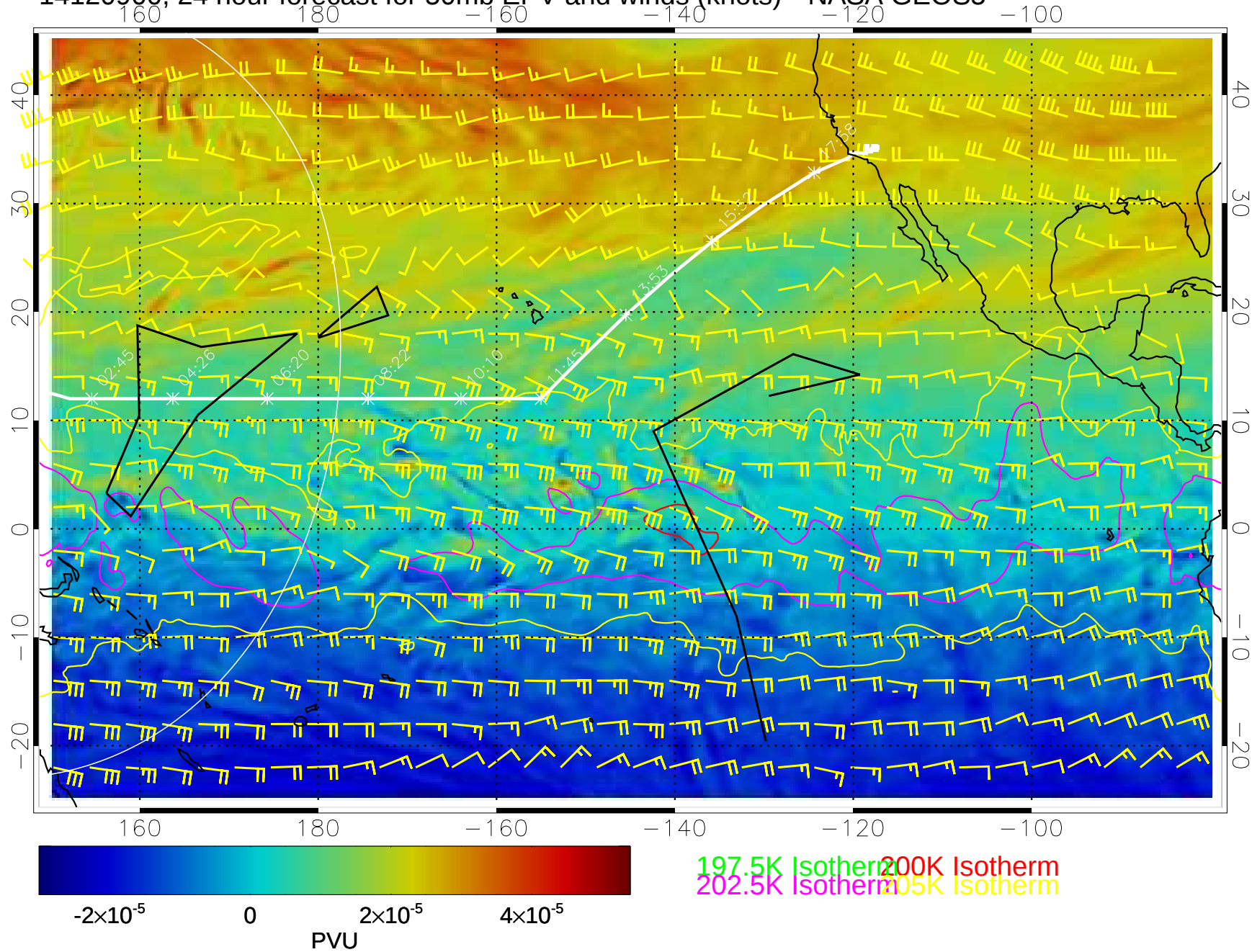
14120900, 24 hour forecast for 50mb EPV and winds (knots)-- NASA GEOS5
