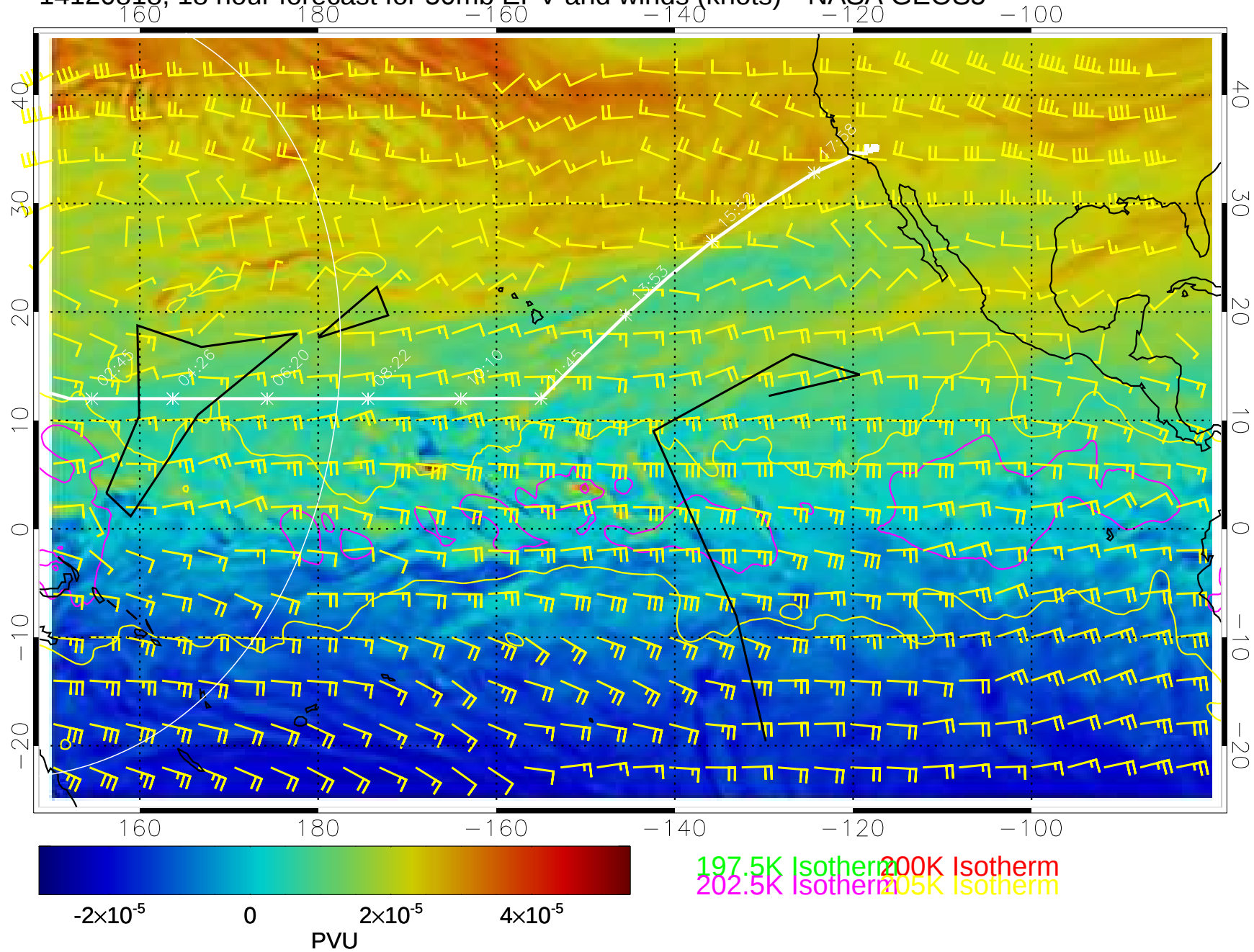
14120818, 18 hour forecast for 50mb EPV and winds (knots)-- NASA GEOS5
