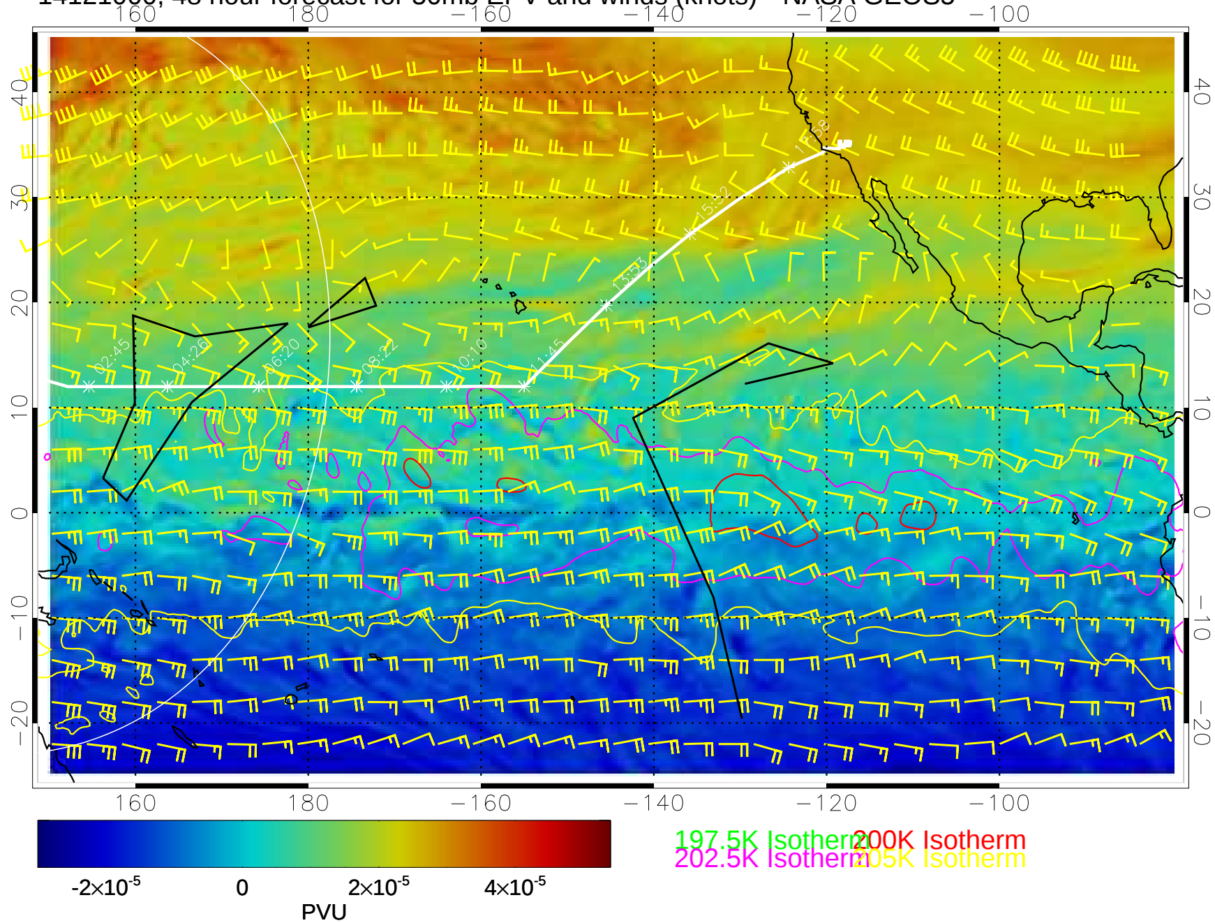
14121000, 48 hour forecast for 50mb EPV and winds (knots)-- NASA GEOS5
