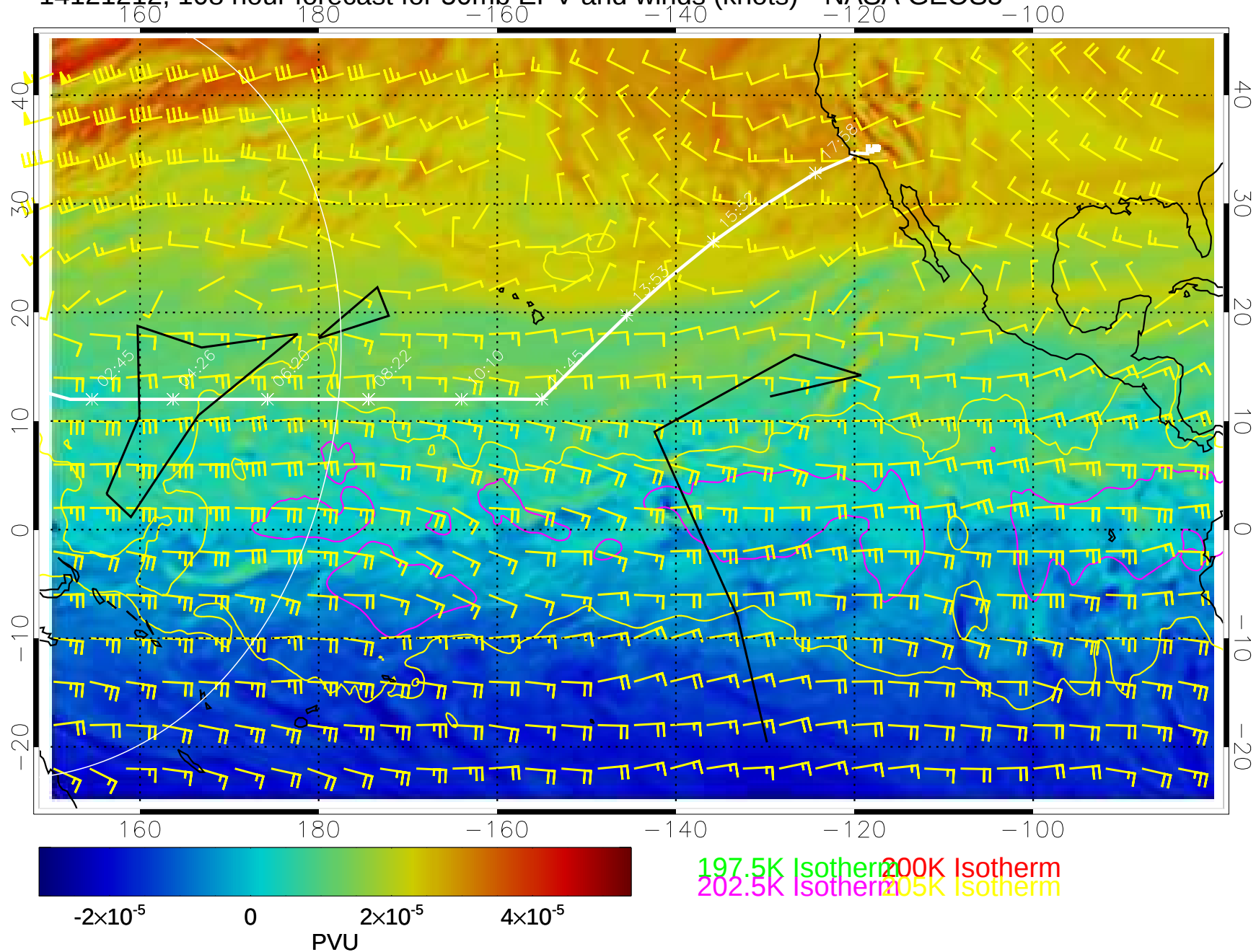
14121212, 108 hour forecast for 50mb EPV and winds (knots)-- NASA GEOS5
