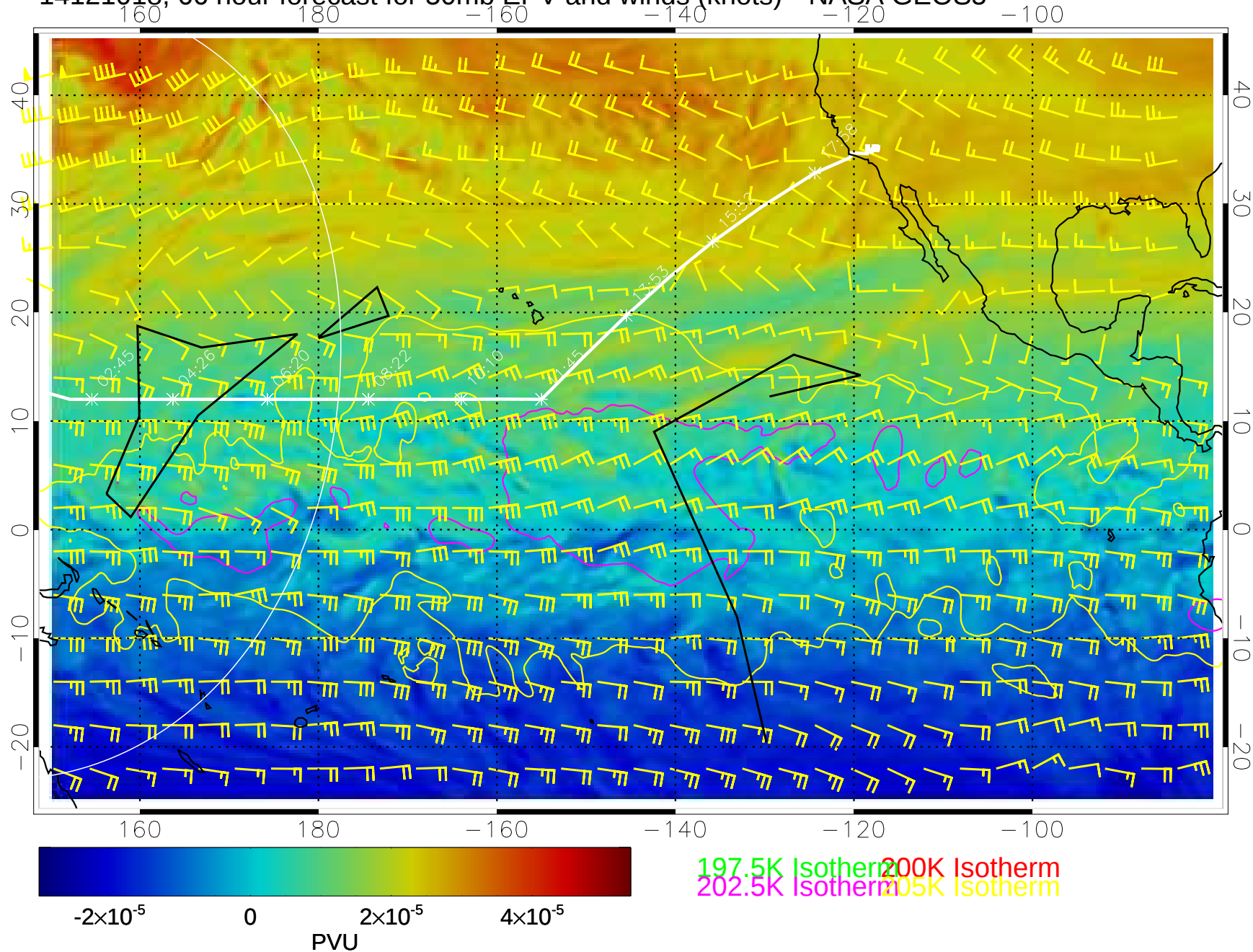
14121018, 66 hour forecast for 50mb EPV and winds (knots)-- NASA GEOS5
