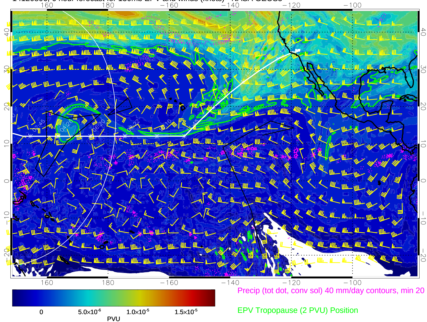
14120806, 6 hour forecast for 150mb EPV and winds (knots) - NASA GEOS5
