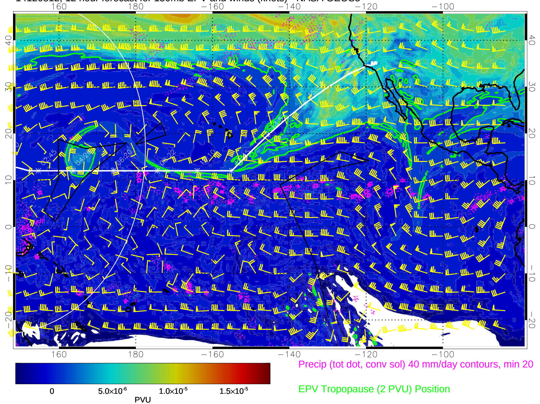
14120812, 12 hour forecast for 150mb EPV and winds (knots) - NASA GEOS5
