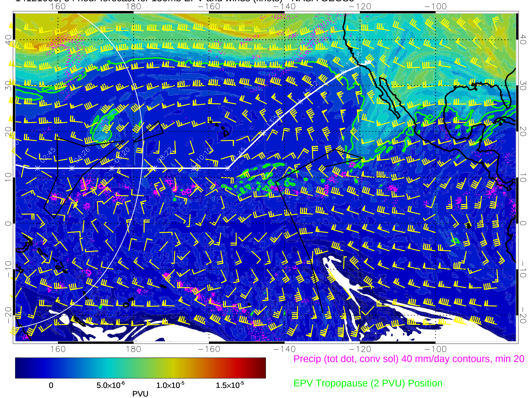
14121006, 54 hour forecast for 150mb EPV and winds (knots) - NASA GEOS5
