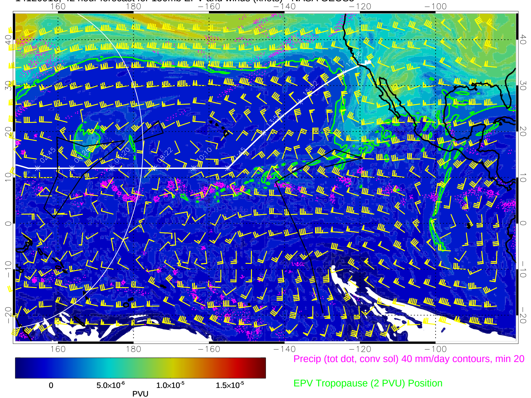
14120918, 42 hour forecast for 150mb EPV and winds (knots) - NASA GEOS5
