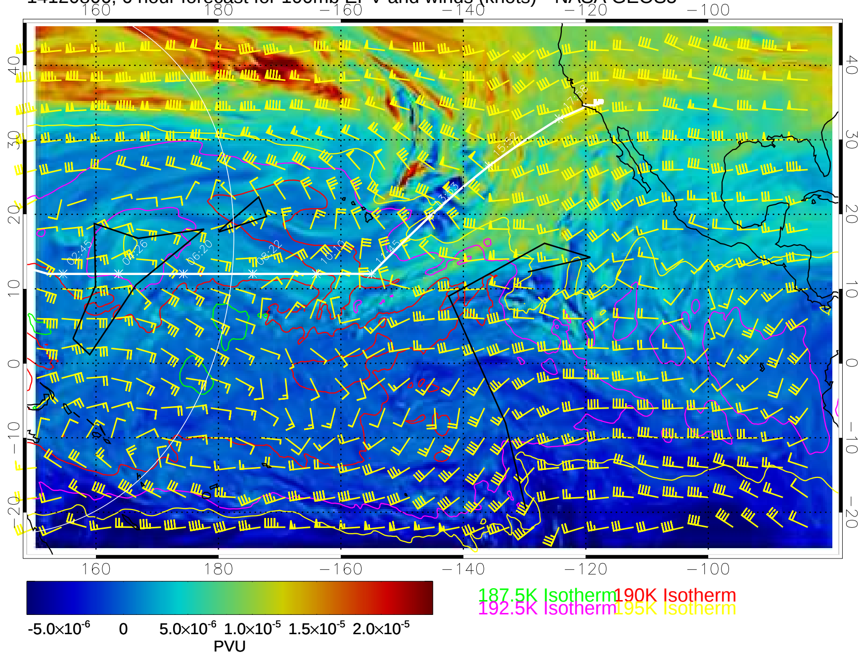
14120806, 6 hour forecast for 100mb EPV and winds (knots)-- NASA GEOS5
