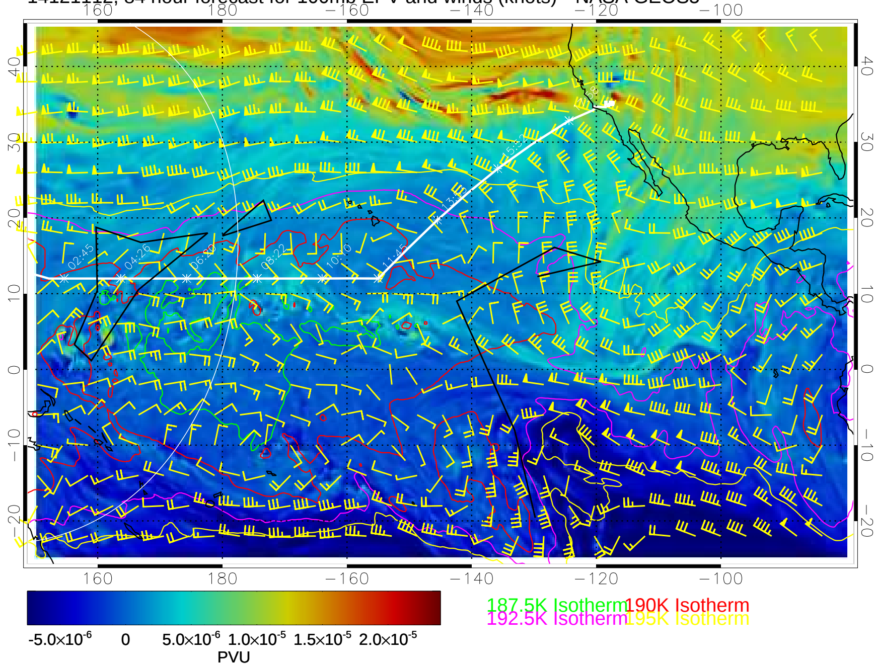
14121112, 84 hour forecast for 100mb EPV and winds (knots)-- NASA GEOS5
