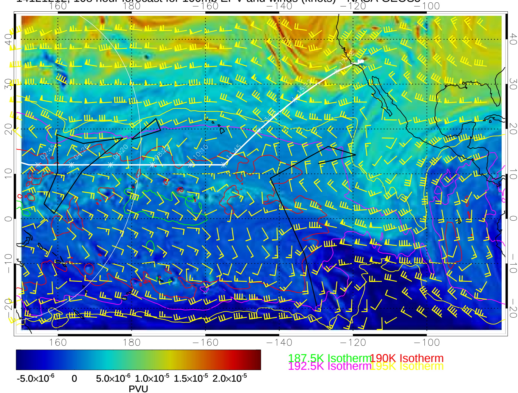
141212Z, 108 hour forecast for 100mb EPV and winds (knots)-- NASA GEOS5
