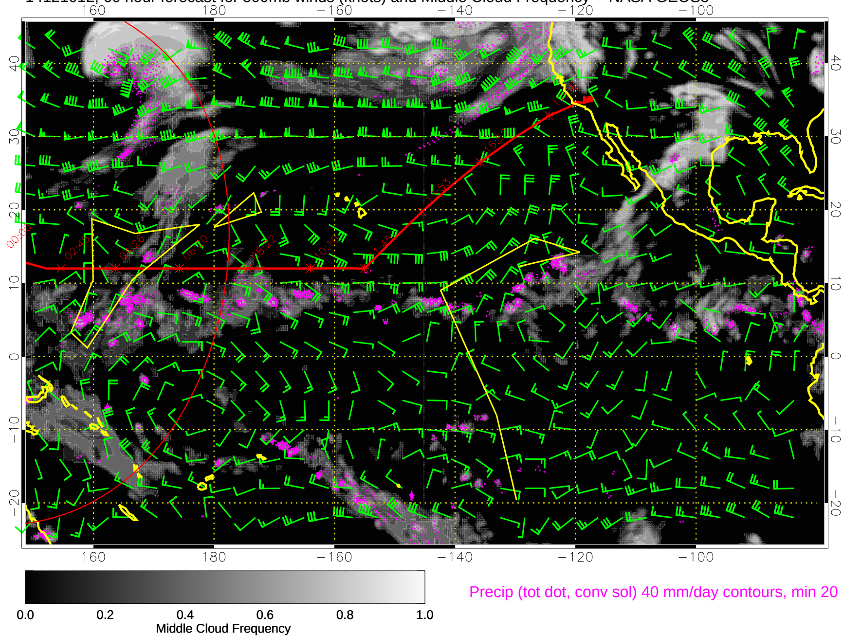
14121012, 60 hour forecast for 500mb winds (knots) and Middle Cloud Frequency -- NASA GEOS5
