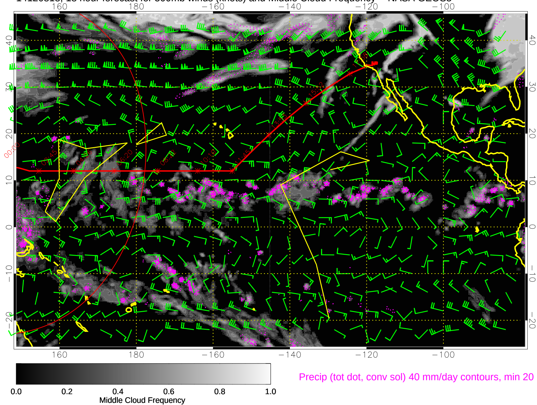
14120818, 18 hour forecast for 500mb winds (knots) and Middle Cloud Frequency -- NASA GEOS5
