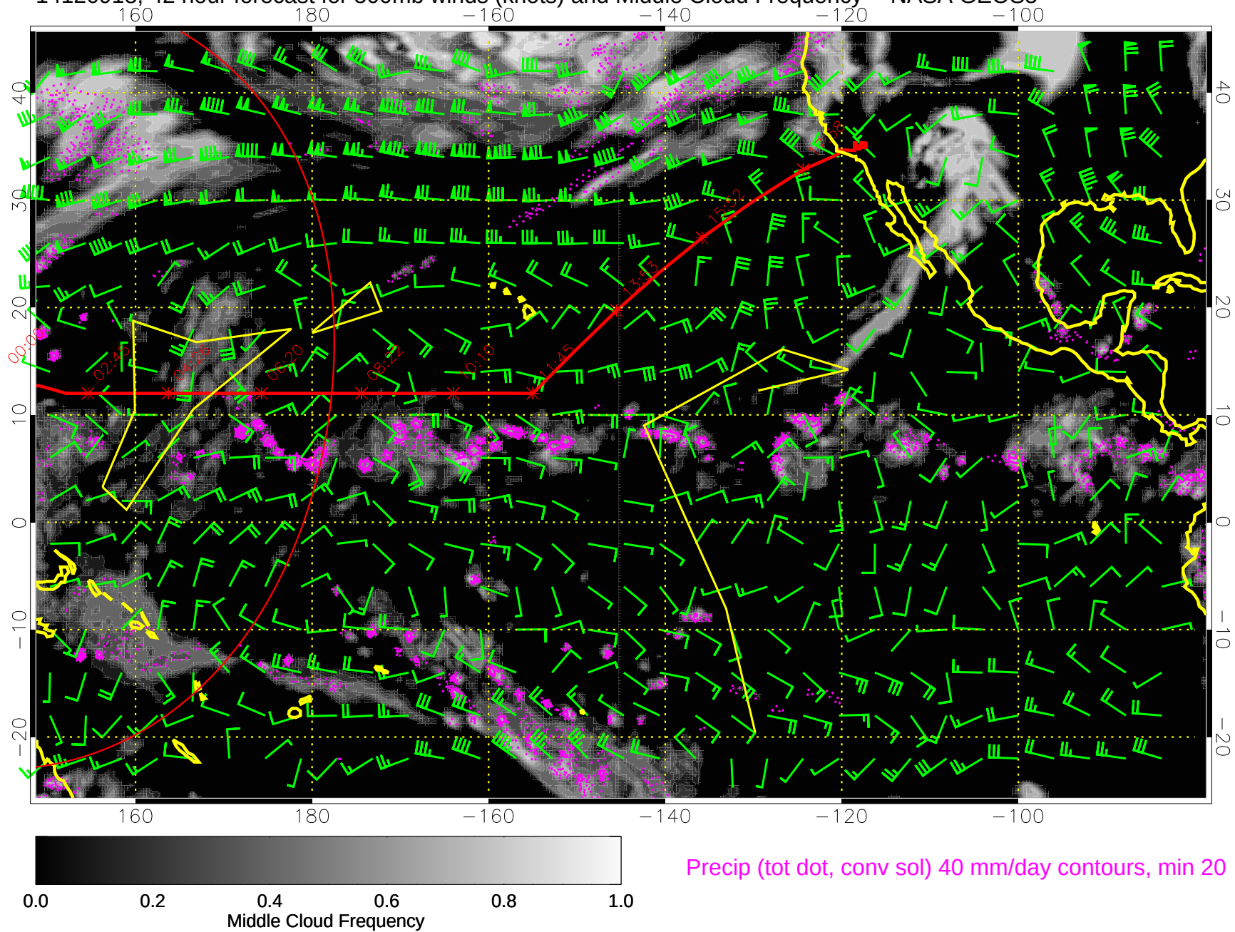
14120918, 42 hour forecast for 500mb winds (knots) and Middle Cloud Frequency -- NASA GEOS5
