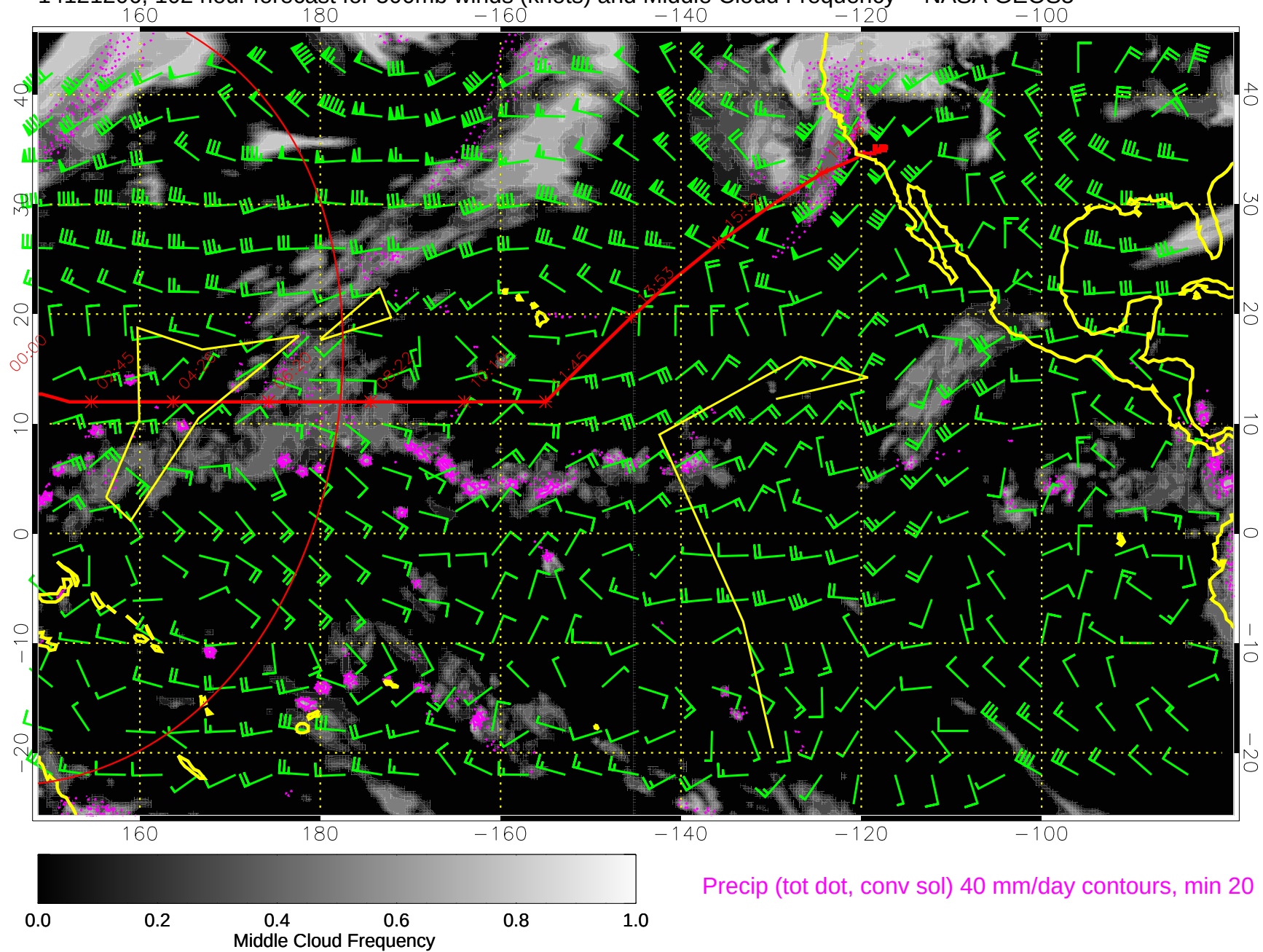
14121206, 102 hour forecast for 500mb winds (knots) and Middle Cloud Frequency -- NASA GEOS5
