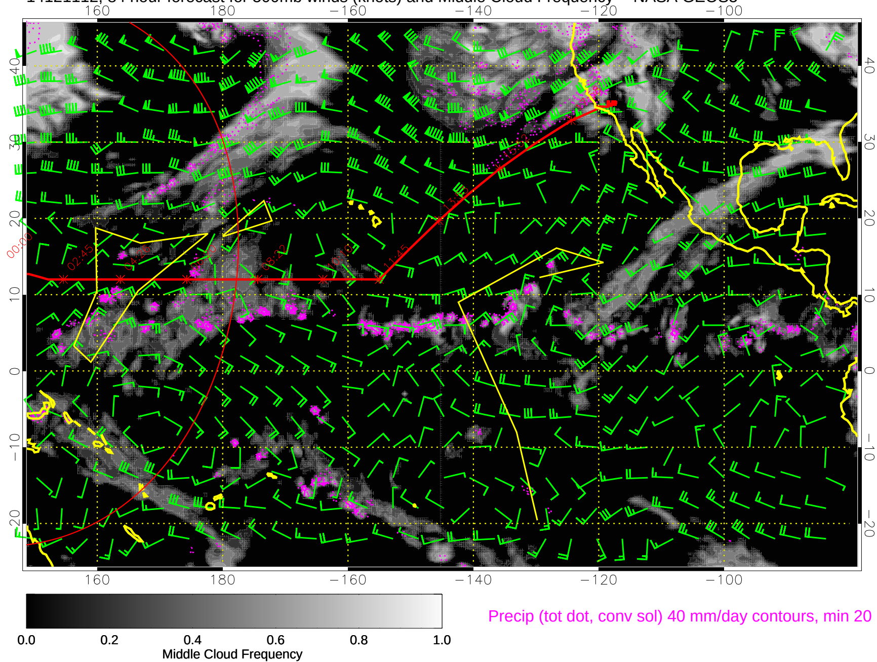
14121112, 84 hour forecast for 500mb winds (knots) and Middle Cloud Frequency -- NASA GEOS5
