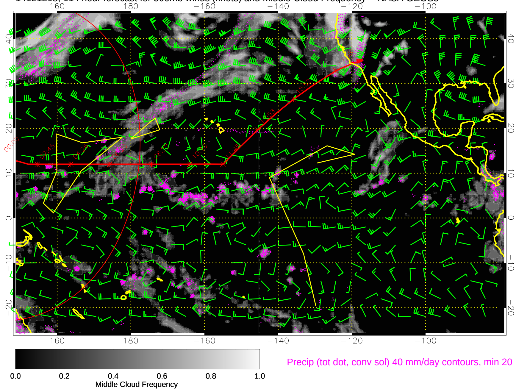
14121218, 114 hour forecast for 500mb winds (knots) and Middle Cloud Frequency -- NASA GEOS5
