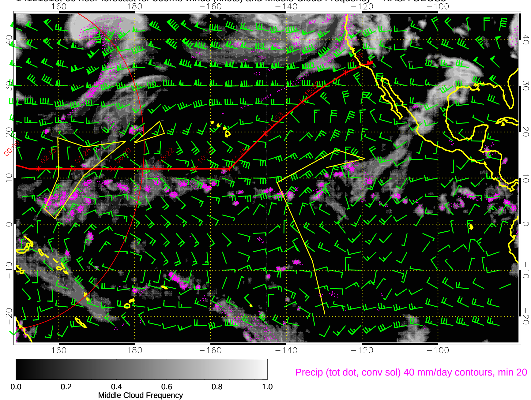
14121018, 66 hour forecast for 500mb winds (knots) and Middle Cloud Frequency -- NASA GEOS5
