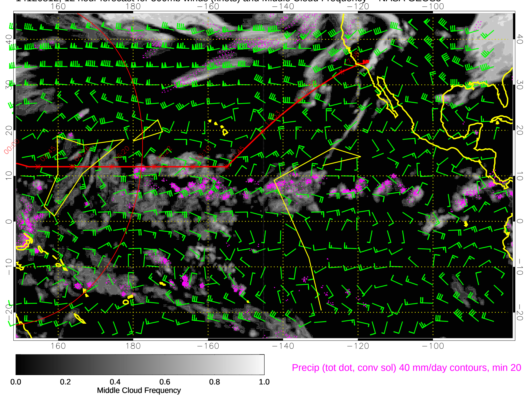
14120812, 12 hour forecast for 500mb winds (knots) and Middle Cloud Frequency -- NASA GEOS5
