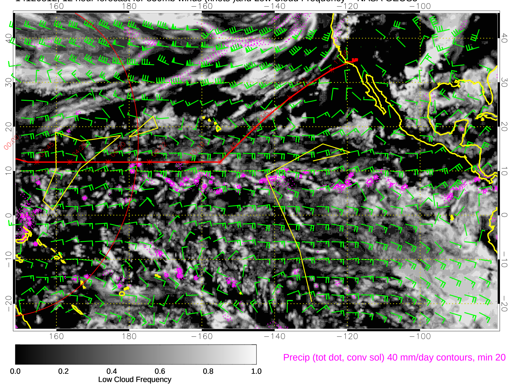
14120812, 12 hour forecast for 850mb winds (knots) and Low Cloud Frequency -- NASA GEOS5
