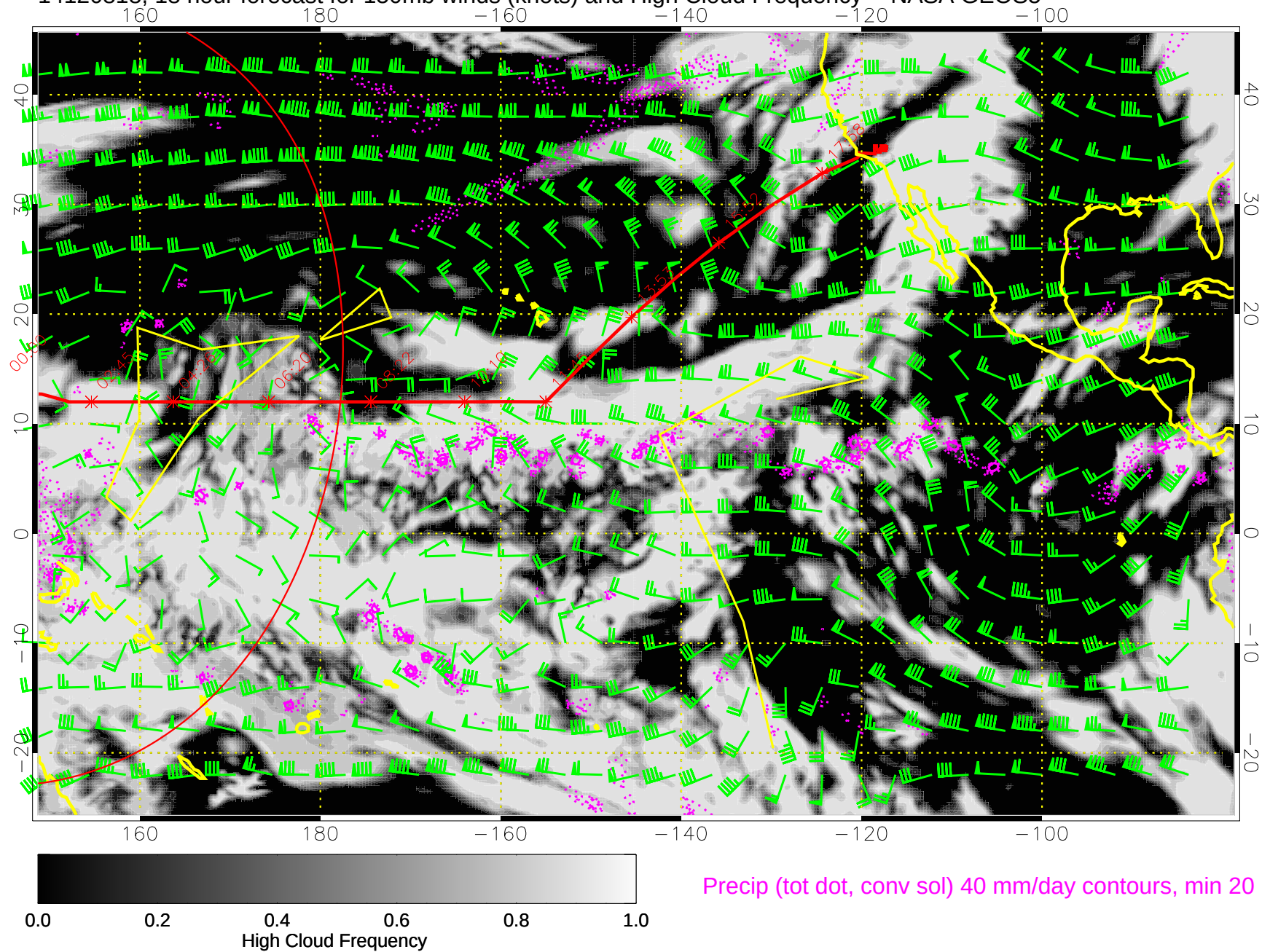
14120818, 18 hour forecast for 150mb winds (knots) and High Cloud Frequency -- NASA GEOS5
