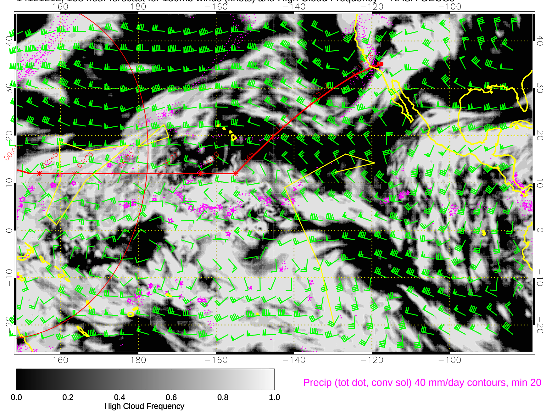
14121212, 108 hour forecast for 150mb winds (knots) and High Cloud Frequency -- NASA GEOS5
