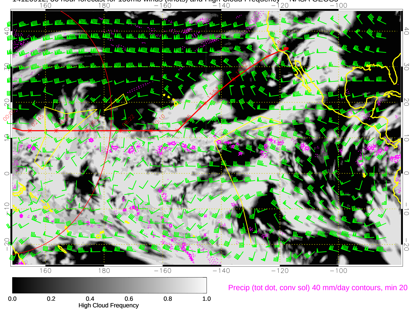
14120912, 36 hour forecast for 150mb winds (knots) and High Cloud Frequency -- NASA GEOS5
