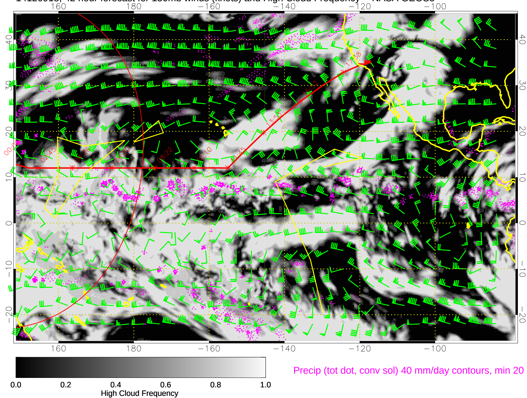
14120918, 42 hour forecast for 150mb winds (knots) and High Cloud Frequency -- NASA GEOS5
