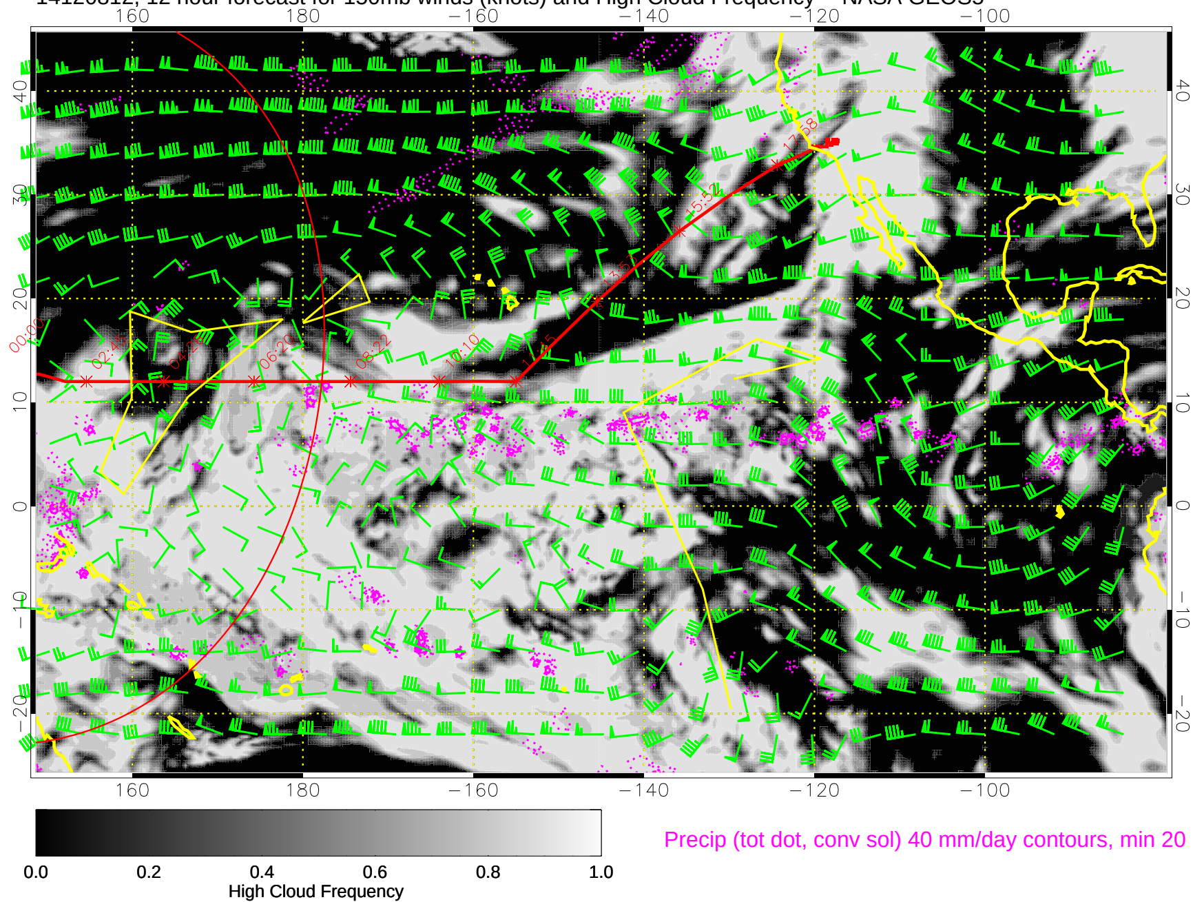
14120812, 12 hour forecast for 150mb winds (knots) and High Cloud Frequency -- NASA GEOS5
