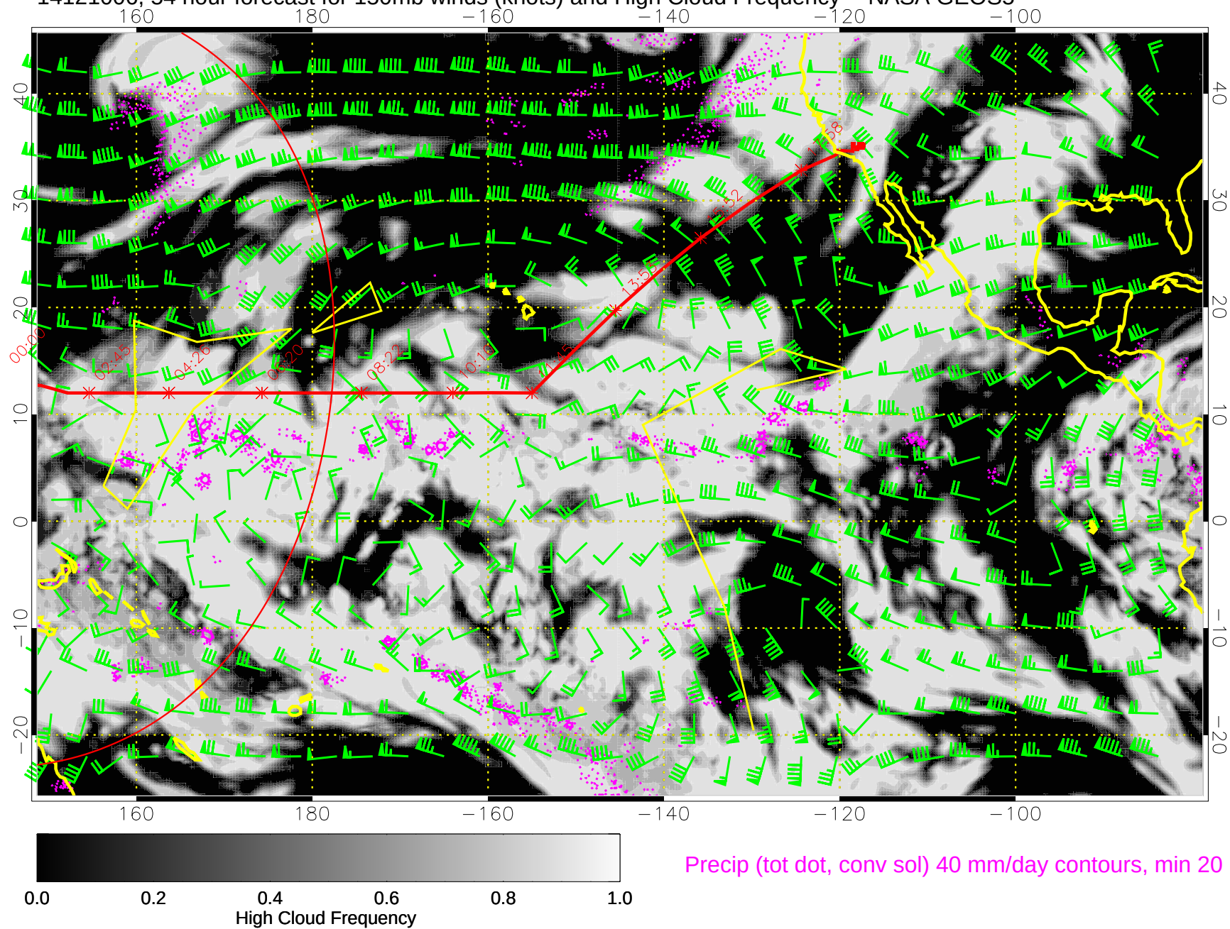
14121006, 54 hour forecast for 150mb winds (knots) and High Cloud Frequency -- NASA GEOS5
