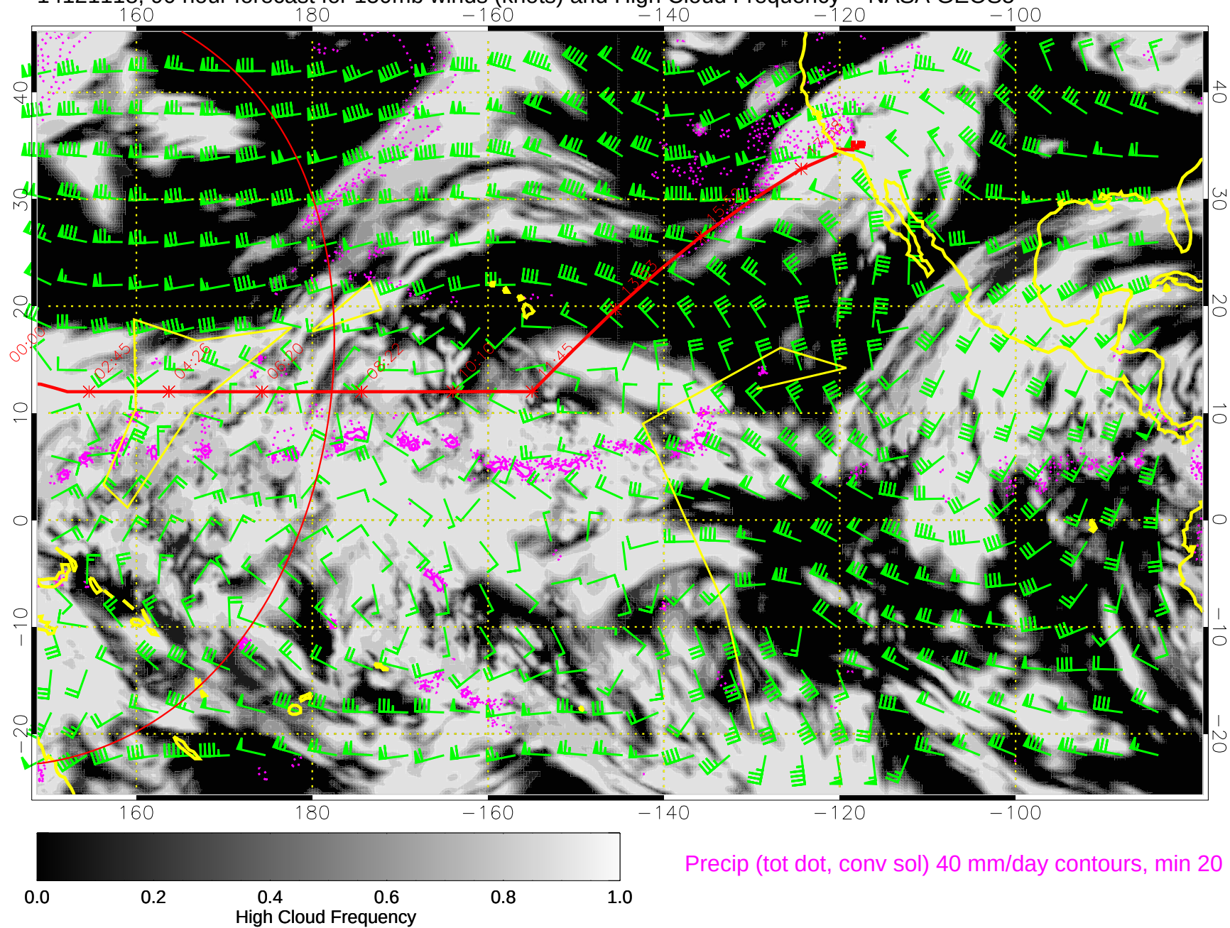
14121118, 90 hour forecast for 150mb winds (knots) and High Cloud Frequency -- NASA GEOS5
