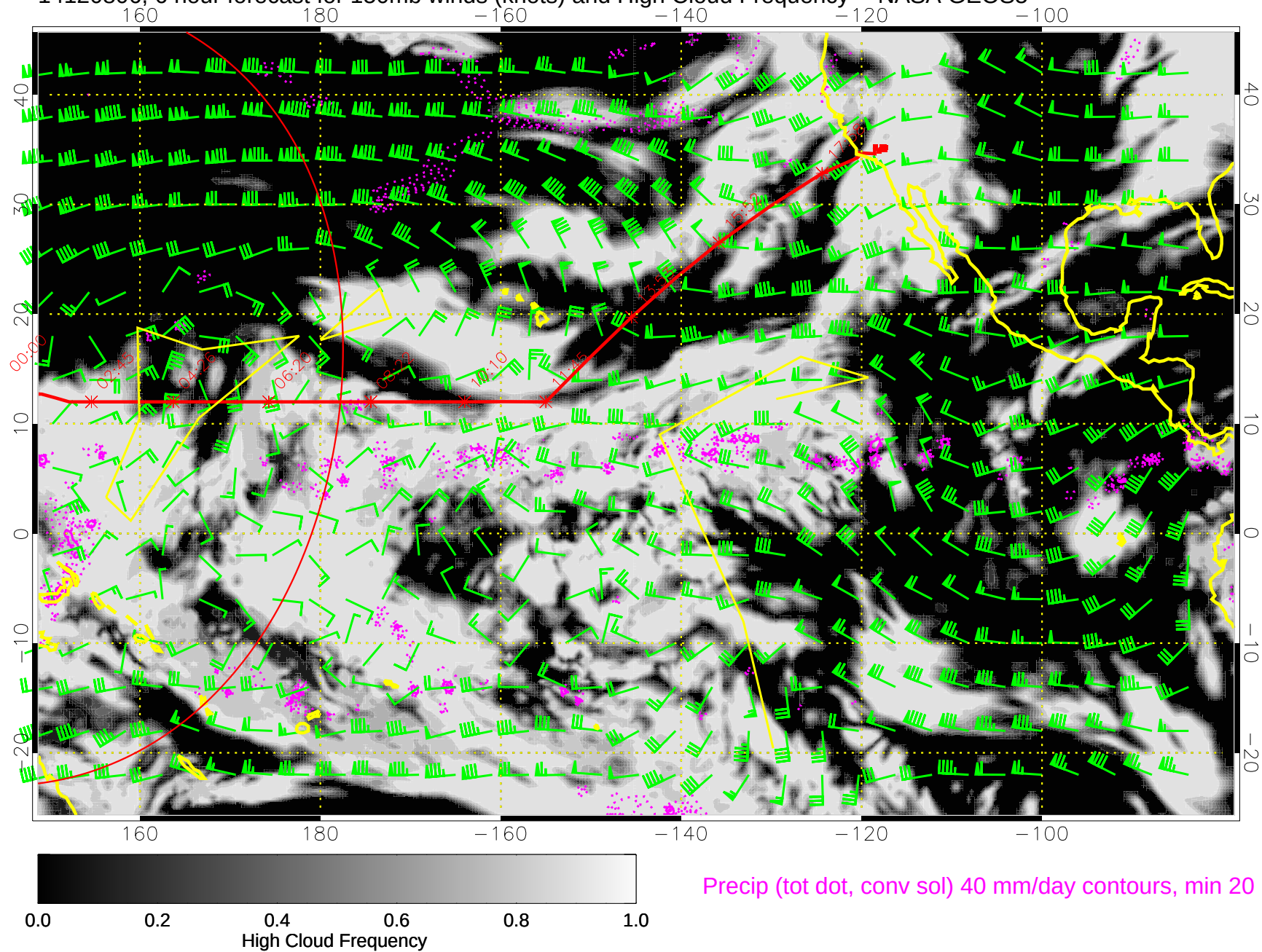
14120806, 6 hour forecast for 150mb winds (knots) and High Cloud Frequency -- NASA GEOS5
