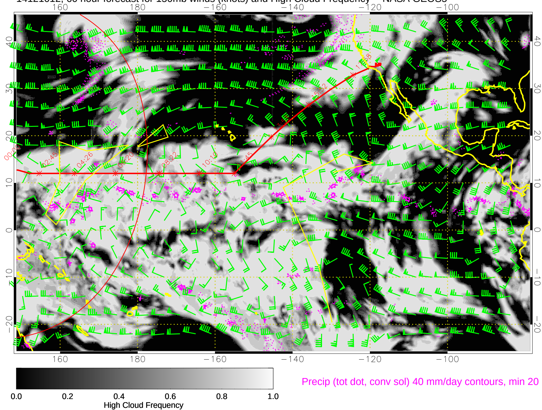
14121012, 60 hour forecast for 150mb winds (knots) and High Cloud Frequency -- NASA GEOS5
