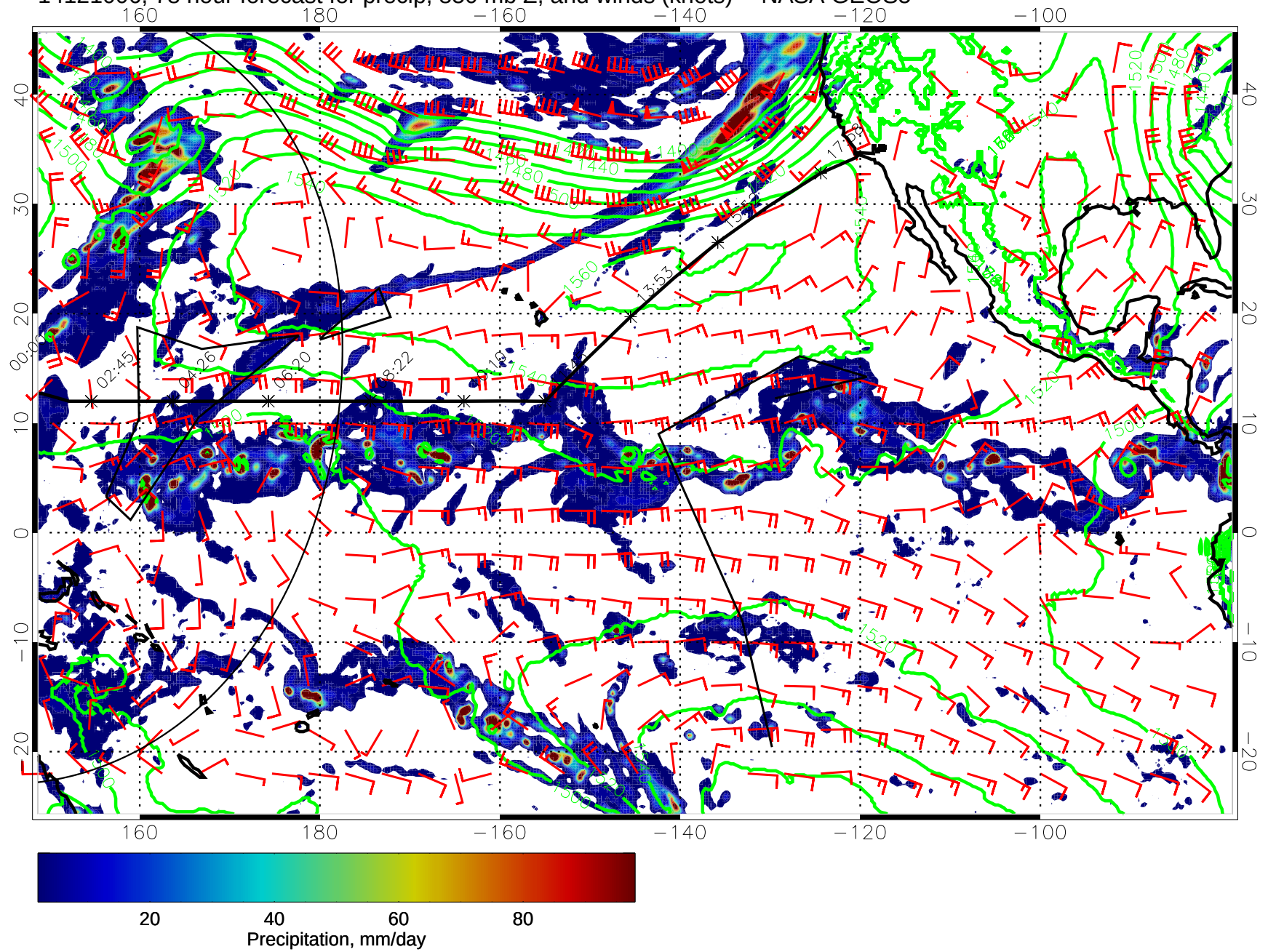
14121006, 78 hour forecast for precip, 850 mb Z, and winds (knots) -- NASA GEOS5
