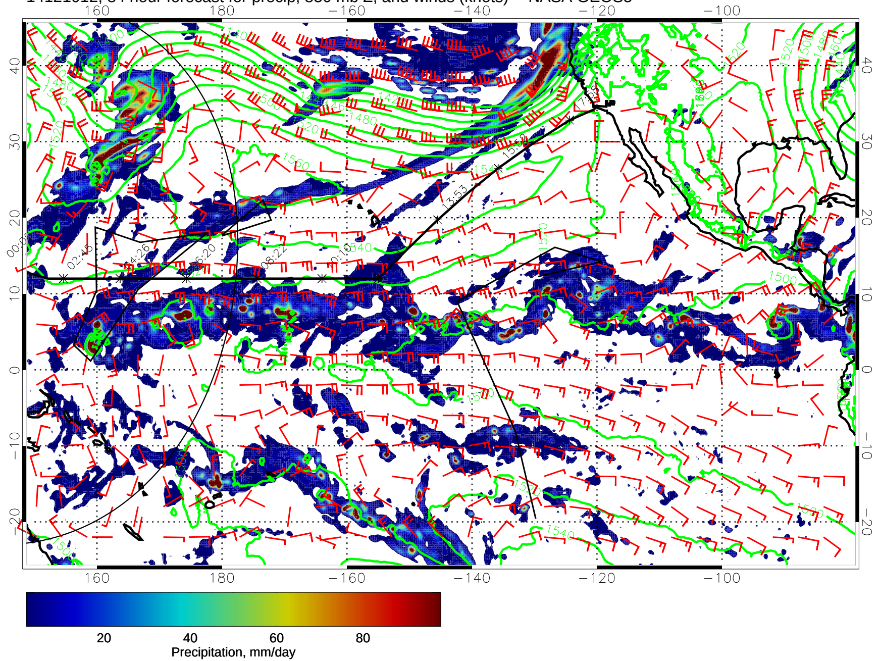
14121012, 84 hour forecast for precip, 850 mb Z, and winds (knots) -- NASA GEOS5
