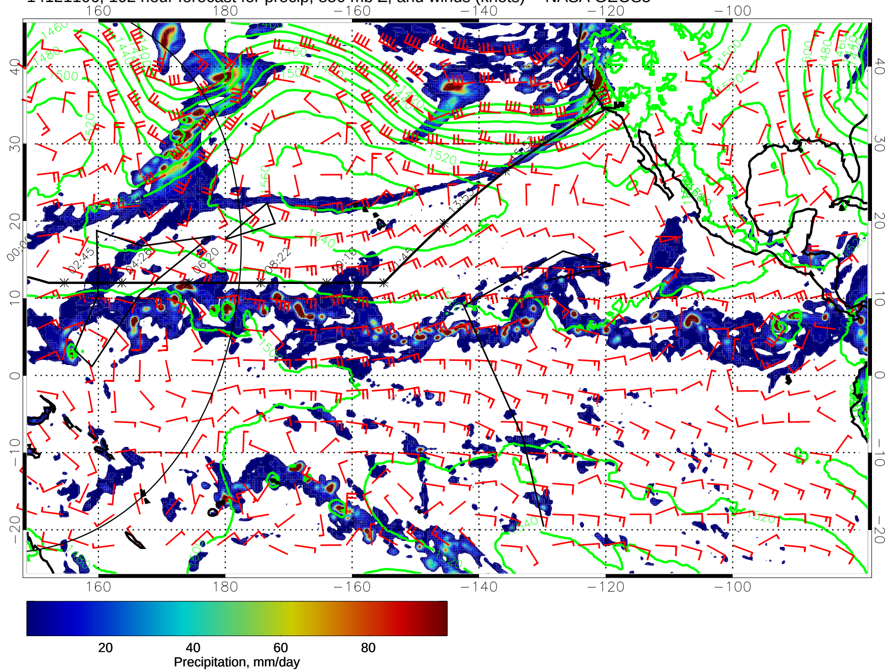
14121106, 102 hour forecast for precip, 850 mb Z, and winds (knots) -- NASA GEOS5
