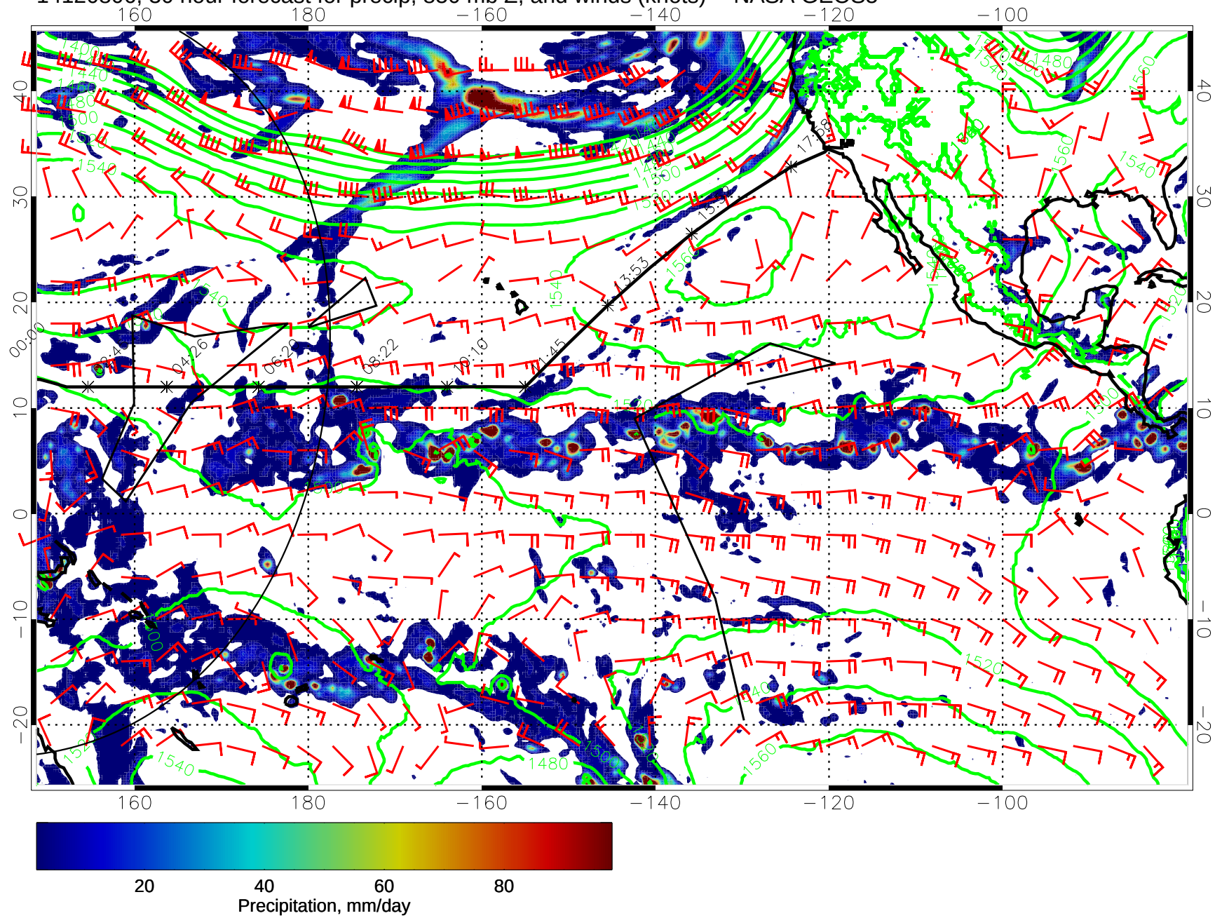
14120806, 30 hour forecast for precip, 850 mb Z, and winds (knots) -- NASA GEOS5
