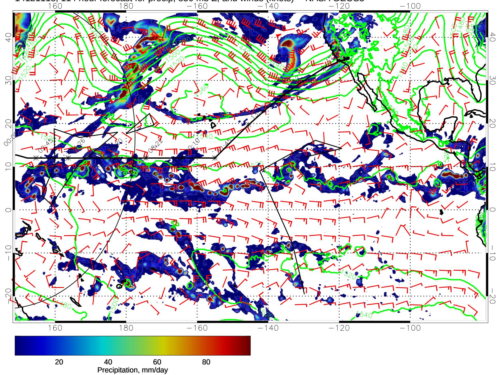
14121118, 114 hour forecast for precip, 850 mb Z, and winds (knots) -- NASA GEOS5
