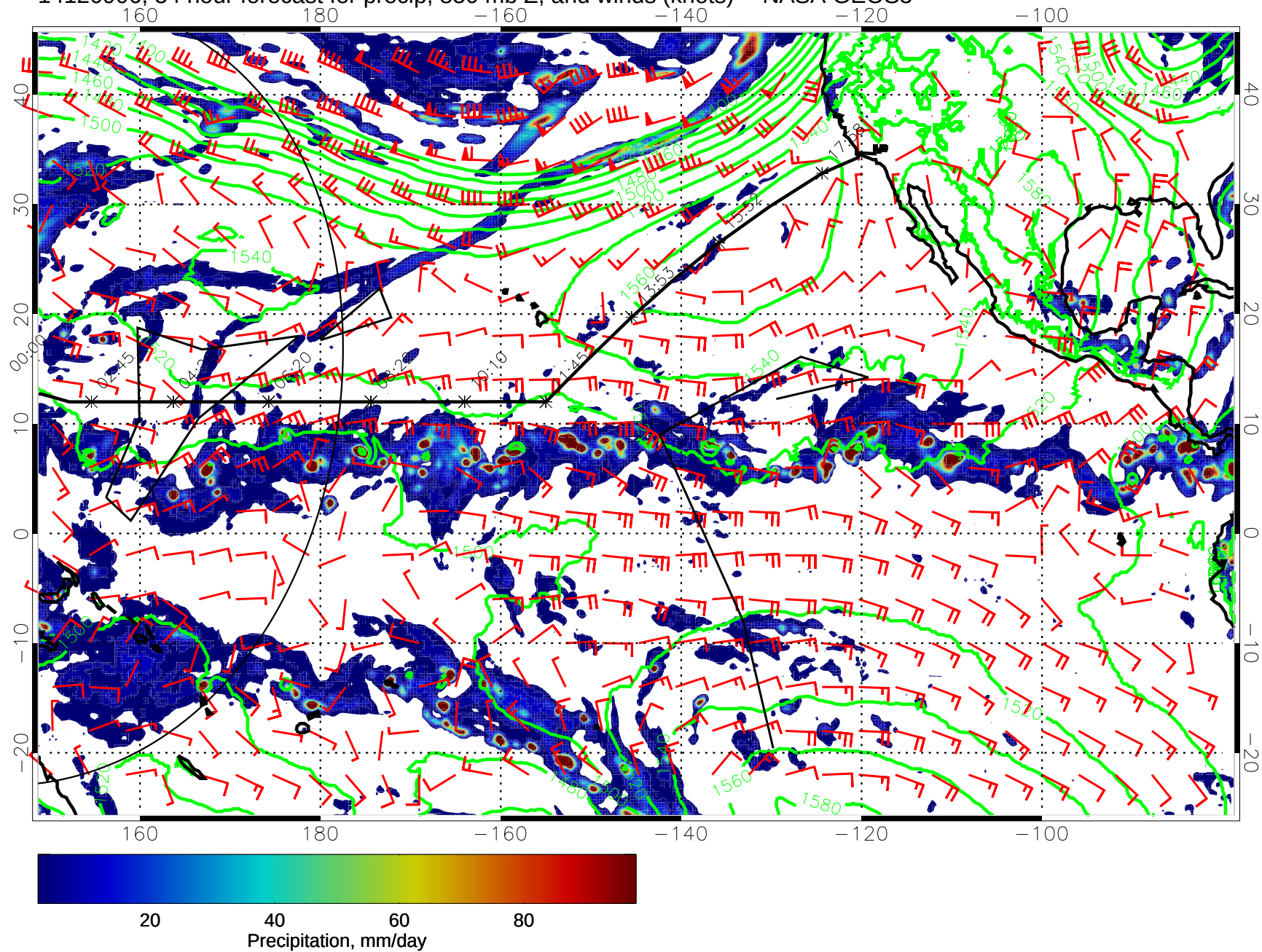
14120906, 54 hour forecast for precip, 850 mb Z, and winds (knots) -- NASA GEOS5
