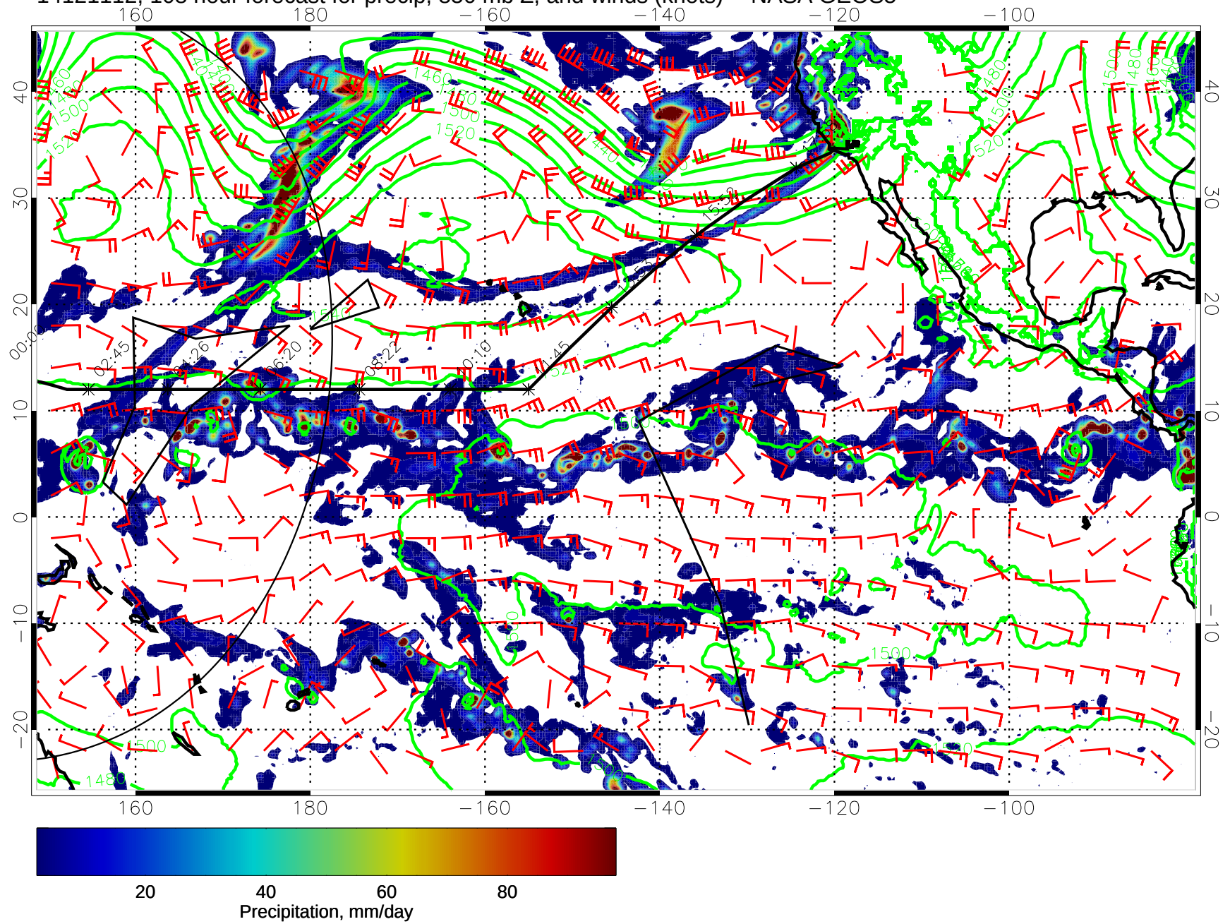
14121112, 108 hour forecast for precip, 850 mb Z, and winds (knots) -- NASA GEOS5
