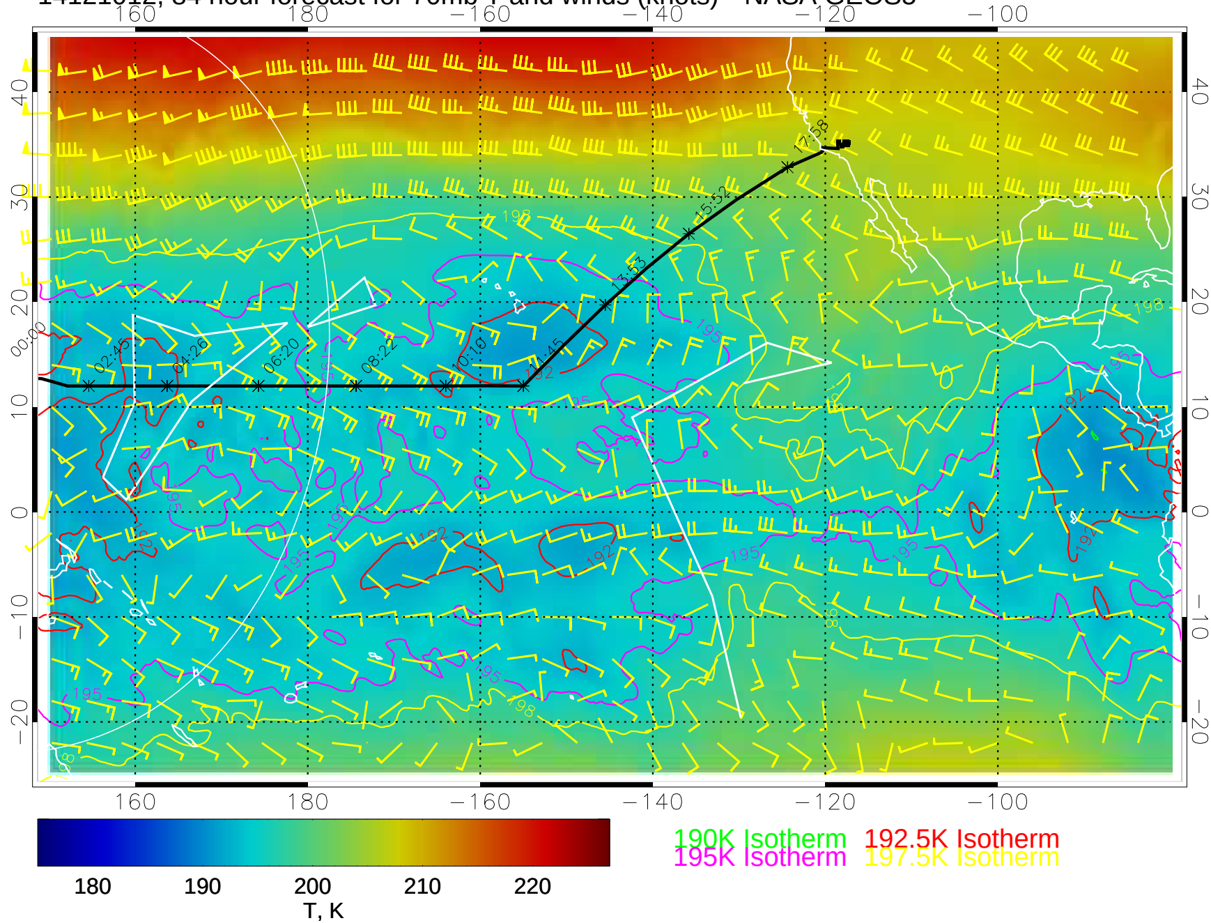
14121012, 84 hour forecast for 70mb T and winds (knots)-- NASA GEOS5
