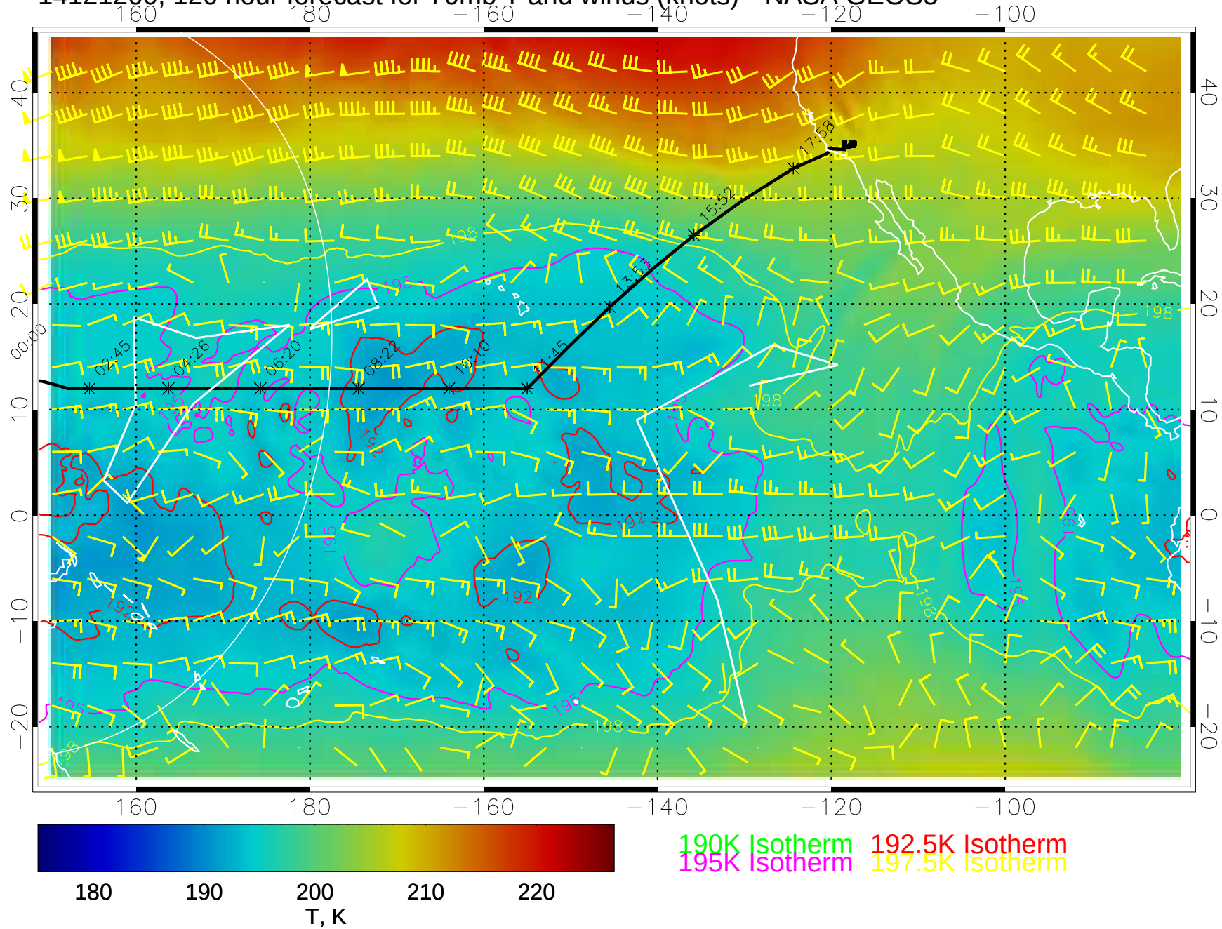
14121200, 120 hour forecast for 70mb T and winds (knots)-- NASA GEOS5
