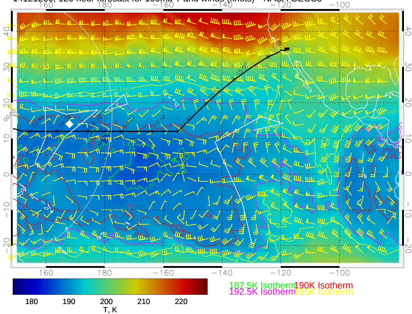
14121200, 120 hour forecast for 100mb T and winds (knots)-- NASA GEOS5
