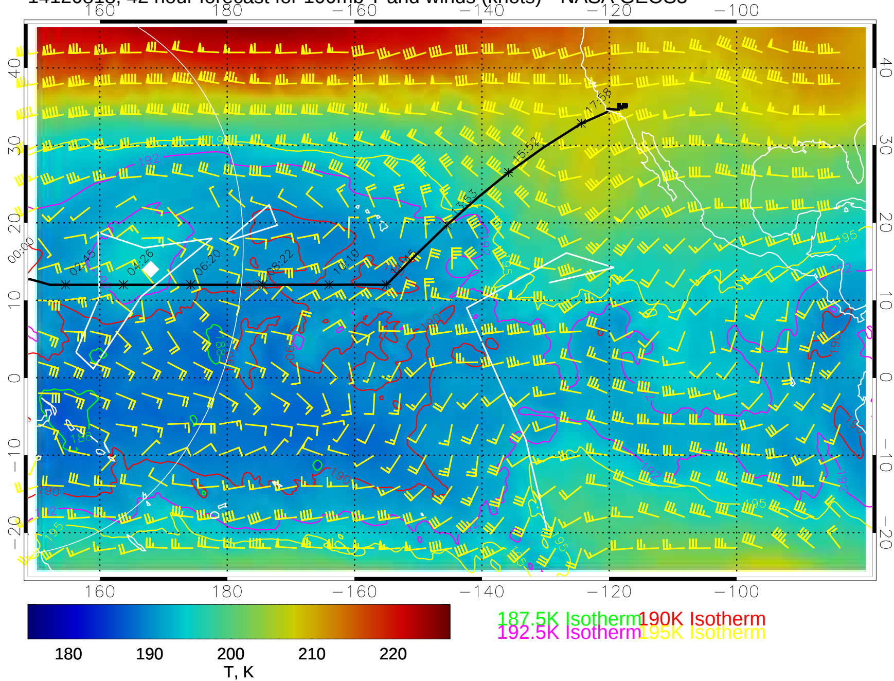
14120818, 42 hour forecast for 100mb T and winds (knots)-- NASA GEOS5
