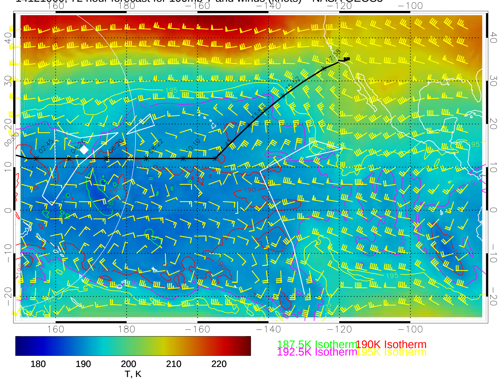
14121000, 72 hour forecast for 100mb T and winds (knots)-- NASA GEOS5
