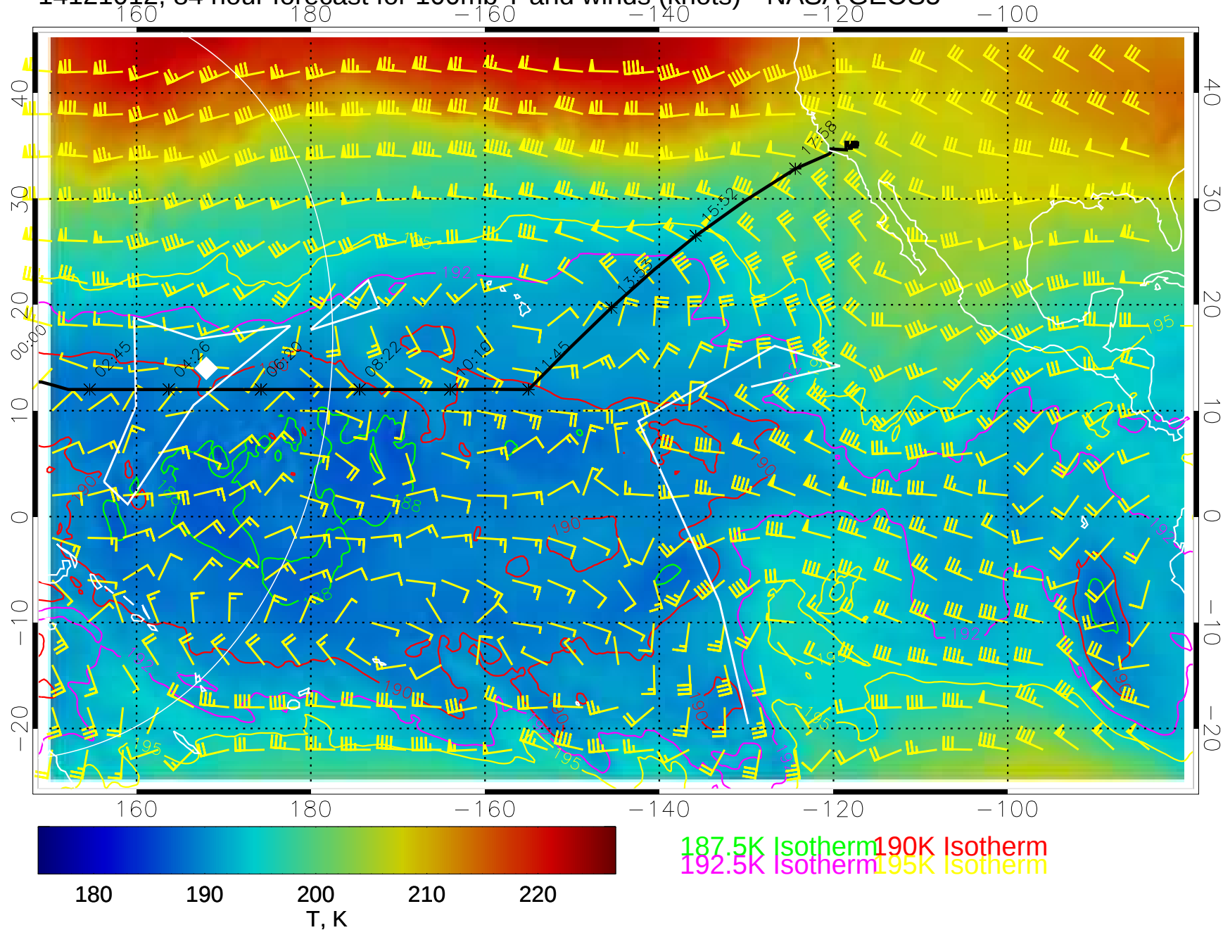
14121012, 84 hour forecast for 100mb T and winds (knots)-- NASA GEOS5
