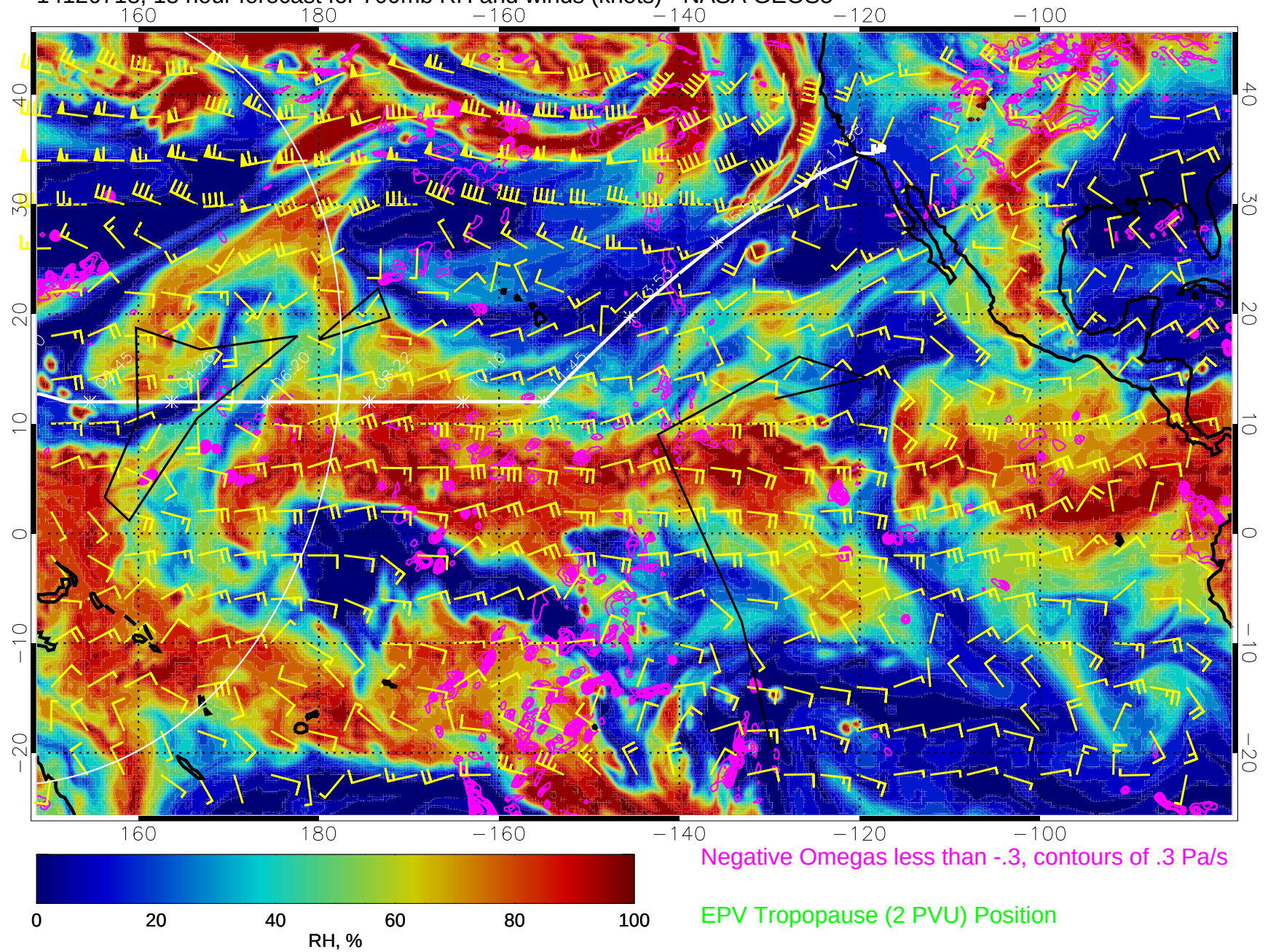
14120718, 18 hour forecast for 700mb RH and winds (knots) - NASA GEOS5
