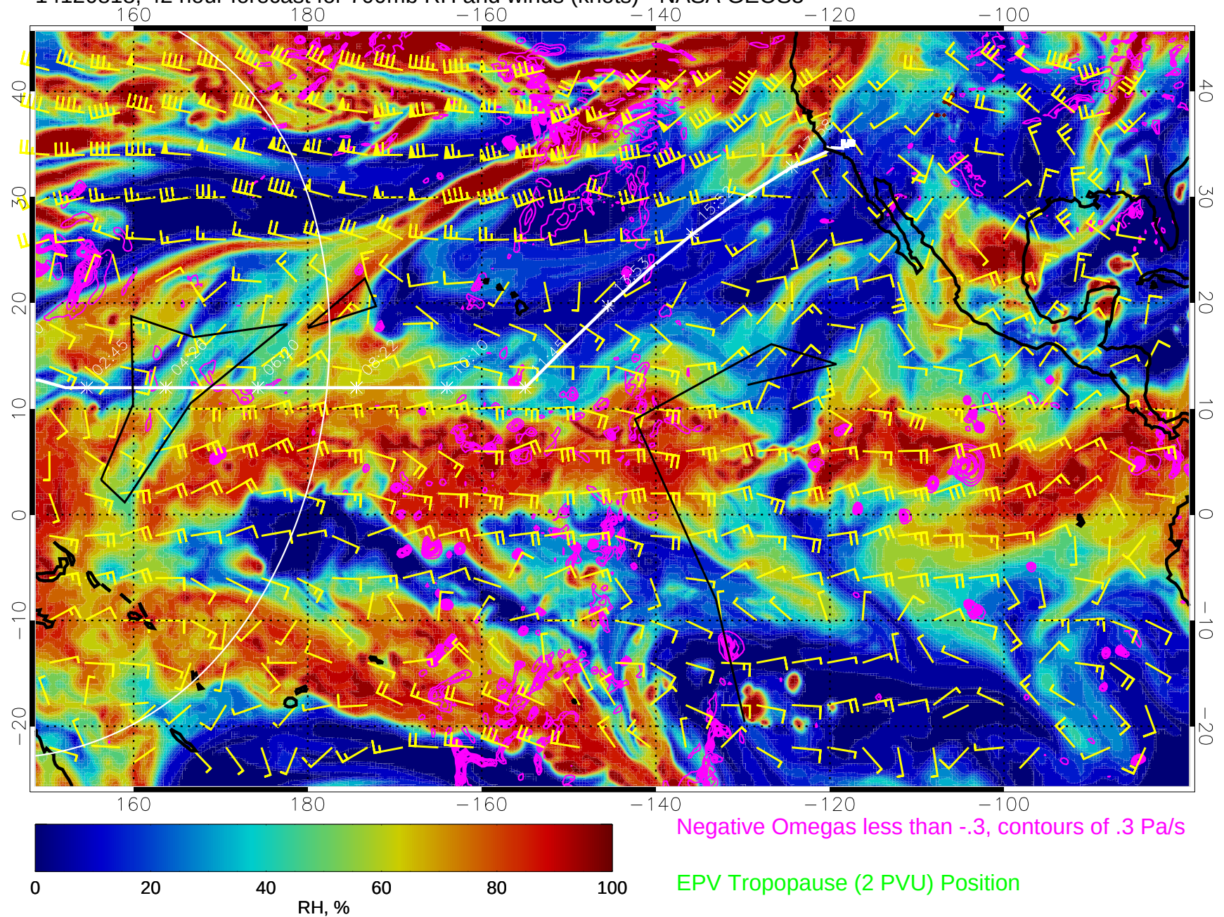
14120818, 42 hour forecast for 700mb RH and winds (knots) - NASA GEOS5
