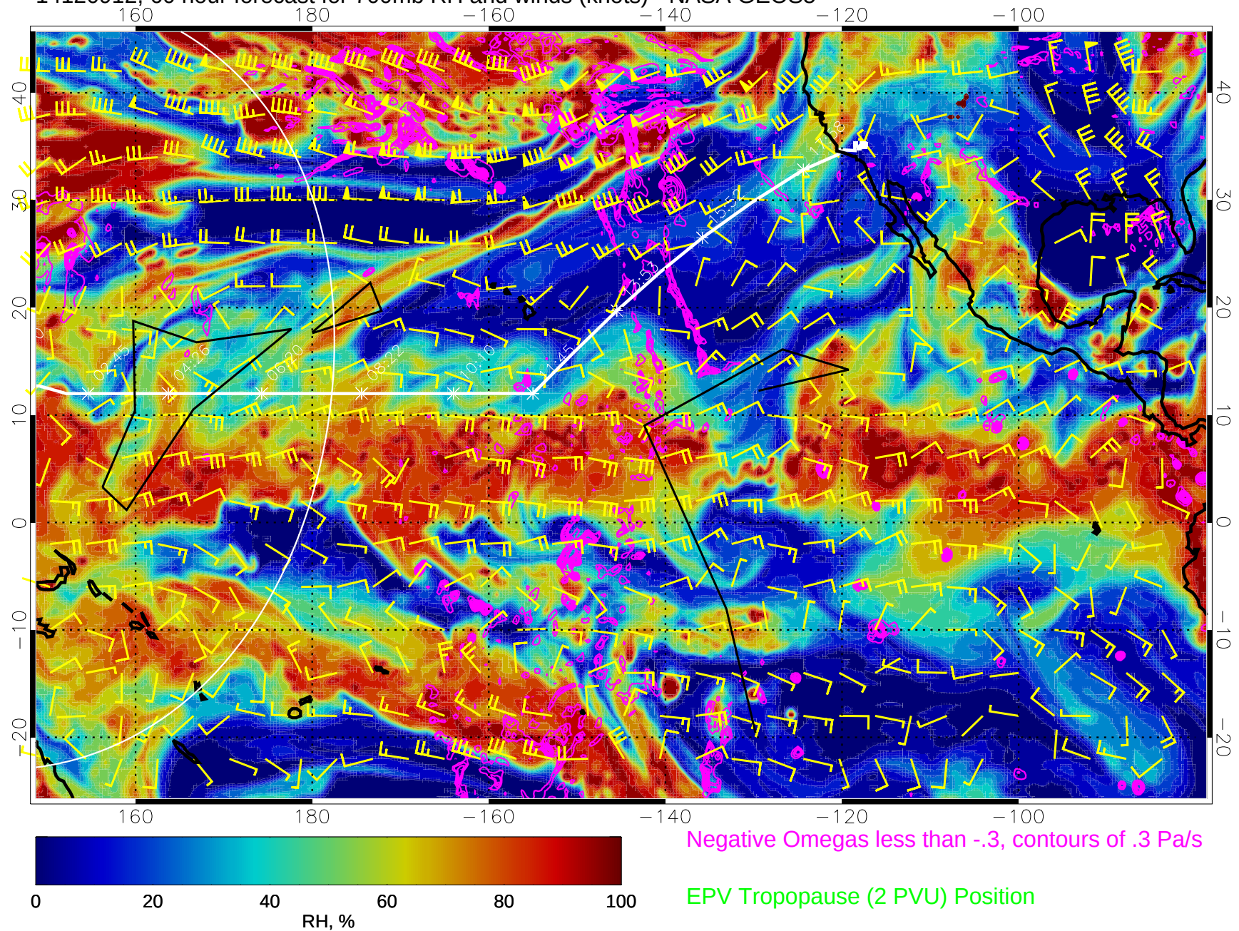
14120912, 60 hour forecast for 700mb RH and winds (knots) - NASA GEOS5
