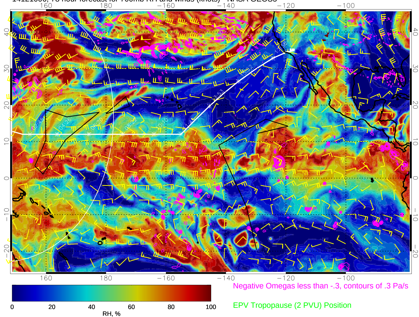
14121006, 78 hour forecast for 700mb RH and winds (knots) - NASA GEOS5
