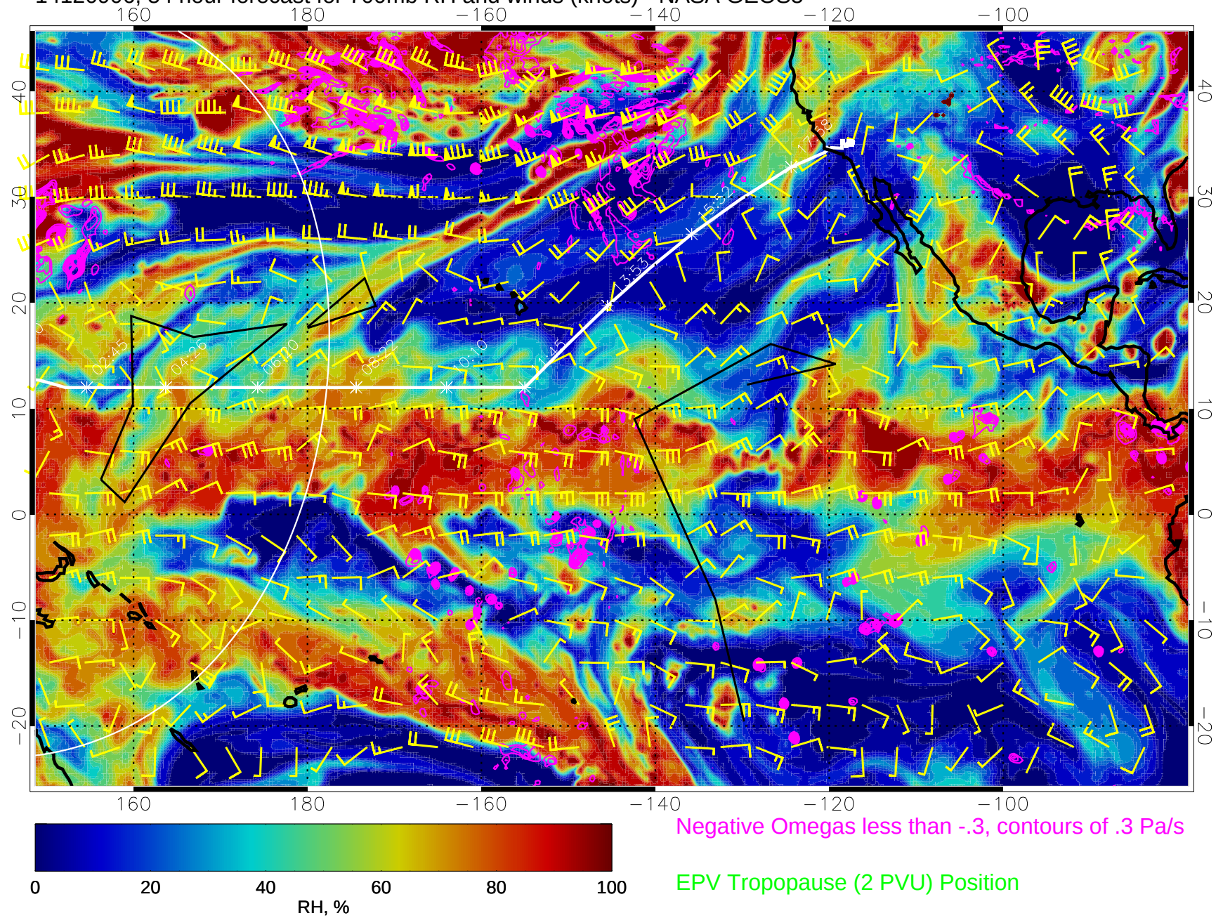
14120906, 54 hour forecast for 700mb RH and winds (knots) - NASA GEOS5
