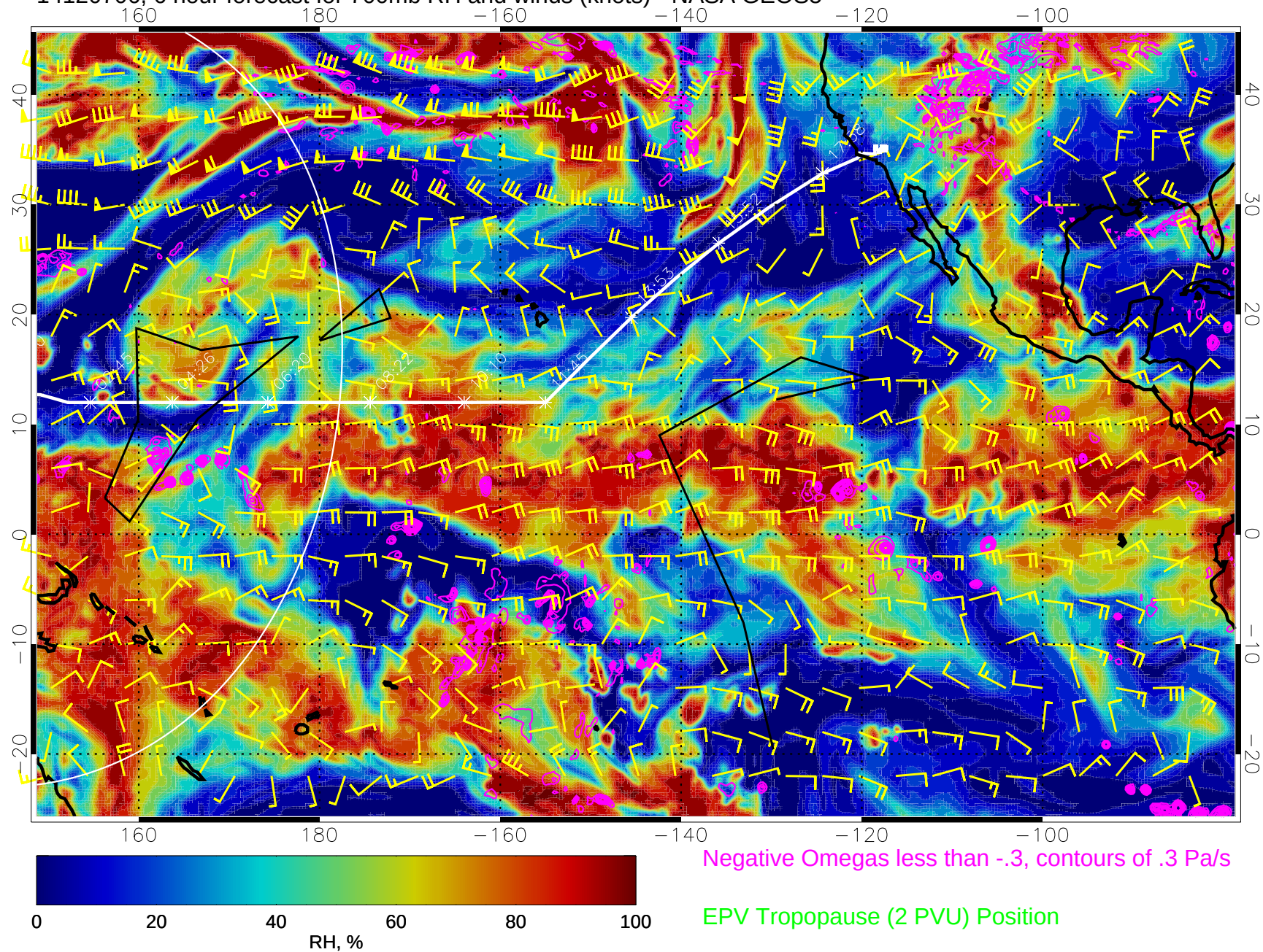
14120706, 6 hour forecast for 700mb RH and winds (knots) - NASA GEOS5
