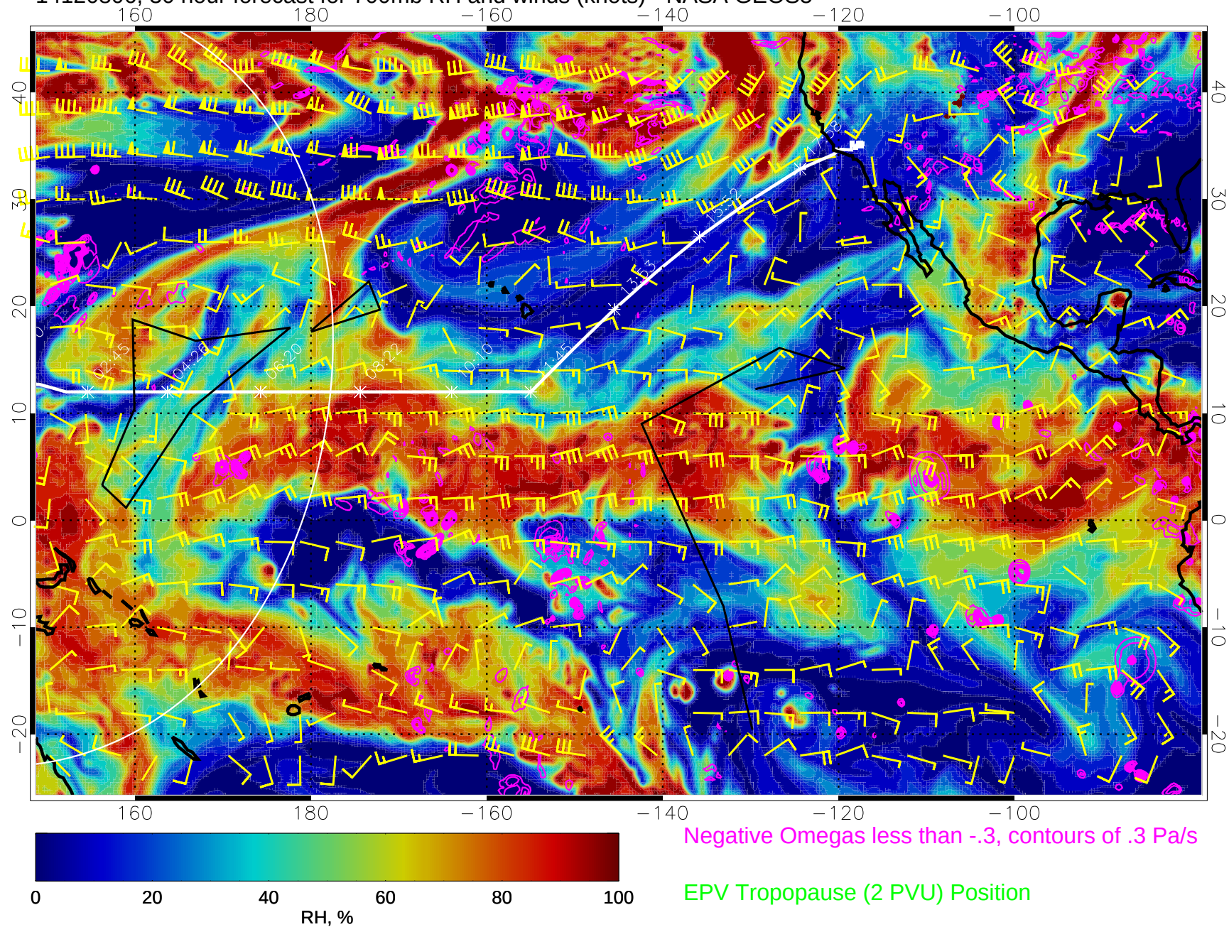
14120806, 30 hour forecast for 700mb RH and winds (knots) - NASA GEOS5
