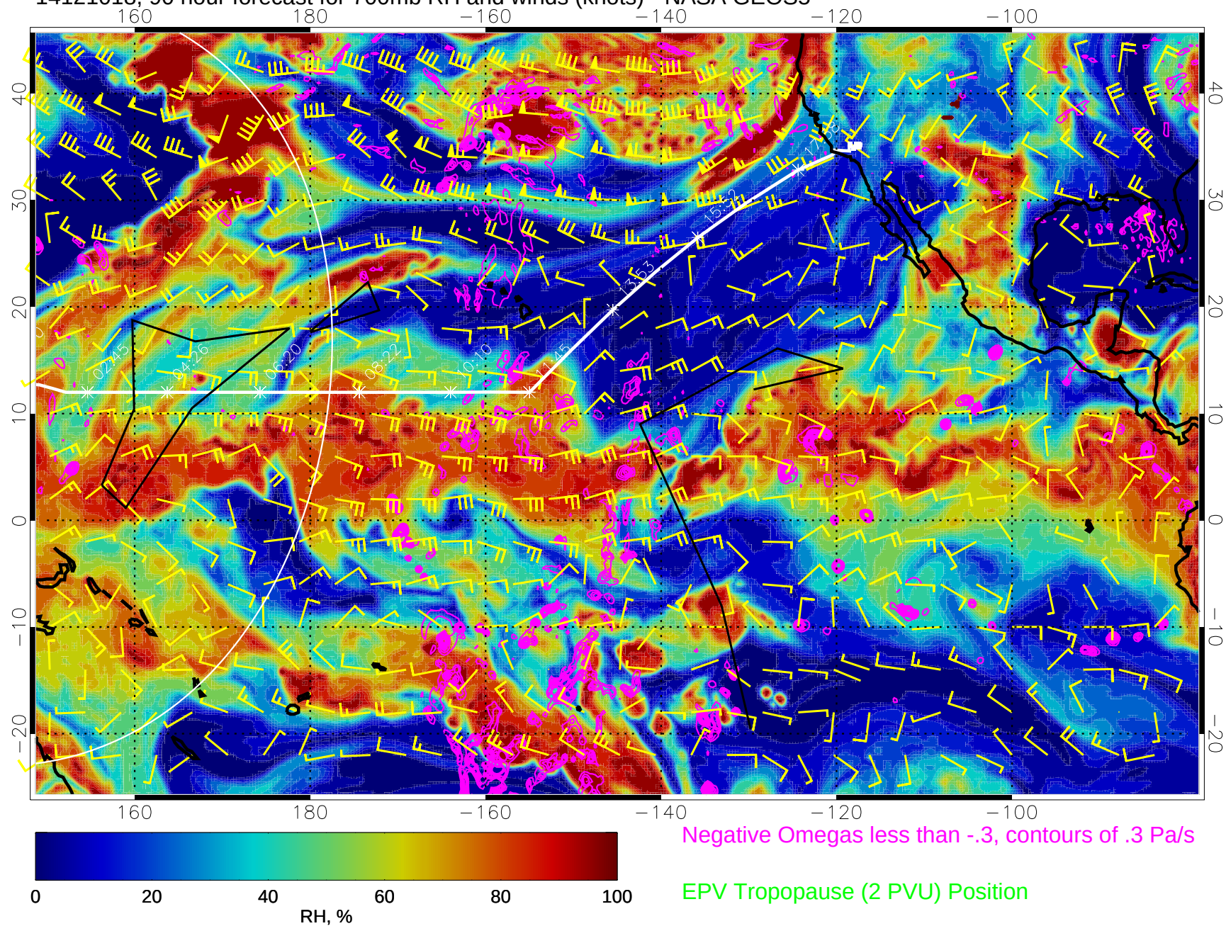
14121018, 90 hour forecast for 700mb RH and winds (knots) - NASA GEOS5
