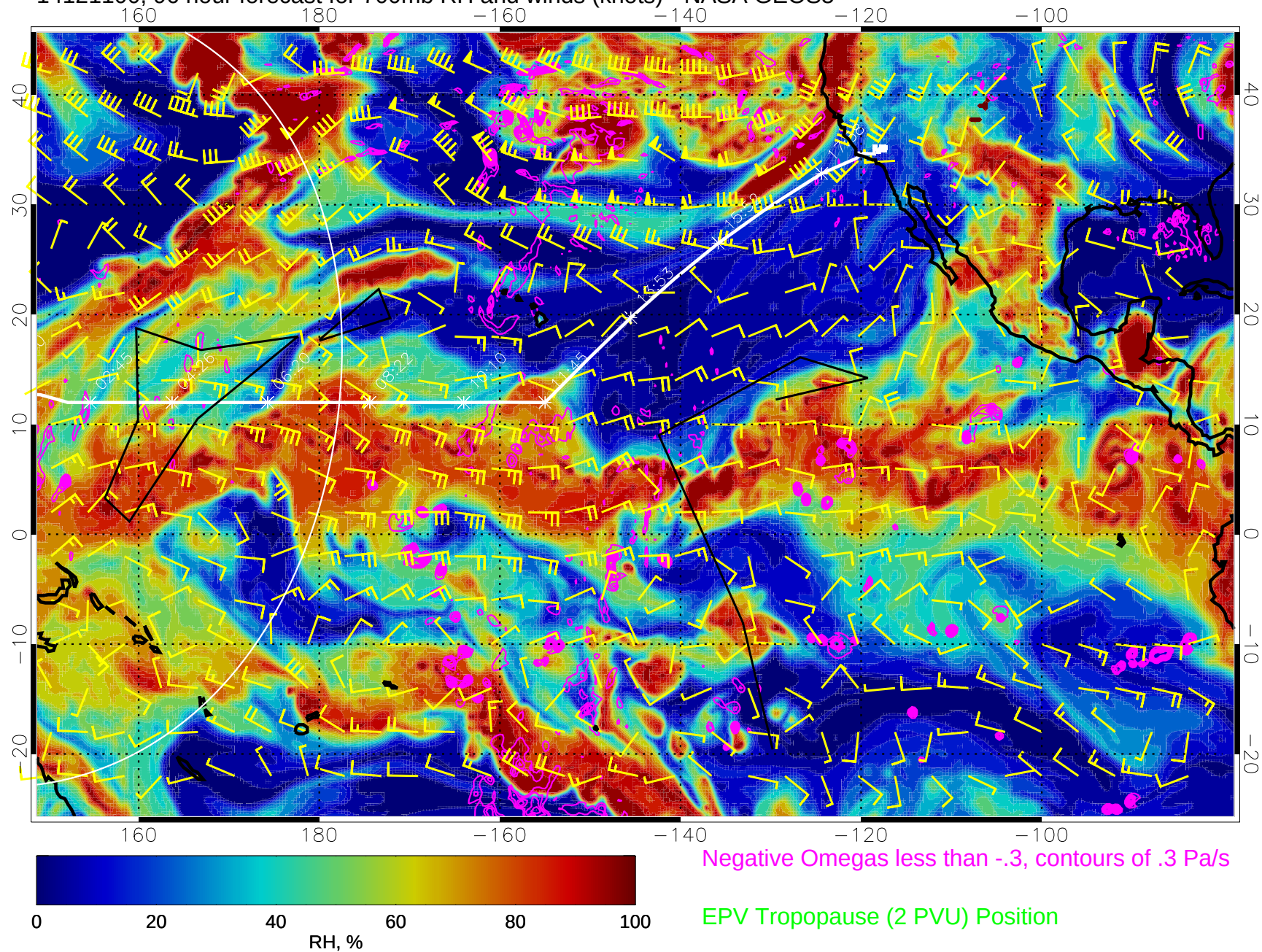
14121100, 96 hour forecast for 700mb RH and winds (knots) - NASA GEOS5
