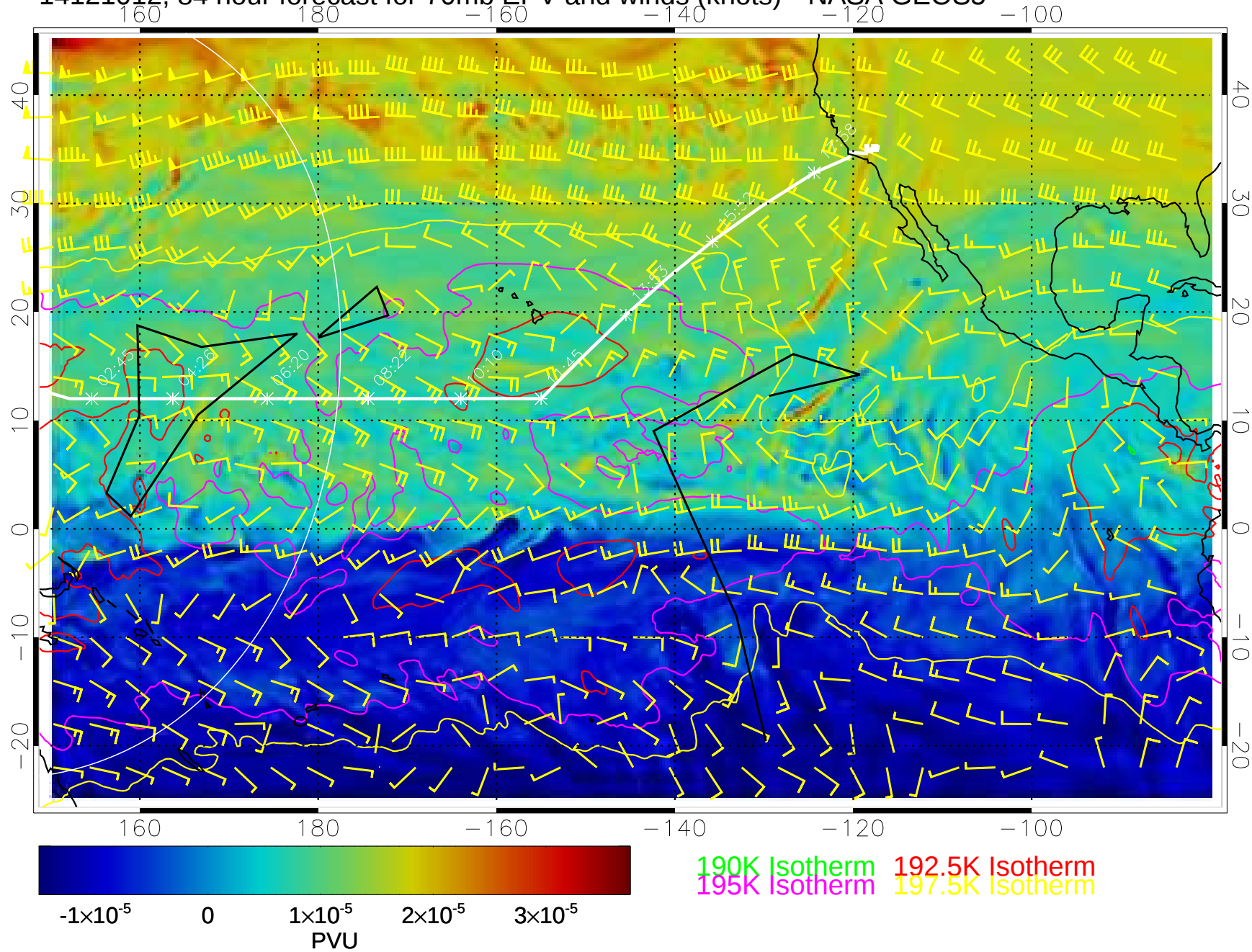
14121012, 84 hour forecast for 70mb EPV and winds (knots)-- NASA GEOS5
