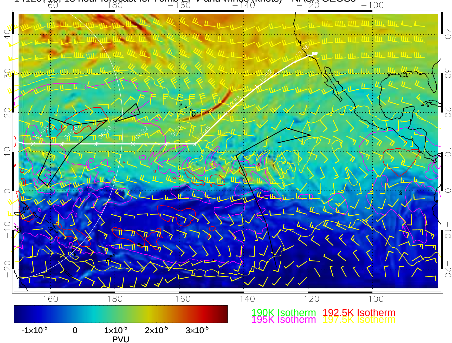
14120718, 18 hour forecast for 70mb EPV and winds (knots)-- NASA GEOS5
