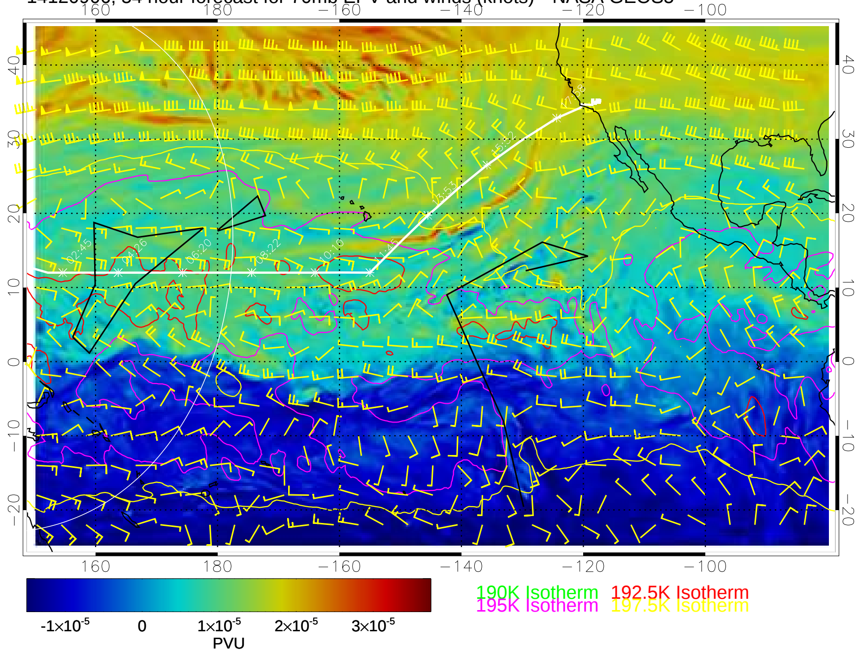
14120906, 54 hour forecast for 70mb EPV and winds (knots)-- NASA GEOS5
