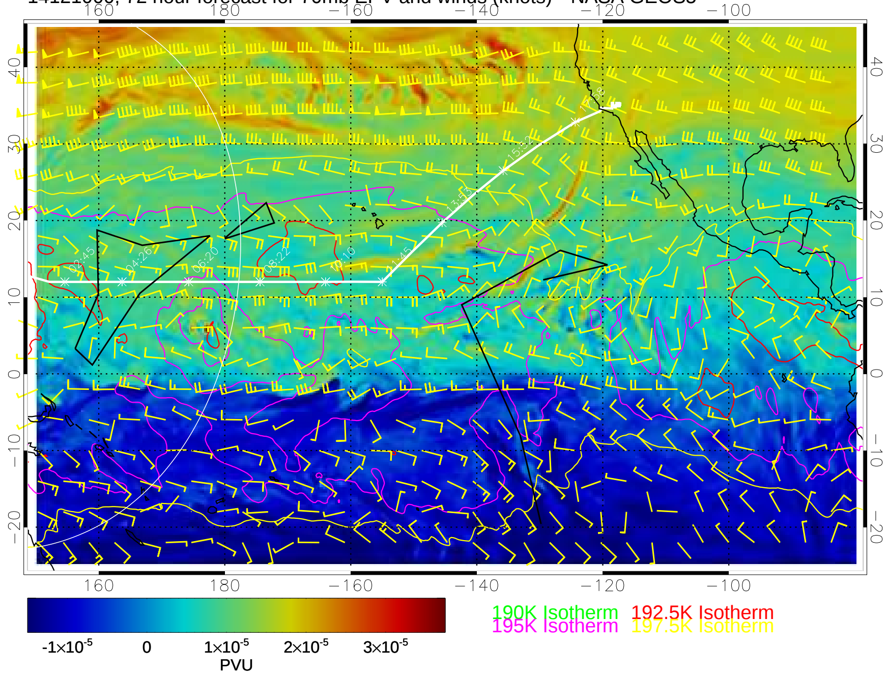
14121000, 72 hour forecast for 70mb EPV and winds (knots)-- NASA GEOS5
