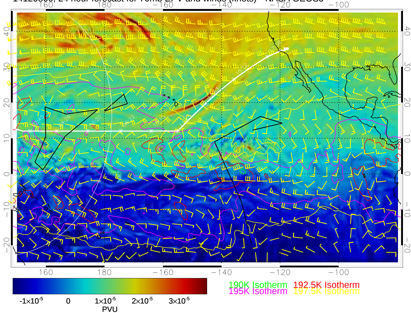
14120800, 24 hour forecast for 70mb EPV and winds (knots)-- NASA GEOS5
