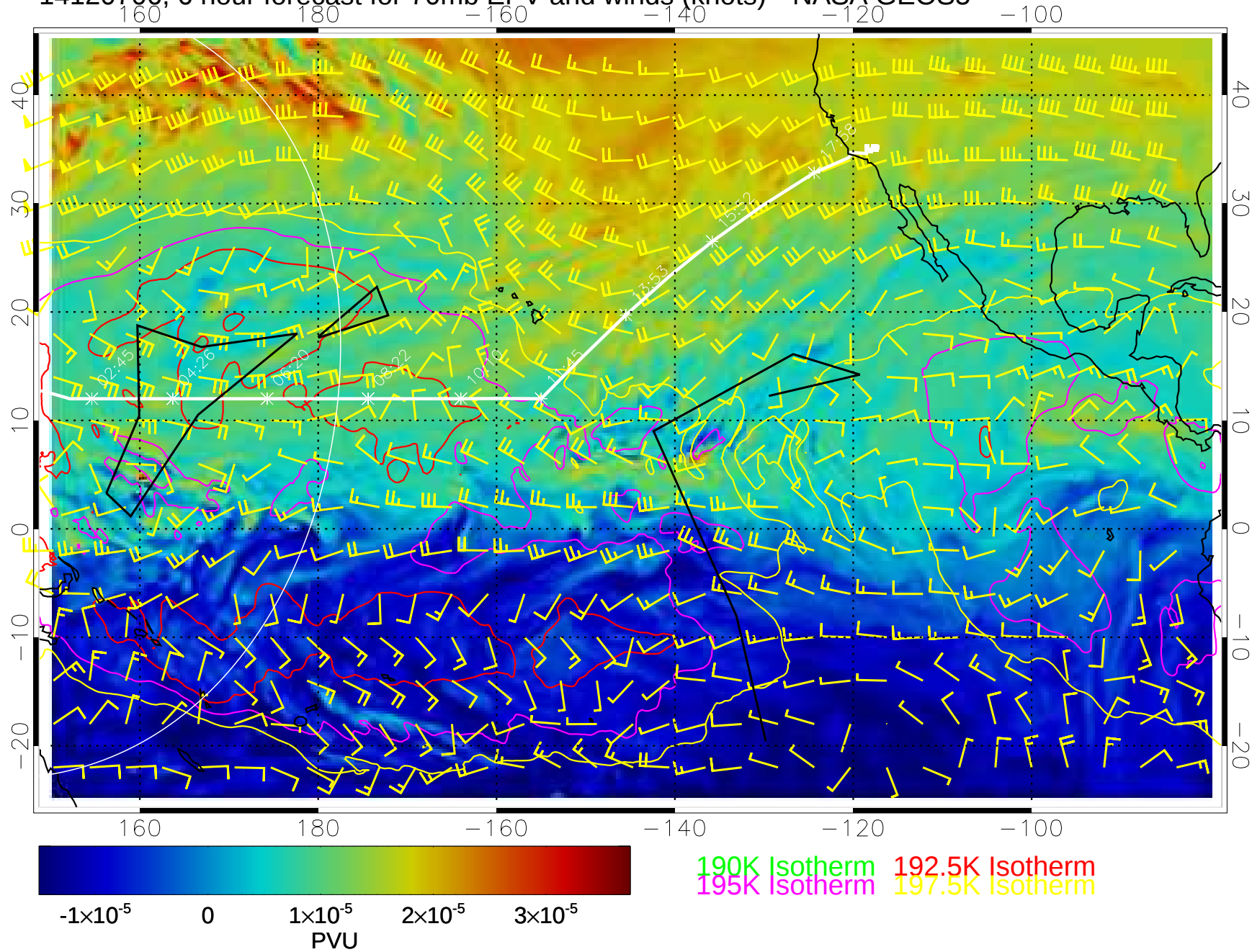
14120706, 6 hour forecast for 70mb EPV and winds (knots)-- NASA GEOS5
