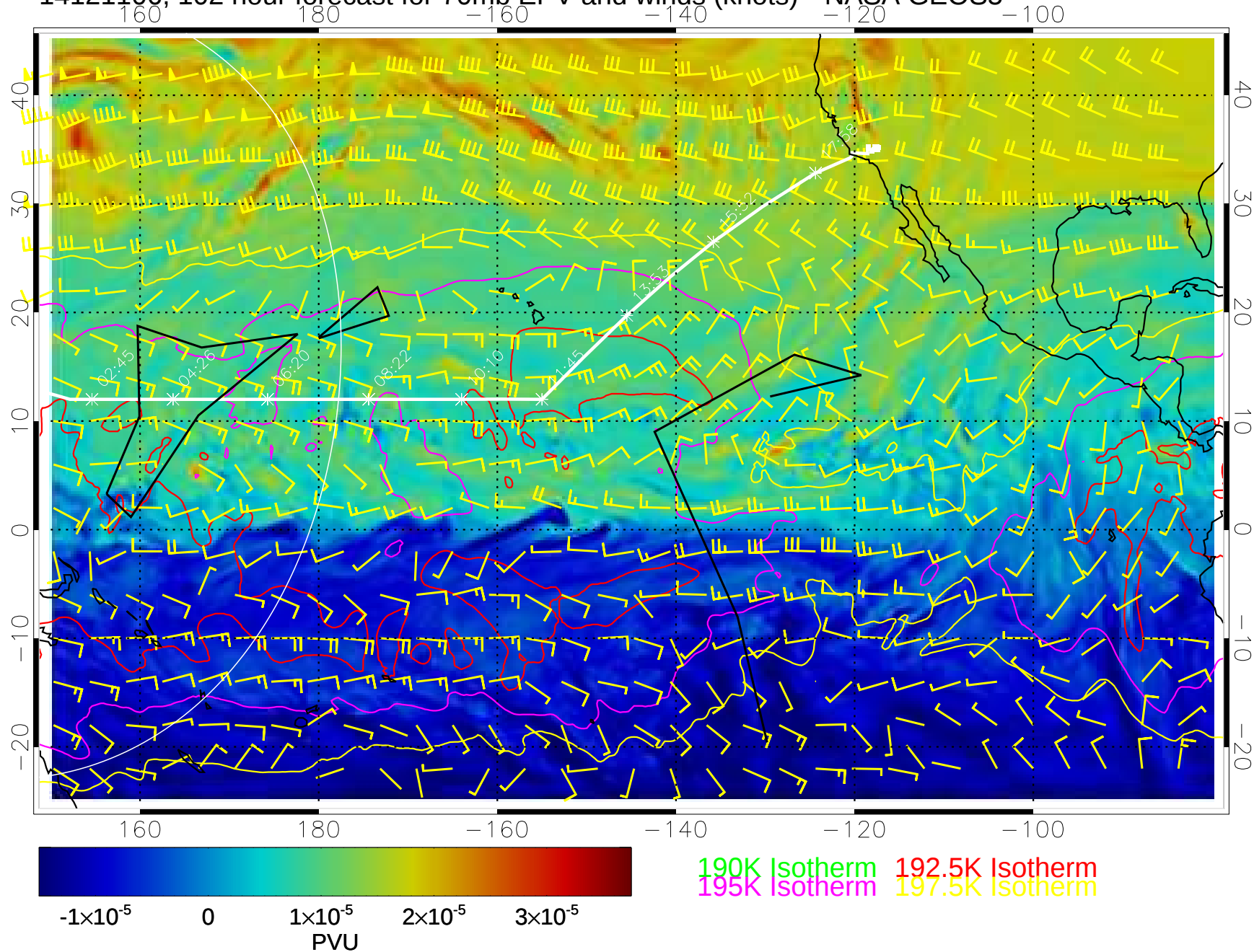
14121106, 102 hour forecast for 70mb EPV and winds (knots)-- NASA GEOS5
