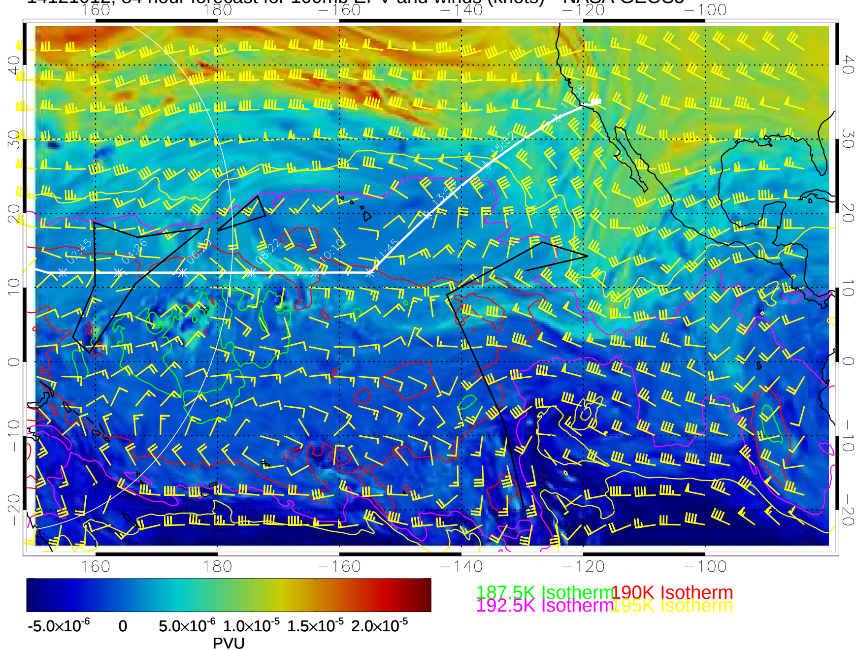
14121012, 84 hour forecast for 100mb EPV and winds (knots)-- NASA GEOS5
