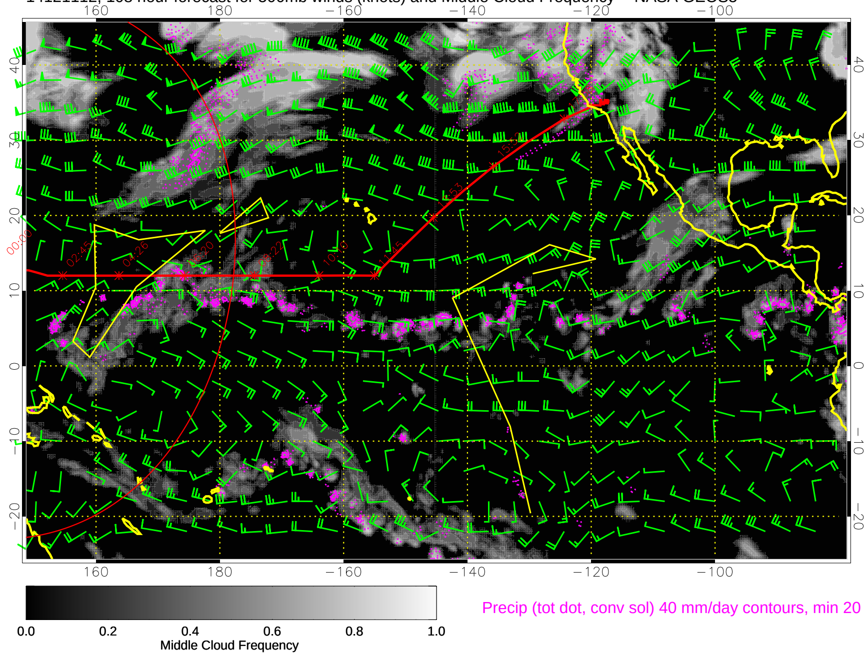
14121112, 108 hour forecast for 500mb winds (knots) and Middle Cloud Frequency -- NASA GEOS5
