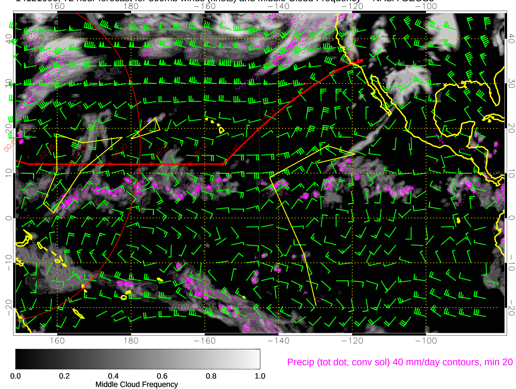
14121000, 72 hour forecast for 500mb winds (knots) and Middle Cloud Frequency -- NASA GEOS5
