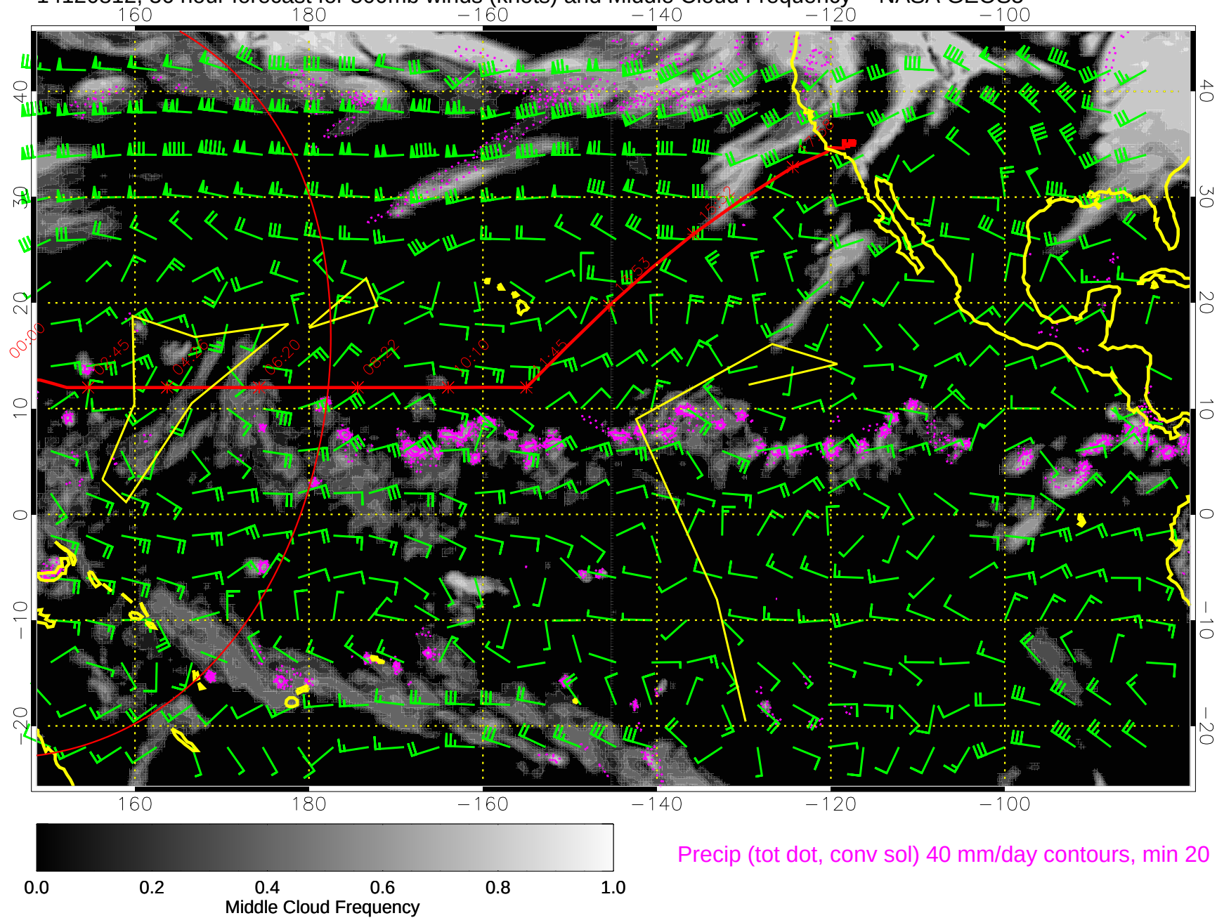
14120812, 36 hour forecast for 500mb winds (knots) and Middle Cloud Frequency -- NASA GEOS5
