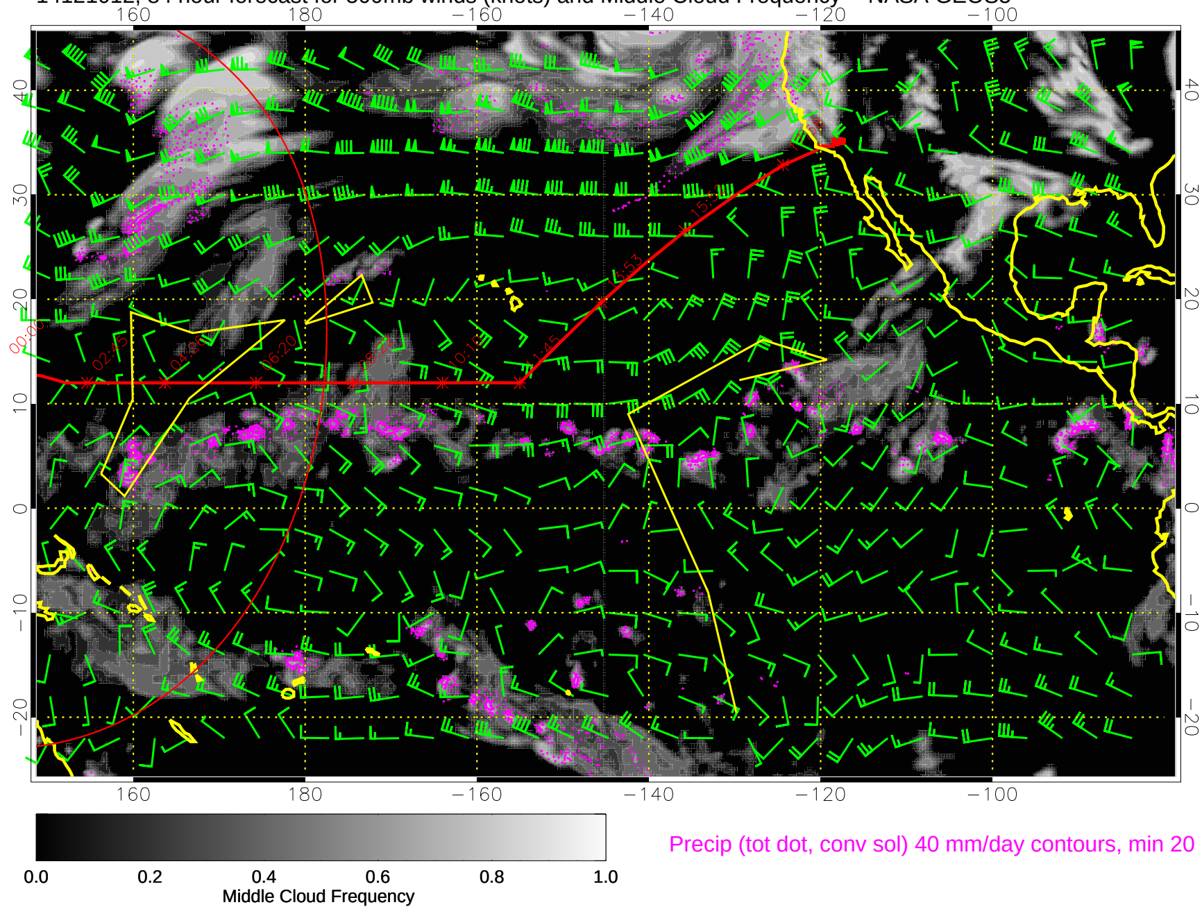
14121012, 84 hour forecast for 500mb winds (knots) and Middle Cloud Frequency -- NASA GEOS5
