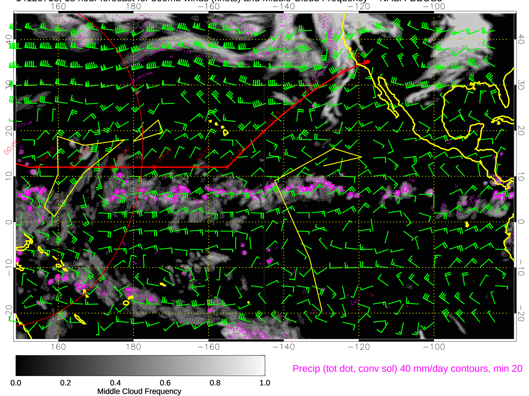
14120718, 18 hour forecast for 500mb winds (knots) and Middle Cloud Frequency -- NASA GEOS5
