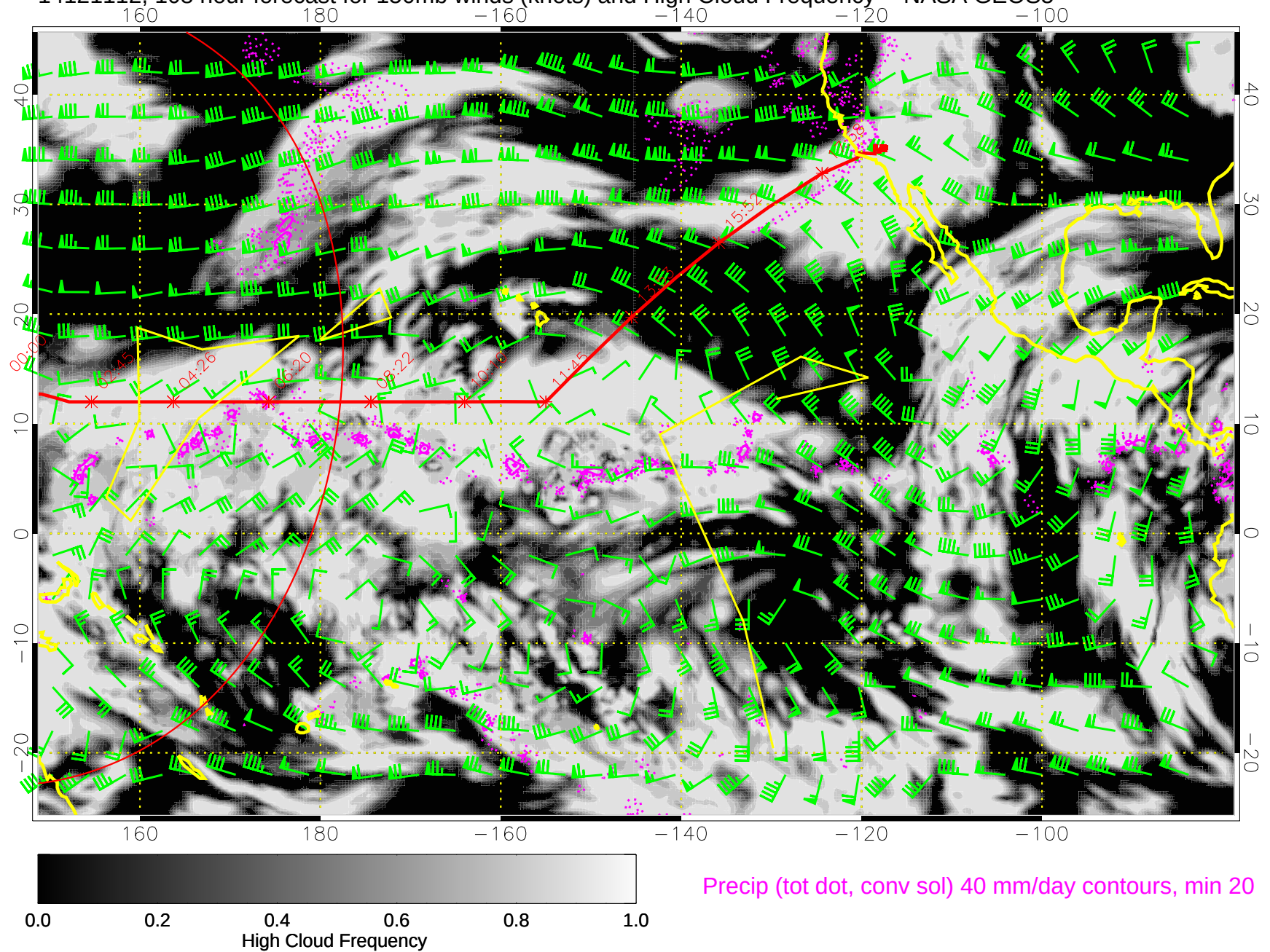
14121112, 108 hour forecast for 150mb winds (knots) and High Cloud Frequency -- NASA GEOS5
