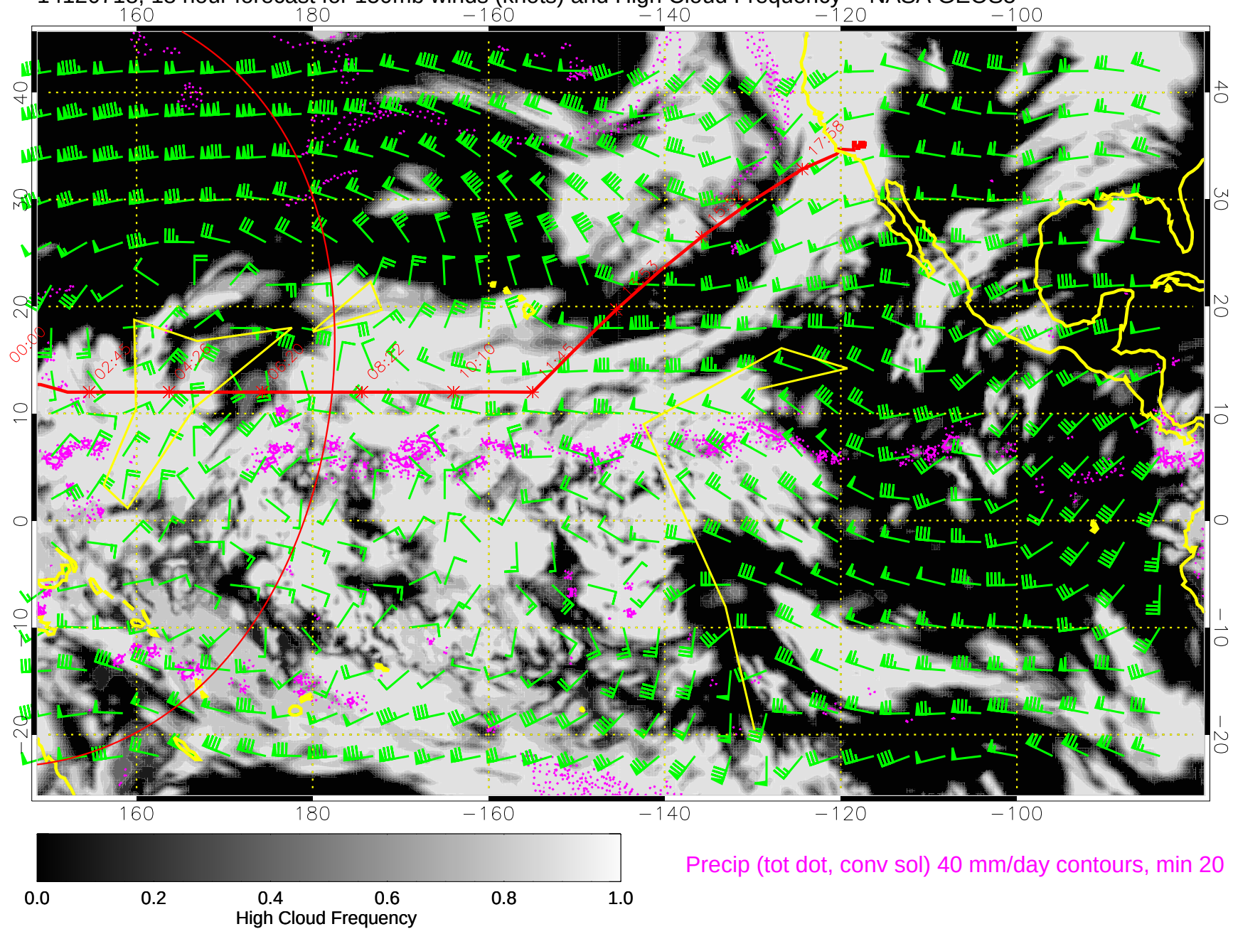
14120718, 18 hour forecast for 150mb winds (knots) and High Cloud Frequency -- NASA GEOS5
