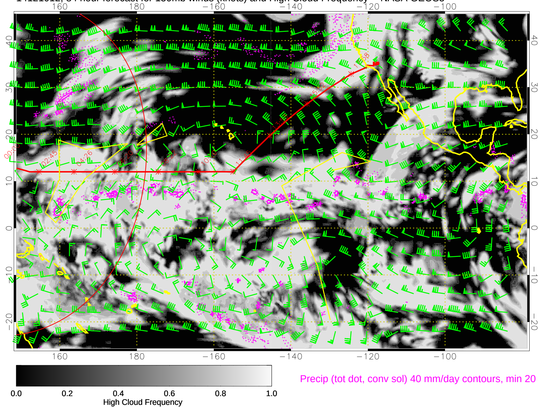
14121012, 84 hour forecast for 150mb winds (knots) and High Cloud Frequency -- NASA GEOS5
