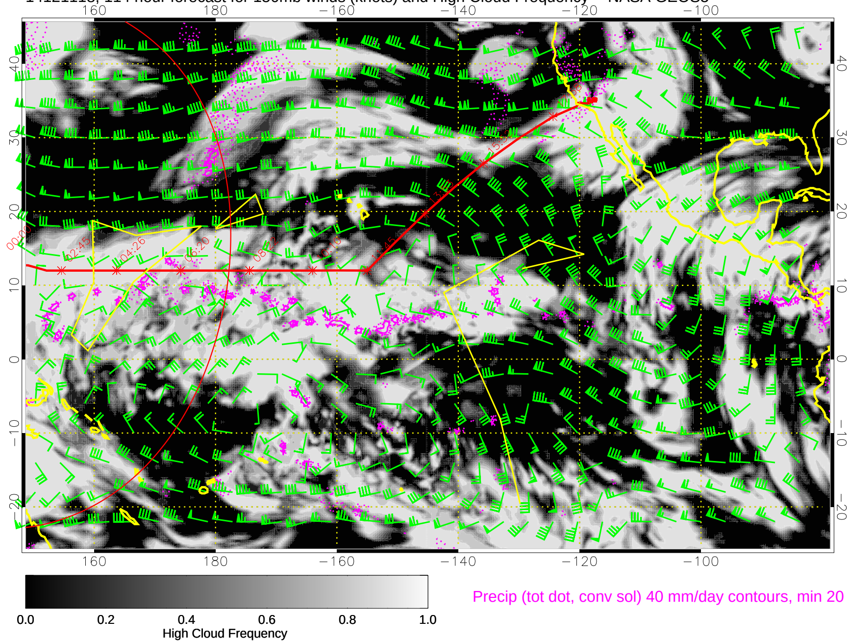
14121118, 114 hour forecast for 150mb winds (knots) and High Cloud Frequency -- NASA GEOS5
