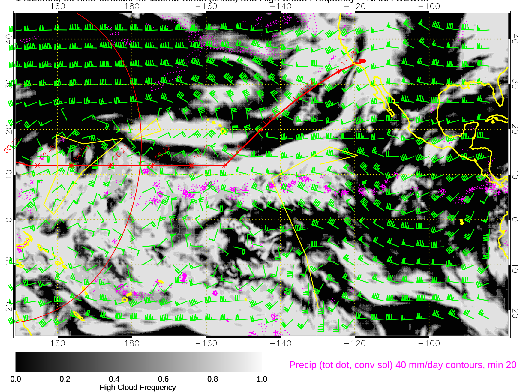
14120806, 30 hour forecast for 150mb winds (knots) and High Cloud Frequency -- NASA GEOS5
