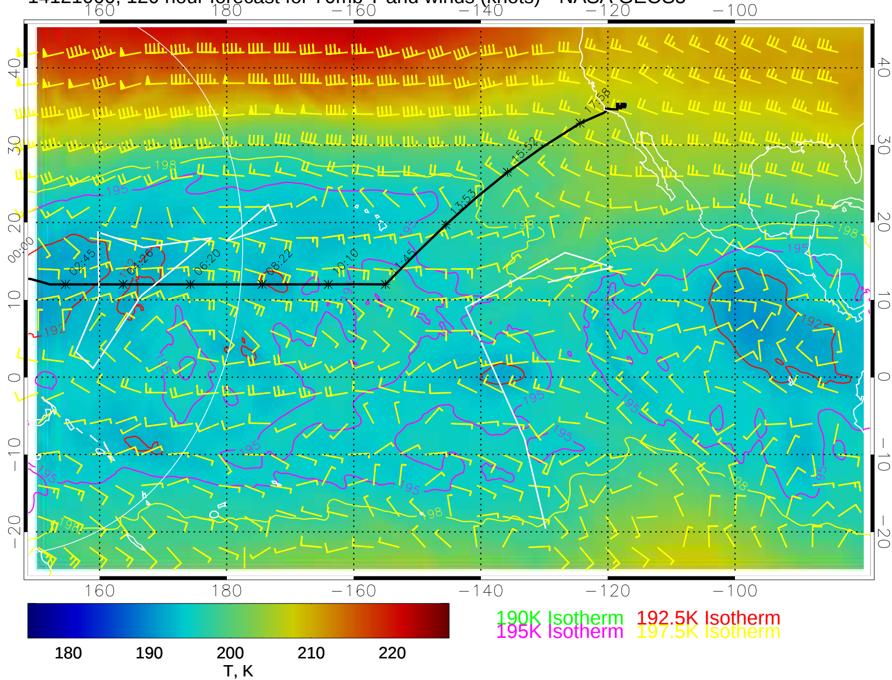
14121000, 120 hour forecast for 70mb T and winds (knots)-- NASA GEOS5
