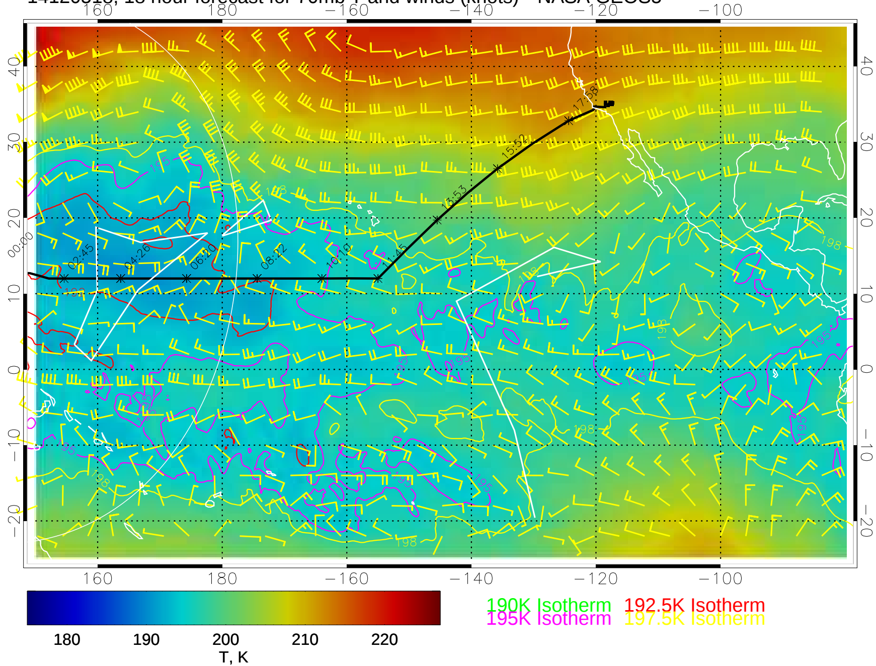
14120518, 18 hour forecast for 70mb T and winds (knots)-- NASA GEOS5
