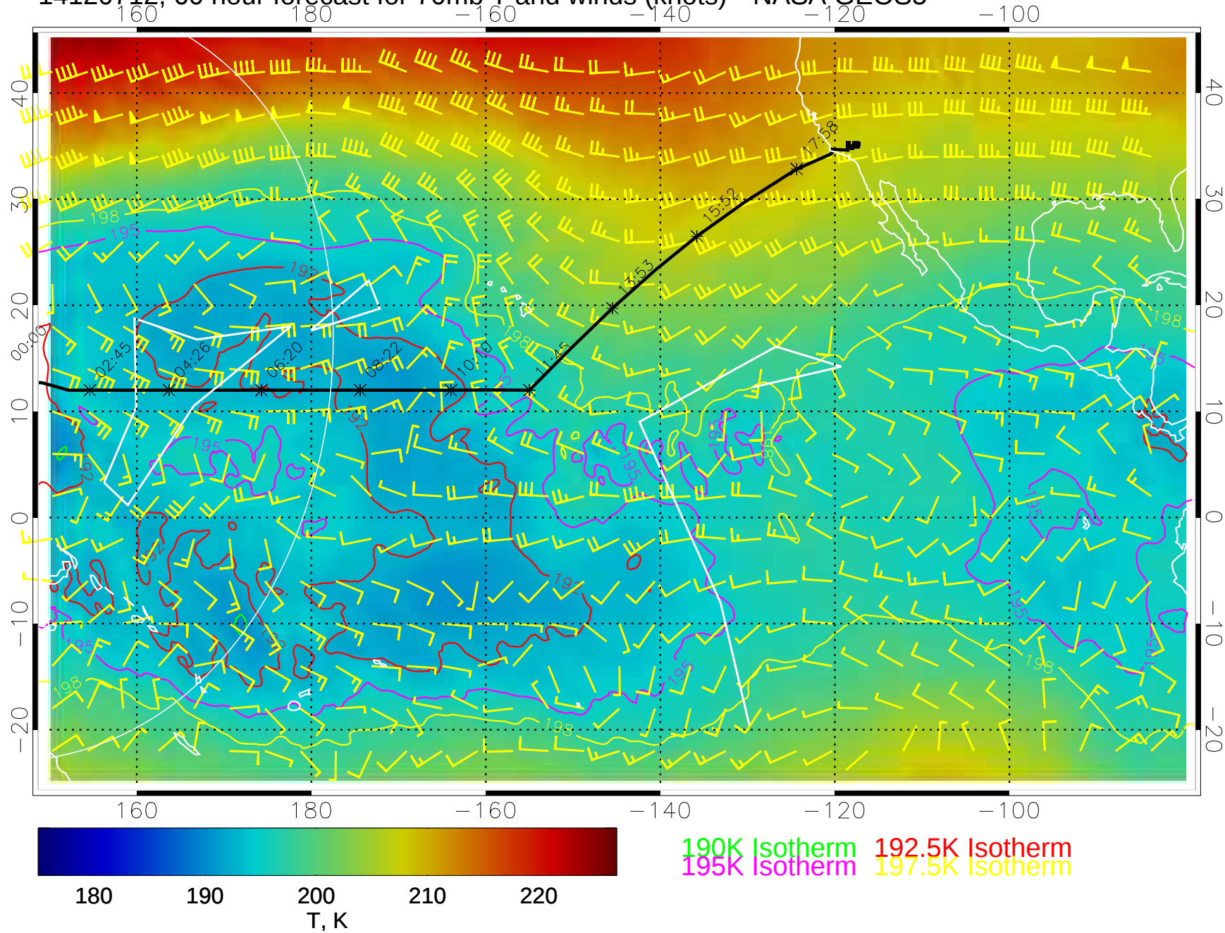
14120712, 60 hour forecast for 70mb T and winds (knots)-- NASA GEOS5
