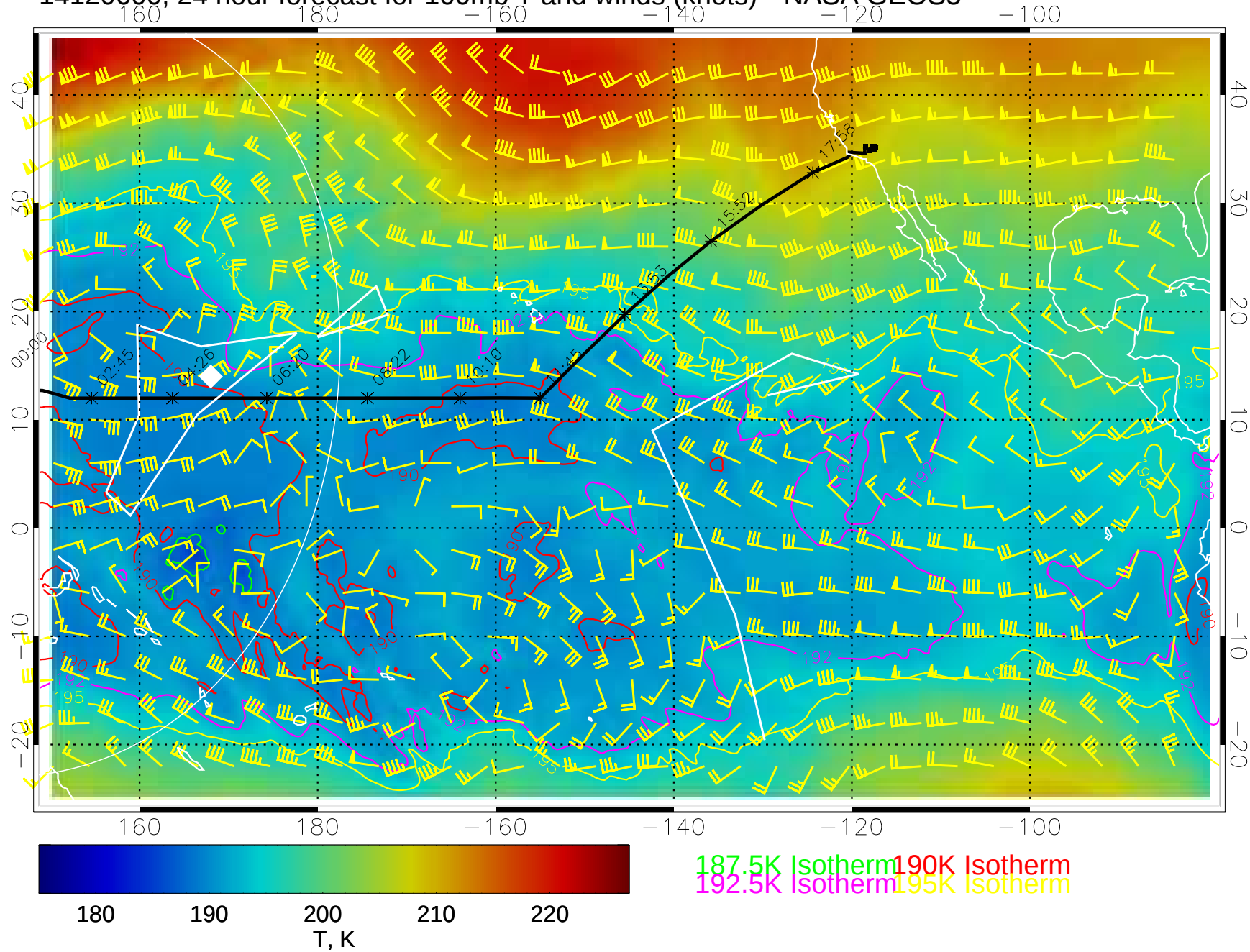
14120600, 24 hour forecast for 100mb T and winds (knots)-- NASA GEOS5
