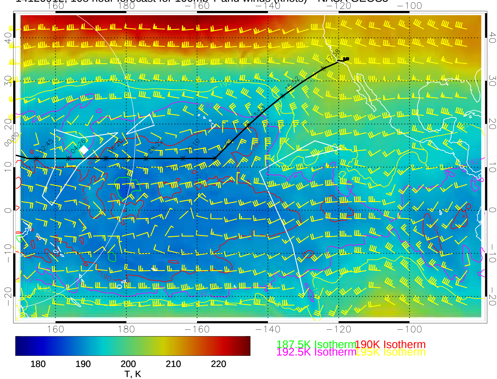
14120912, 108 hour forecast for 100mb T and winds (knots)-- NASA GEOS5
