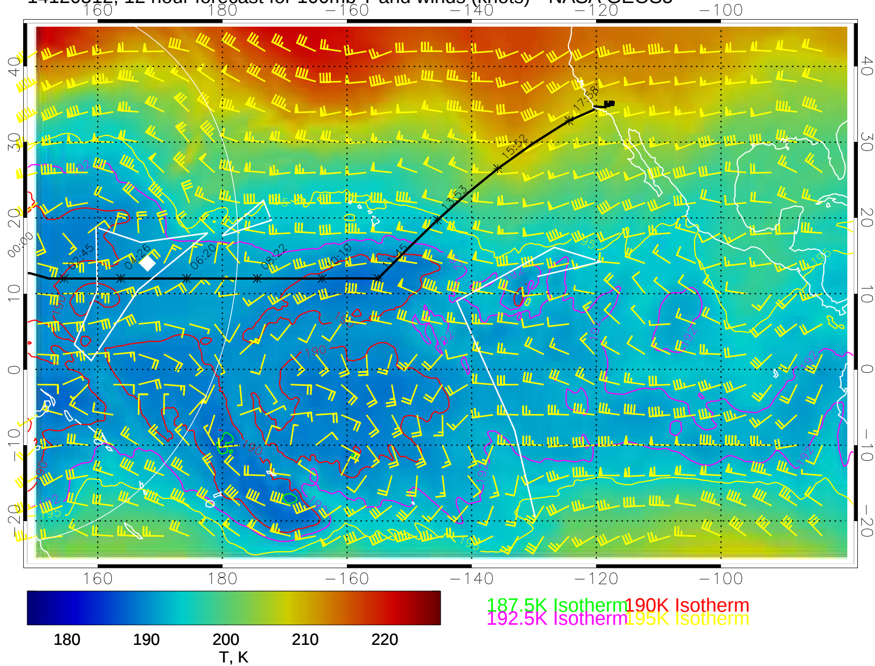
14120512, 12 hour forecast for 100mb T and winds (knots)-- NASA GEOS5
