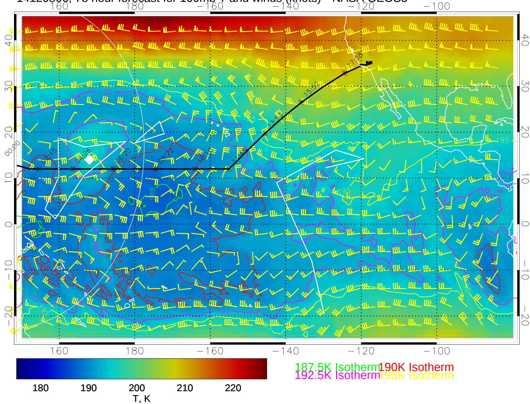
14120806, 78 hour forecast for 100mb T and winds (knots)-- NASA GEOS5
