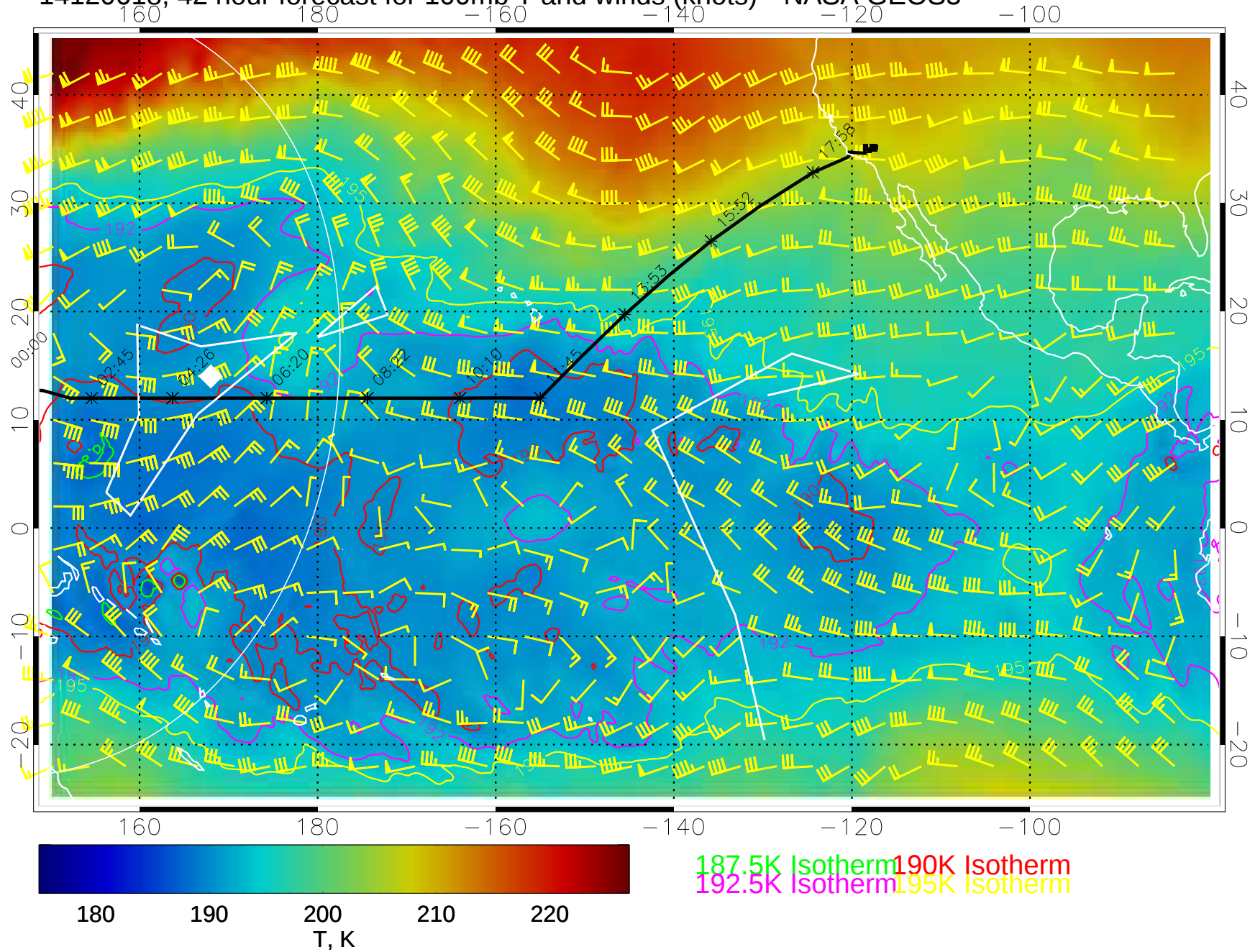
14120618, 42 hour forecast for 100mb T and winds (knots)-- NASA GEOS5
