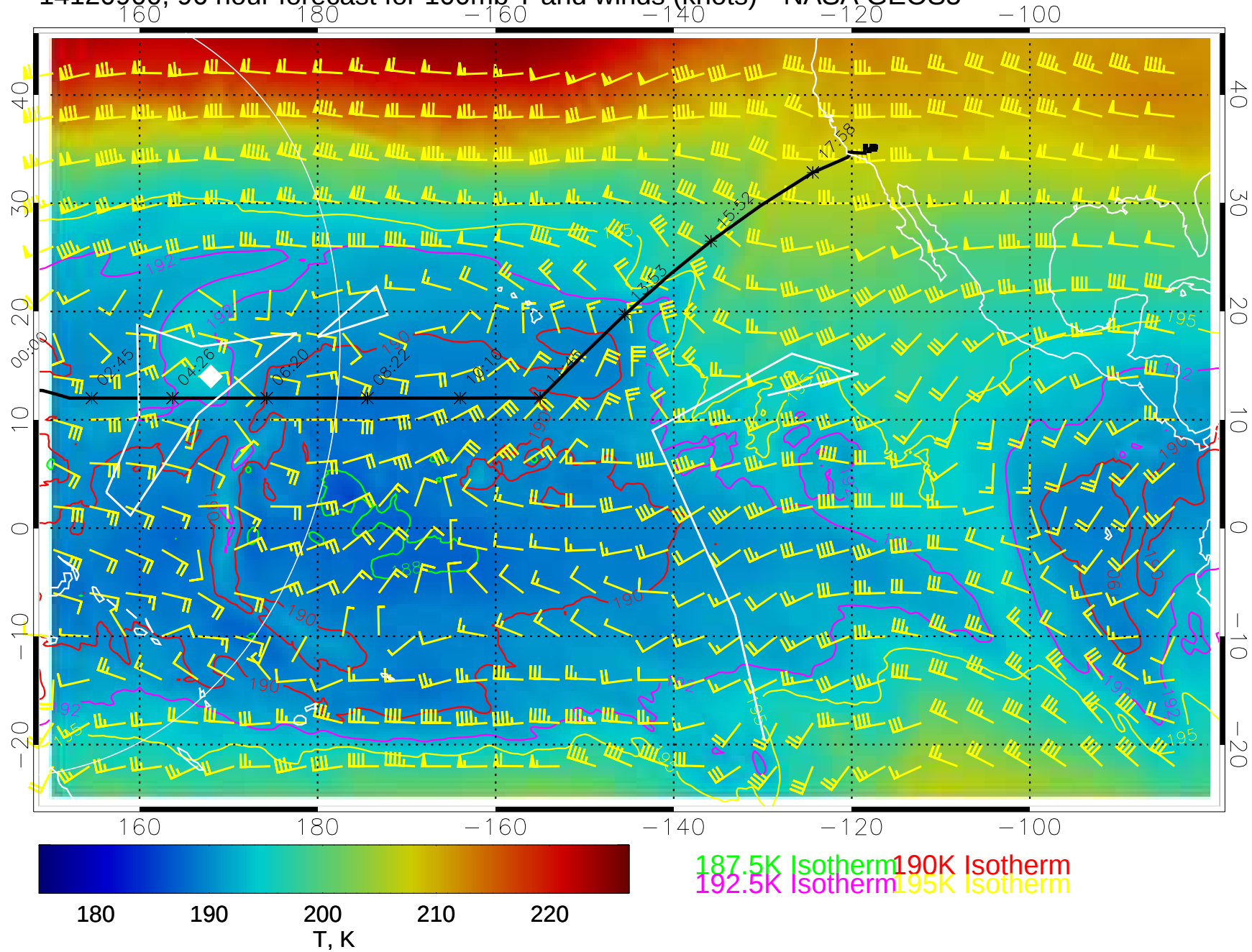
14120900, 96 hour forecast for 100mb T and winds (knots)-- NASA GEOS5
