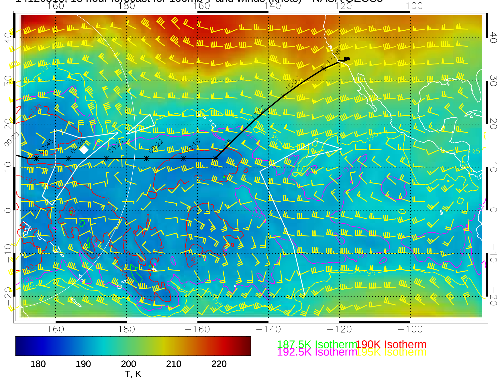
14120518, 18 hour forecast for 100mb T and winds (knots)-- NASA GEOS5
