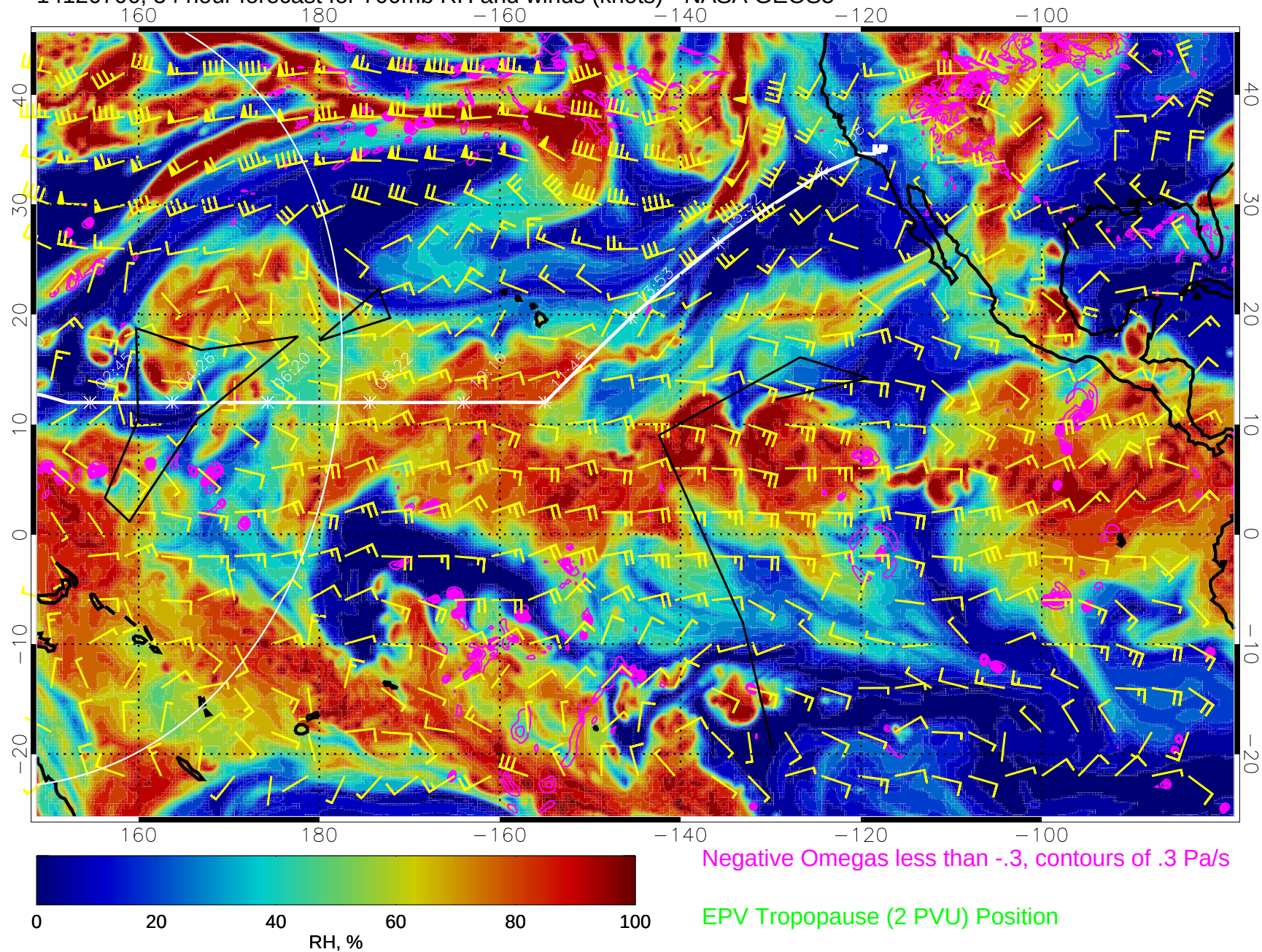
14120706, 54 hour forecast for 700mb RH and winds (knots) - NASA GEOS5
