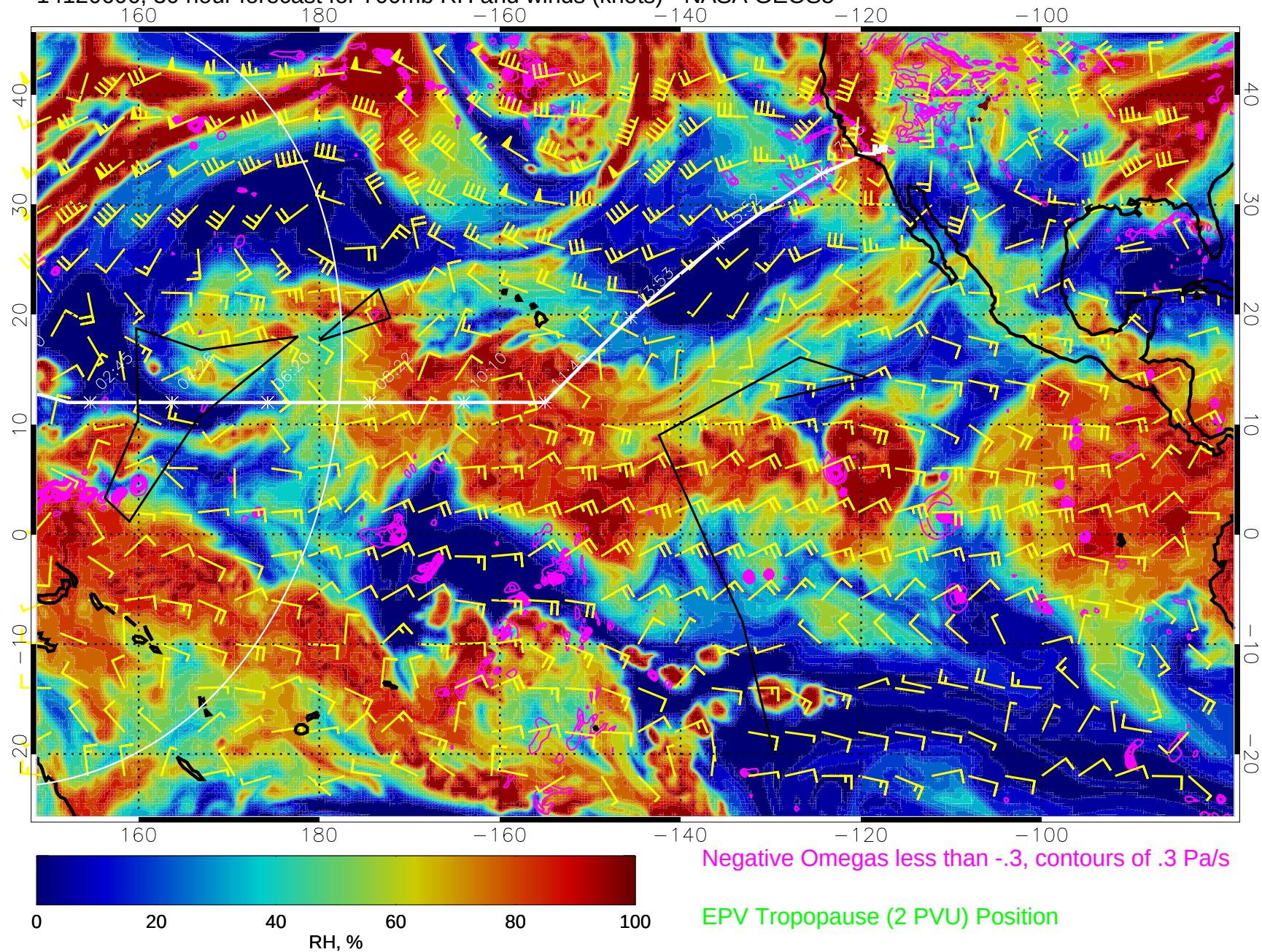
14120606, 30 hour forecast for 700mb RH and winds (knots) - NASA GEOS5
