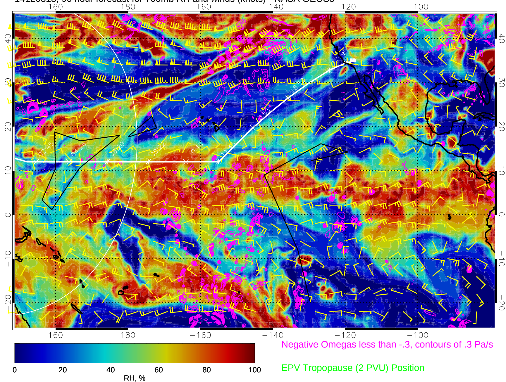
14120818, 90 hour forecast for 700mb RH and winds (knots) - NASA GEOS5
