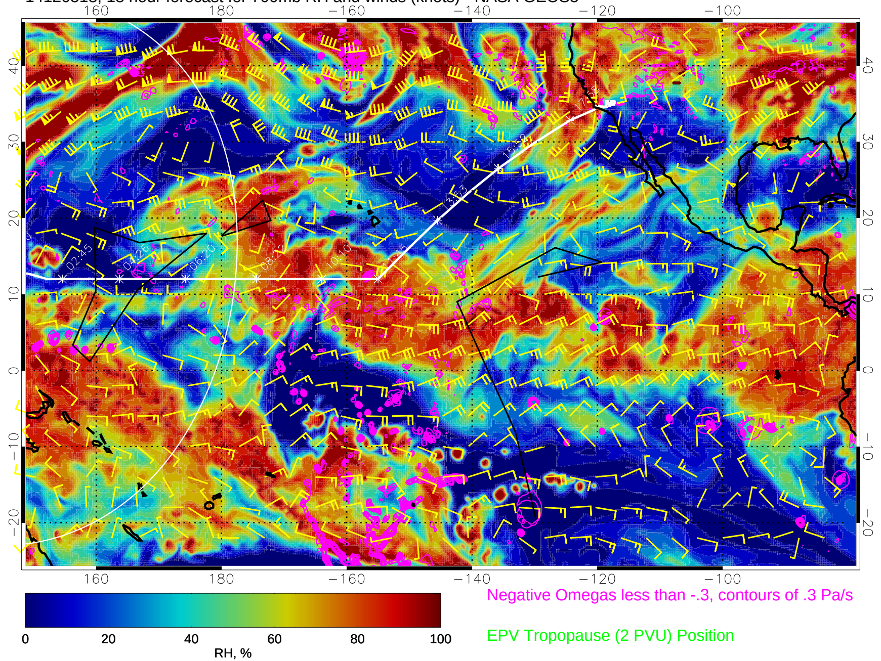
14120518, 18 hour forecast for 700mb RH and winds (knots) - NASA GEOS5
