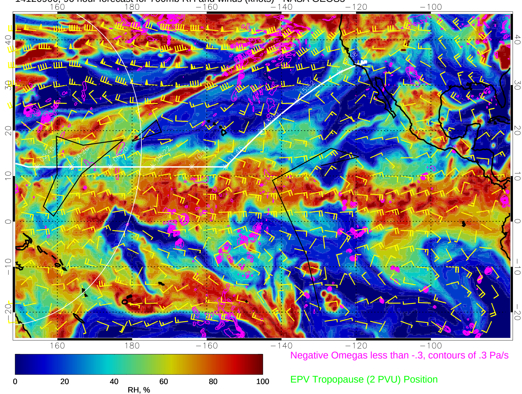
14120900, 96 hour forecast for 700mb RH and winds (knots) - NASA GEOS5
