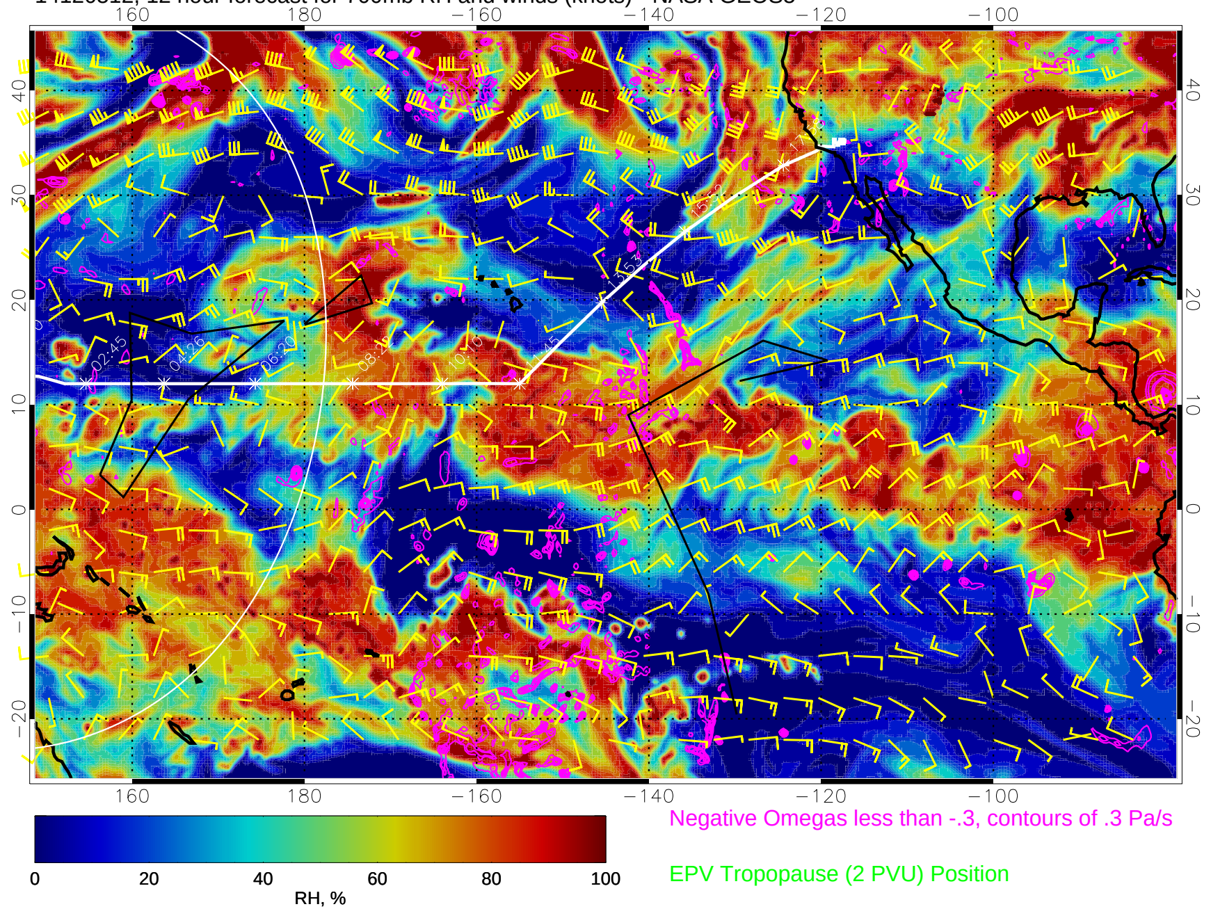
14120512, 12 hour forecast for 700mb RH and winds (knots) - NASA GEOS5
