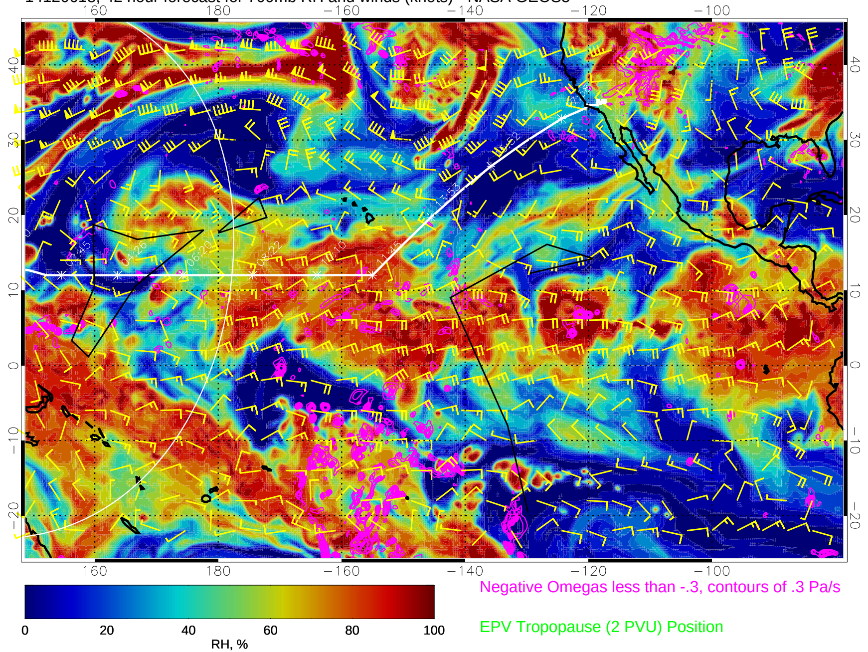
14120618, 42 hour forecast for 700mb RH and winds (knots) - NASA GEOS5
