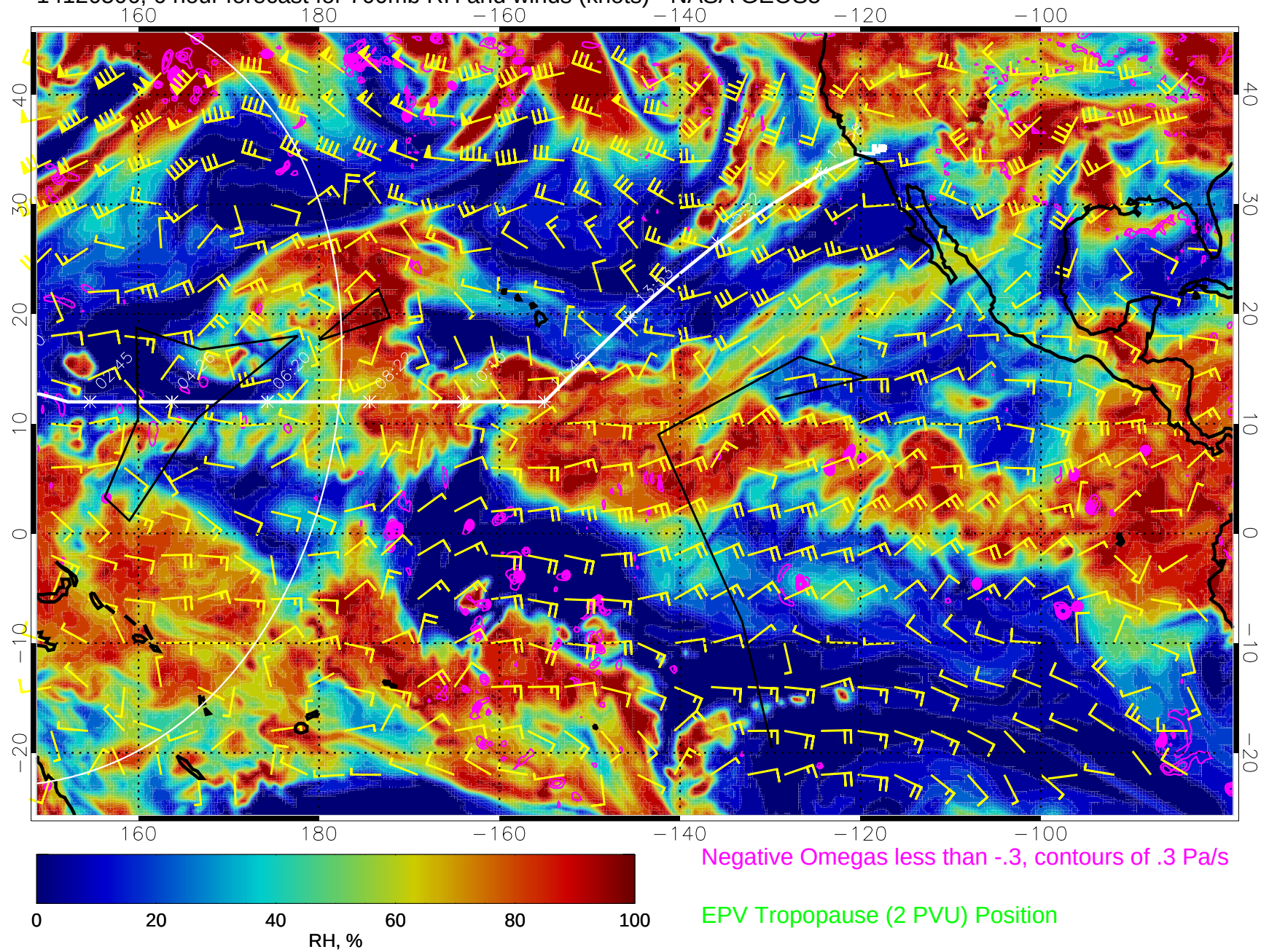
14120506, 6 hour forecast for 700mb RH and winds (knots) - NASA GEOS5
