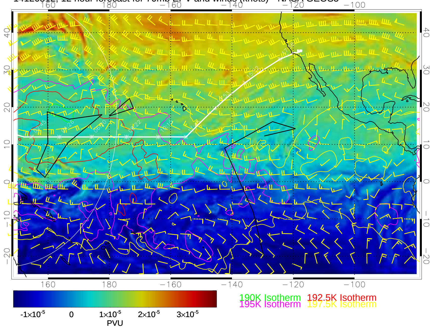
14120512, 12 hour forecast for 70mb EPV and winds (knots)-- NASA GEOS5
