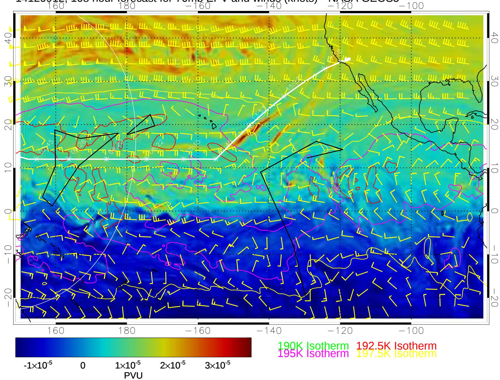
14120912, 108 hour forecast for 70mb EPV and winds (knots)-- NASA GEOS5
