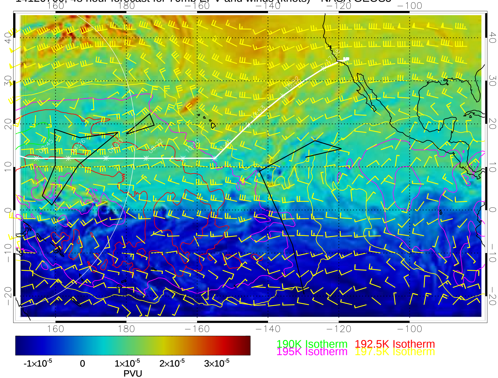
14120700, 48 hour forecast for 70mb EPV and winds (knots)-- NASA GEOS5
