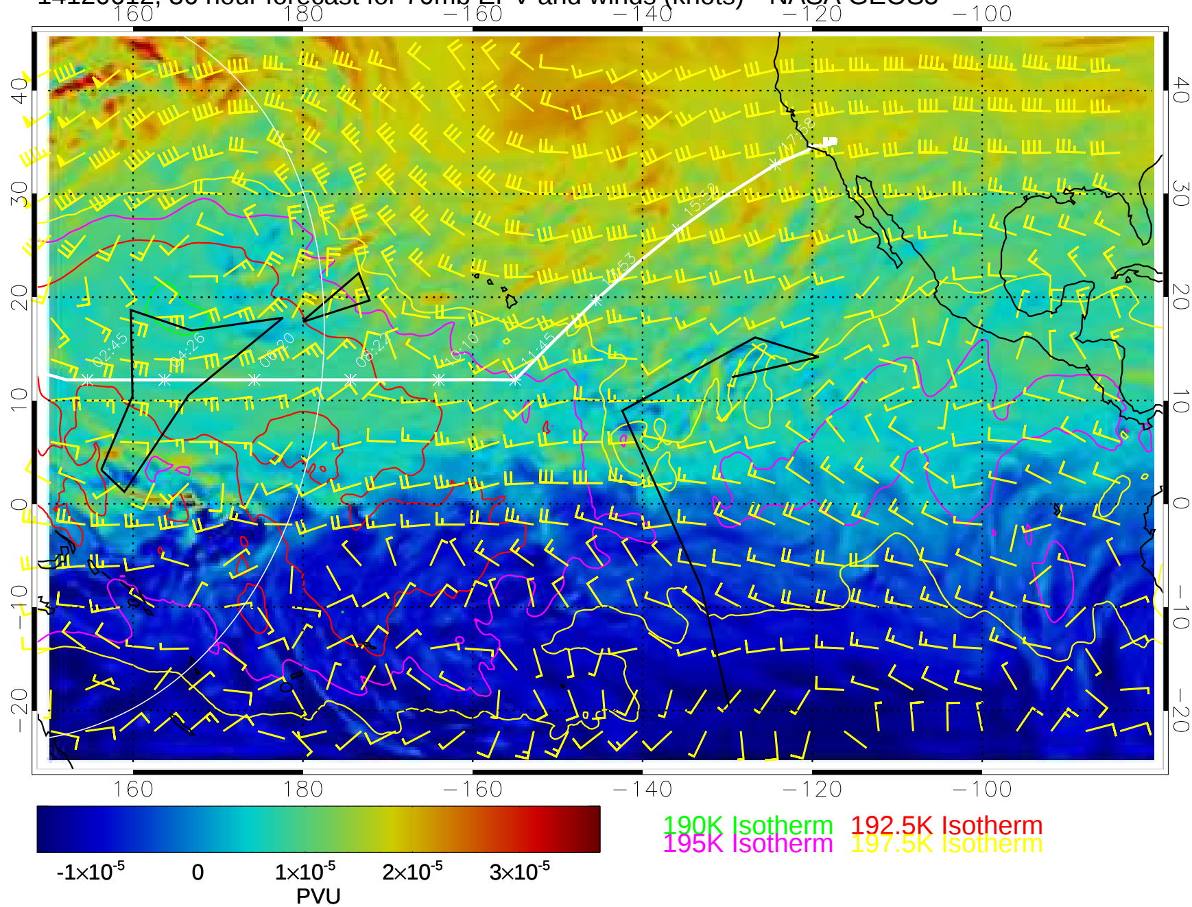
14120612, 36 hour forecast for 70mb EPV and winds (knots)-- NASA GEOS5
