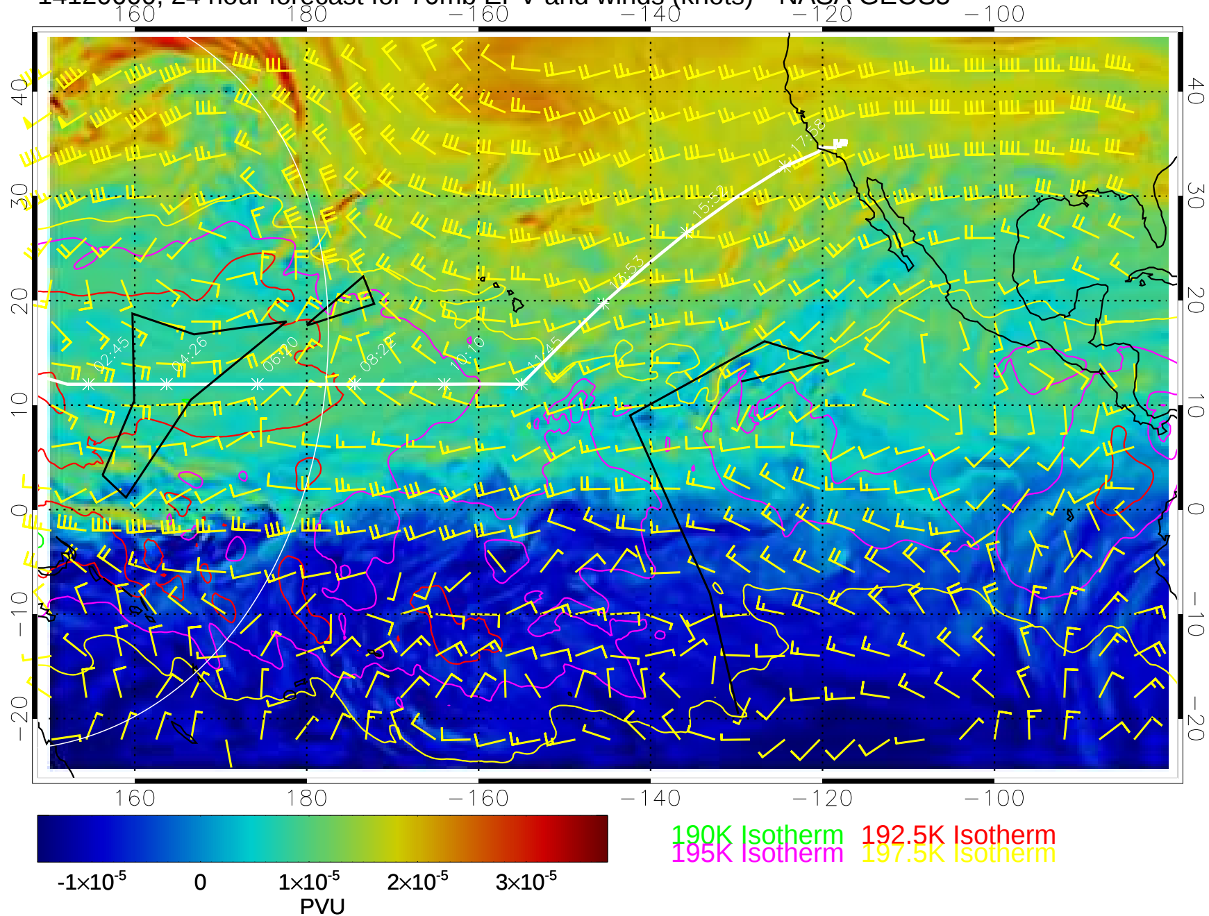
14120600, 24 hour forecast for 70mb EPV and winds (knots)-- NASA GEOS5
