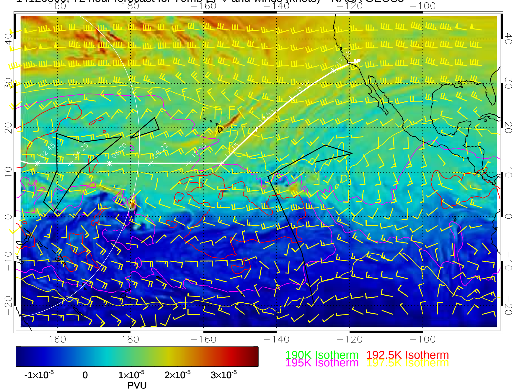
14120800, 72 hour forecast for 70mb EPV and winds (knots)-- NASA GEOS5
