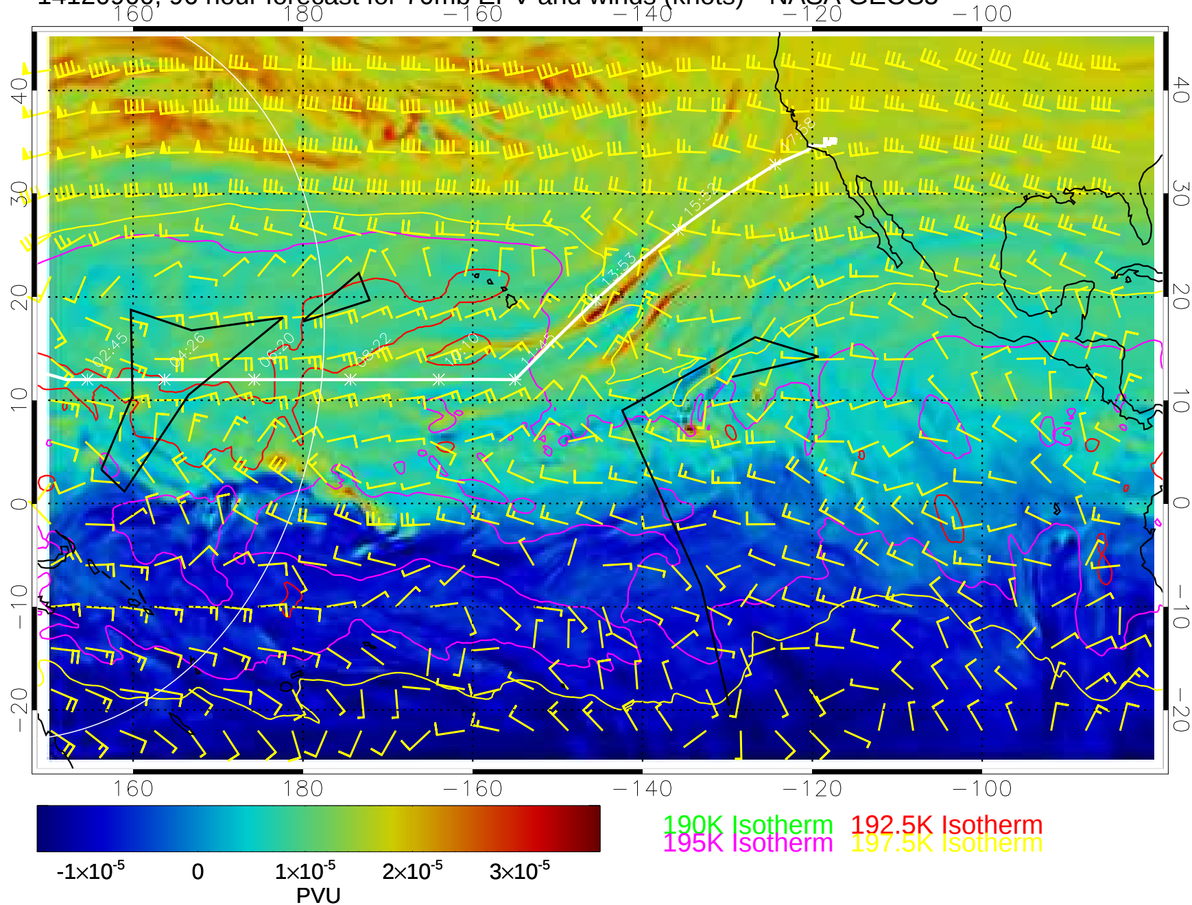
14120900, 96 hour forecast for 70mb EPV and winds (knots)-- NASA GEOS5
