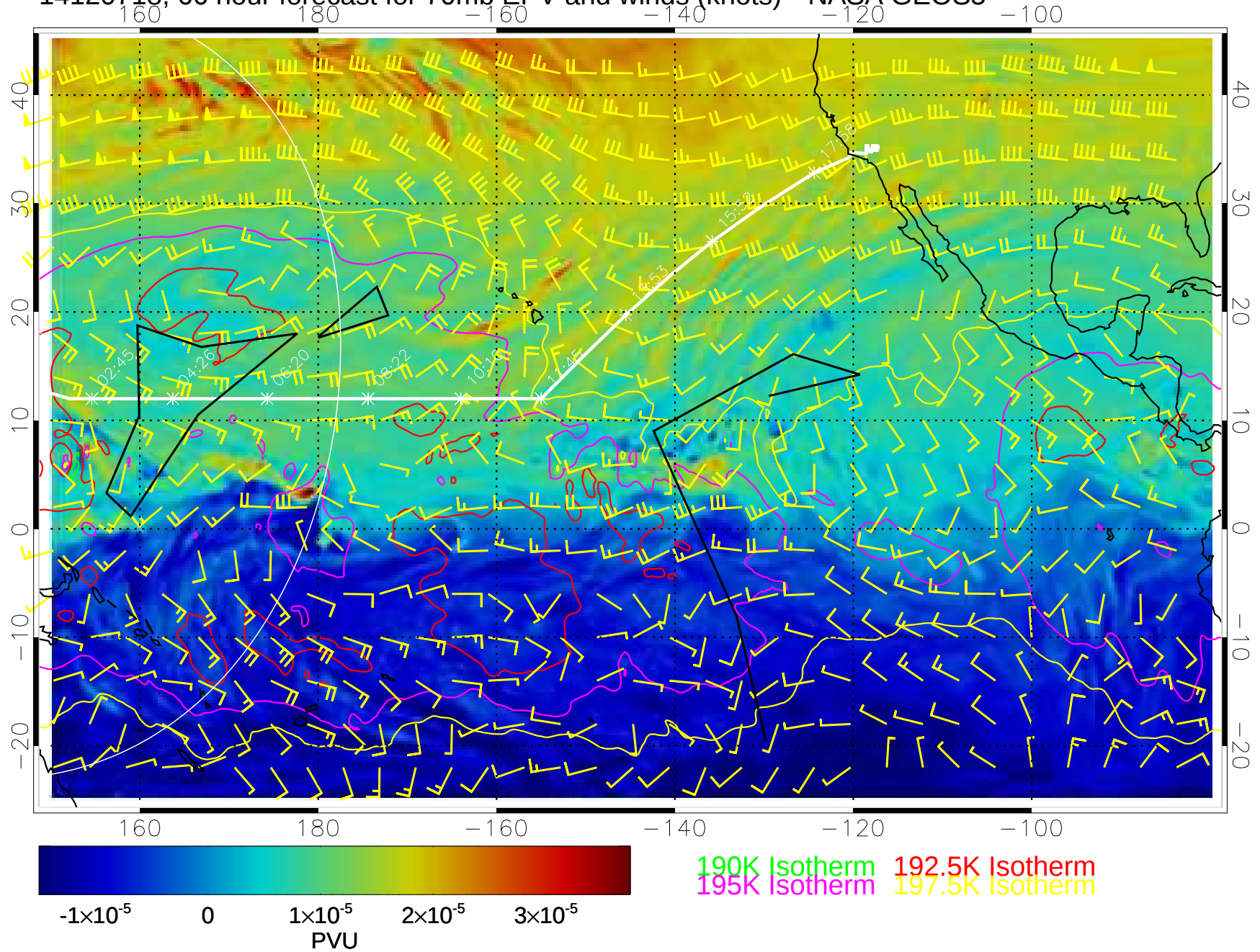
14120718, 66 hour forecast for 70mb EPV and winds (knots)-- NASA GEOS5
