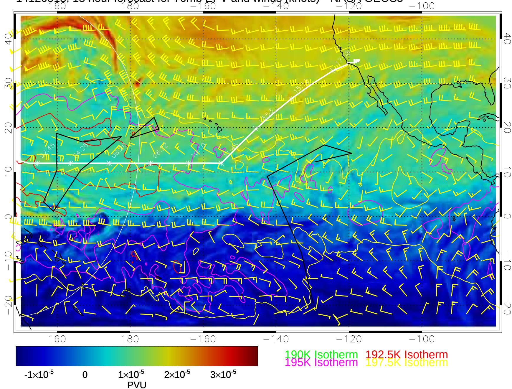
14120518, 18 hour forecast for 70mb EPV and winds (knots)-- NASA GEOS5
