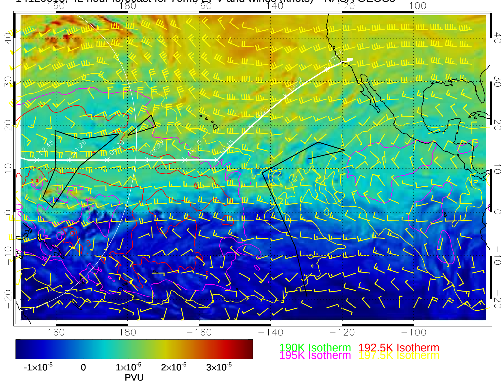
14120618, 42 hour forecast for 70mb EPV and winds (knots)-- NASA GEOS5
