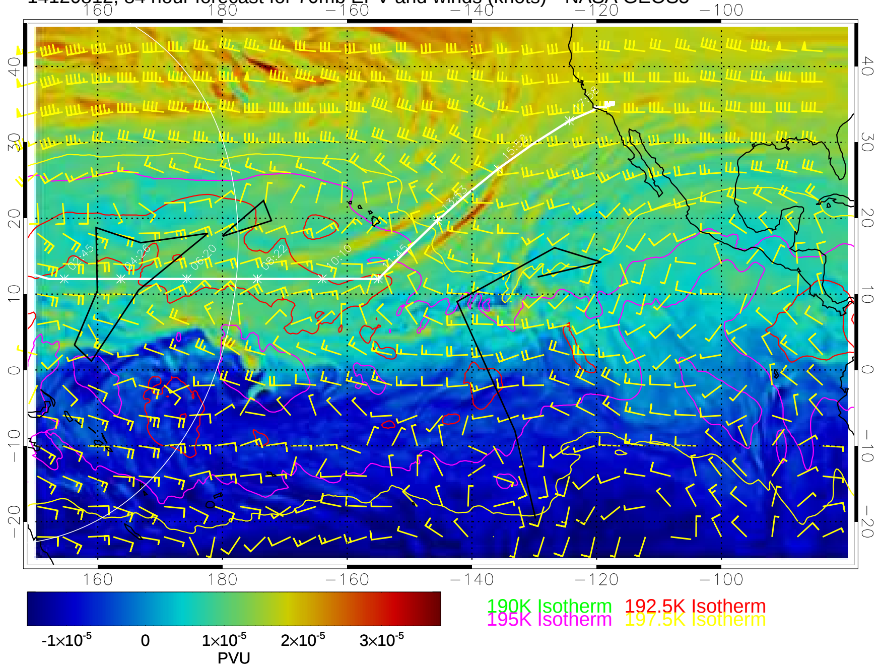
14120812, 84 hour forecast for 70mb EPV and winds (knots)-- NASA GEOS5
