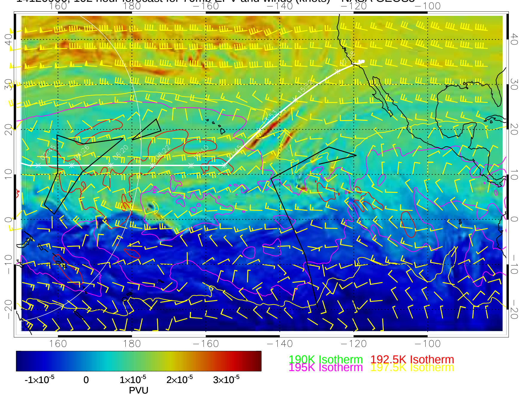
14120906, 102 hour forecast for 70mb EPV and winds (knots)-- NASA GEOS5
