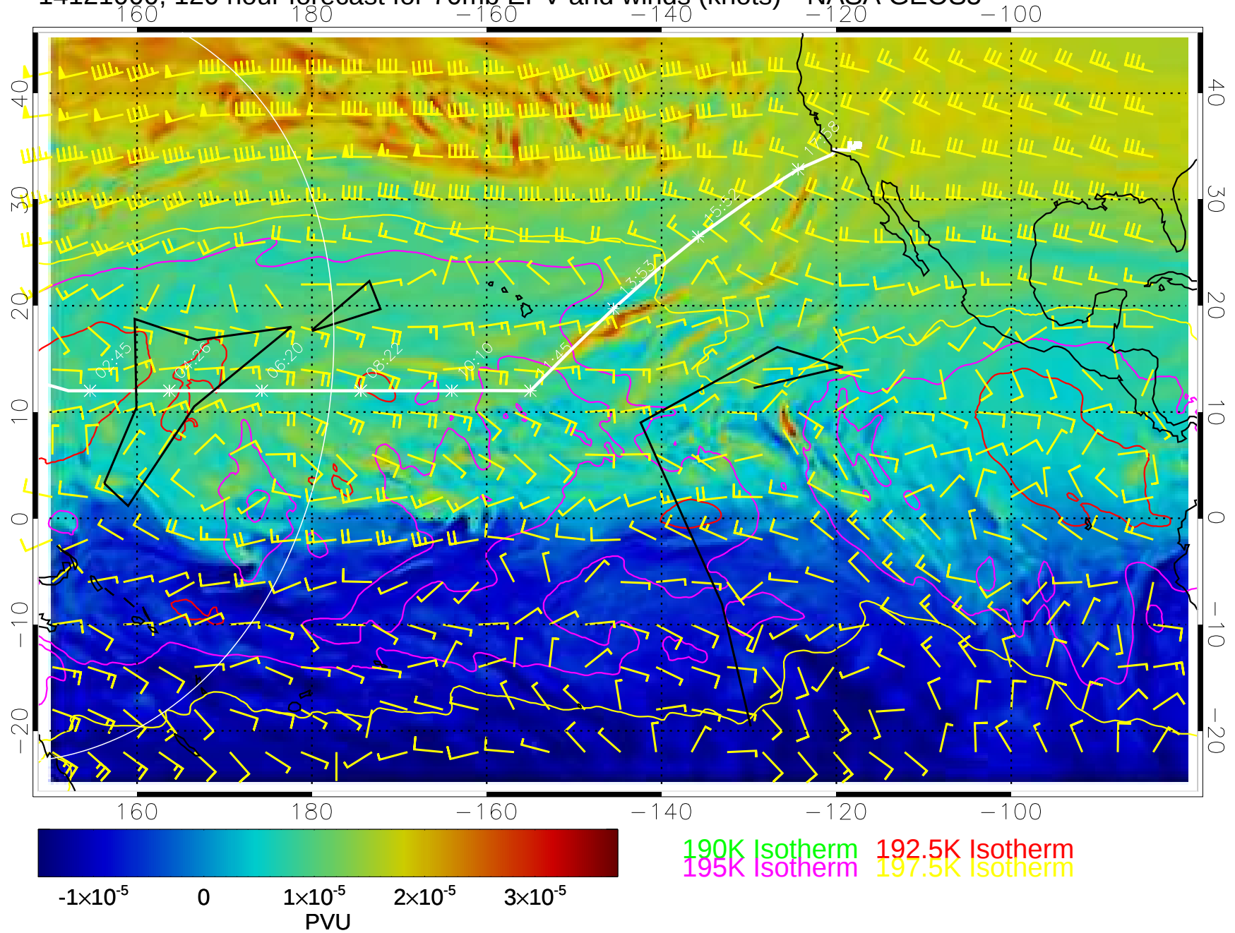
14121000, 120 hour forecast for 70mb EPV and winds (knots)-- NASA GEOS5
