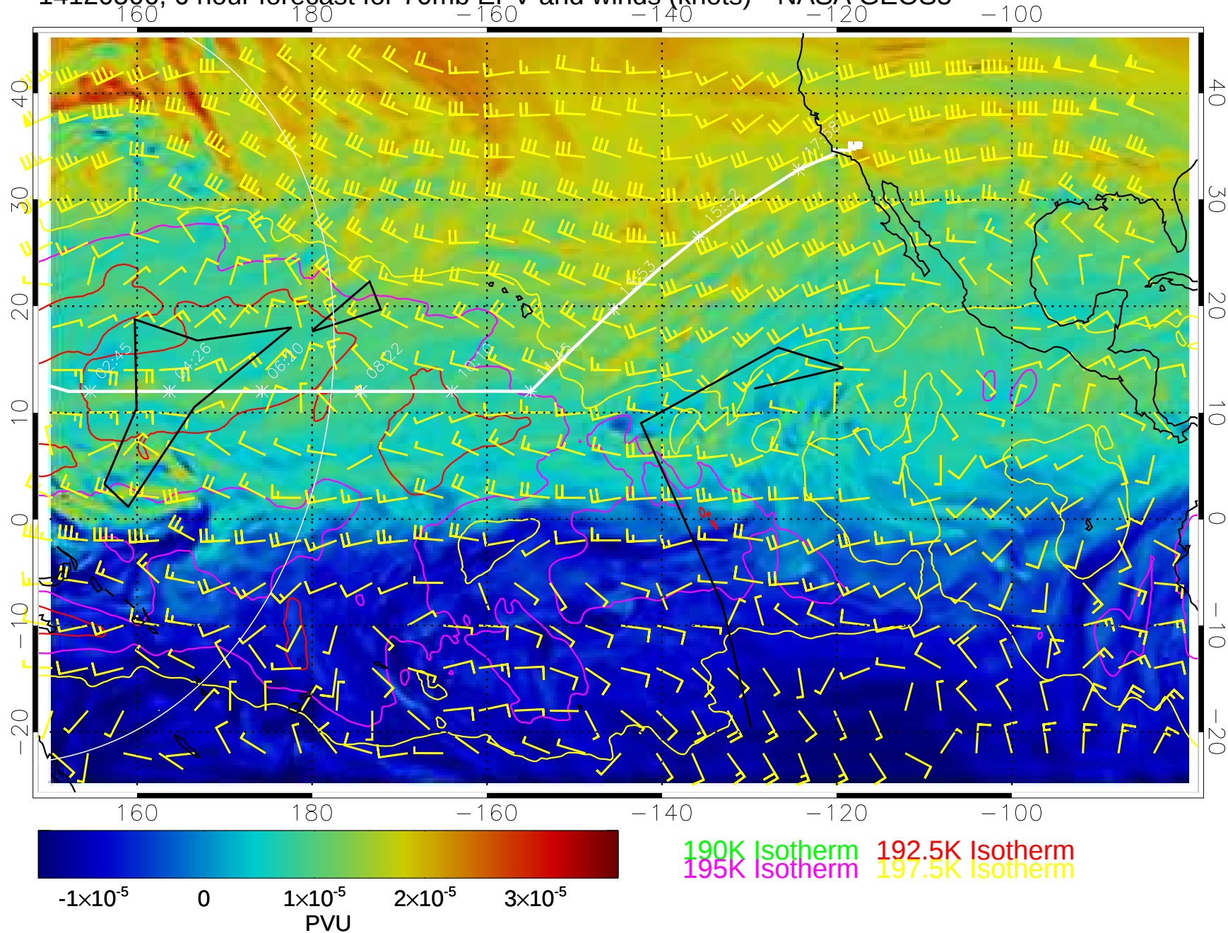
14120506, 6 hour forecast for 70mb EPV and winds (knots)-- NASA GEOS5
