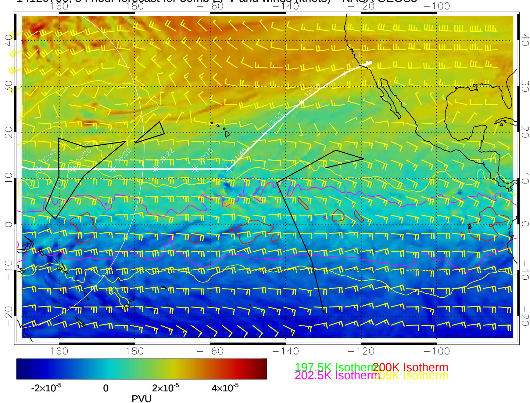
14120706, 54 hour forecast for 50mb EPV and winds (knots)-- NASA GEOS5
