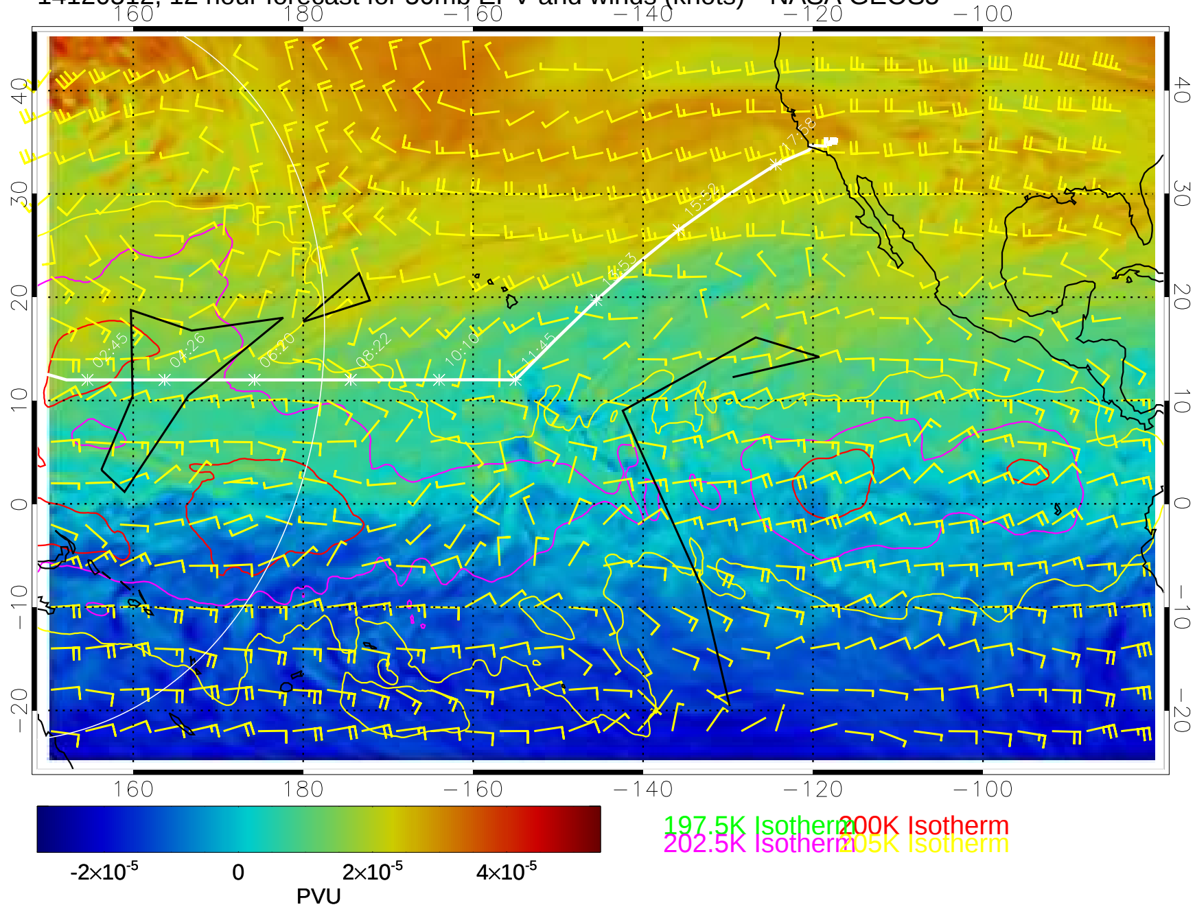
14120512, 12 hour forecast for 50mb EPV and winds (knots)-- NASA GEOS5
