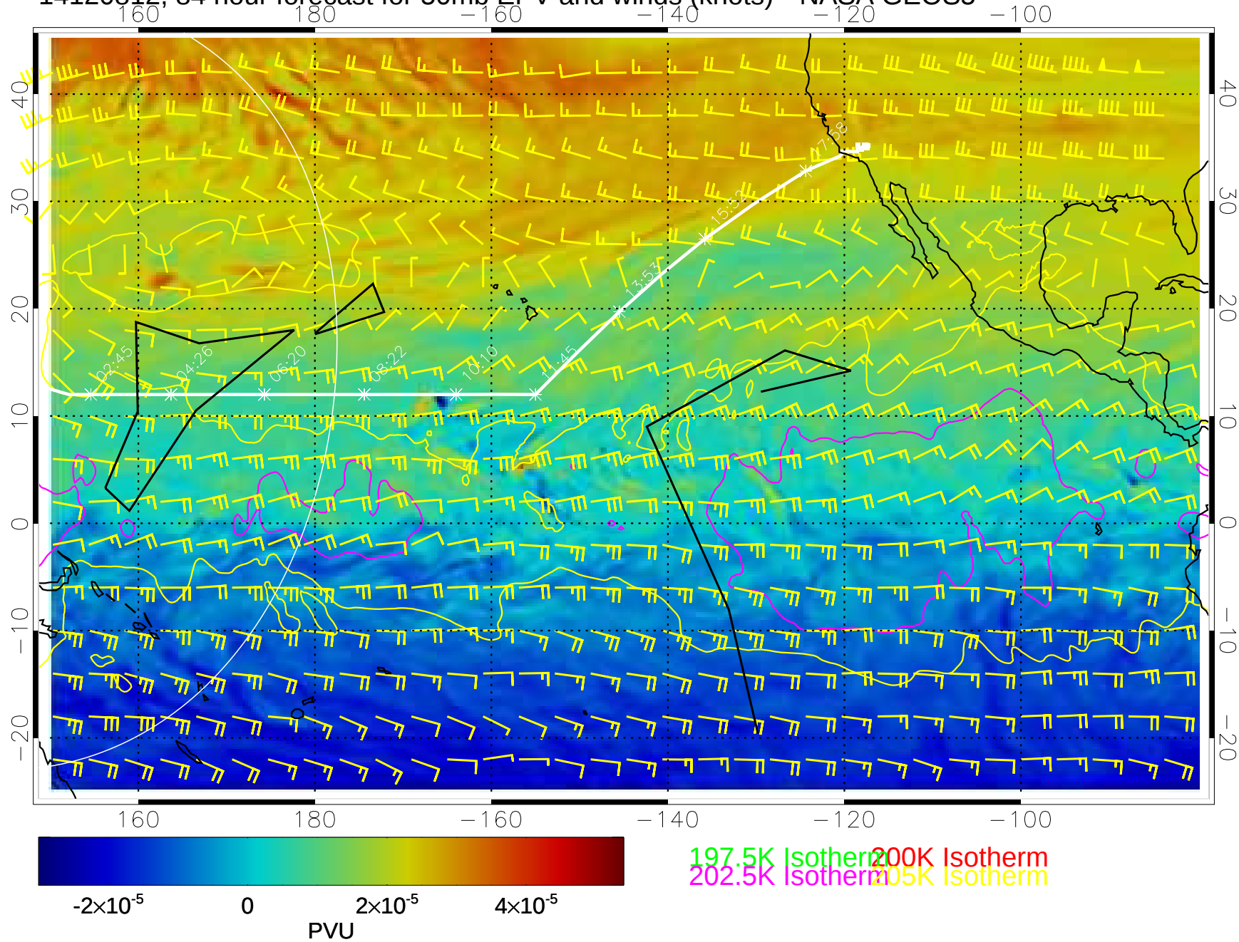
14120812, 84 hour forecast for 50mb EPV and winds (knots)-- NASA GEOS5
