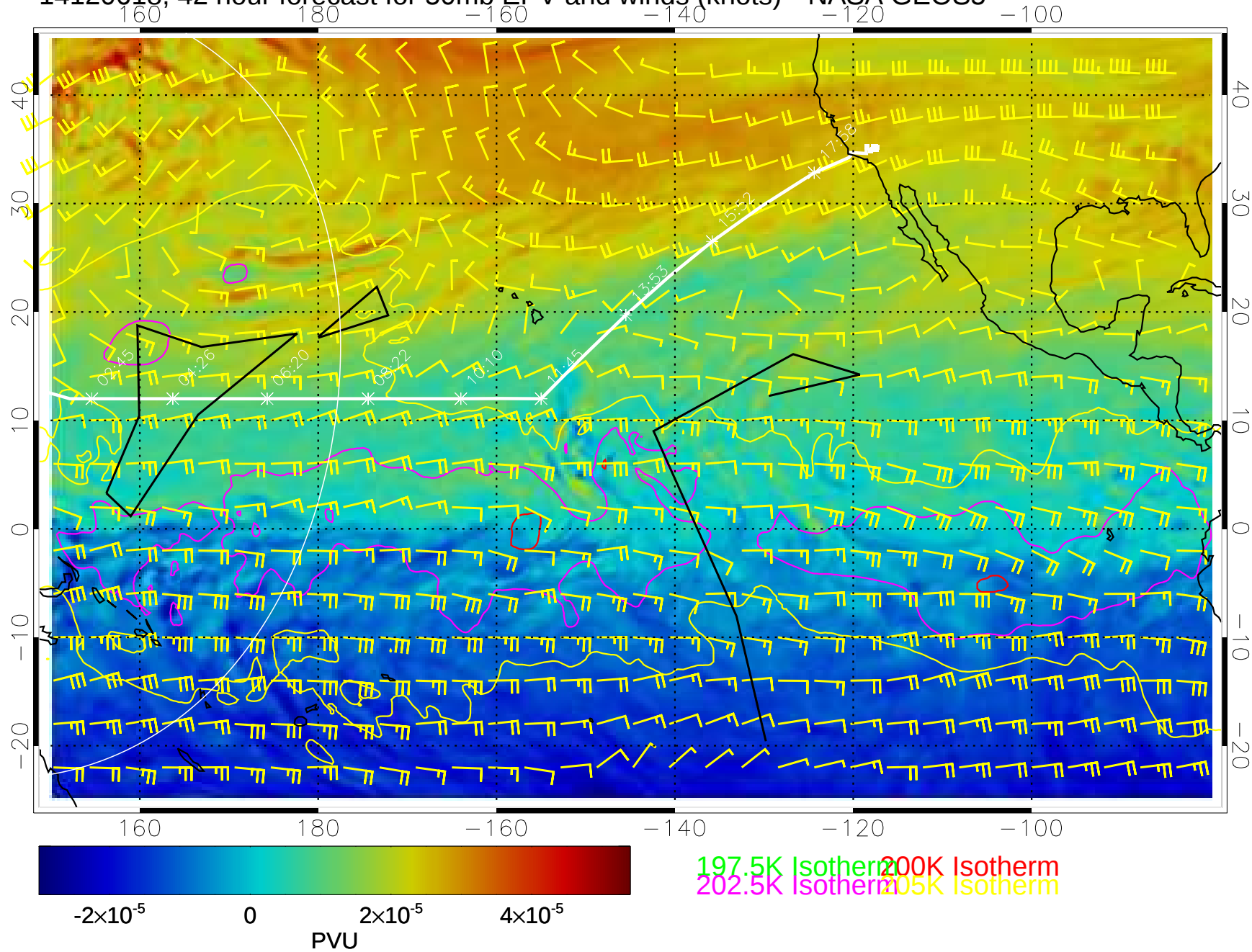
14120618, 42 hour forecast for 50mb EPV and winds (knots)-- NASA GEOS5
