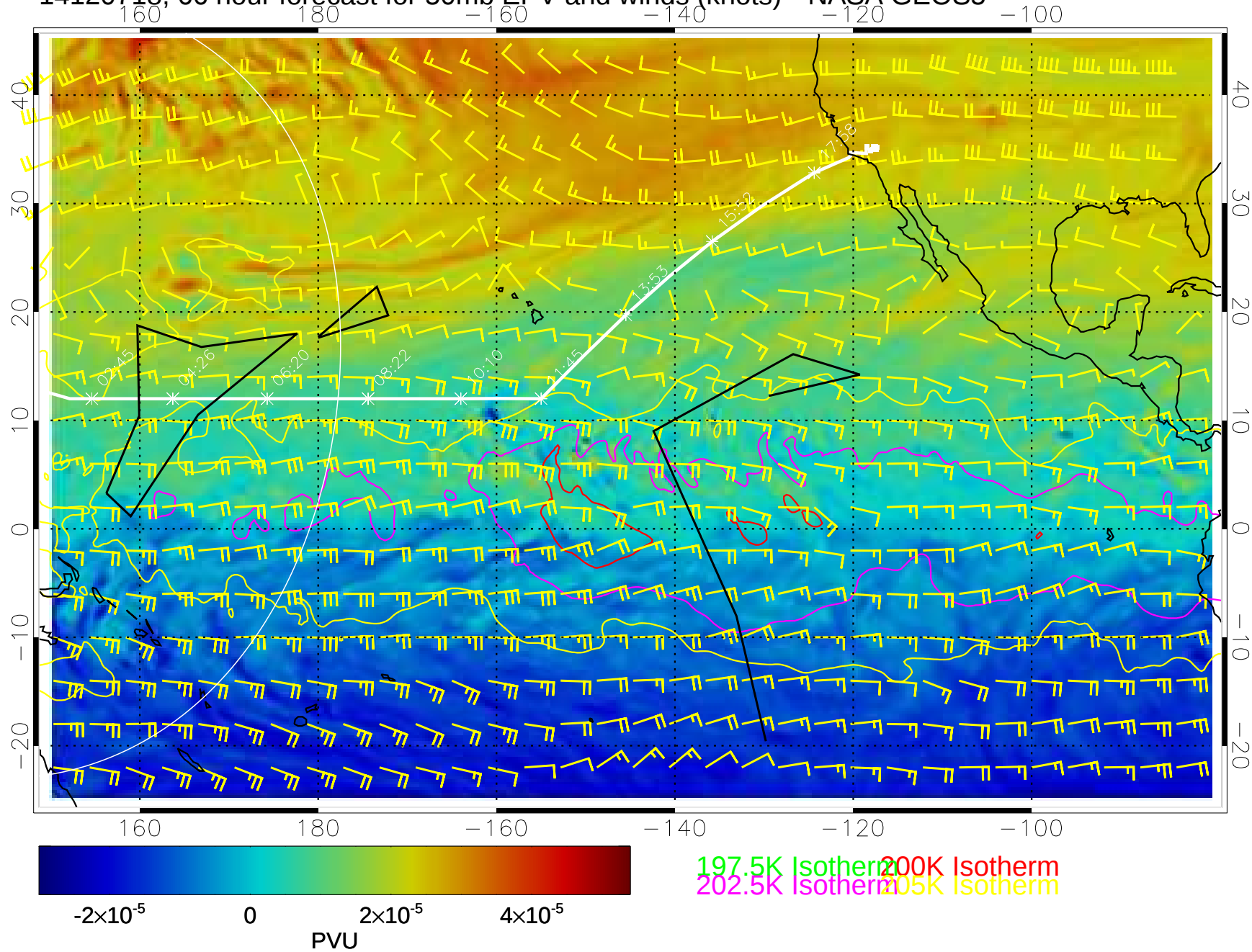
14120718, 66 hour forecast for 50mb EPV and winds (knots)-- NASA GEOS5
