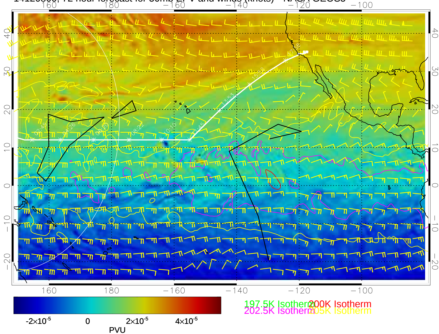
14120800, 72 hour forecast for 50mb EPV and winds (knots)-- NASA GEOS5
