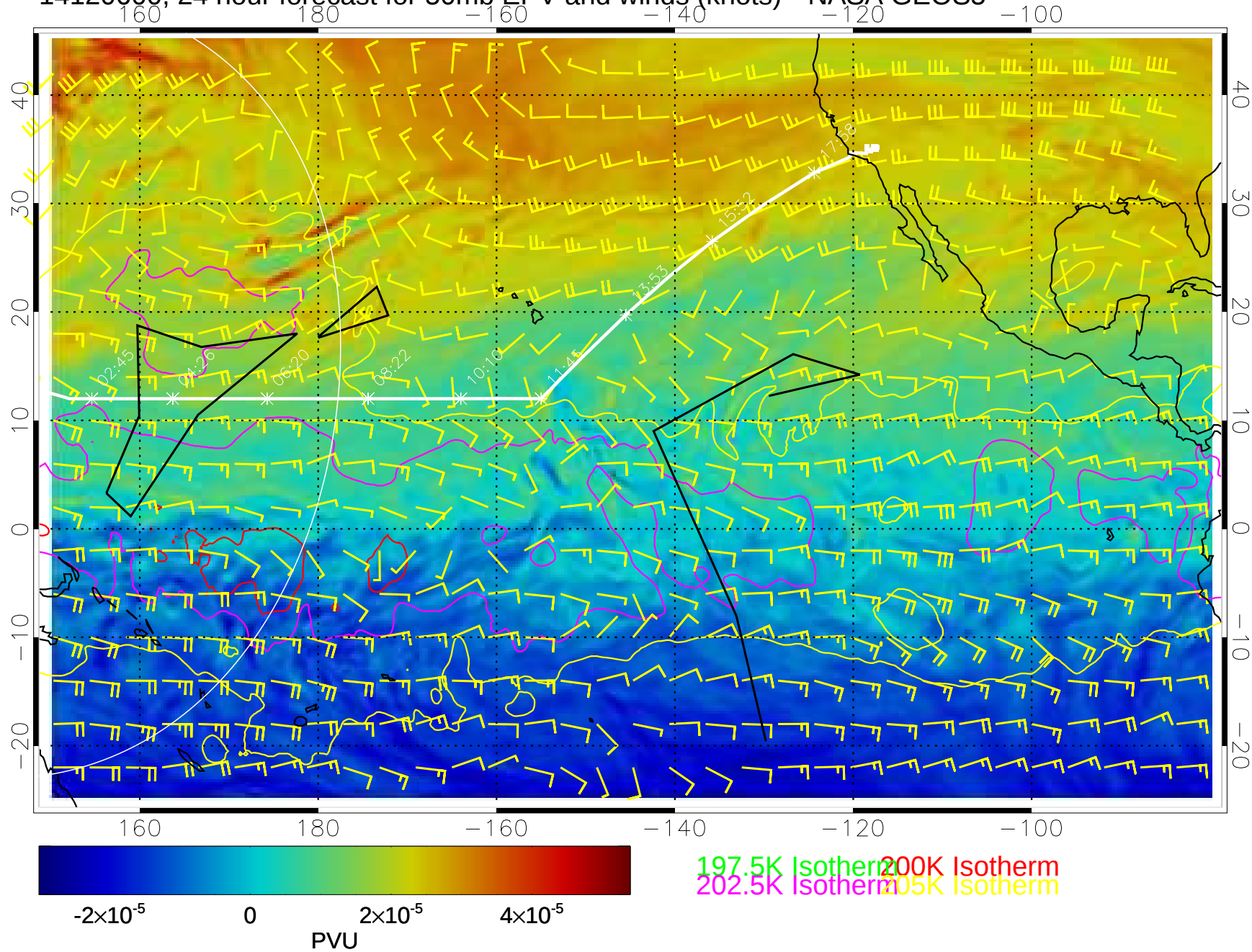
14120600, 24 hour forecast for 50mb EPV and winds (knots)-- NASA GEOS5
