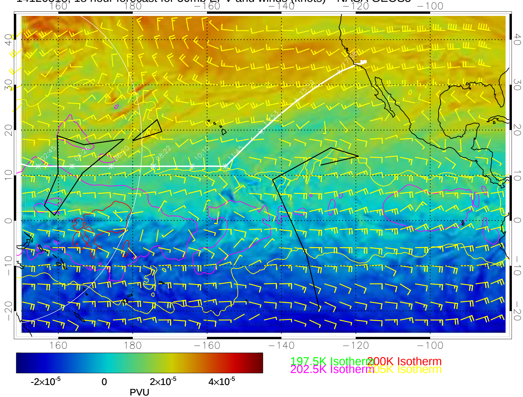
14120518, 18 hour forecast for 50mb EPV and winds (knots)-- NASA GEOS5
