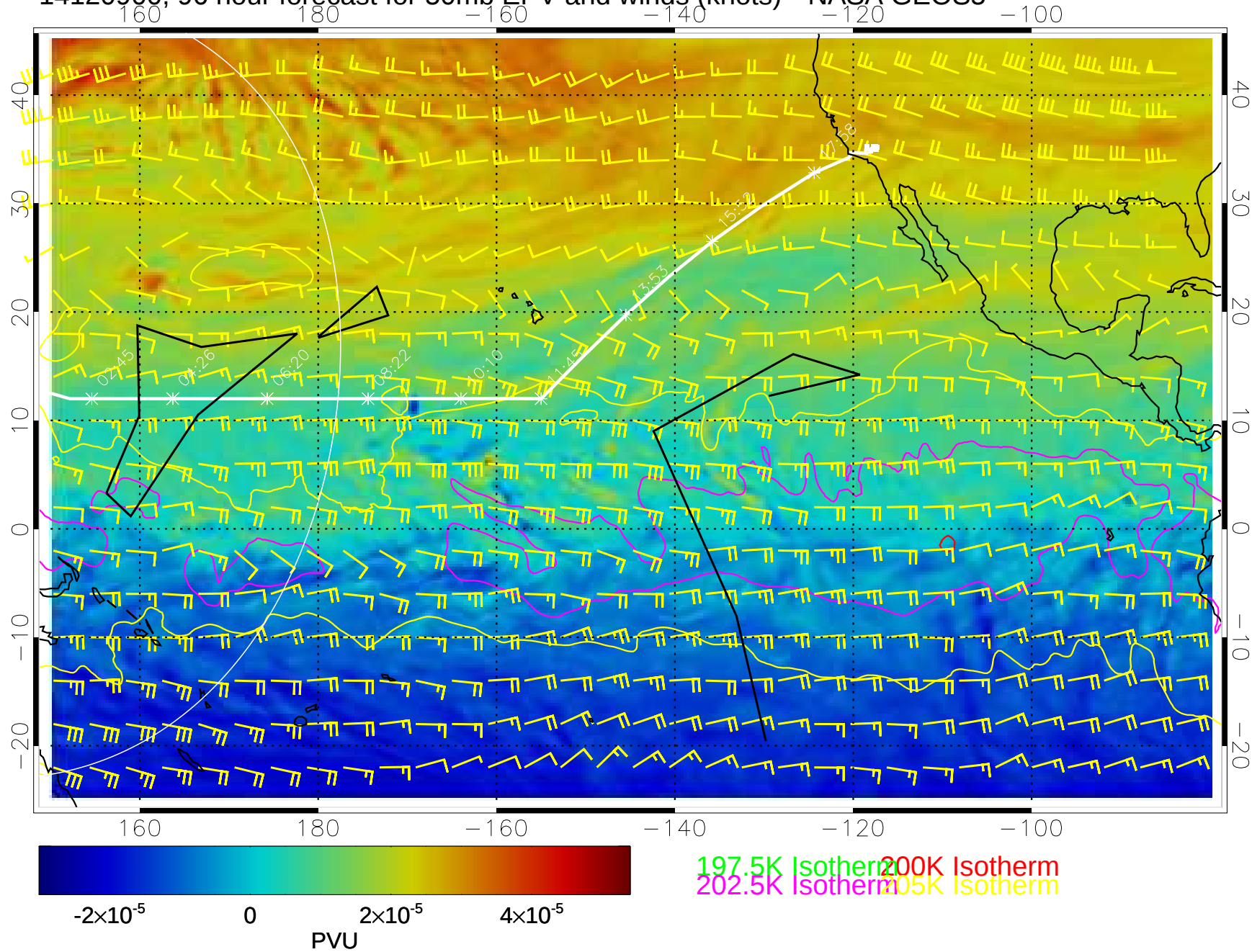
14120900, 96 hour forecast for 50mb EPV and winds (knots)-- NASA GEOS5
