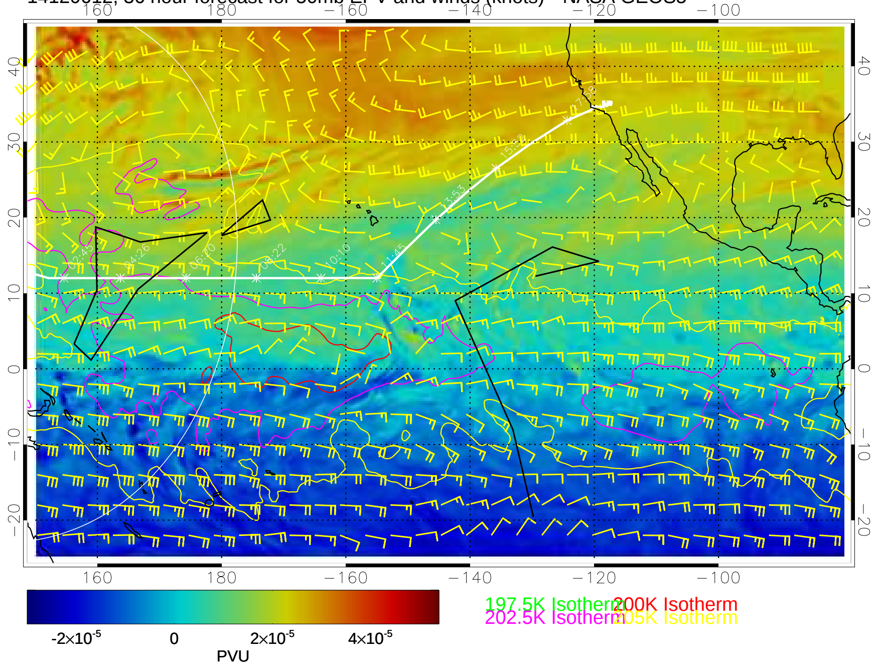
14120612, 36 hour forecast for 50mb EPV and winds (knots)-- NASA GEOS5
