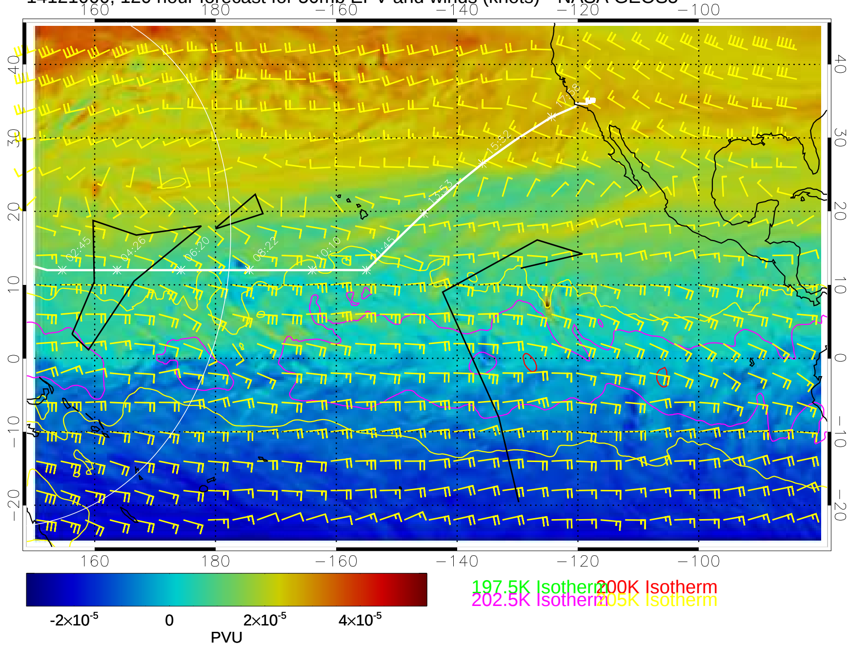
14121000, 120 hour forecast for 50mb EPV and winds (knots)-- NASA GEOS5
