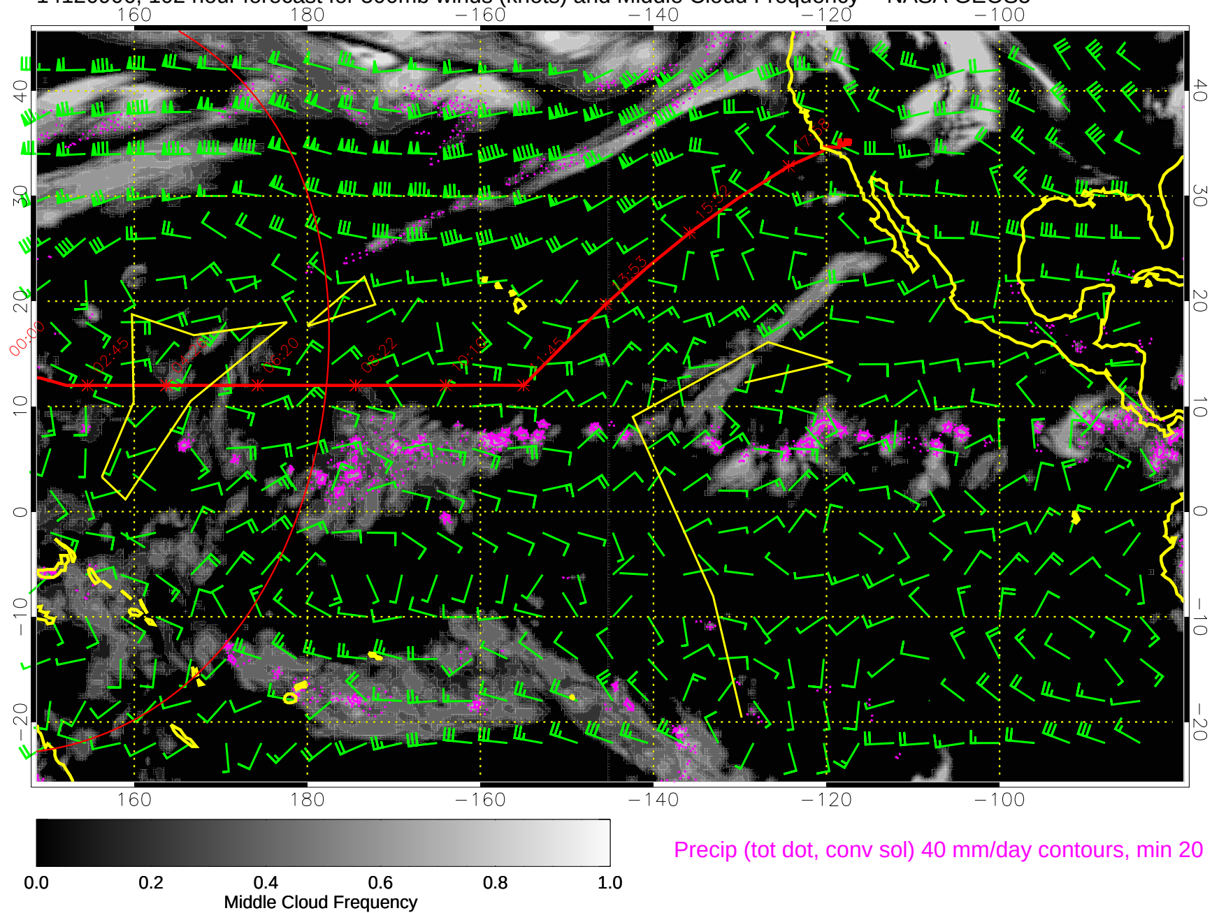
14120906, 102 hour forecast for 500mb winds (knots) and Middle Cloud Frequency -- NASA GEOS5
