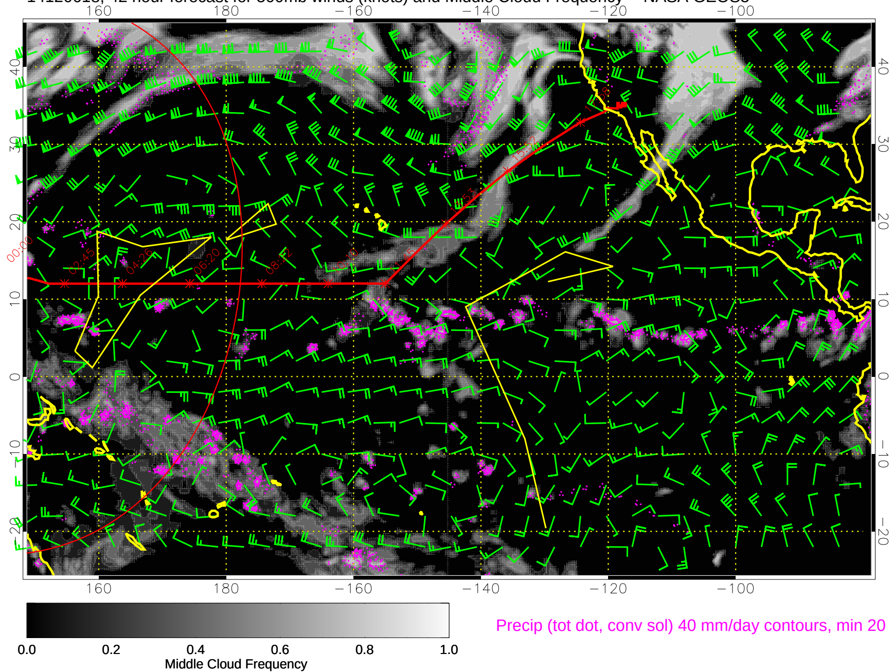
14120618, 42 hour forecast for 500mb winds (knots) and Middle Cloud Frequency -- NASA GEOS5
