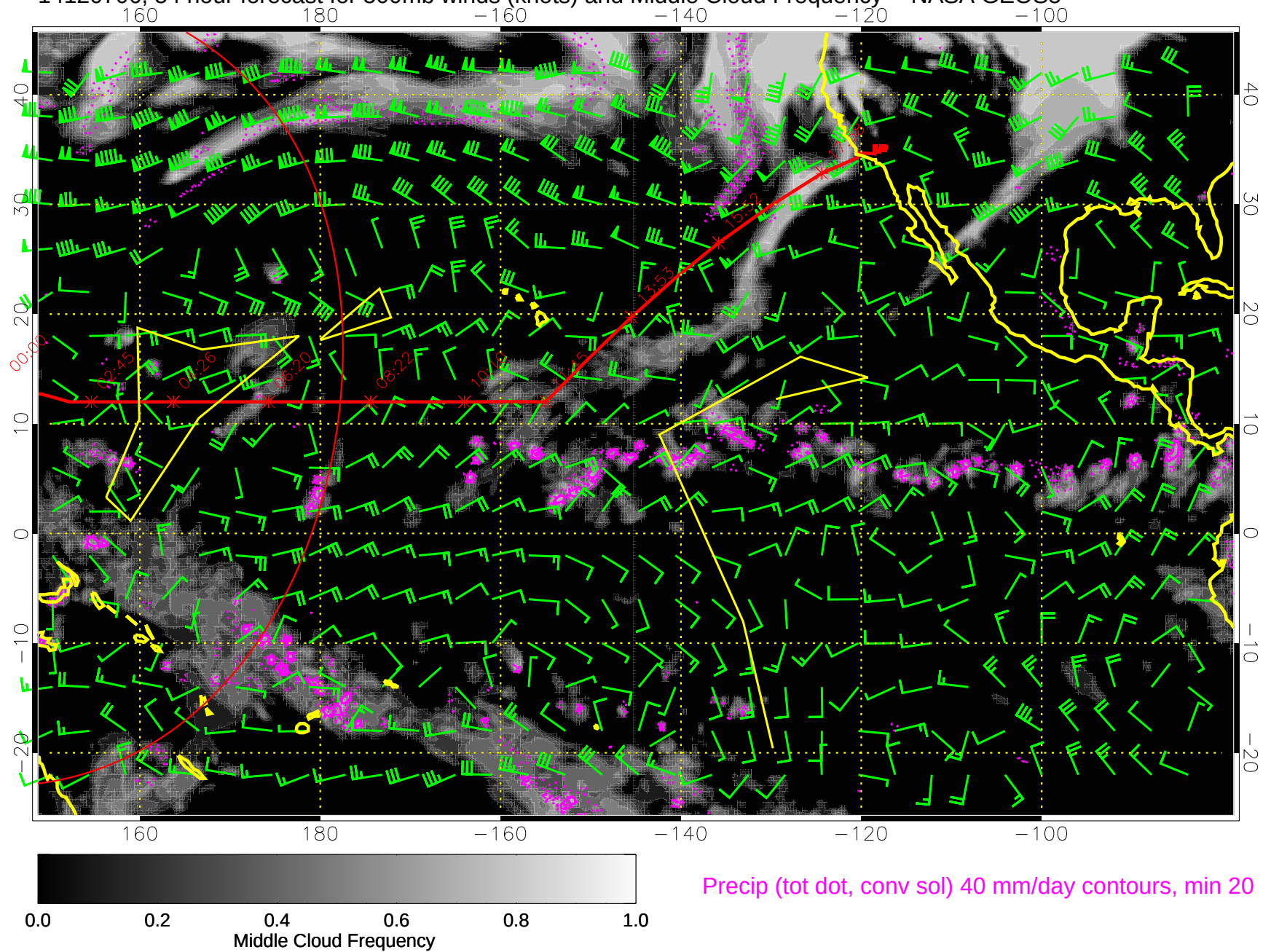
14120706, 54 hour forecast for 500mb winds (knots) and Middle Cloud Frequency -- NASA GEOS5
