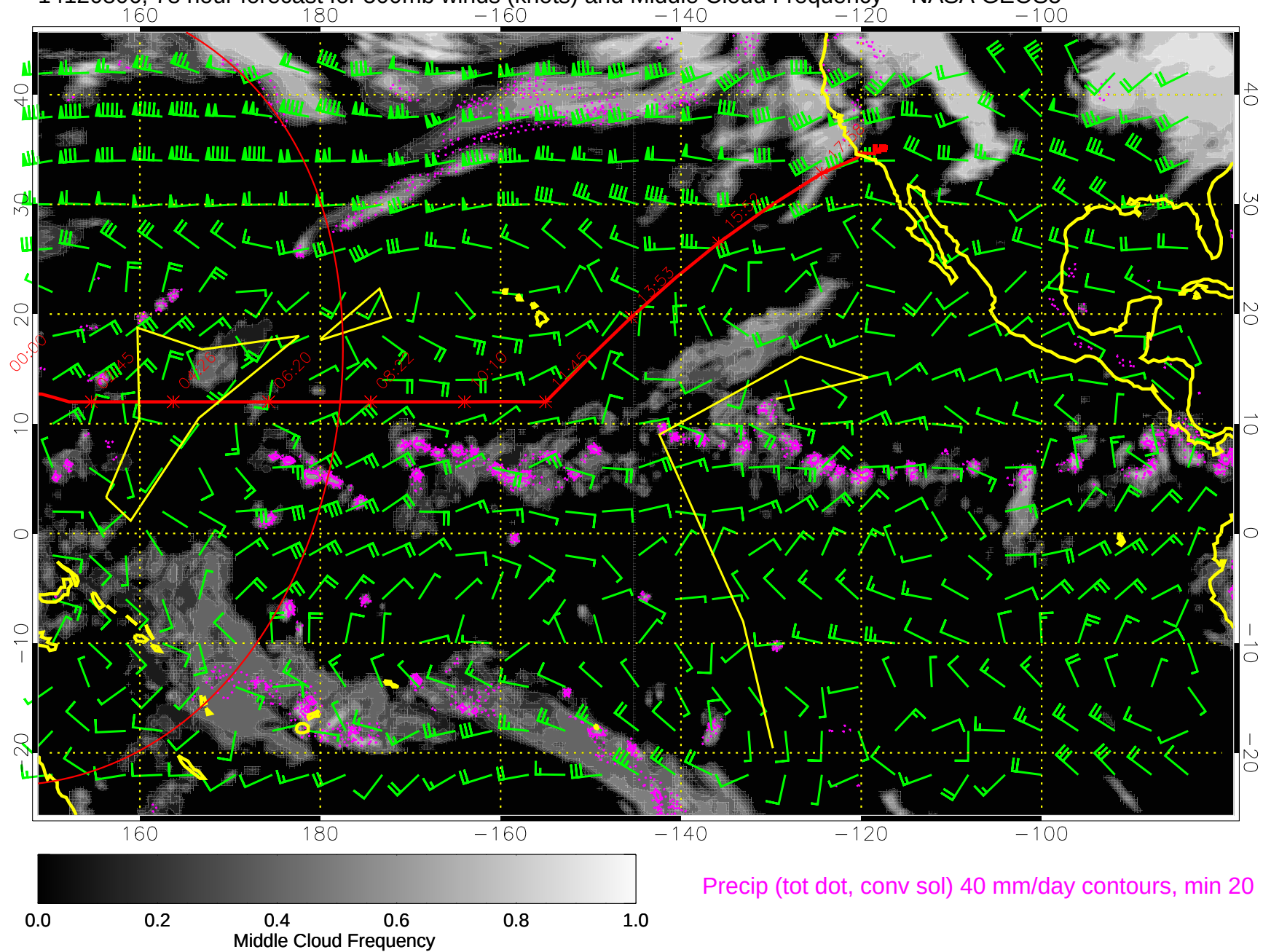
14120806, 78 hour forecast for 500mb winds (knots) and Middle Cloud Frequency -- NASA GEOS5
