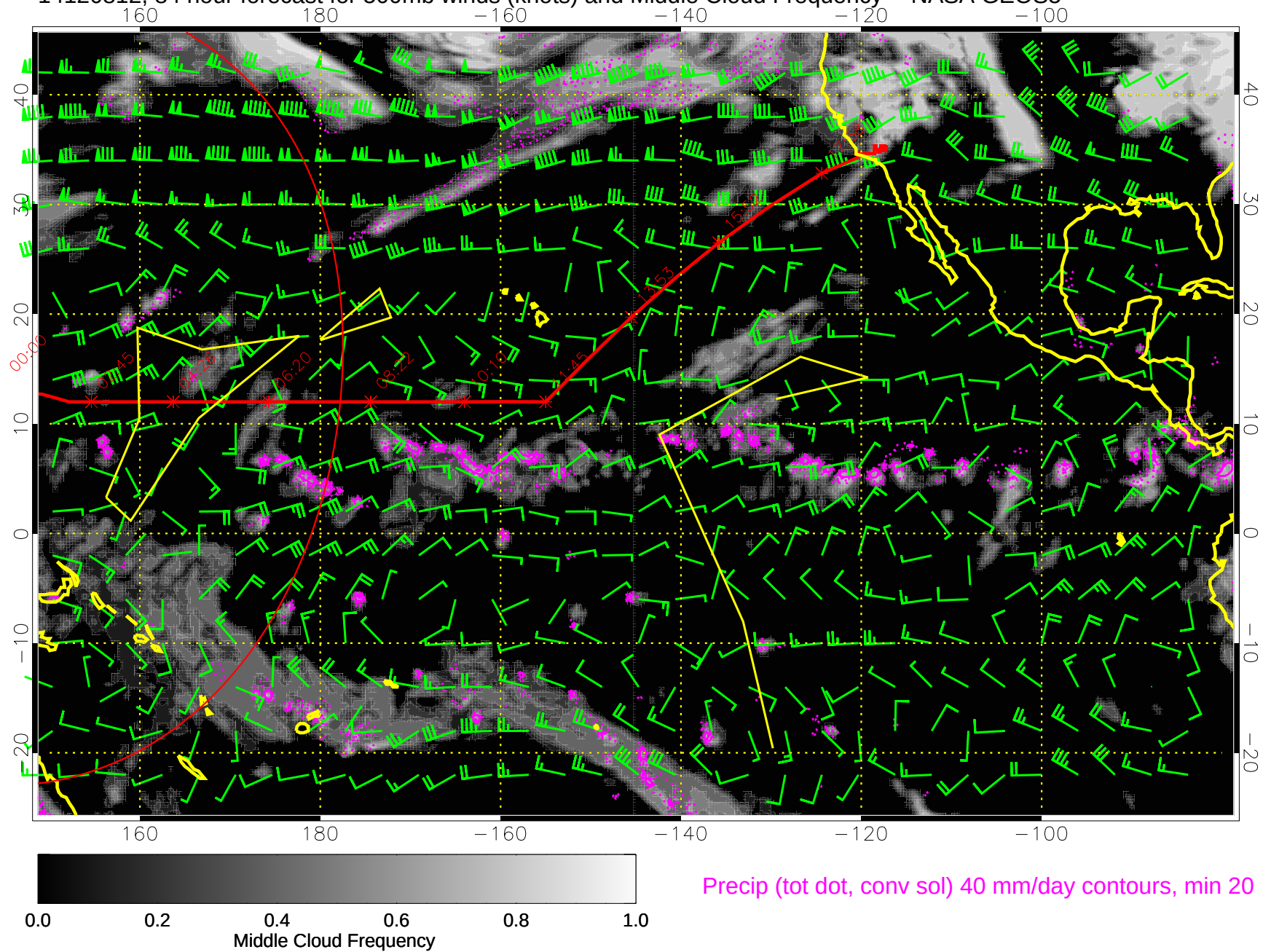
14120812, 84 hour forecast for 500mb winds (knots) and Middle Cloud Frequency -- NASA GEOS5
