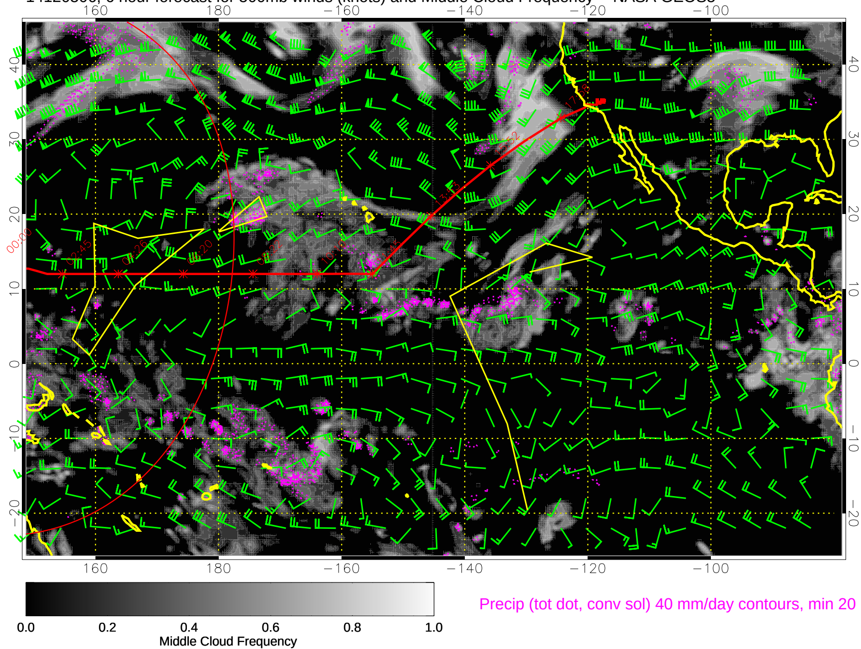
14120506, 6 hour forecast for 500mb winds (knots) and Middle Cloud Frequency -- NASA GEOS5
