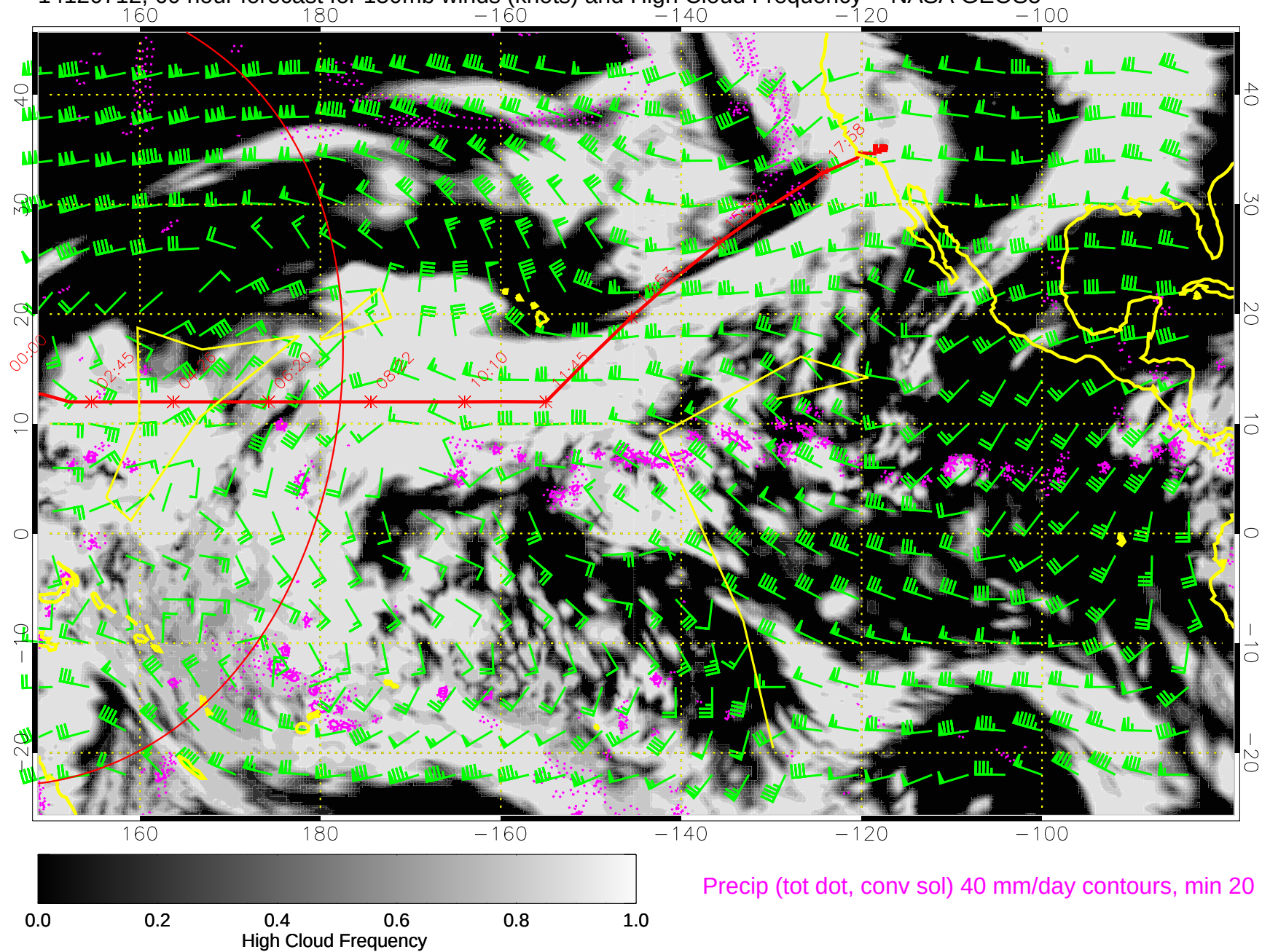
14120712, 60 hour forecast for 150mb winds (knots) and High Cloud Frequency -- NASA GEOS5
