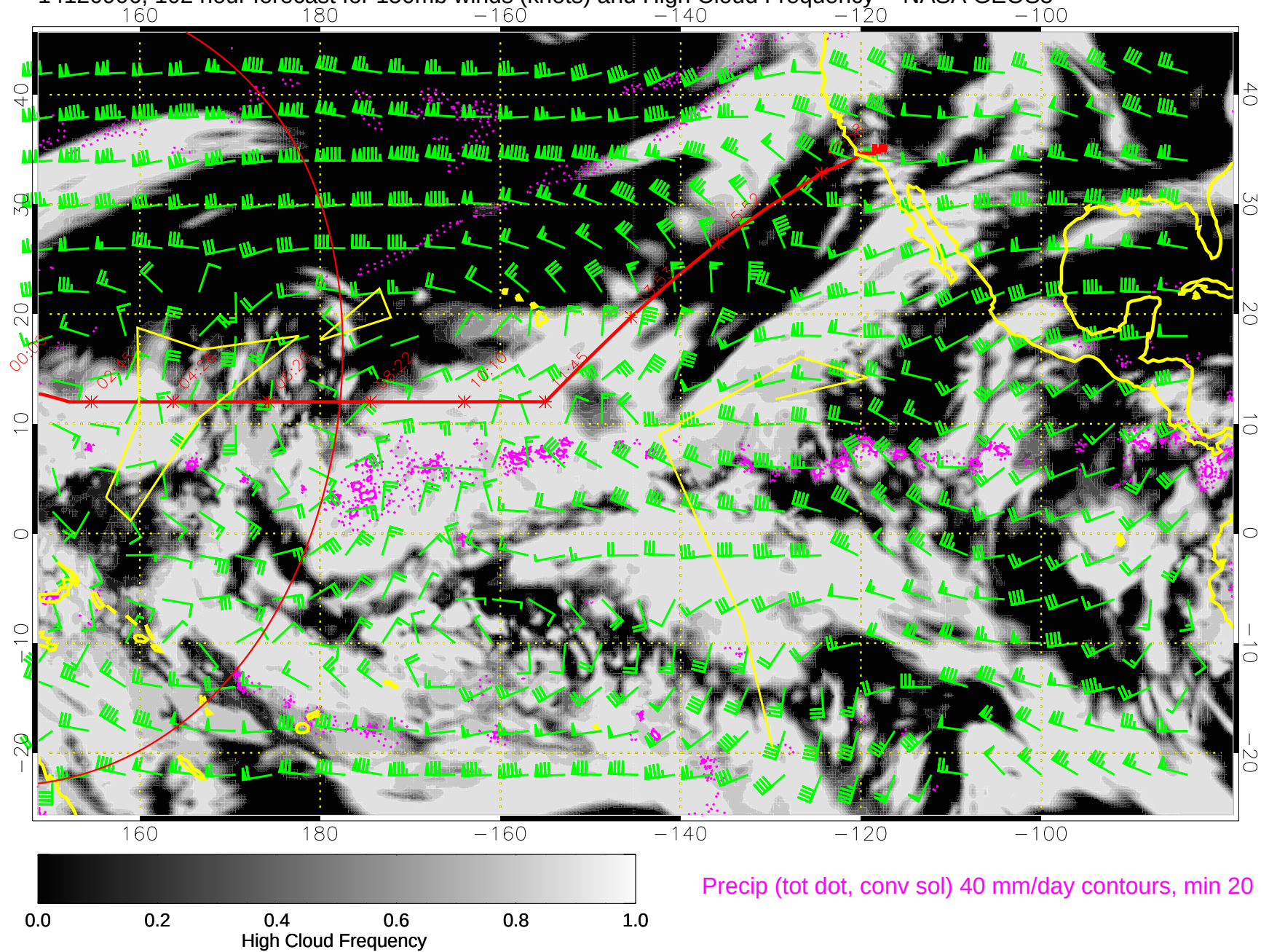
14120906, 102 hour forecast for 150mb winds (knots) and High Cloud Frequency -- NASA GEOS5
