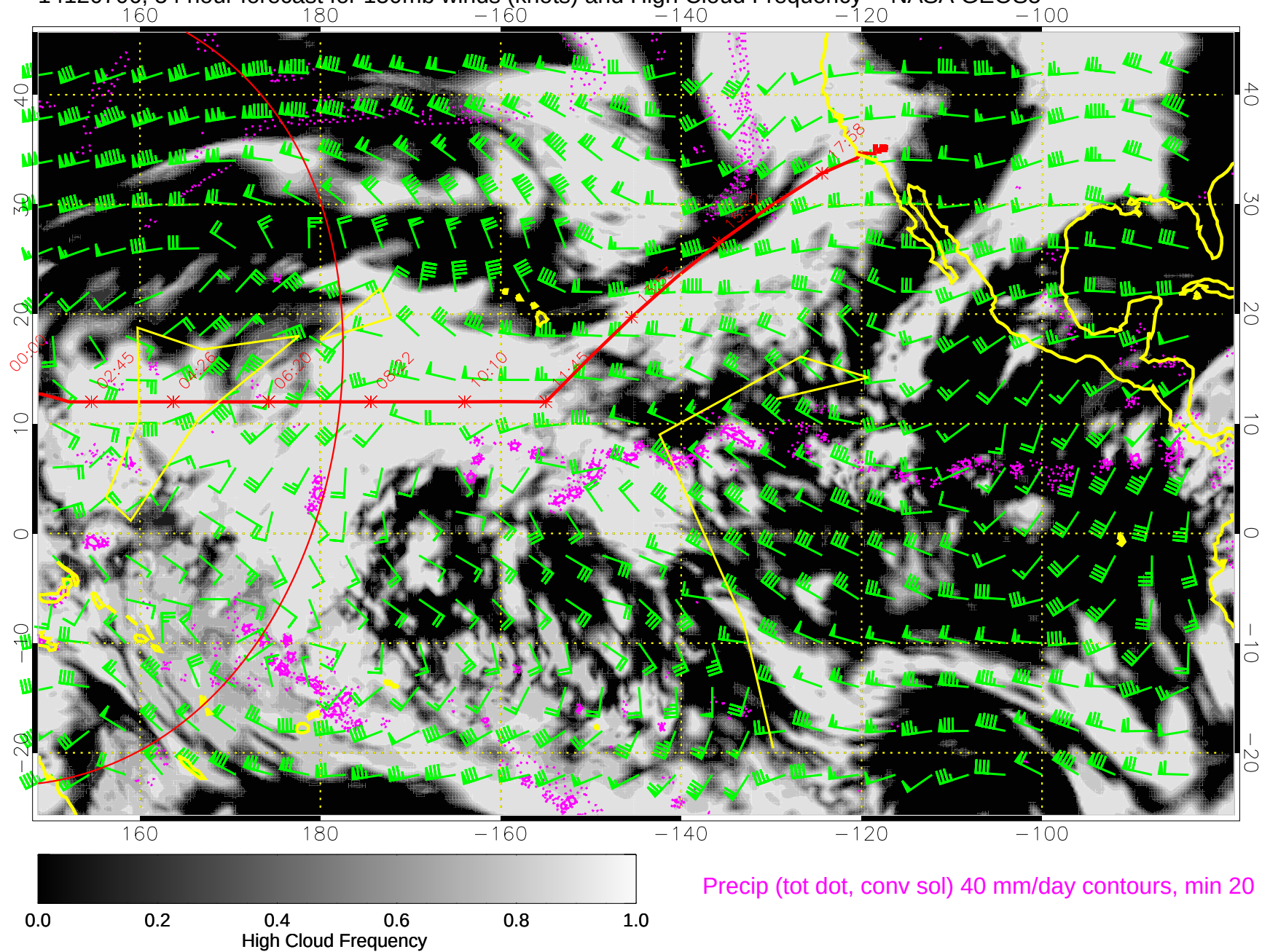
14120706, 54 hour forecast for 150mb winds (knots) and High Cloud Frequency -- NASA GEOS5
