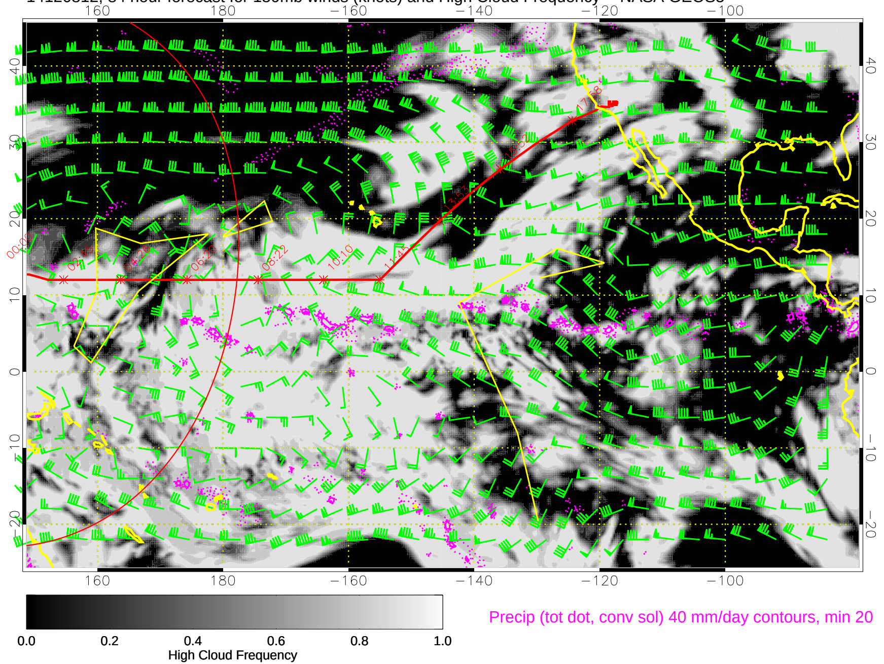
14120812, 84 hour forecast for 150mb winds (knots) and High Cloud Frequency -- NASA GEOS5
