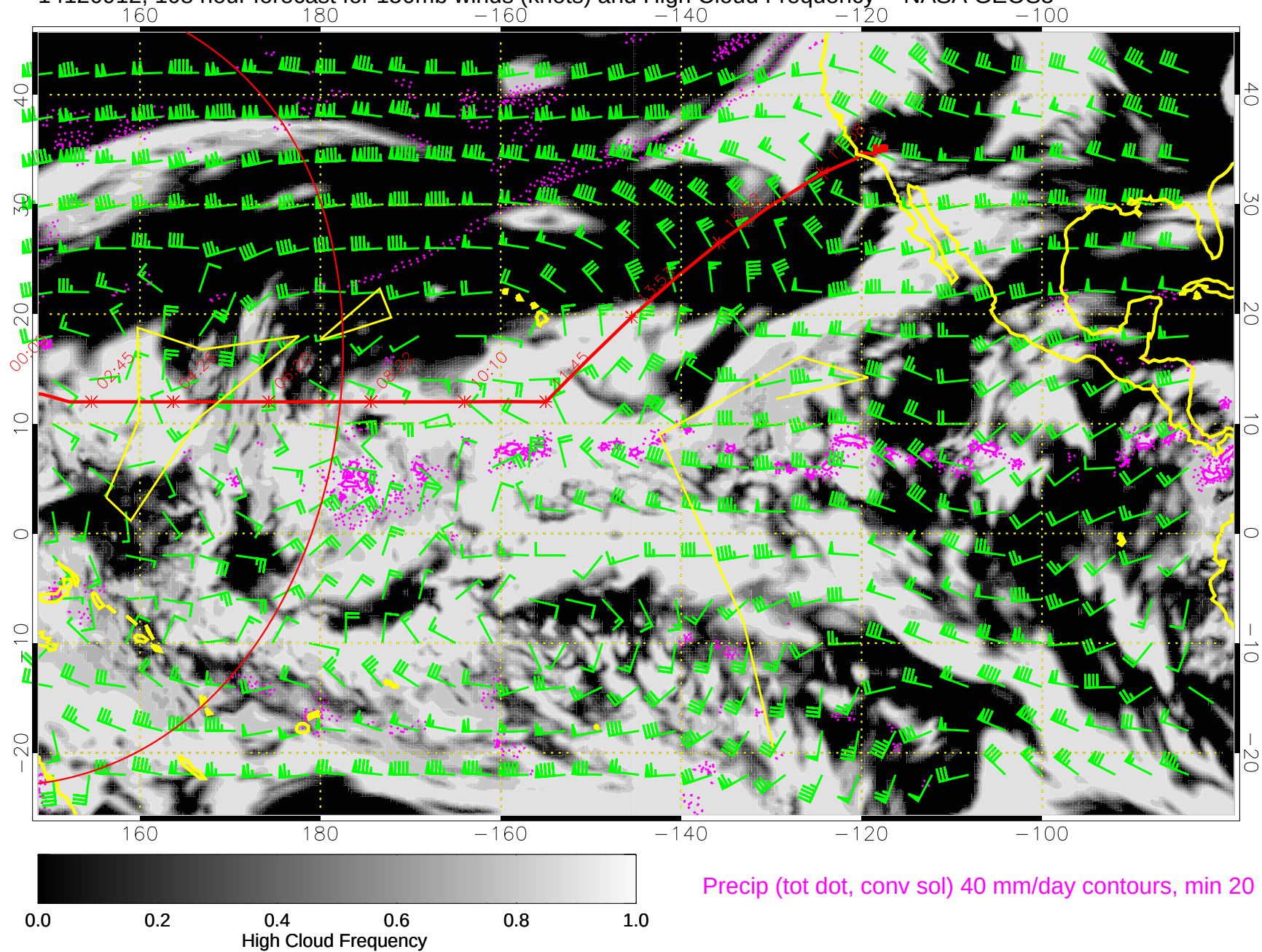
14120912, 108 hour forecast for 150mb winds (knots) and High Cloud Frequency -- NASA GEOS5
