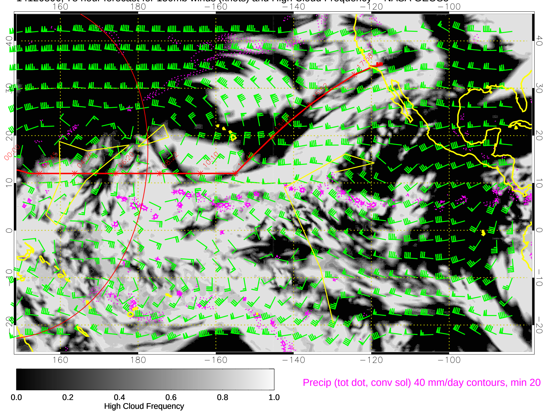
14120806, 78 hour forecast for 150mb winds (knots) and High Cloud Frequency -- NASA GEOS5
