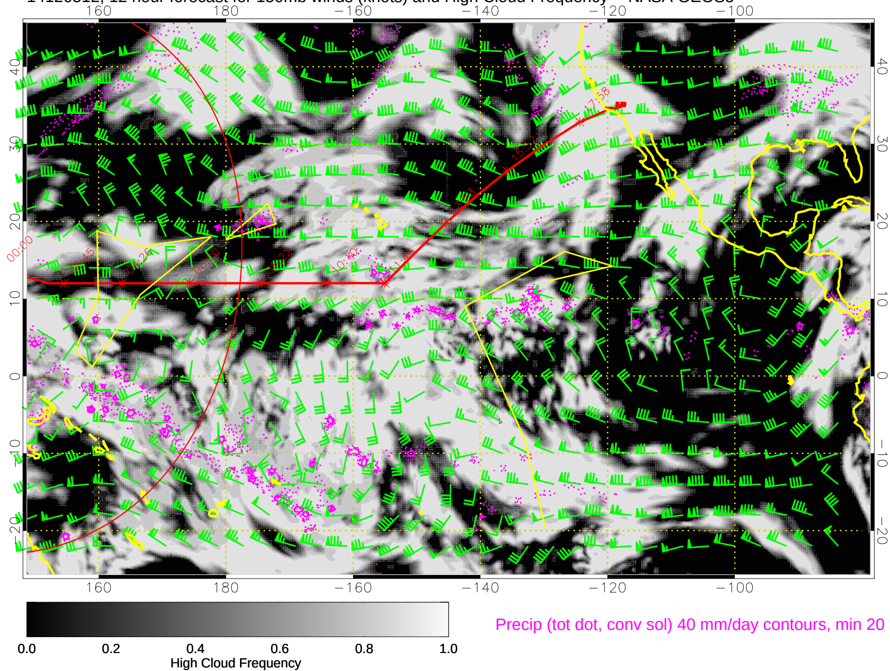
14120512, 12 hour forecast for 150mb winds (knots) and High Cloud Frequency -- NASA GEOS5
