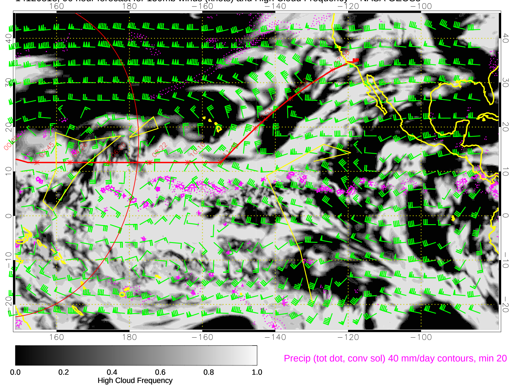
14120818, 90 hour forecast for 150mb winds (knots) and High Cloud Frequency -- NASA GEOS5
