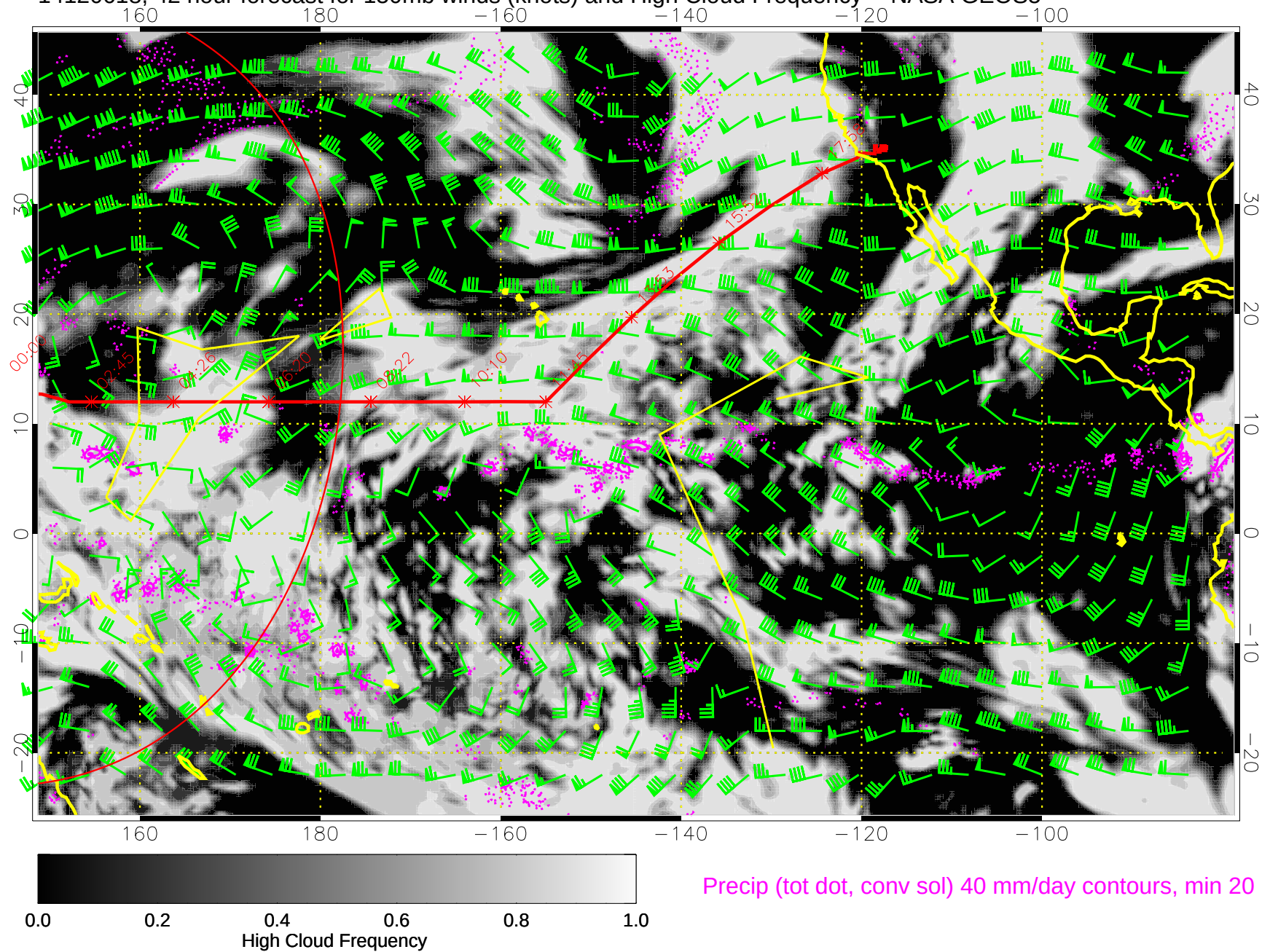
14120618, 42 hour forecast for 150mb winds (knots) and High Cloud Frequency -- NASA GEOS5
