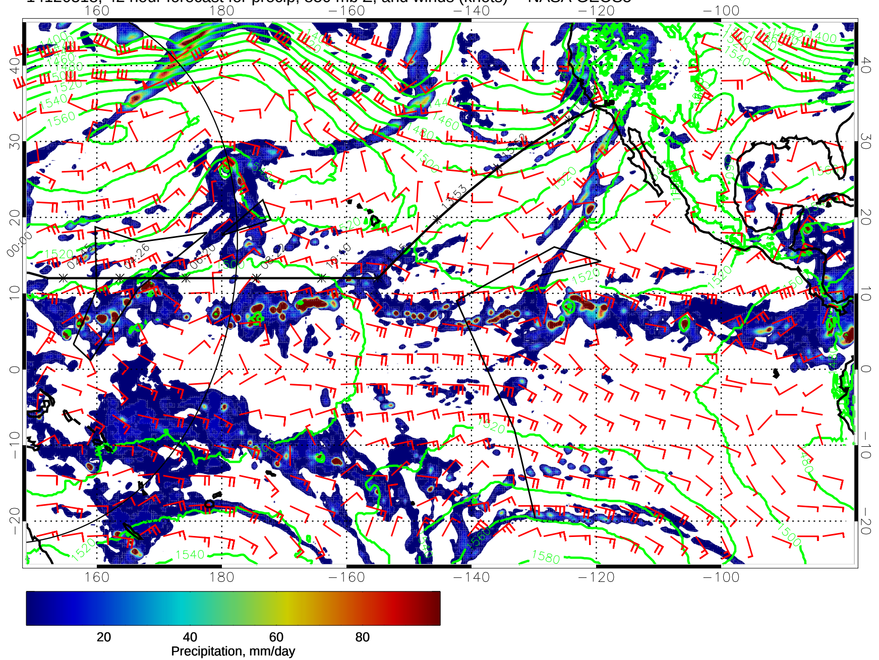
14120318, 42 hour forecast for precip, 850 mb Z, and winds (knots) -- NASA GEOS5
