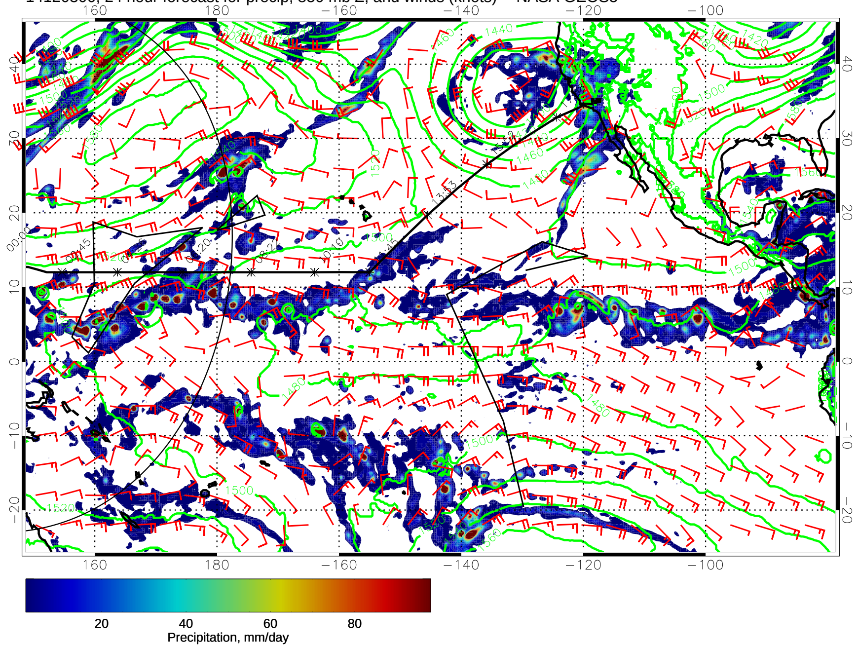
14120300, 24 hour forecast for precip, 850 mb Z, and winds (knots) -- NASA GEOS5
