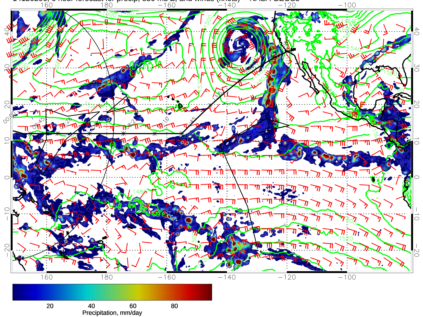
14120206, 6 hour forecast for precip, 850 mb Z, and winds (knots) -- NASA GEOS5
