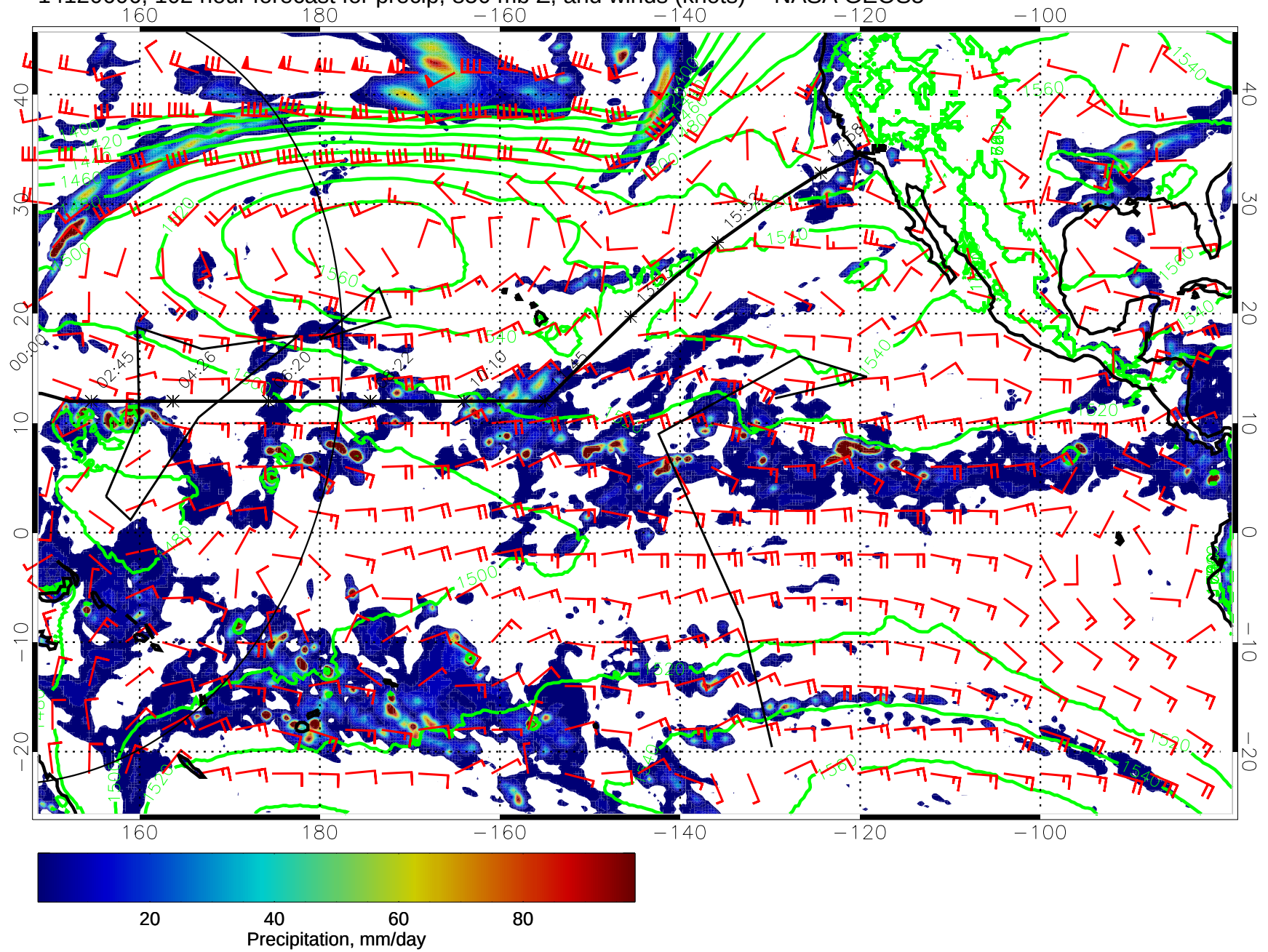
14120606, 102 hour forecast for precip, 850 mb Z, and winds (knots) -- NASA GEOS5
