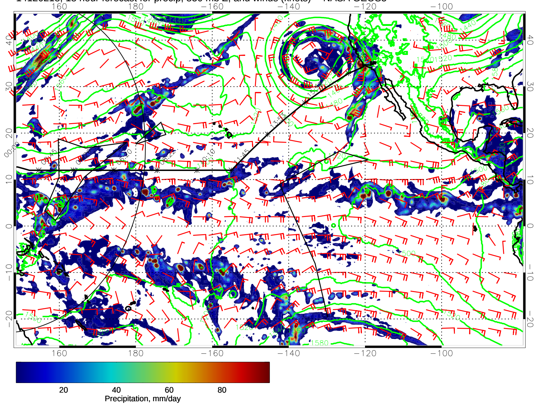
14120218, 18 hour forecast for precip, 850 mb Z, and winds (knots) -- NASA GEOS5
