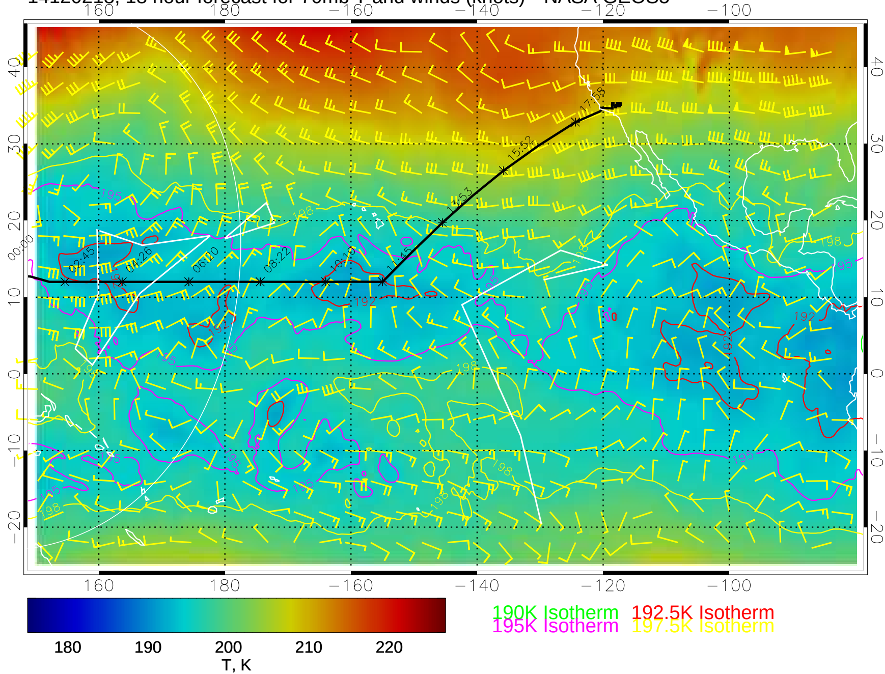
14120218, 18 hour forecast for 70mb T and winds (knots)-- NASA GEOS5
