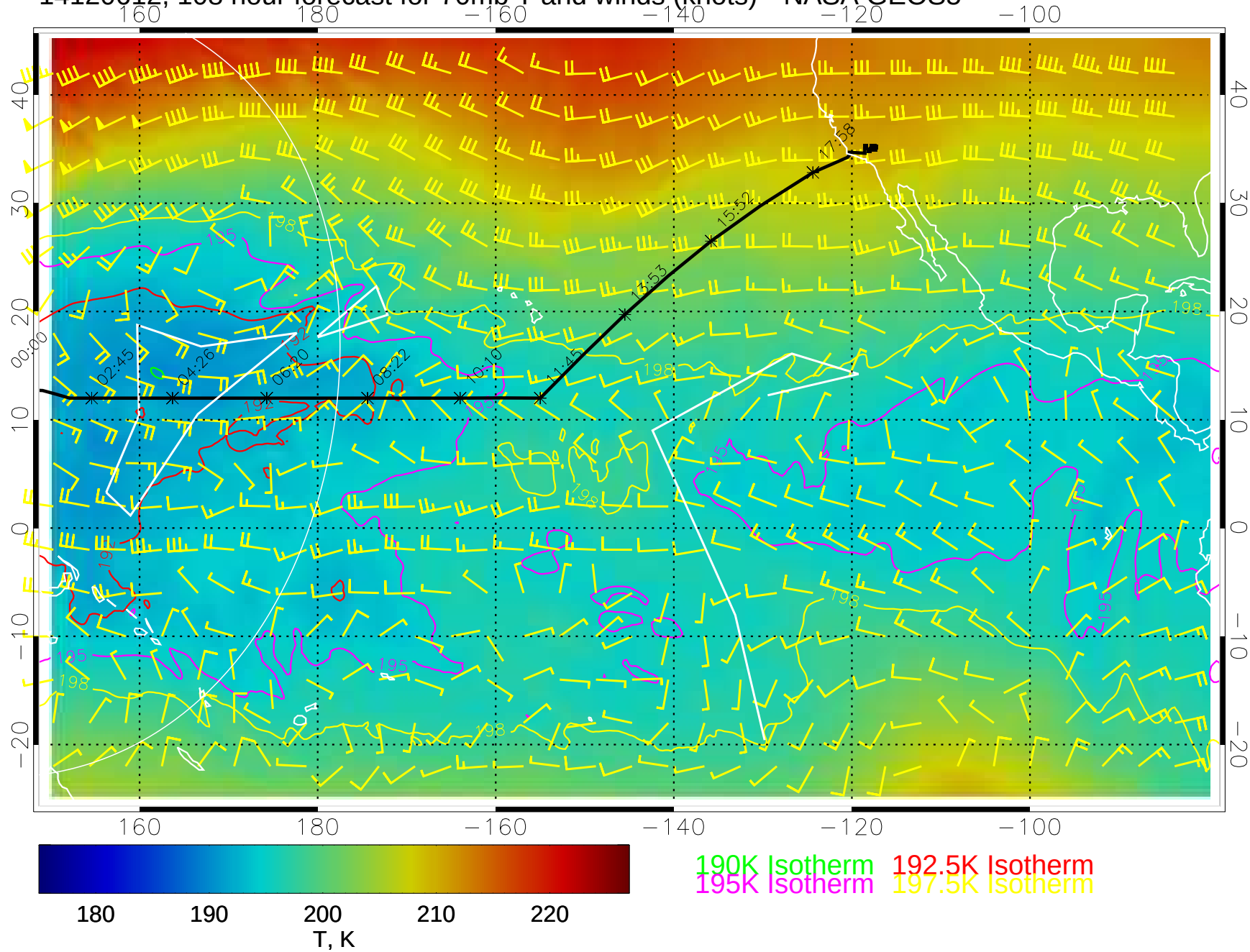
14120612, 108 hour forecast for 70mb T and winds (knots)-- NASA GEOS5
