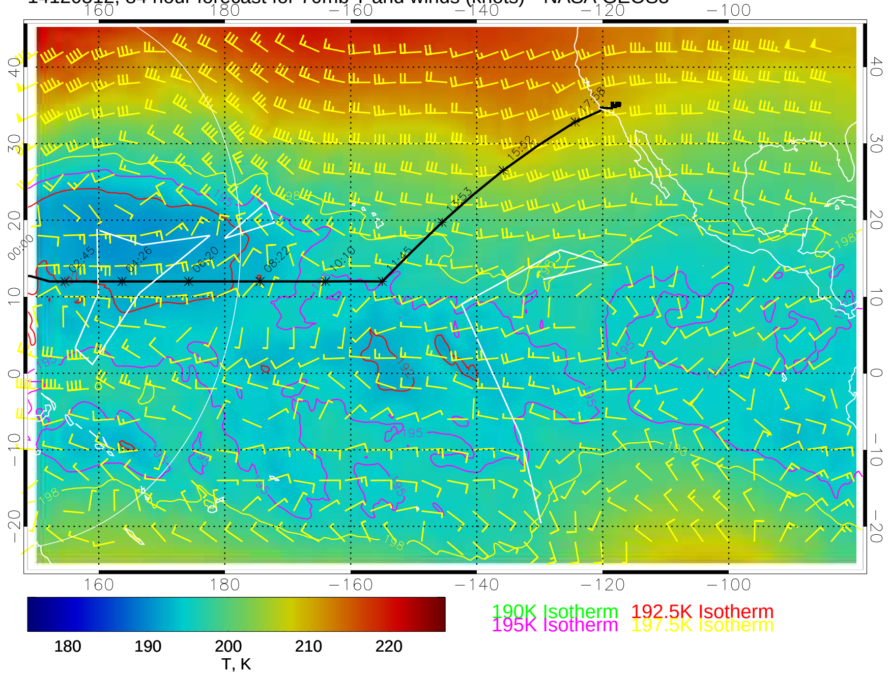
14120512, 84 hour forecast for 70mb T and winds (knots)-- NASA GEOS5
