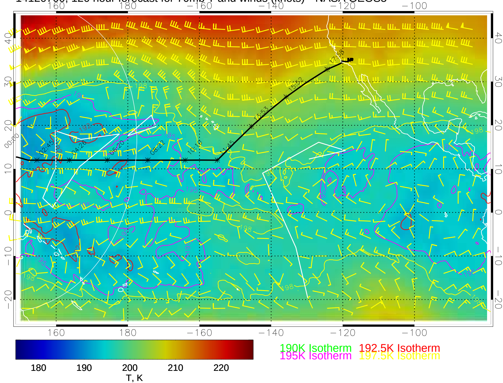
14120700, 120 hour forecast for 70mb T and winds (knots)-- NASA GEOS5
