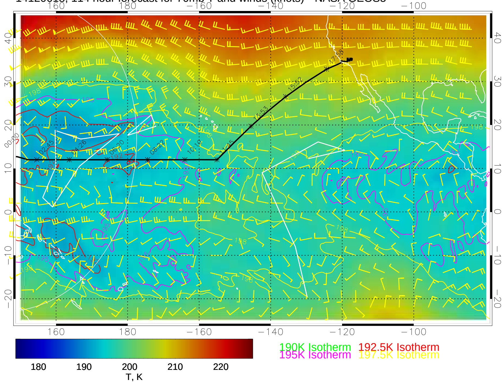
14120618, 114 hour forecast for 70mb T and winds (knots)-- NASA GEOS5
