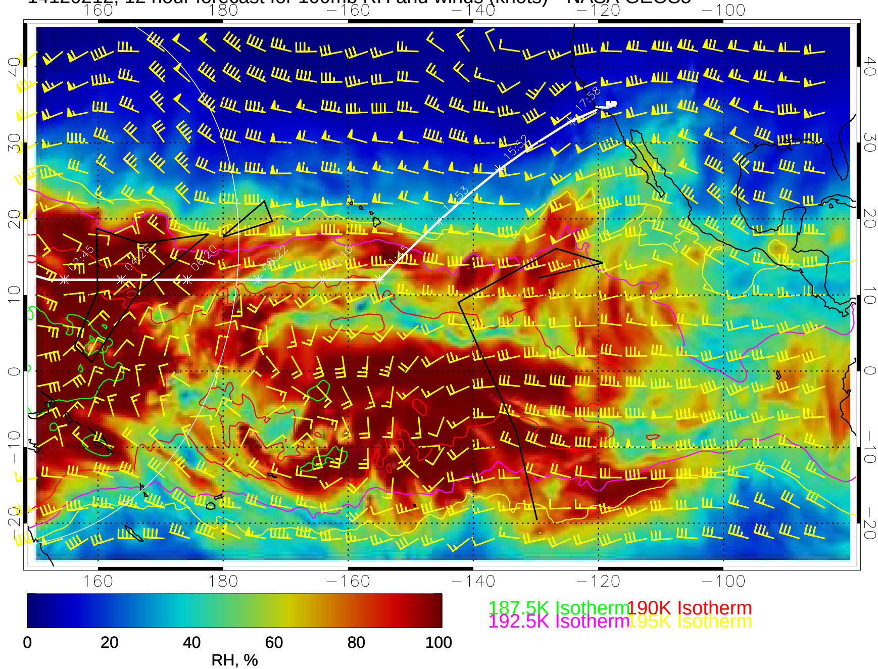
14120212, 12 hour forecast for 100mb RH and winds (knots)-- NASA GEOS5
