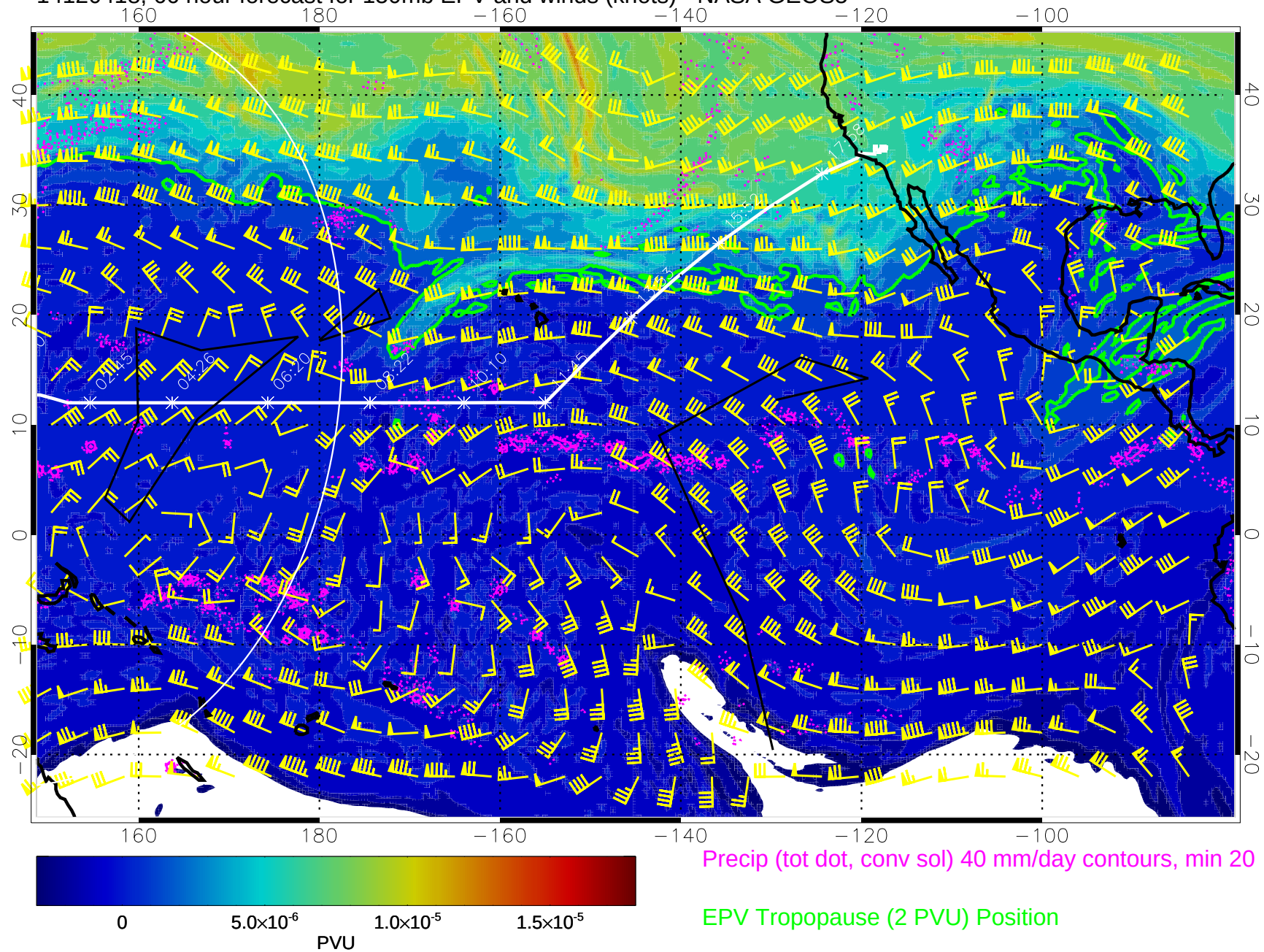
14120418, 66 hour forecast for 150mb EPV and winds (knots) - NASA GEOS5
