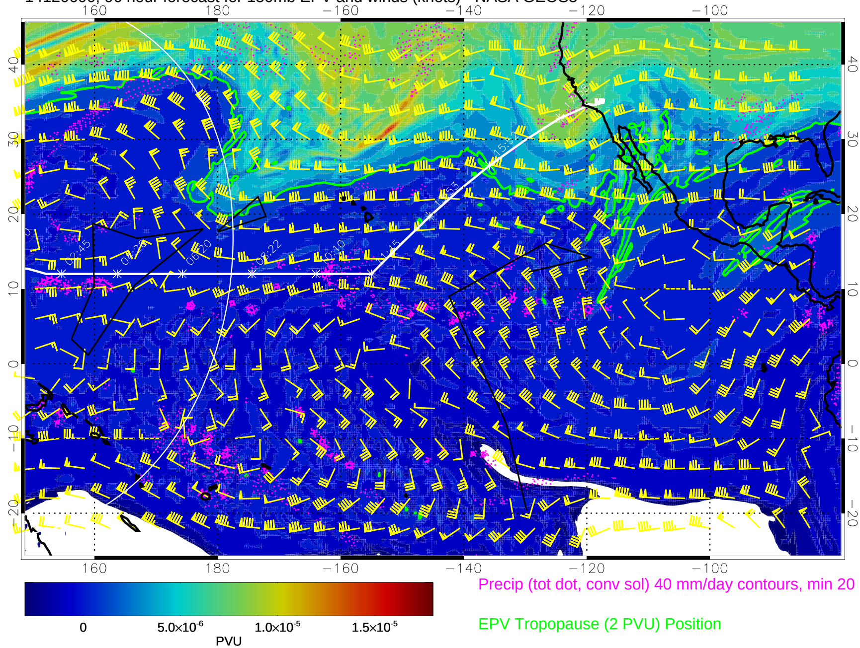
14120600, 96 hour forecast for 150mb EPV and winds (knots) - NASA GEOS5
