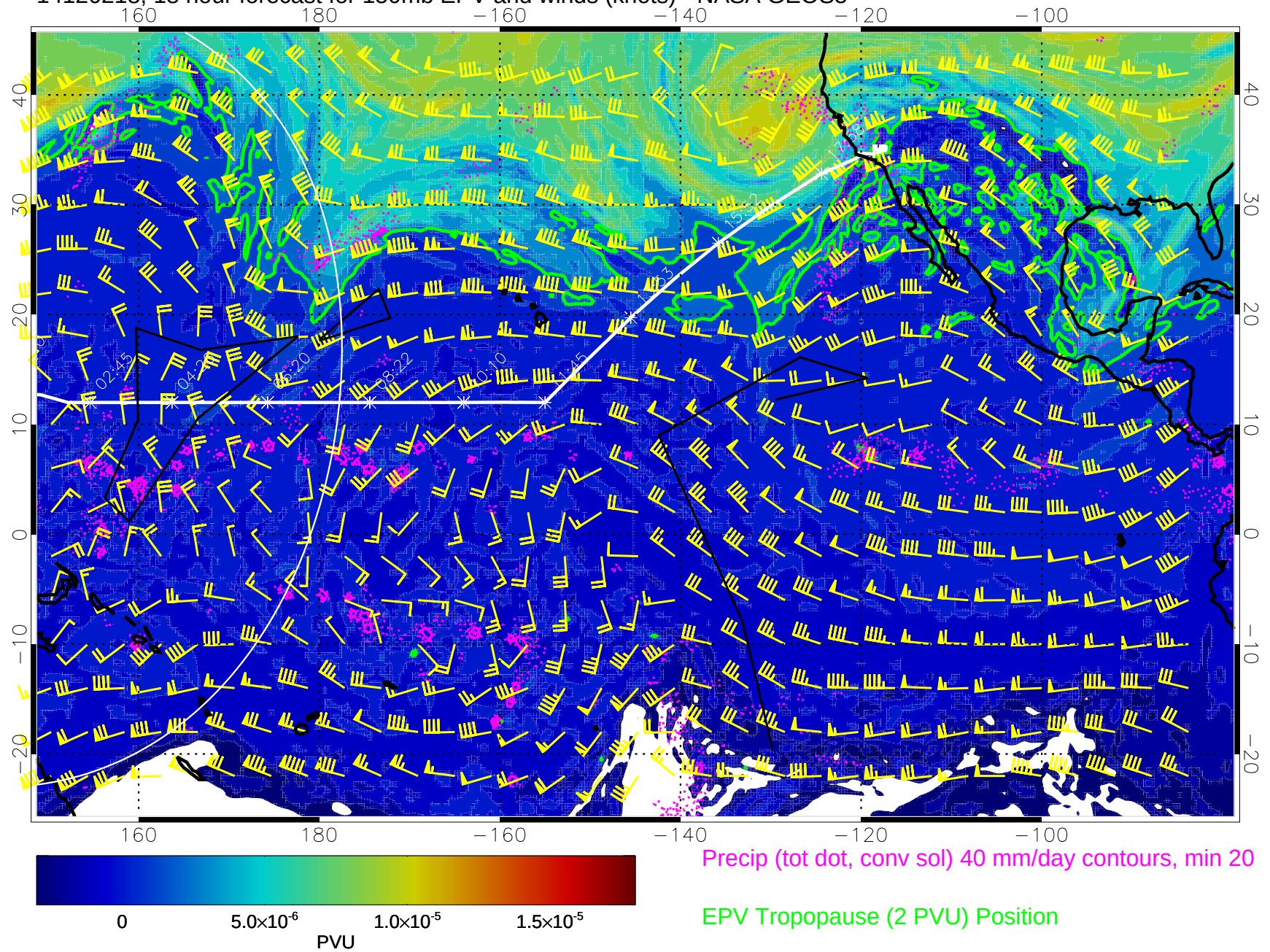
14120218, 18 hour forecast for 150mb EPV and winds (knots) - NASA GEOS5
