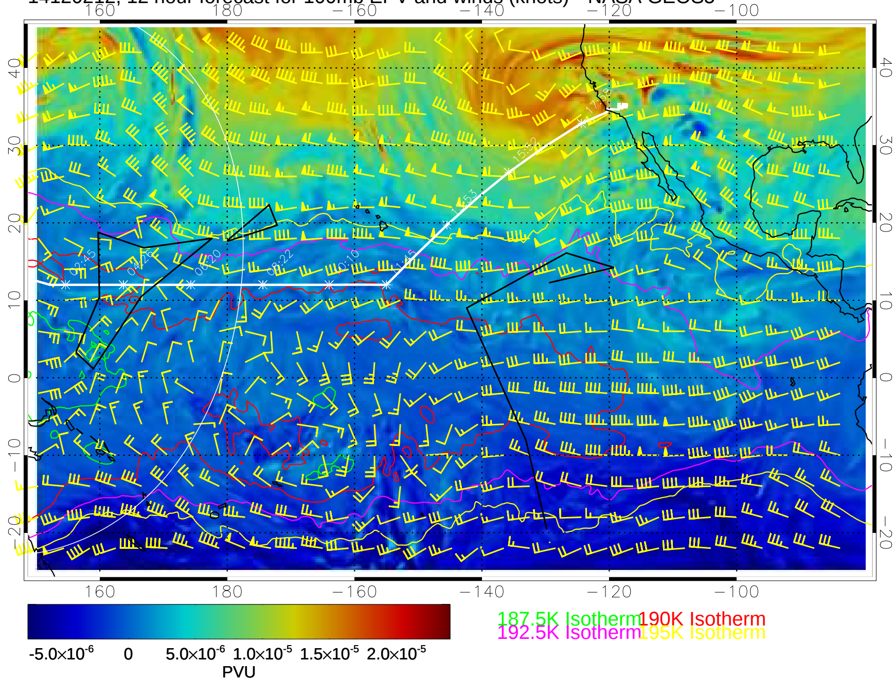
14120212, 12 hour forecast for 100mb EPV and winds (knots)-- NASA GEOS5
