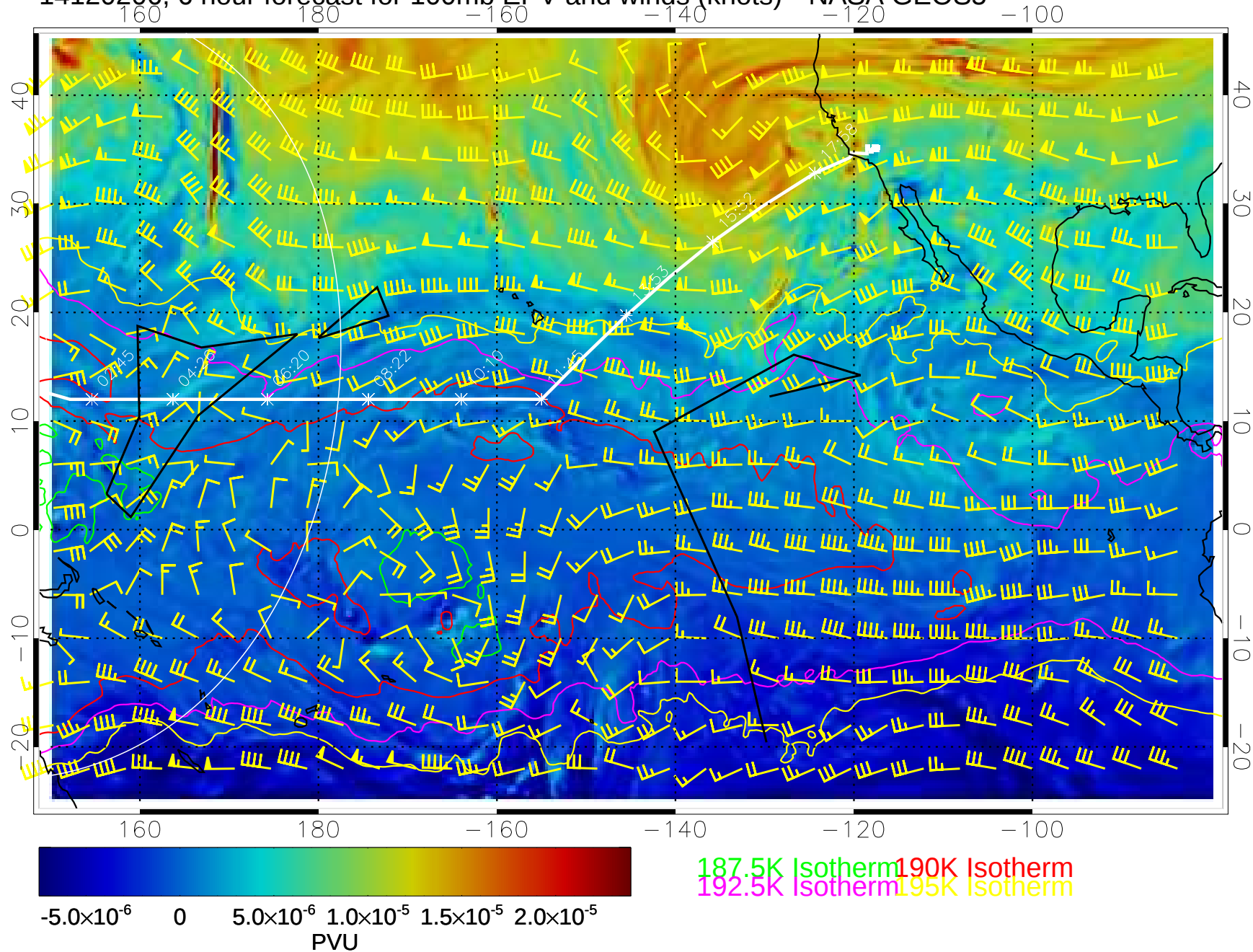
14120206, 6 hour forecast for 100mb EPV and winds (knots)-- NASA GEOS5
