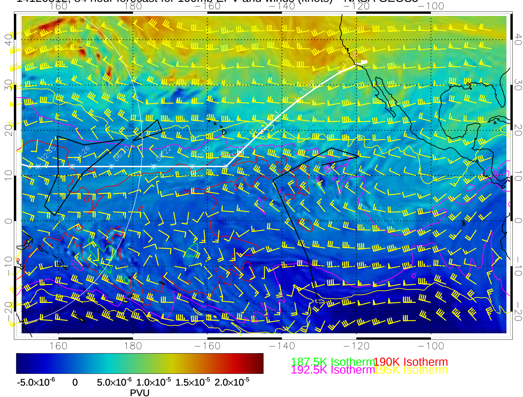
14120512, 84 hour forecast for 100mb EPV and winds (knots)-- NASA GEOS5
