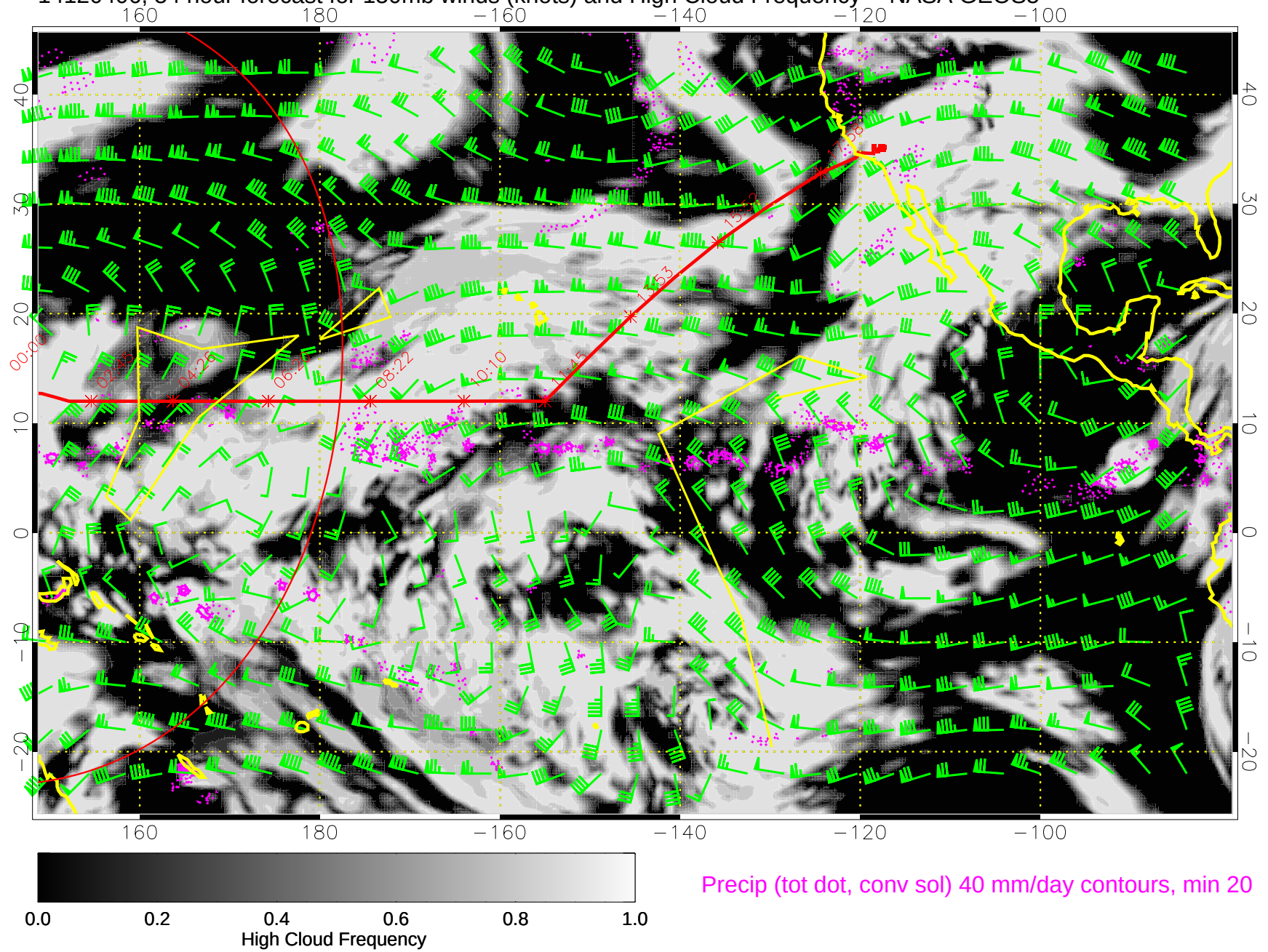
14120406, 54 hour forecast for 150mb winds (knots) and High Cloud Frequency -- NASA GEOS5
