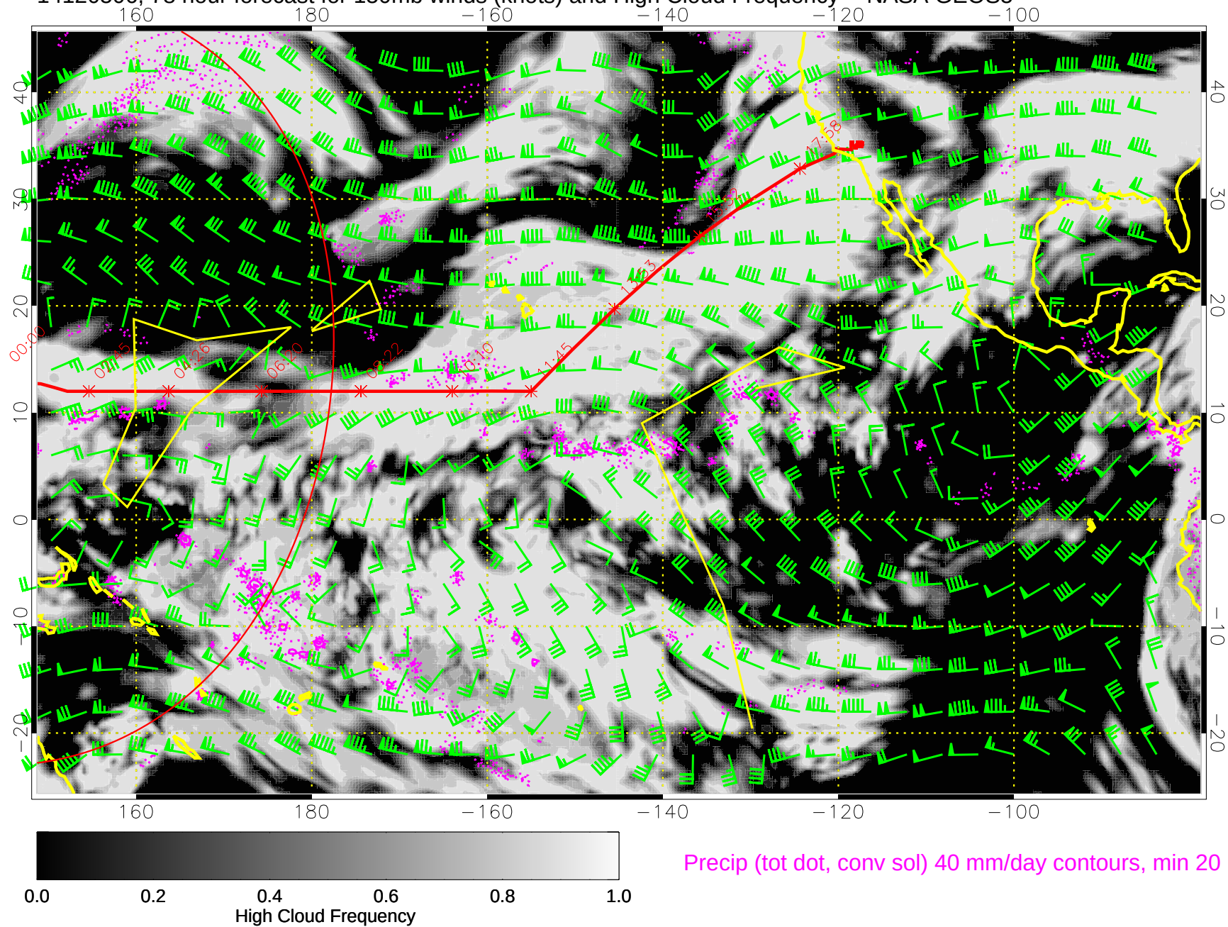
14120506, 78 hour forecast for 150mb winds (knots) and High Cloud Frequency -- NASA GEOS5
