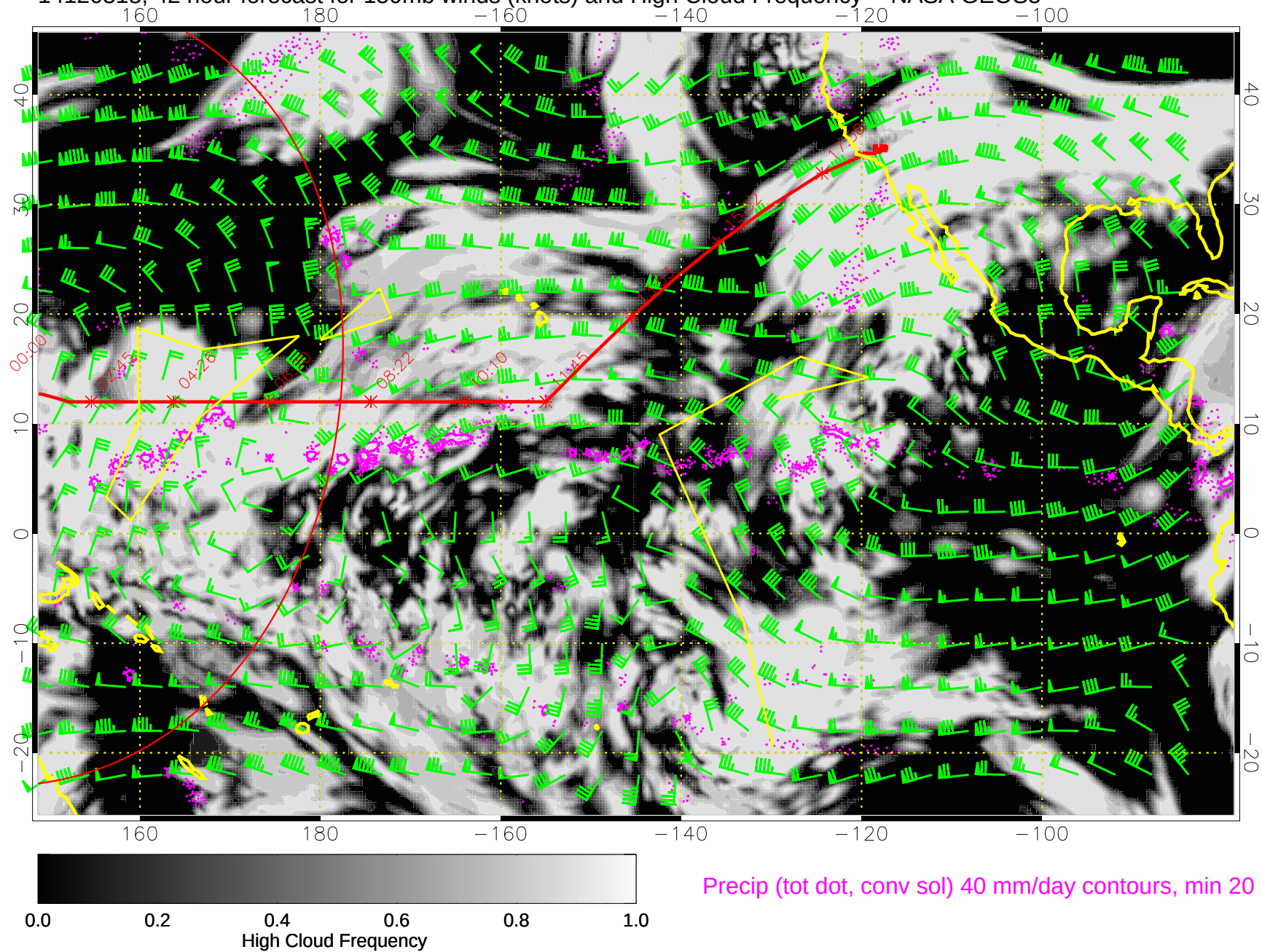
14120318, 42 hour forecast for 150mb winds (knots) and High Cloud Frequency -- NASA GEOS5
