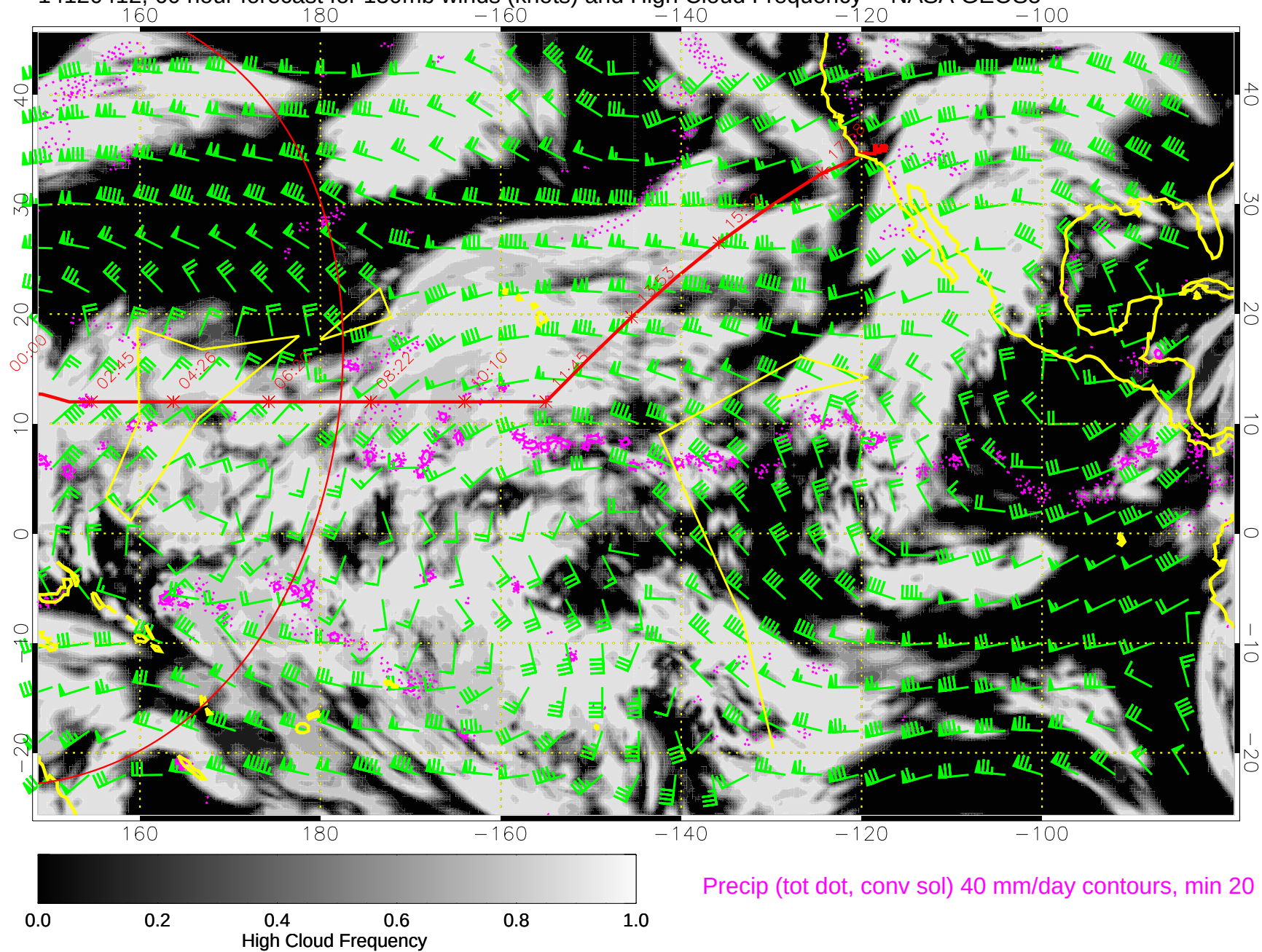
14120412, 60 hour forecast for 150mb winds (knots) and High Cloud Frequency -- NASA GEOS5
