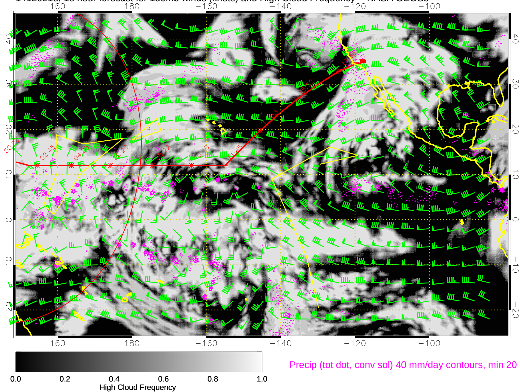
14120218, 18 hour forecast for 150mb winds (knots) and High Cloud Frequency -- NASA GEOS5
