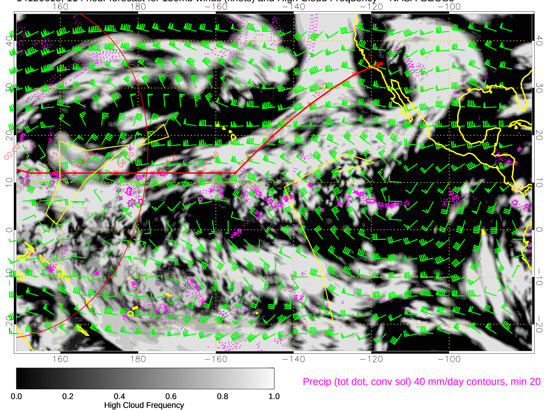
14120618, 114 hour forecast for 150mb winds (knots) and High Cloud Frequency -- NASA GEOS5
