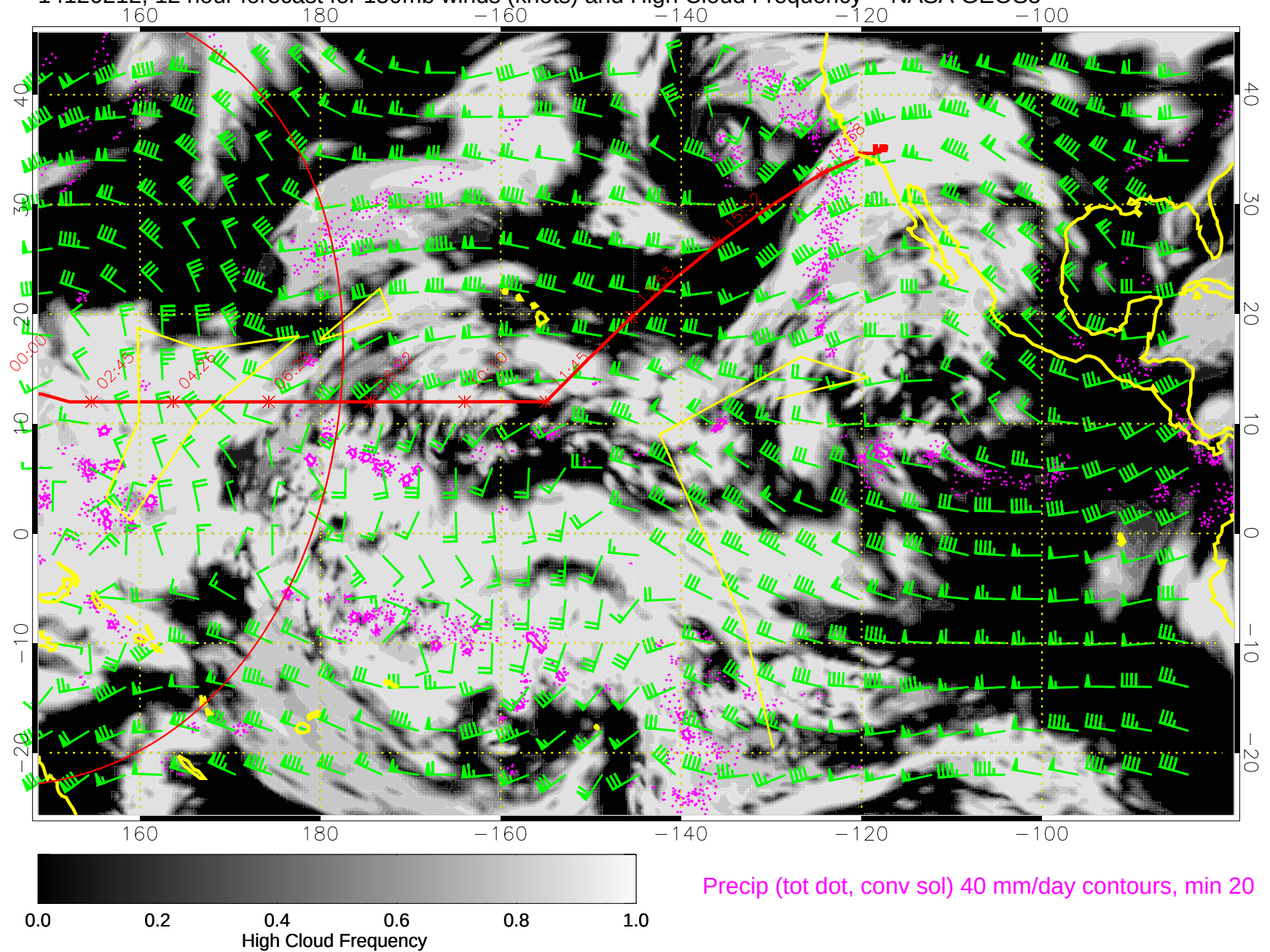
14120212, 12 hour forecast for 150mb winds (knots) and High Cloud Frequency -- NASA GEOS5
