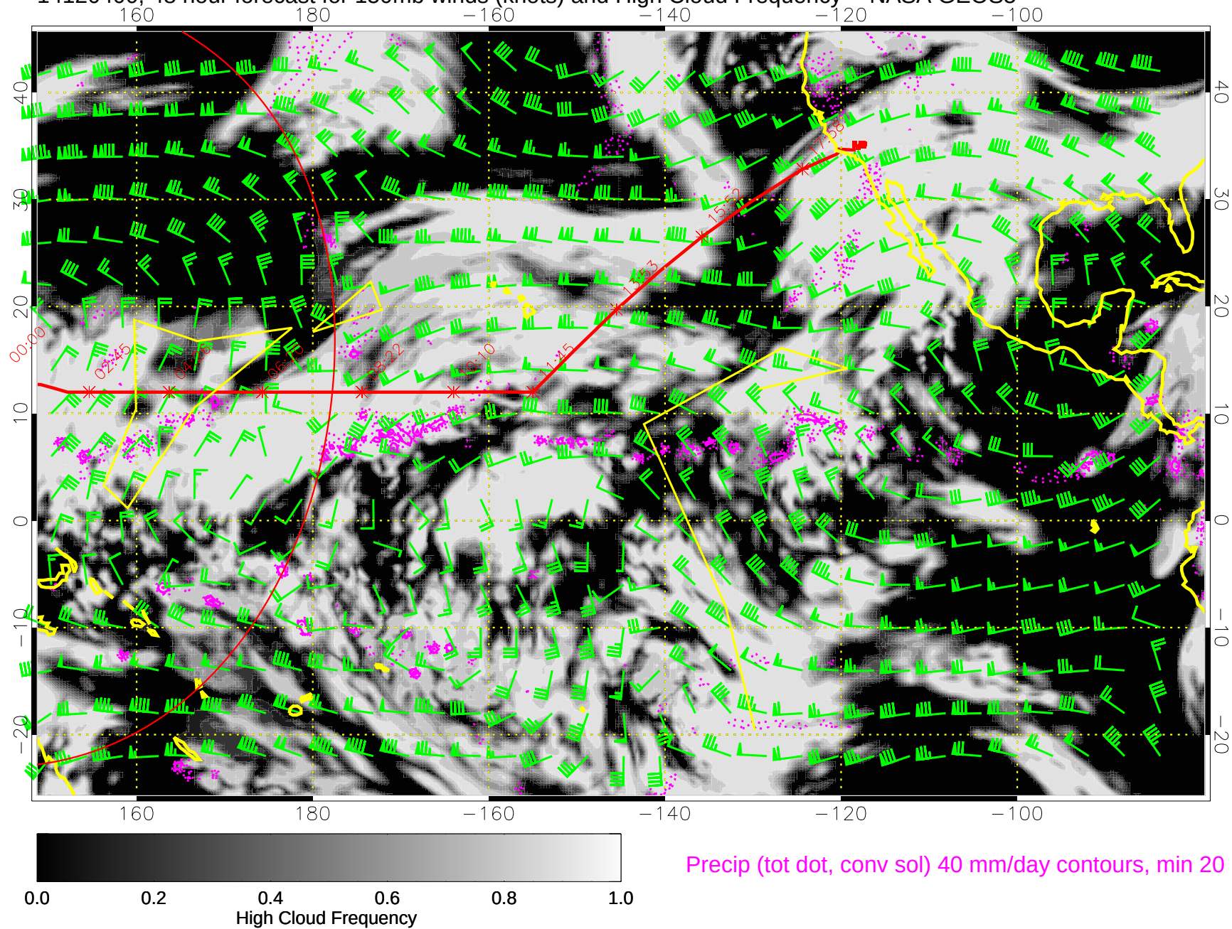
14120400, 48 hour forecast for 150mb winds (knots) and High Cloud Frequency -- NASA GEOS5
