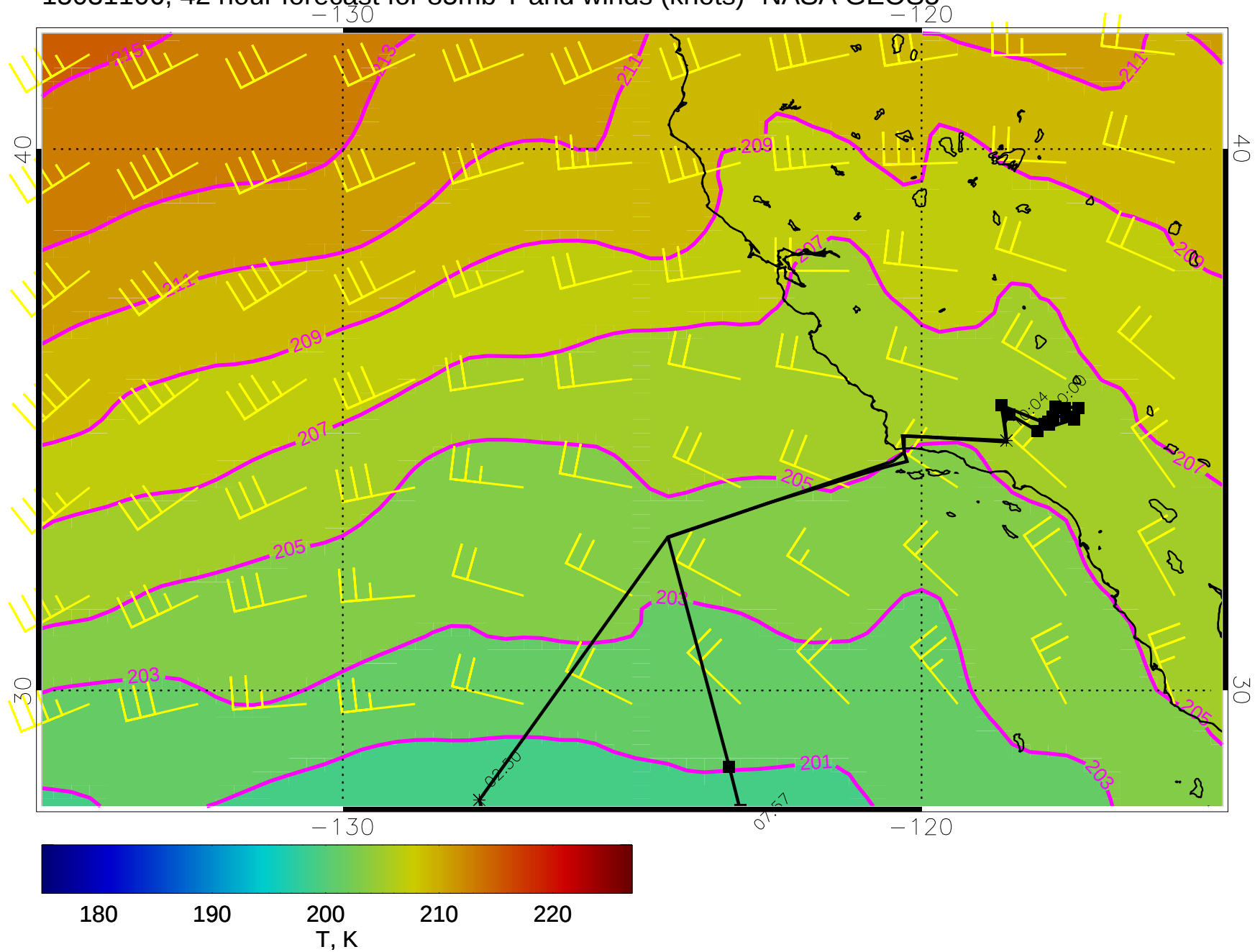
15031106, 42 hour forecast for 85mb T and winds (knots)- NASA GEOS5
