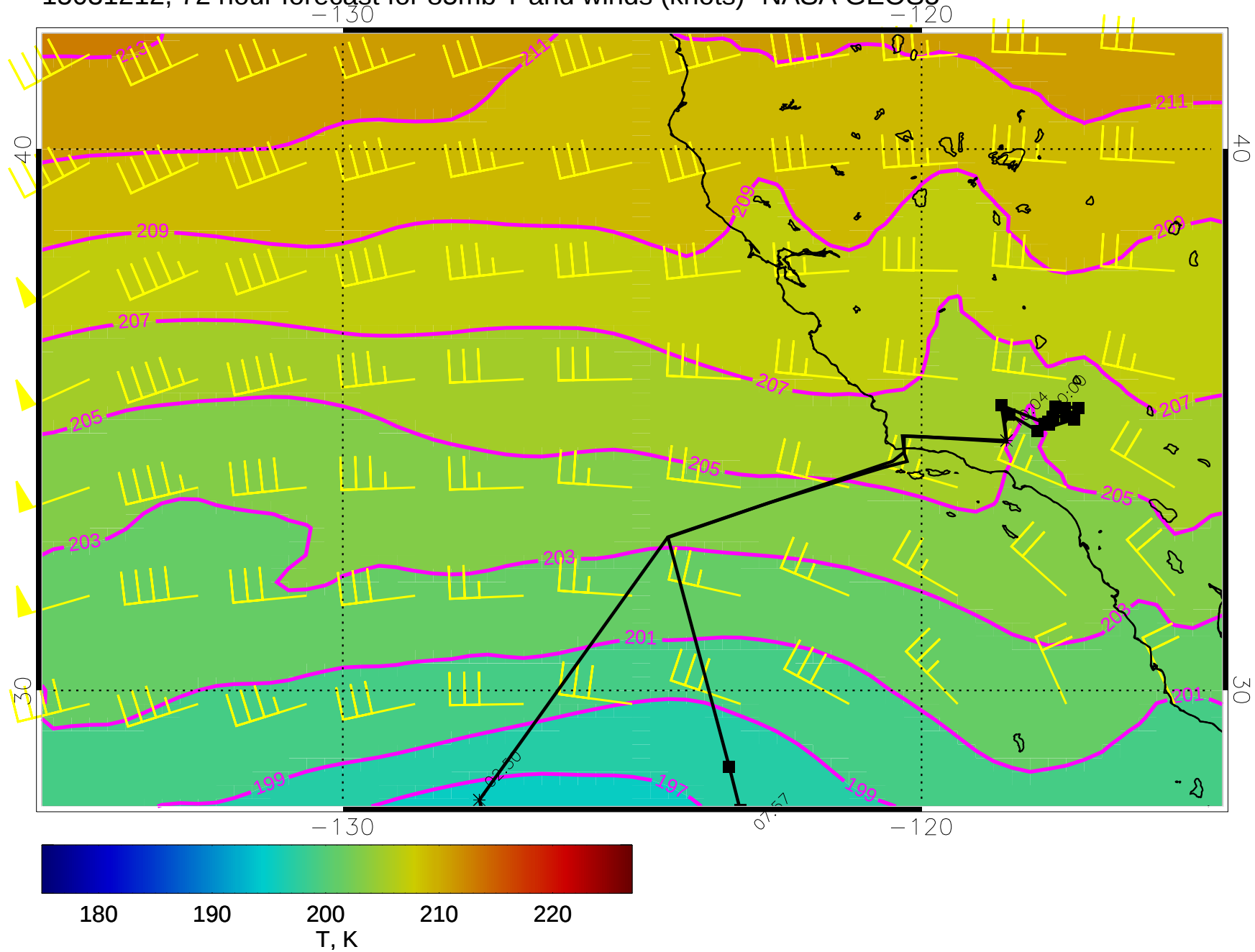
15031212, 72 hour forecast for 85mb T and winds (knots)- NASA GEOS5
