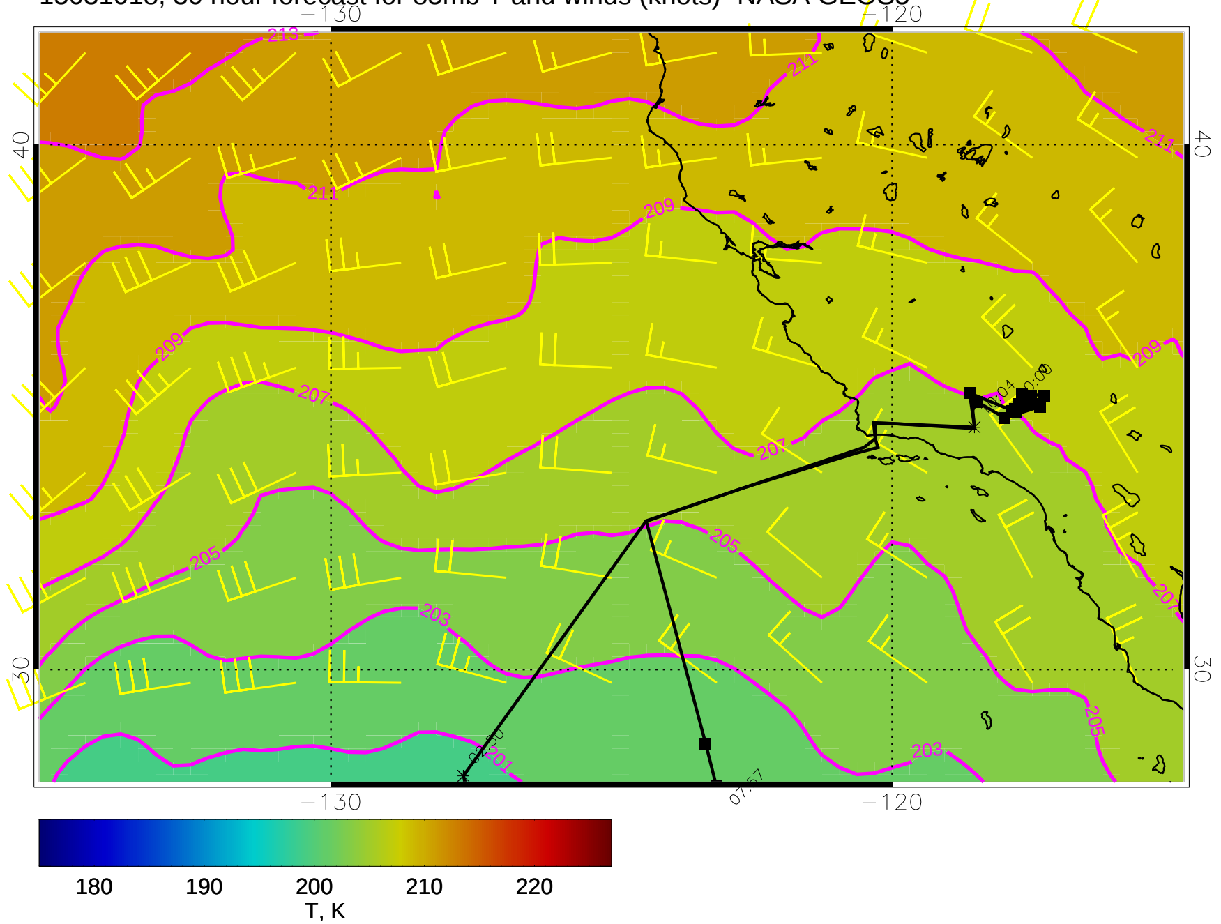
15031018, 30 hour forecast for 85mb T and winds (knots)- NASA GEOS5
