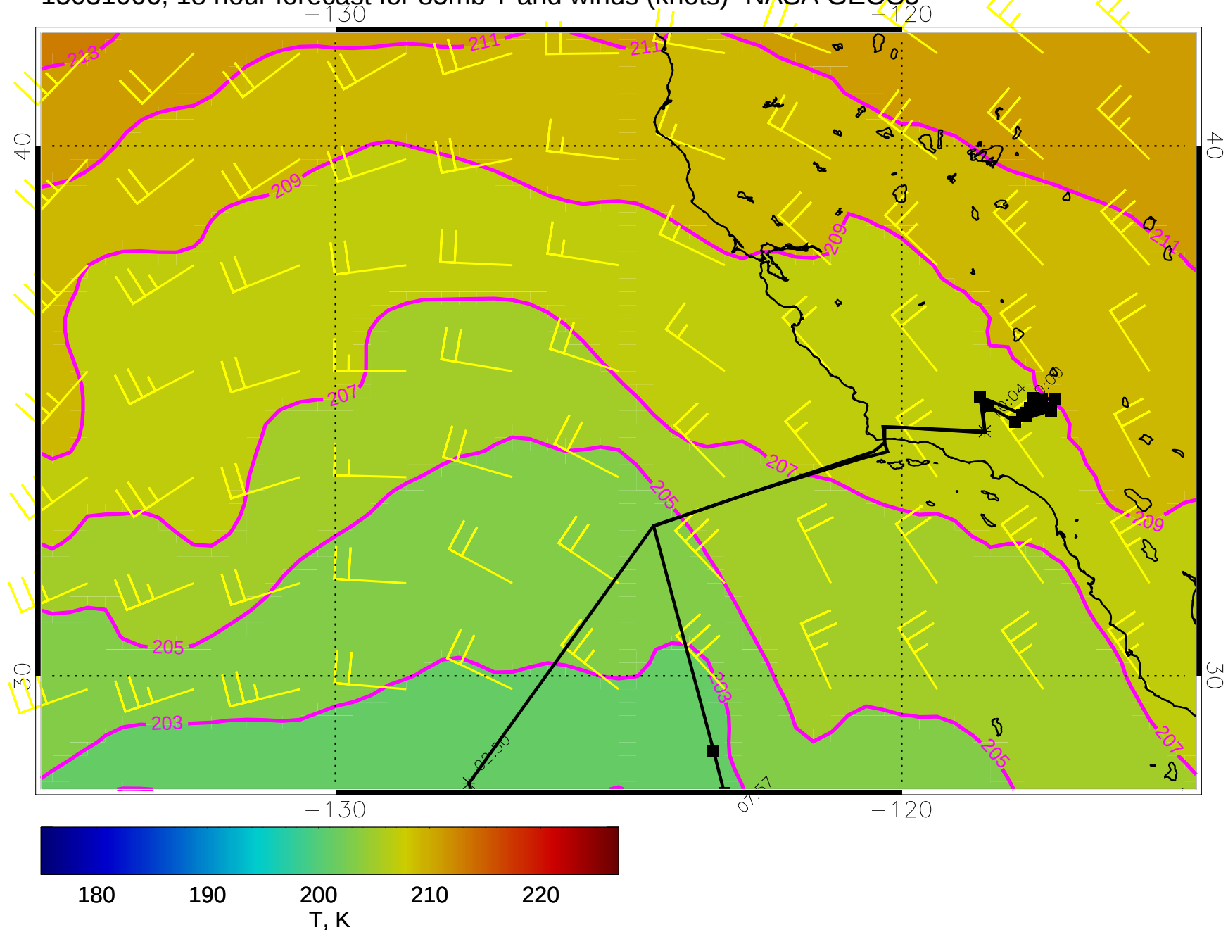
15031006, 18 hour forecast for 85mb T and winds (knots)- NASA GEOS5
