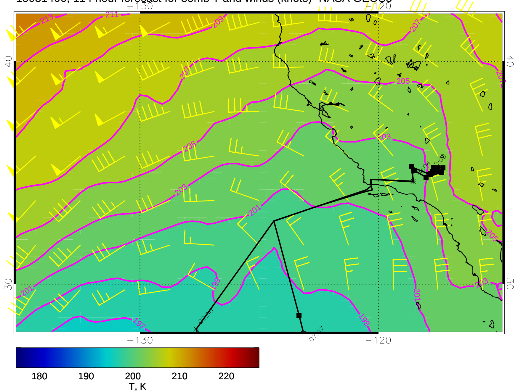
15031406, 114 hour forecast for 85mb T and winds (knots)- NASA GEOS5
