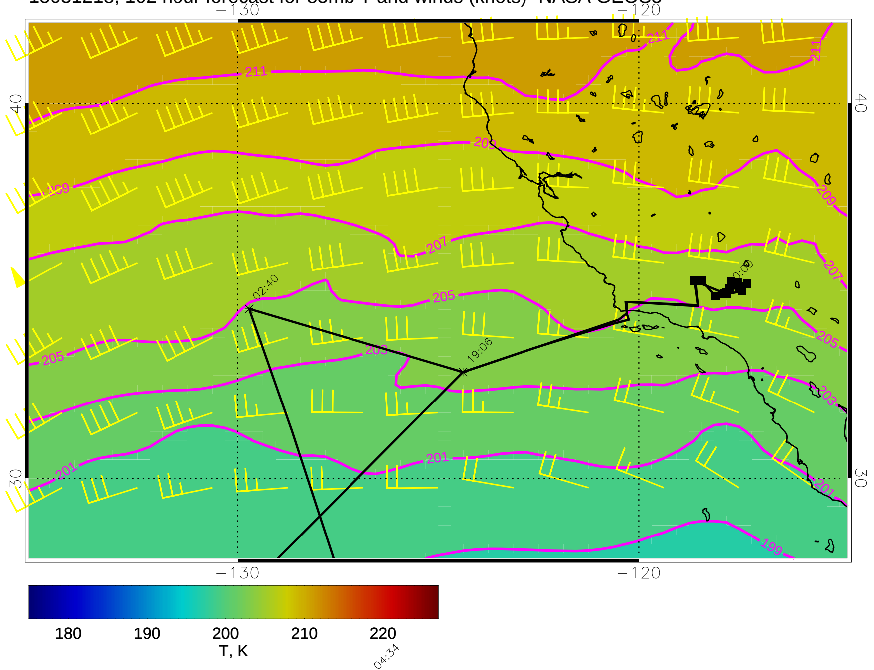
15031218, 102 hour forecast for 85mb T and winds (knots)- NASA GEOS5
