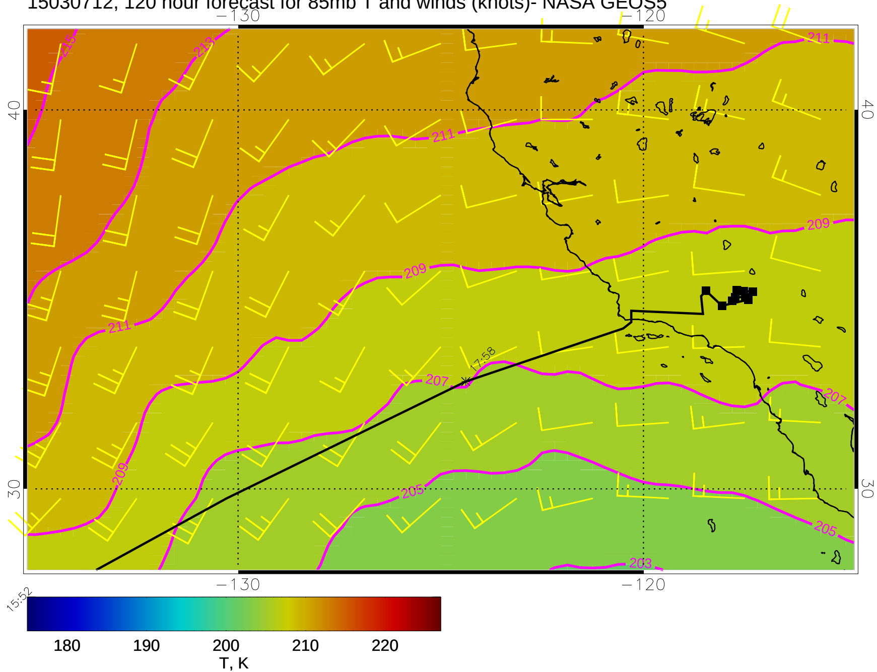
15030712, 120 hour forecast for 85mb T and winds (knots)- NASA GEOS5
