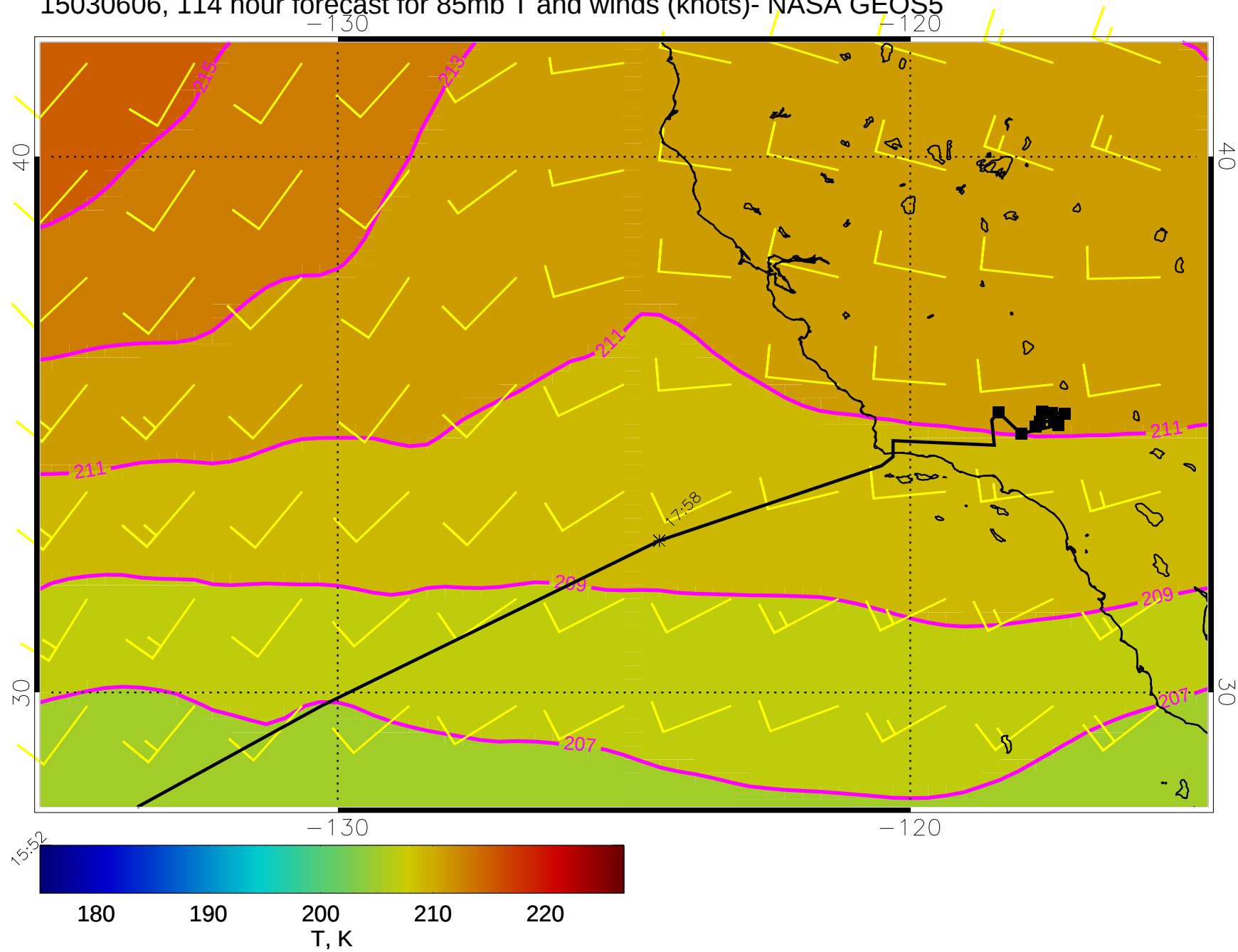
15030606, 114 hour forecast for 85mb T and winds (knots)- NASA GEOS5
