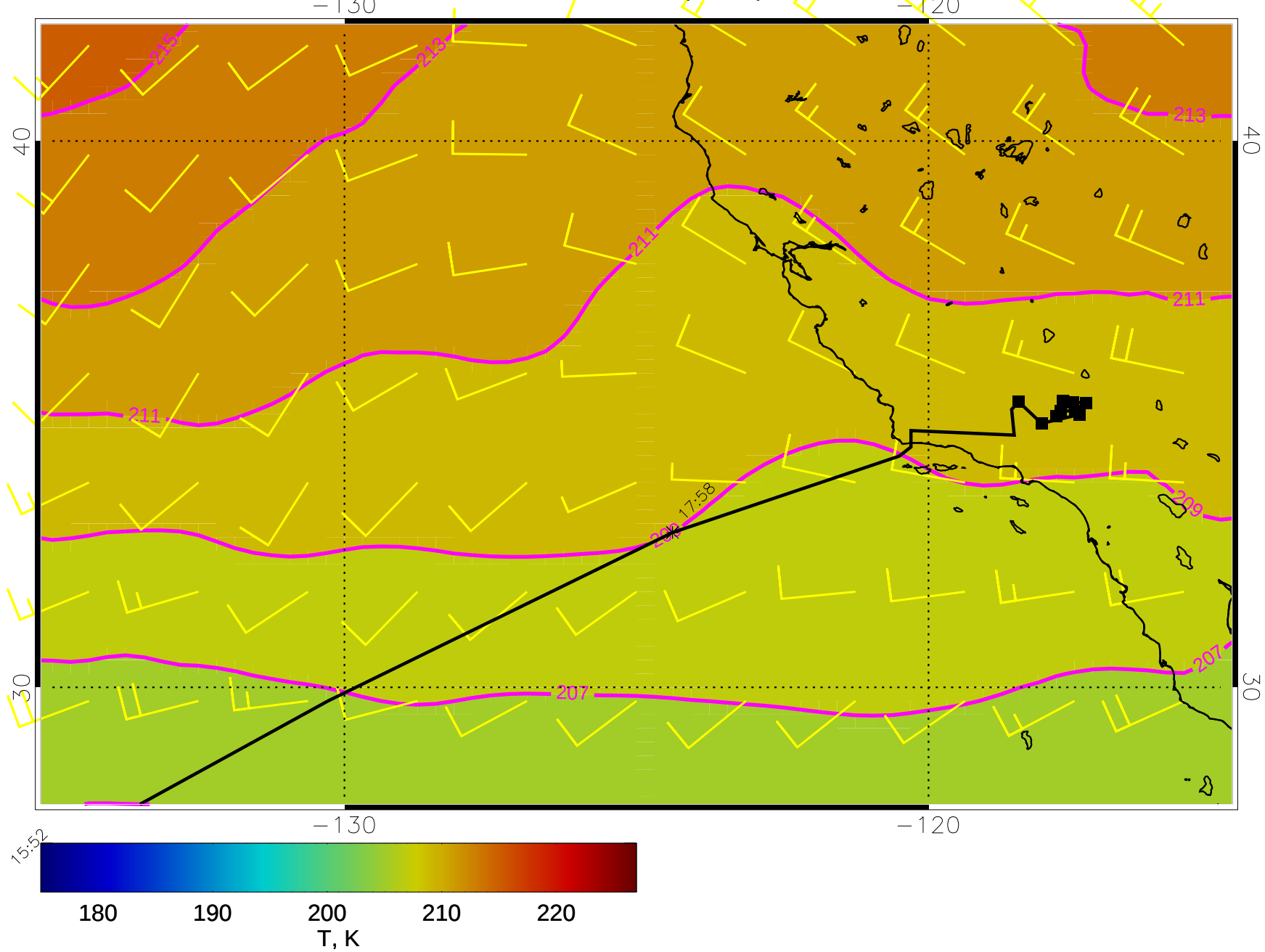
15030512, 108 hour forecast for 85mb T and winds (knots)- NASA GEOS5
