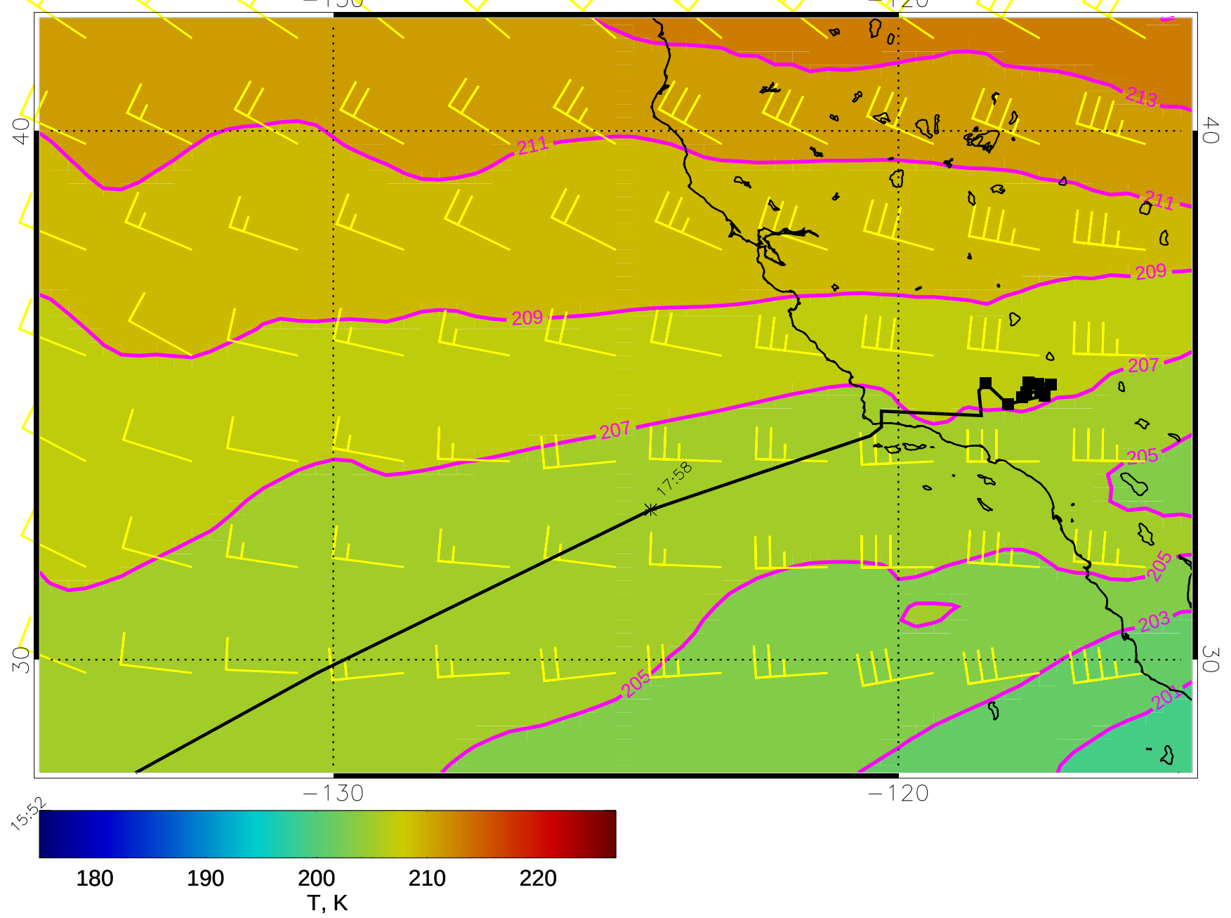
15022012, 24 hour forecast for 85mb T and winds (knots)- NASA GEOS5
