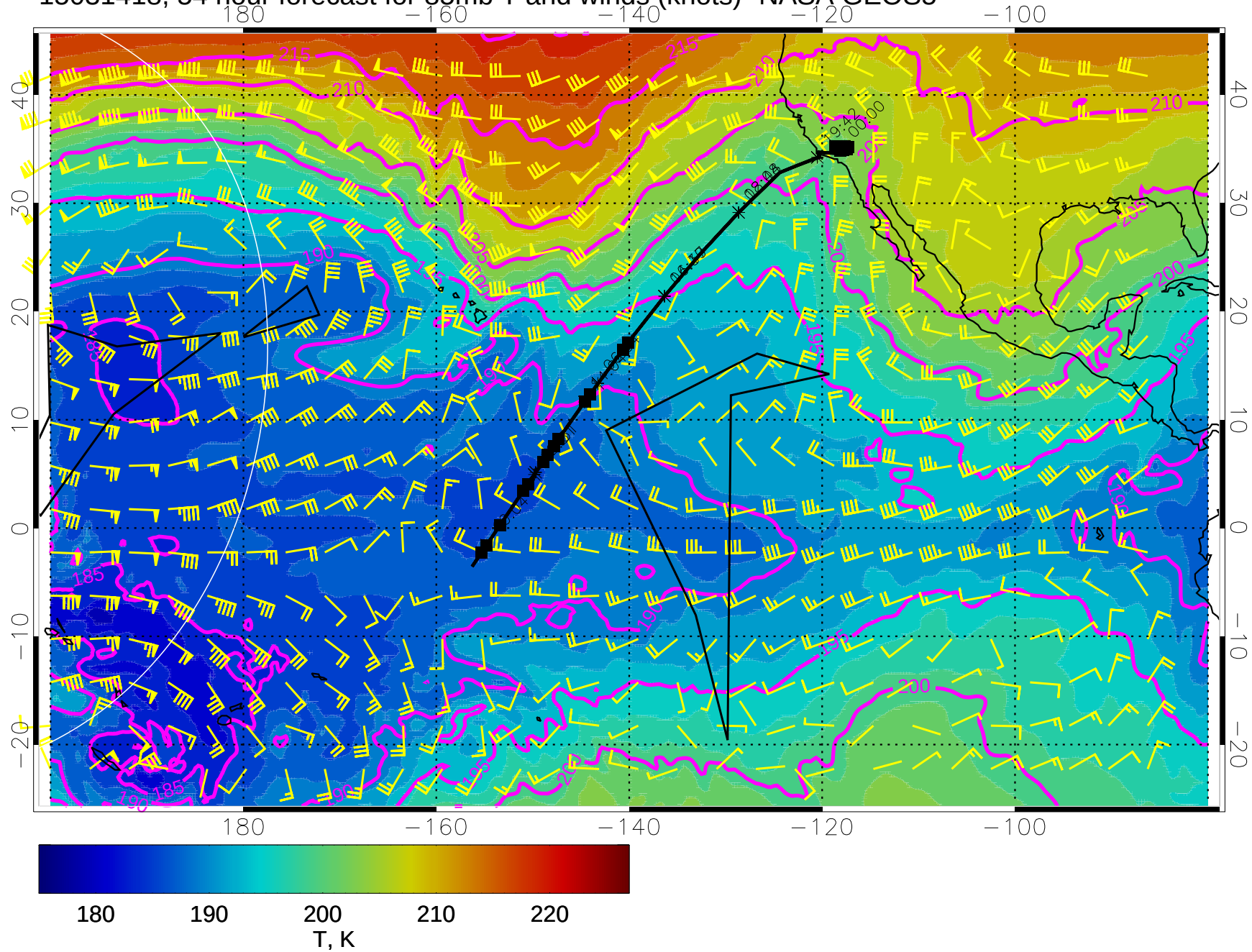
15031418, 54 hour forecast for 85mb T and winds (knots)- NASA GEOS5
