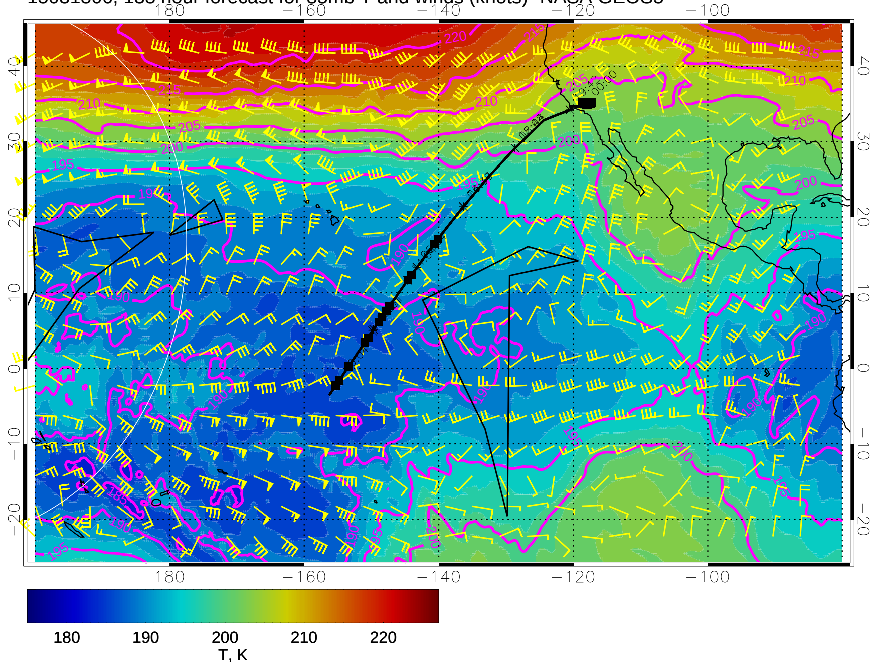
15031806, 138 hour forecast for 85mb T and winds (knots)- NASA GEOS5
