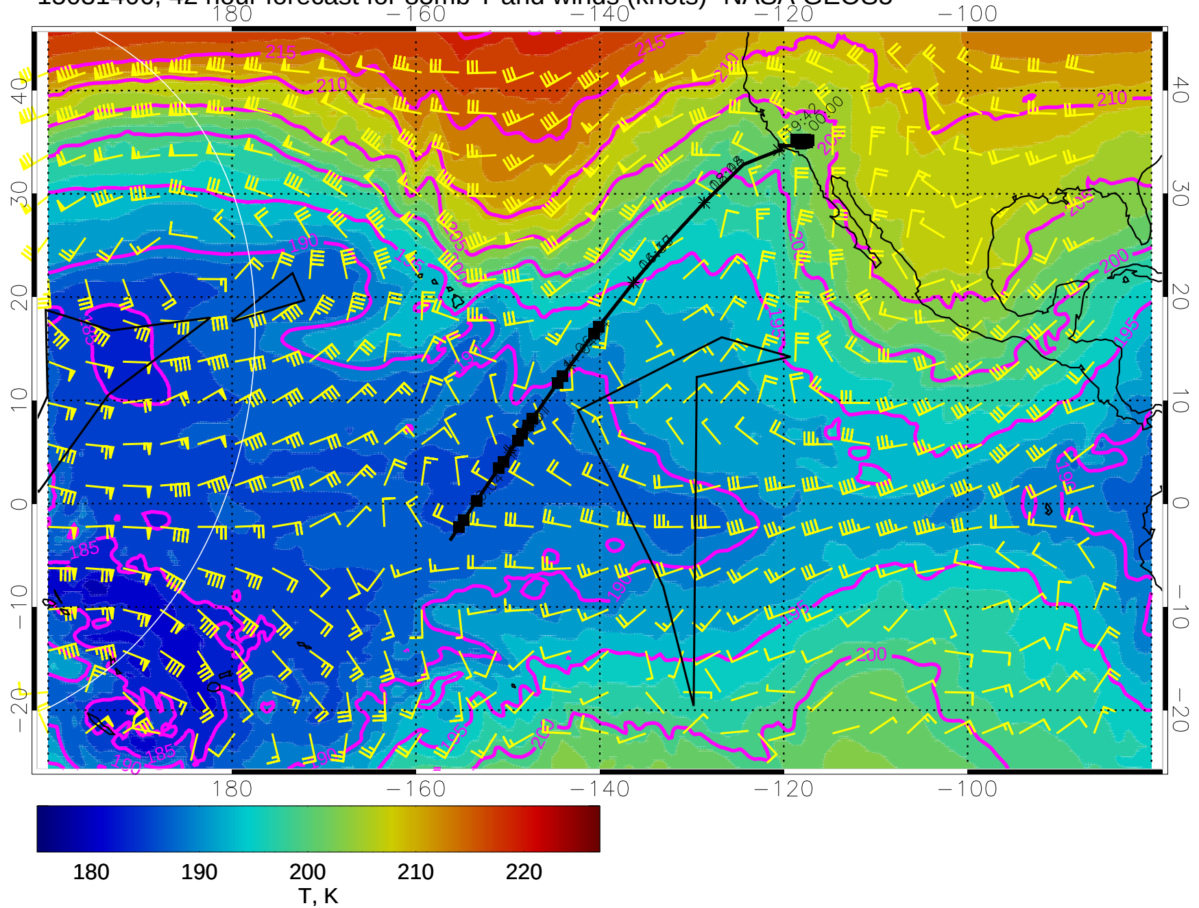
15031406, 42 hour forecast for 85mb T and winds (knots)- NASA GEOS5
