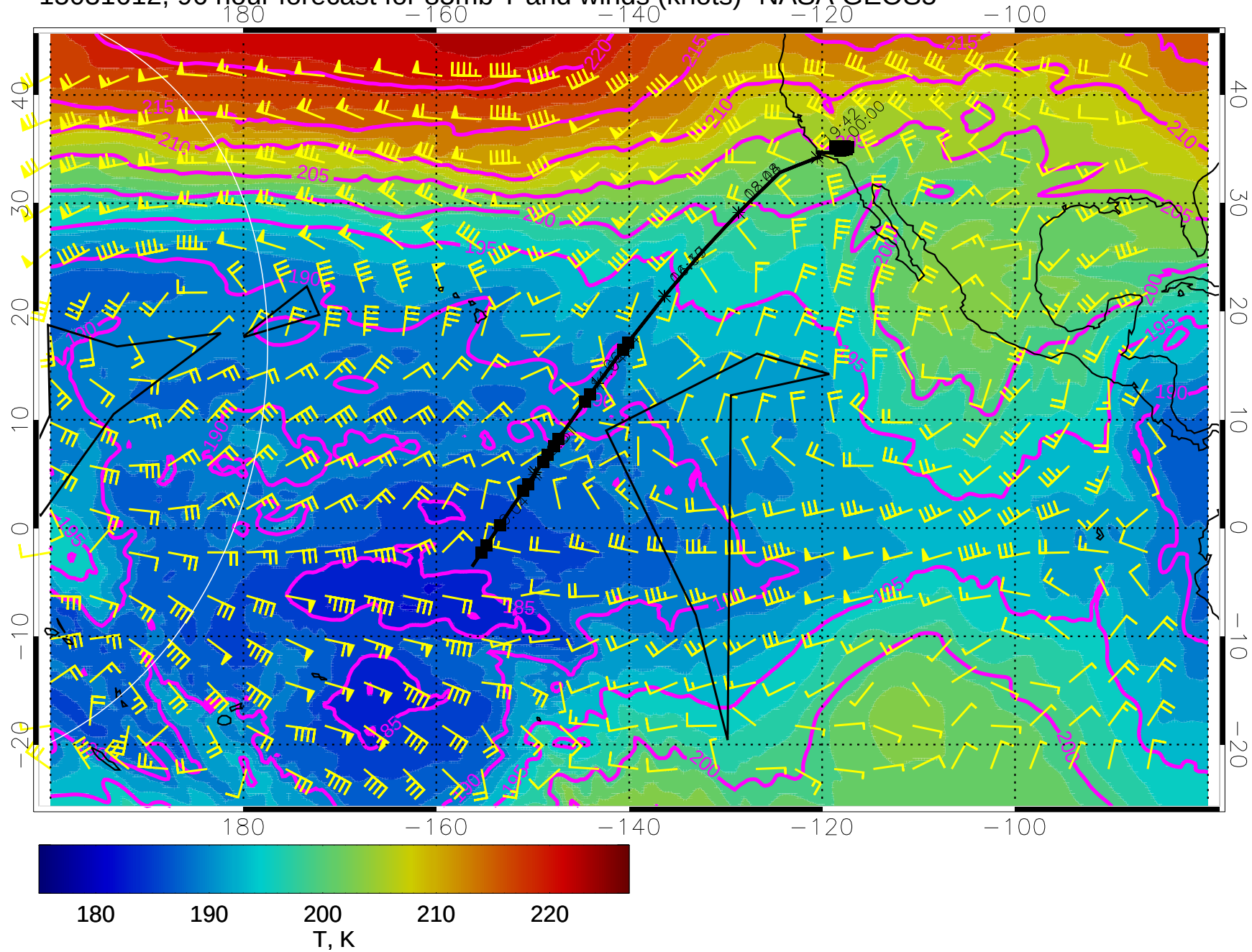
15031612, 96 hour forecast for 85mb T and winds (knots)- NASA GEOS5
