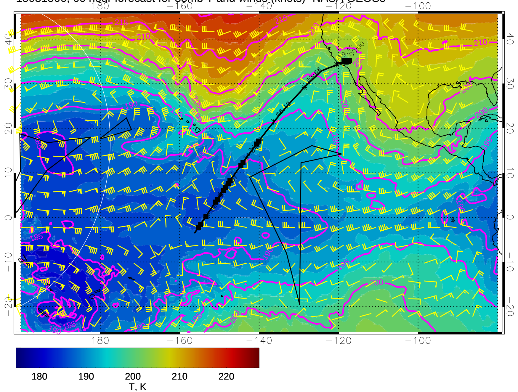
15031506, 66 hour forecast for 85mb T and winds (knots)- NASA GEOS5
