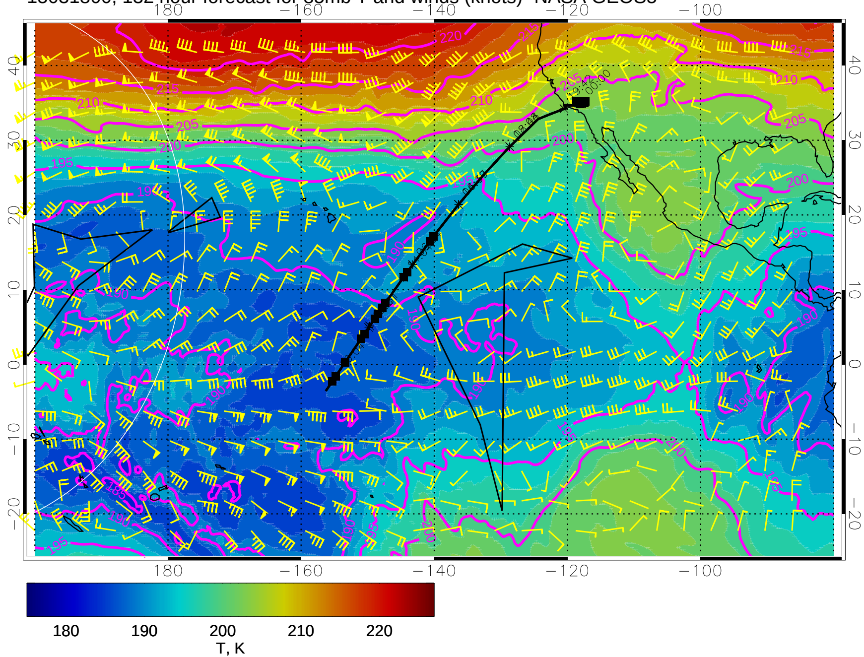
15031800, 132 hour forecast for 85mb T and winds (knots)- NASA GEOS5
