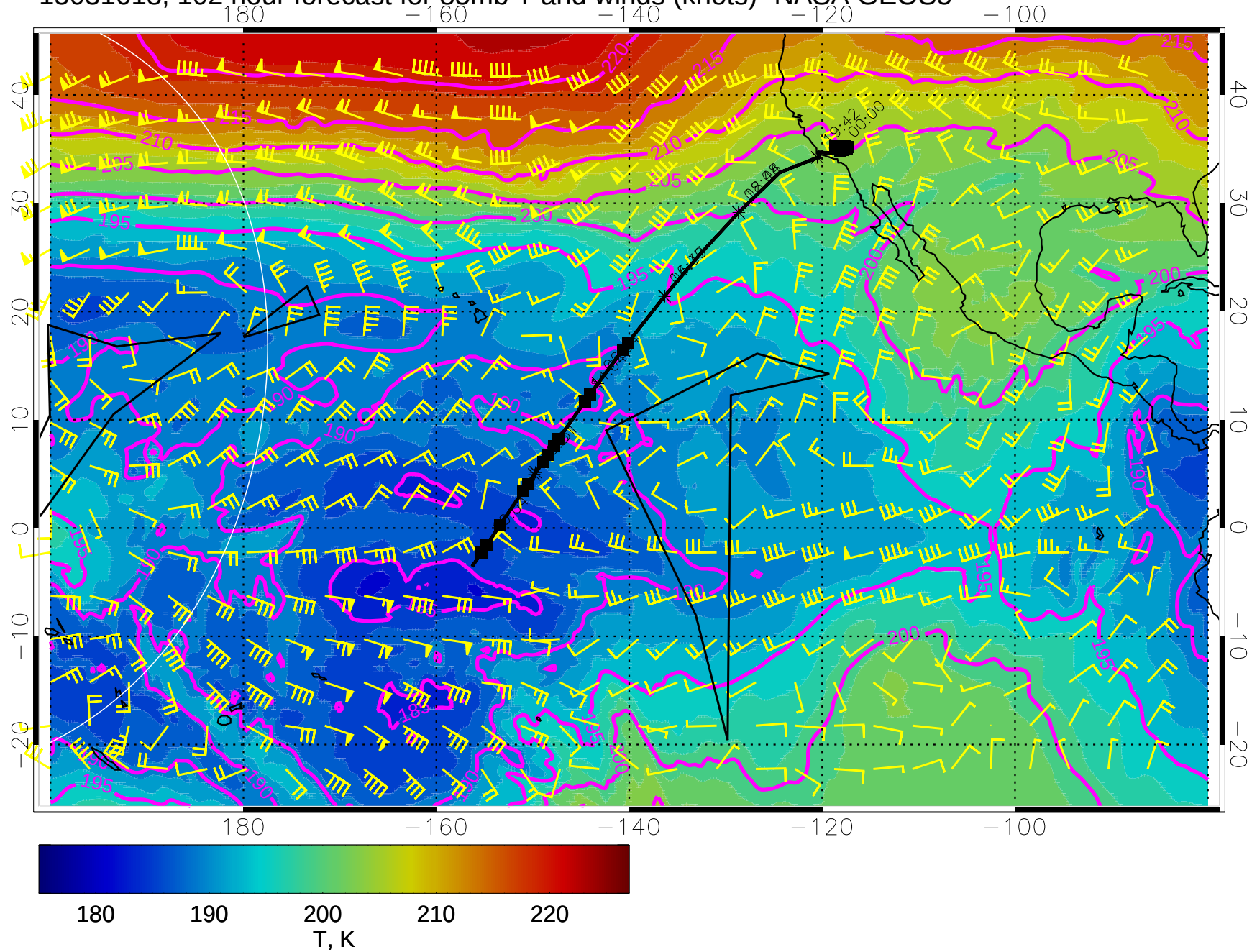
15031618, 102 hour forecast for 85mb T and winds (knots)- NASA GEOS5
