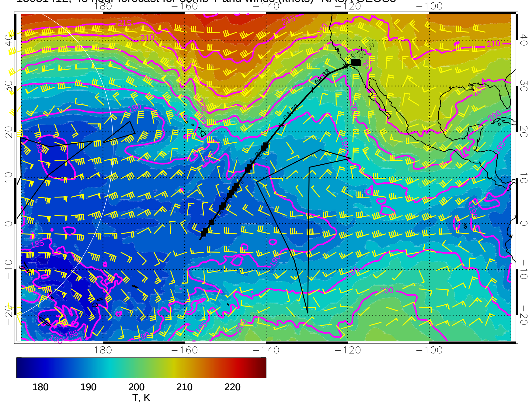
15031412, 48 hour forecast for 85mb T and winds (knots)- NASA GEOS5
