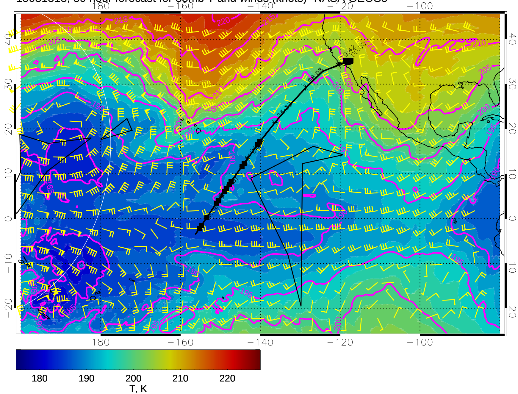
15031318, 30 hour forecast for 85mb T and winds (knots)- NASA GEOS5
