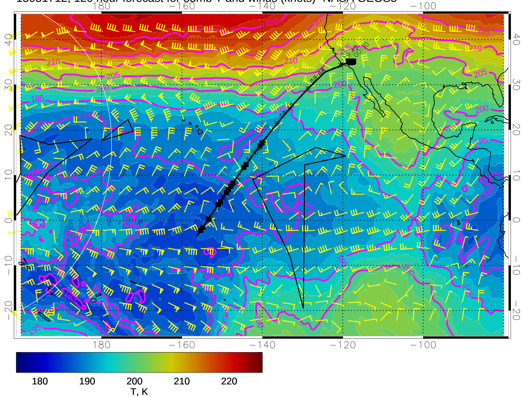
15031712, 120 hour forecast for 85mb T and winds (knots)- NASA GEOS5
