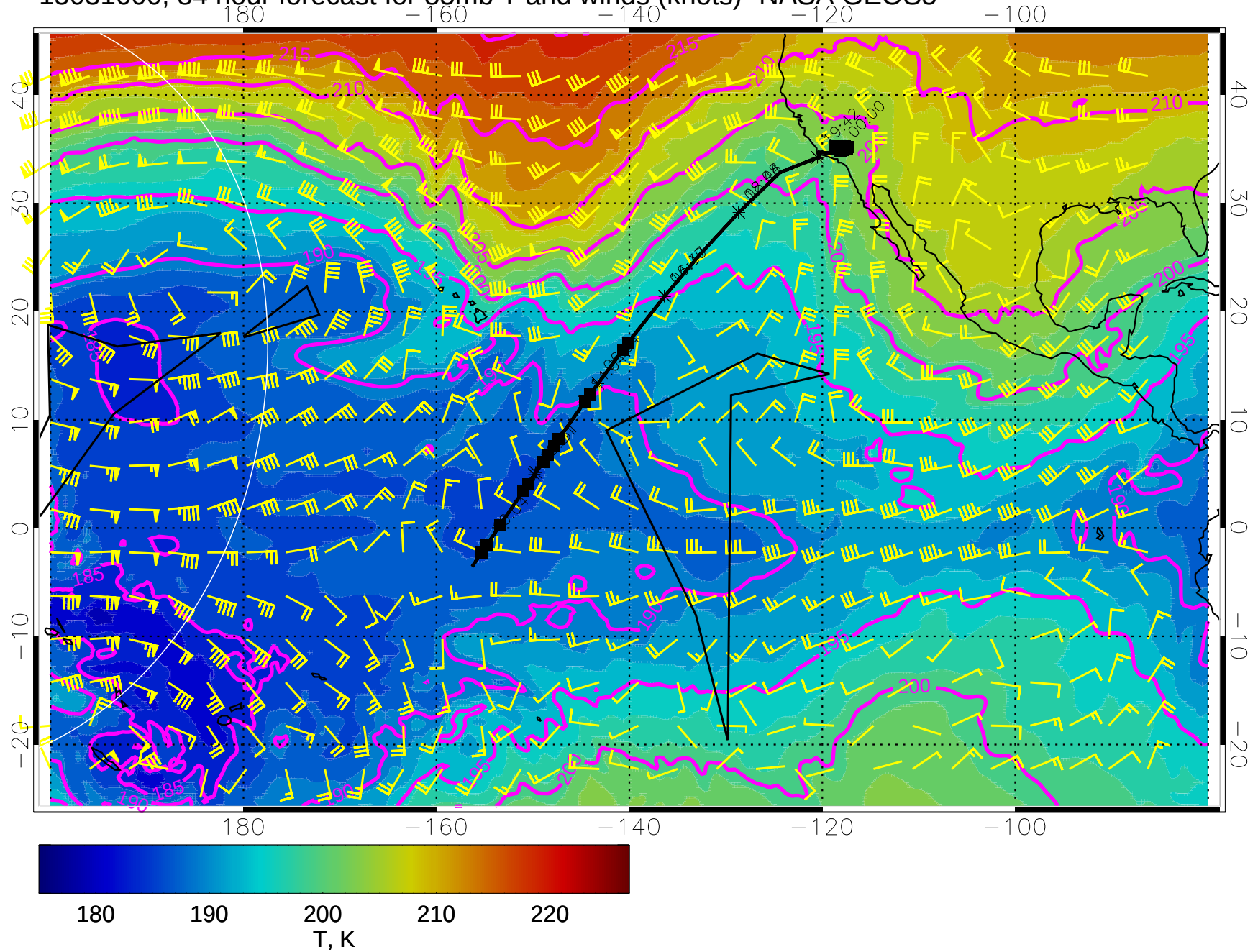
15031600, 84 hour forecast for 85mb T and winds (knots)- NASA GEOS5
