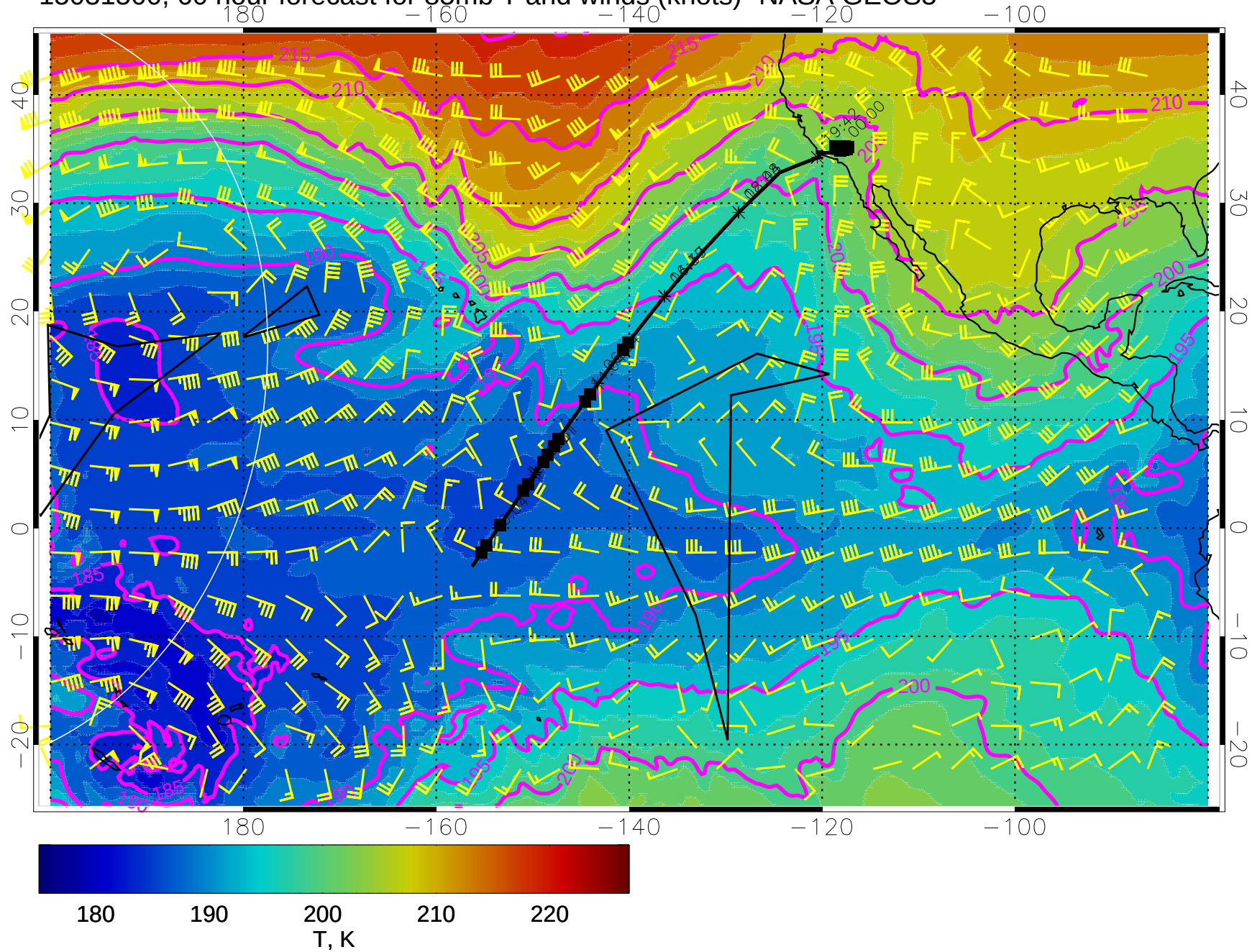
15031500, 60 hour forecast for 85mb T and winds (knots)- NASA GEOS5
