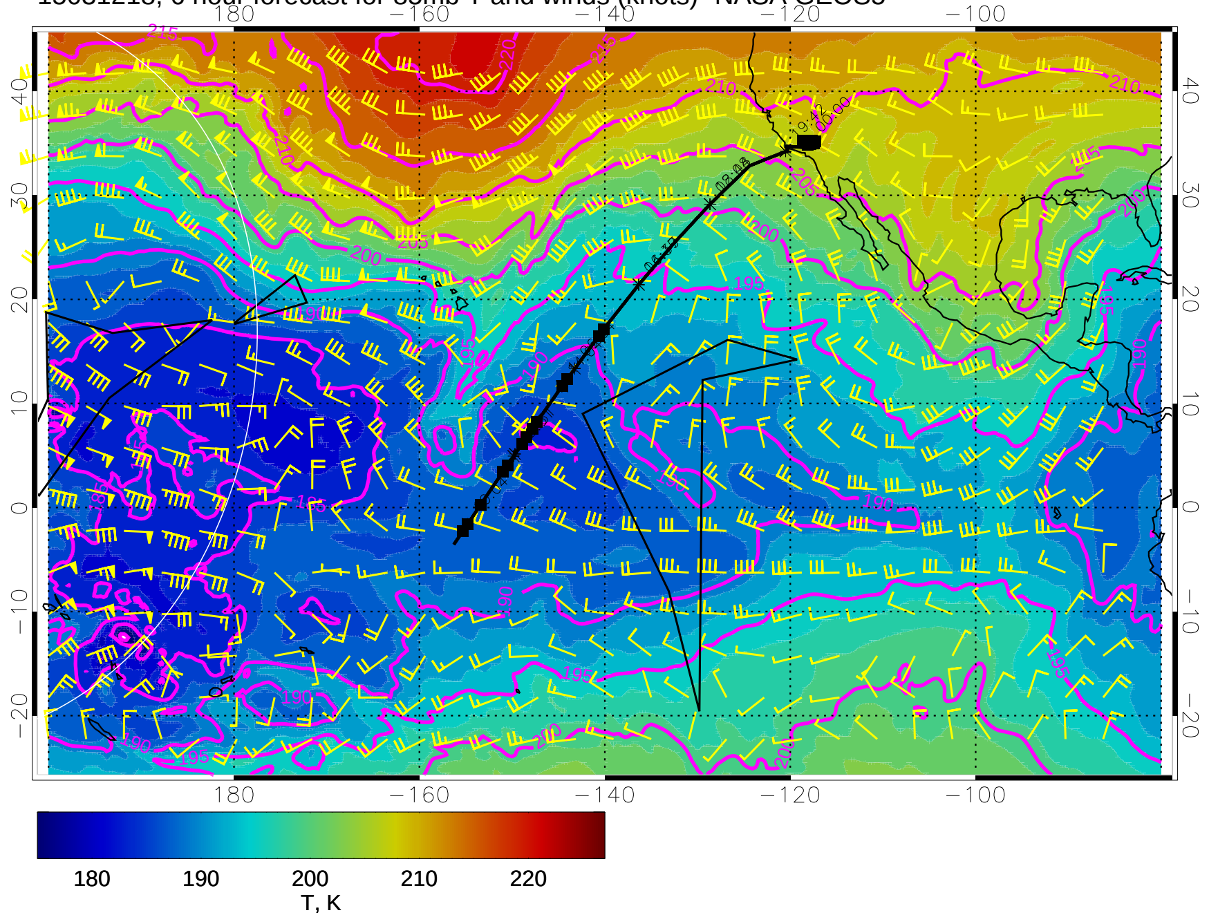
15031218, 6 hour forecast for 85mb T and winds (knots)- NASA GEOS5
