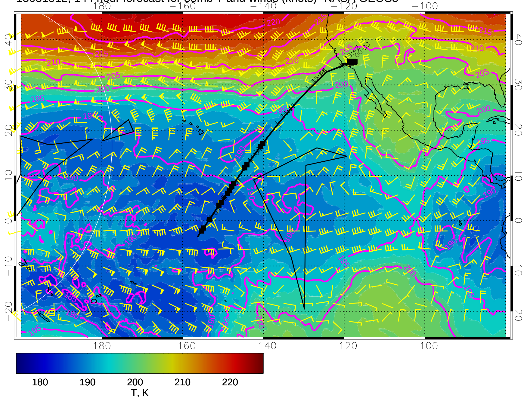
15031812, 144 hour forecast for 85mb T and winds (knots)- NASA GEOS5
