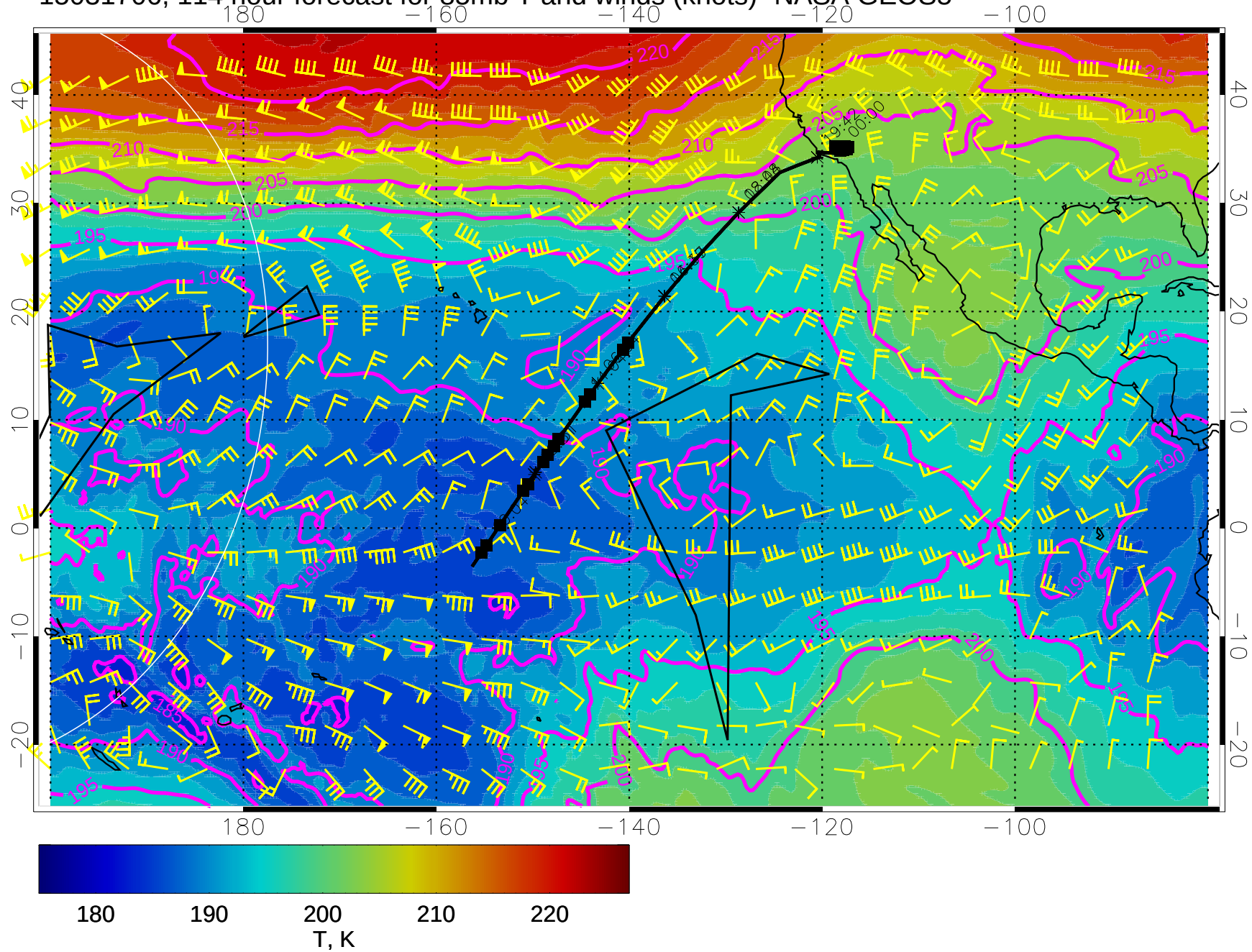
15031706, 114 hour forecast for 85mb T and winds (knots)- NASA GEOS5
