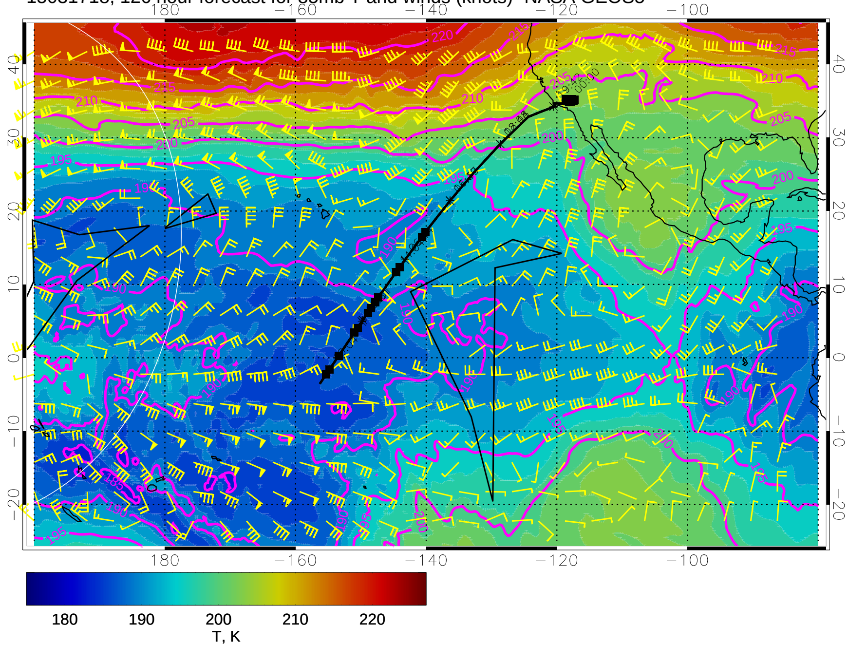
15031718, 126 hour forecast for 85mb T and winds (knots)- NASA GEOS5
