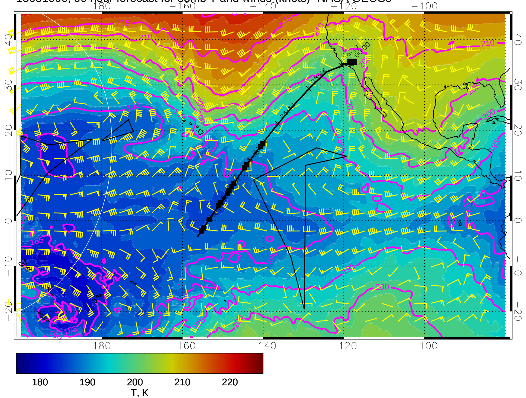
15031606, 90 hour forecast for 85mb T and winds (knots)- NASA GEOS5
