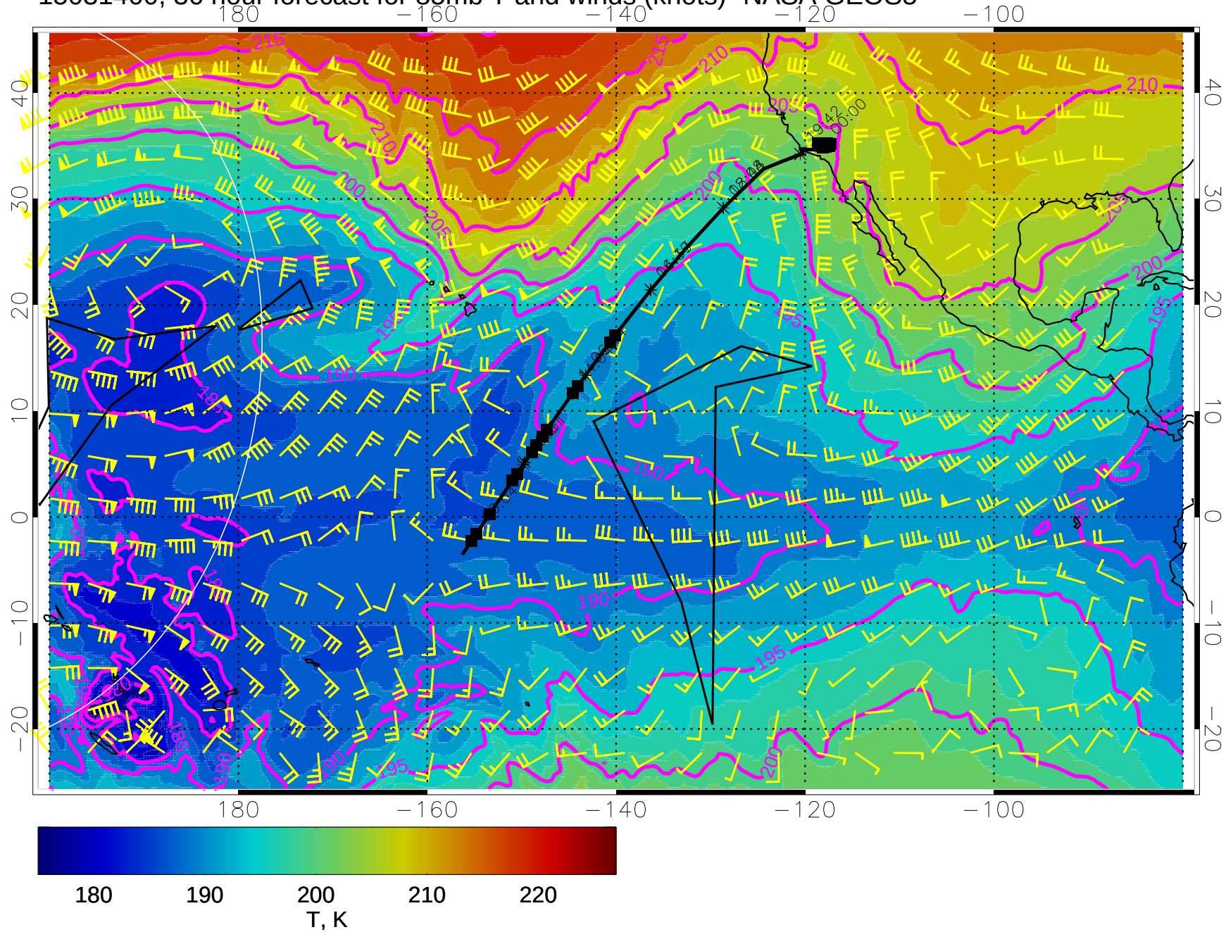
15031400, 36 hour forecast for 85mb T and winds (knots)- NASA GEOS5
