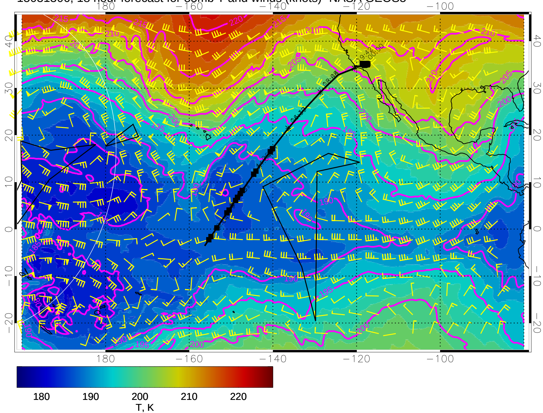
15031306, 18 hour forecast for 85mb T and winds (knots)- NASA GEOS5
