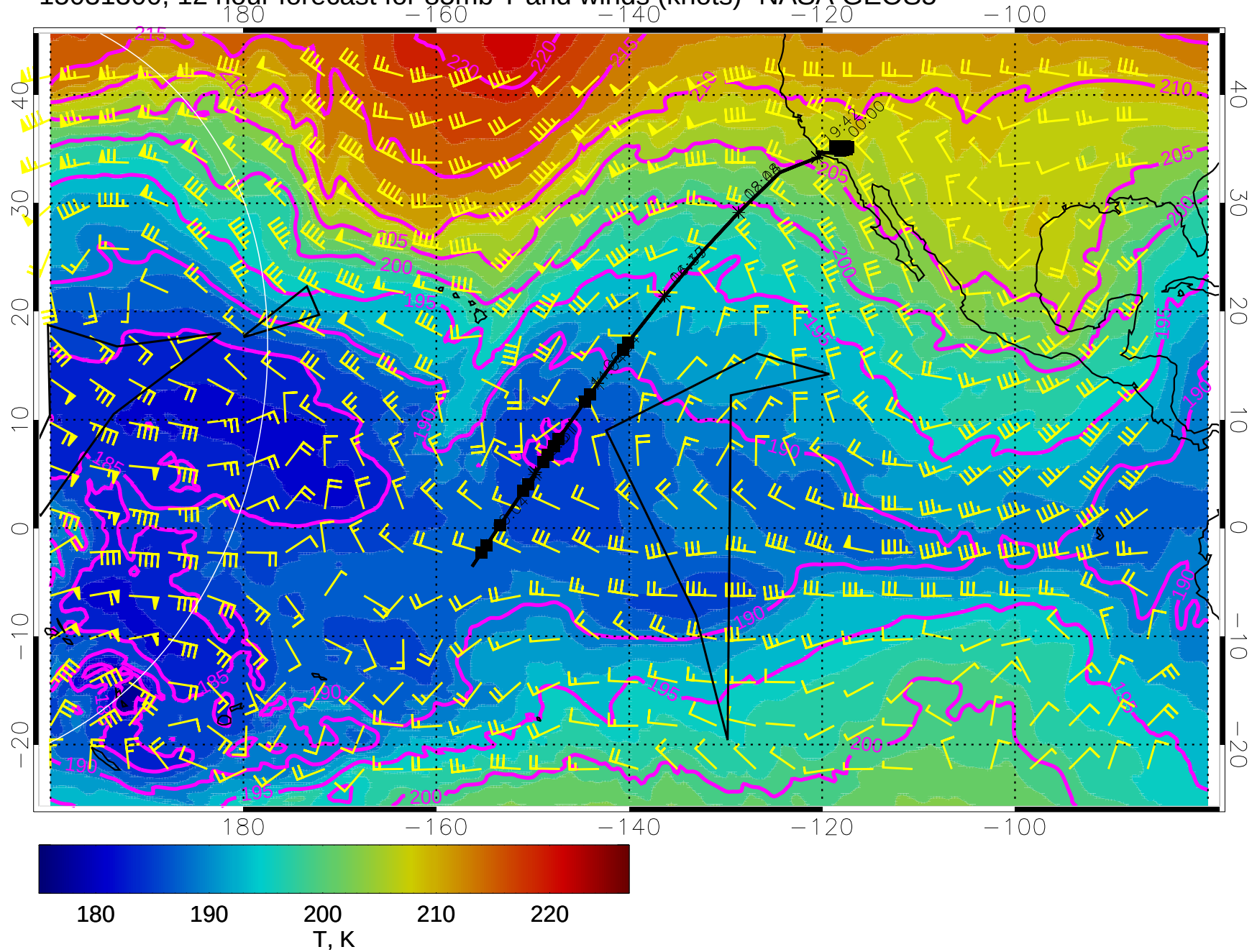
15031300, 12 hour forecast for 85mb T and winds (knots)- NASA GEOS5
