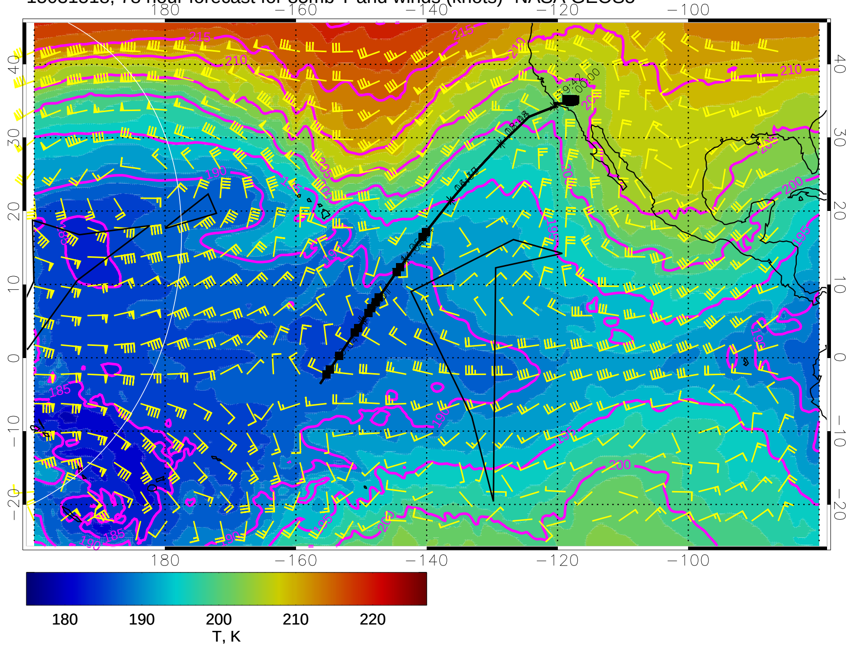
15031518, 78 hour forecast for 85mb T and winds (knots)- NASA GEOS5
