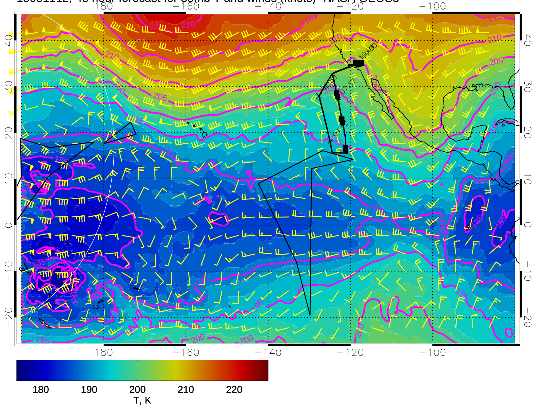
15031112, 48 hour forecast for 85mb T and winds (knots)- NASA GEOS5
