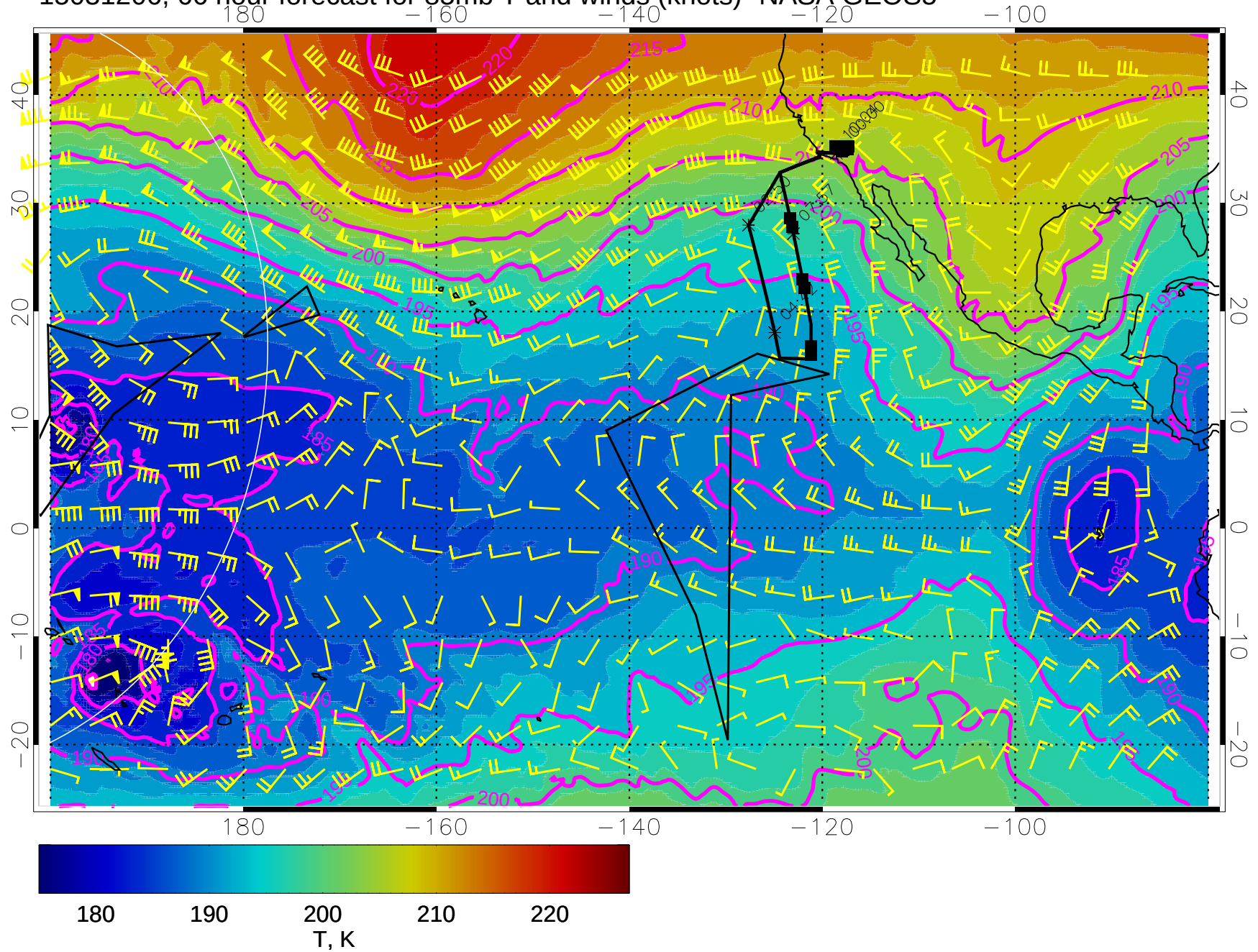
15031206, 66 hour forecast for 85mb T and winds (knots)- NASA GEOS5
