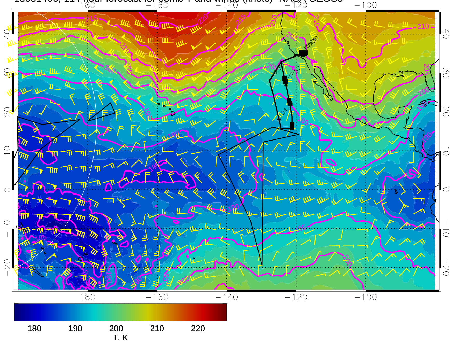
15031406, 114 hour forecast for 85mb T and winds (knots)- NASA GEOS5
