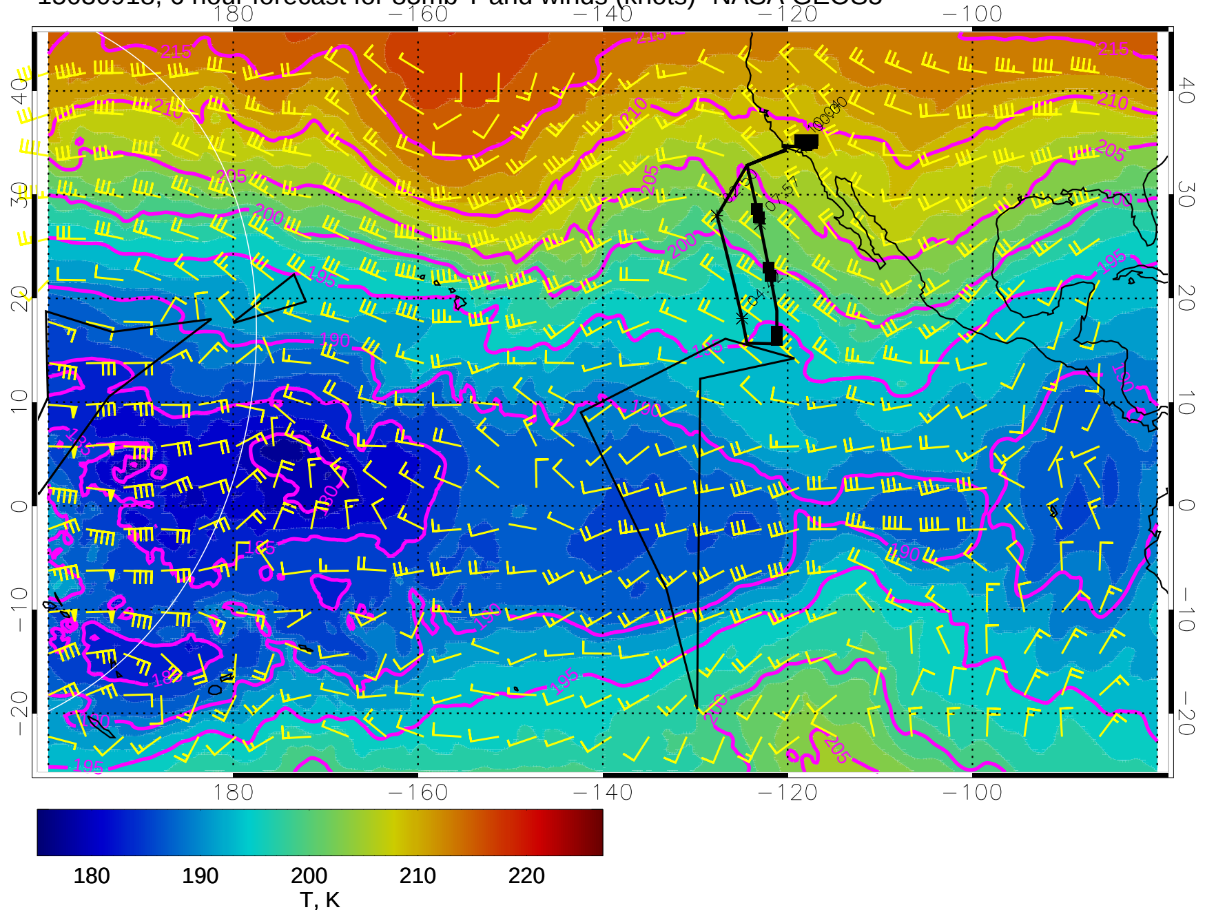
15030918, 6 hour forecast for 85mb T and winds (knots)- NASA GEOS5
