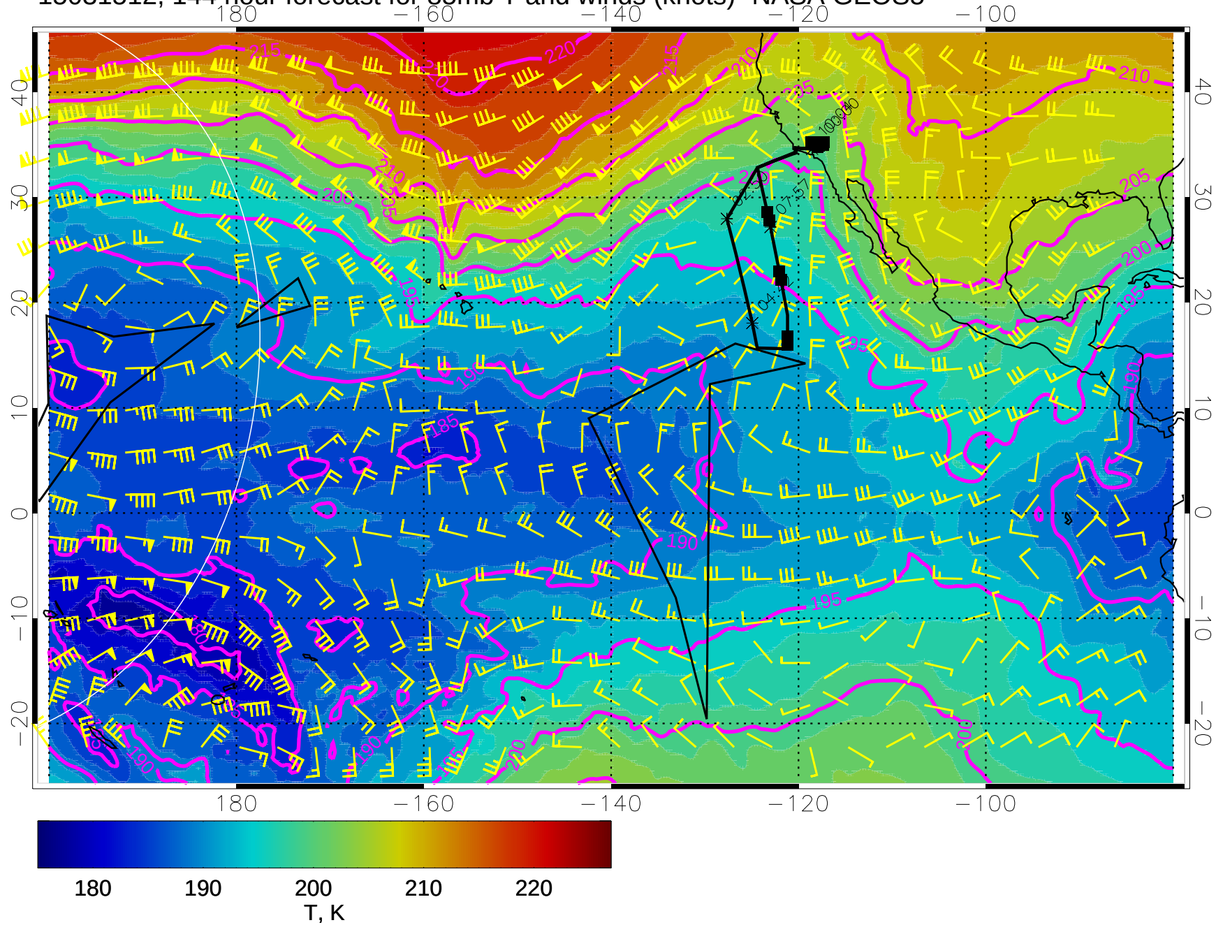
15031512, 144 hour forecast for 85mb T and winds (knots)- NASA GEOS5
