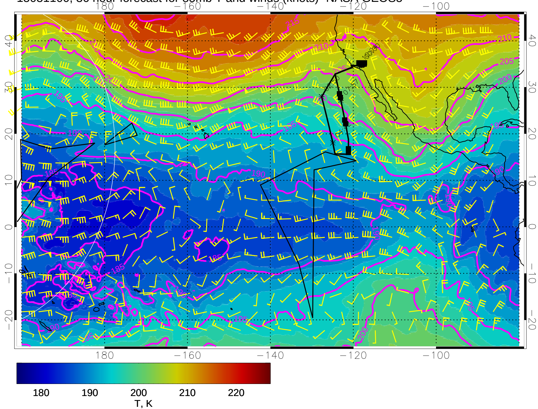
15031100, 36 hour forecast for 85mb T and winds (knots)- NASA GEOS5
