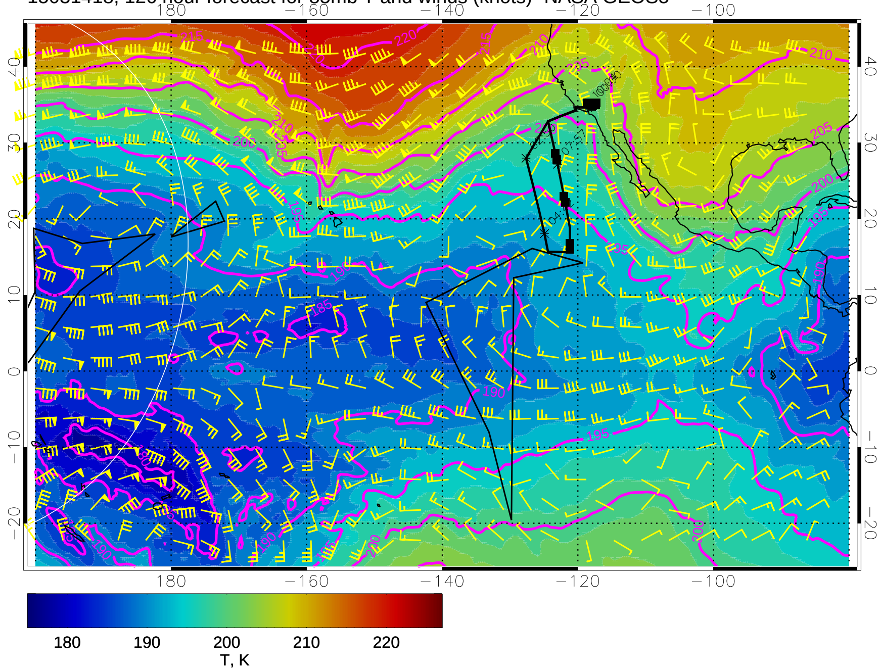
15031418, 126 hour forecast for 85mb T and winds (knots)- NASA GEOS5
