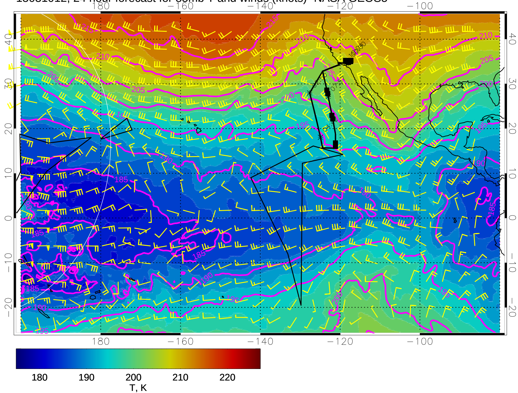
15031012, 24 hour forecast for 85mb T and winds (knots)- NASA GEOS5
