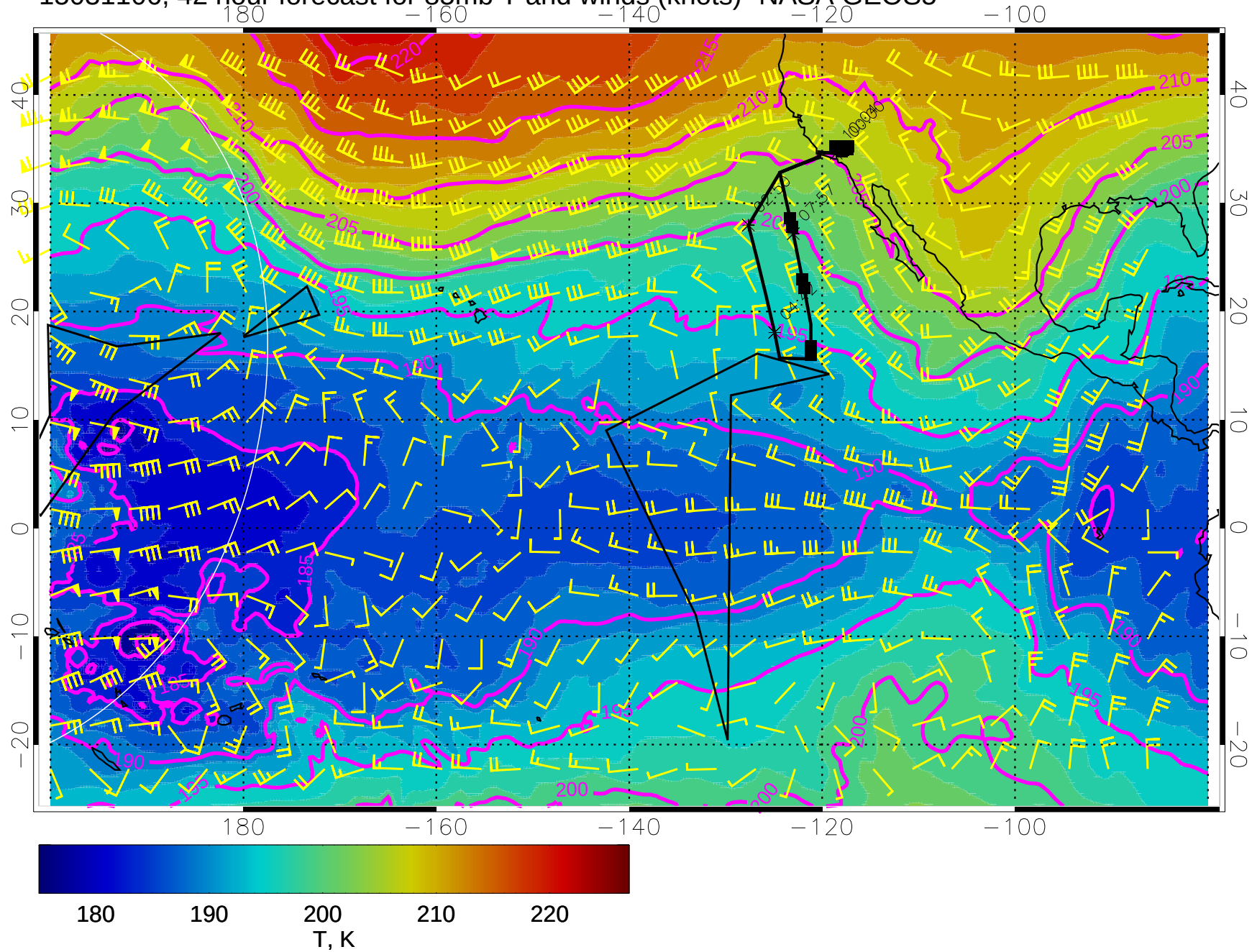
15031106, 42 hour forecast for 85mb T and winds (knots)- NASA GEOS5
