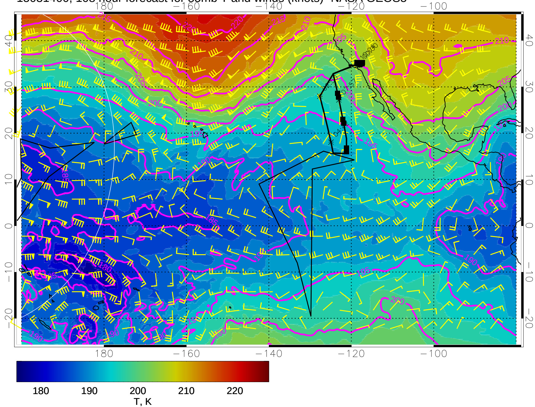
15031400, 108 hour forecast for 85mb T and winds (knots)- NASA GEOS5
