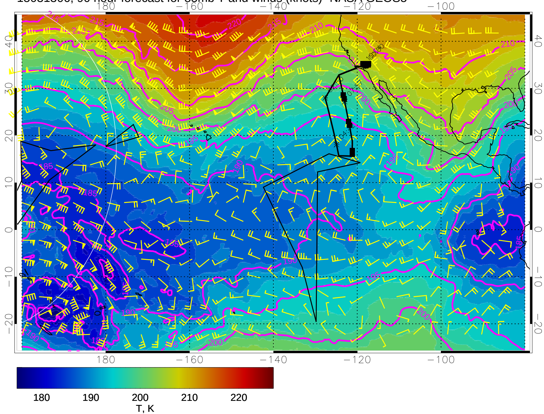
15031306, 90 hour forecast for 85mb T and winds (knots)- NASA GEOS5
