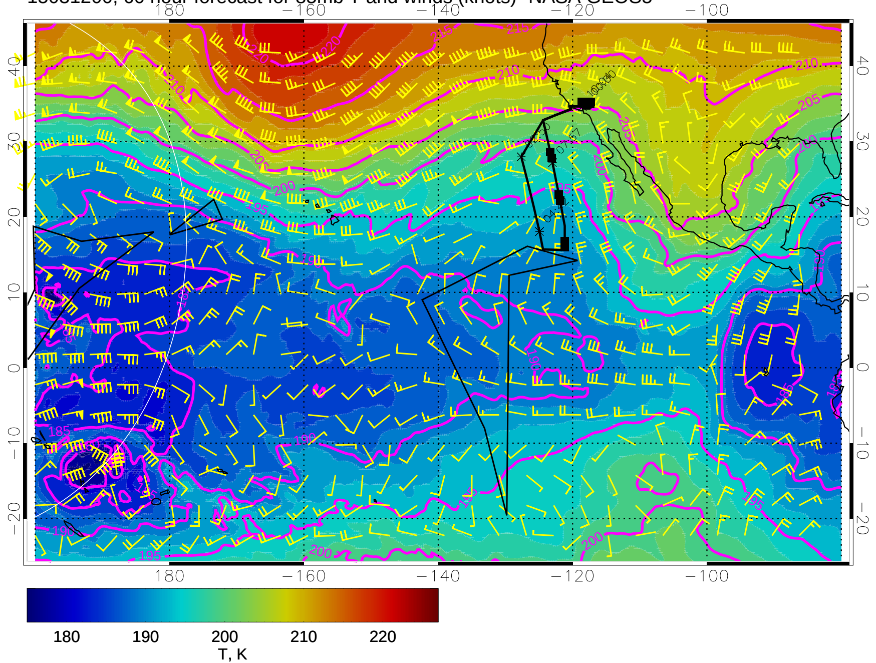
15031200, 60 hour forecast for 85mb T and winds (knots)- NASA GEOS5
