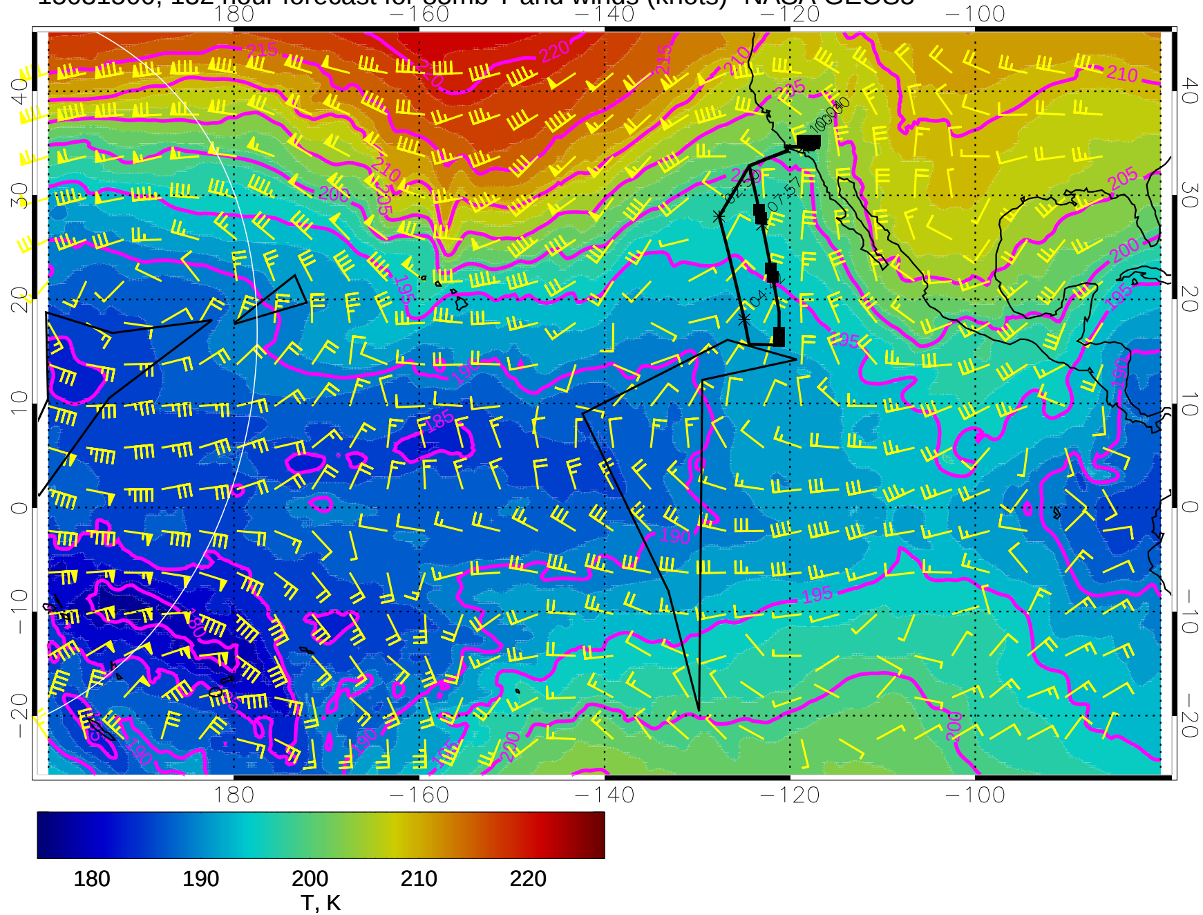
15031500, 132 hour forecast for 85mb T and winds (knots)- NASA GEOS5
