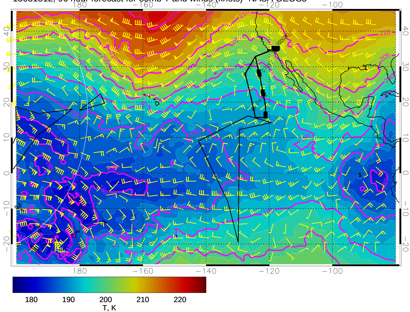
15031312, 96 hour forecast for 85mb T and winds (knots)- NASA GEOS5
