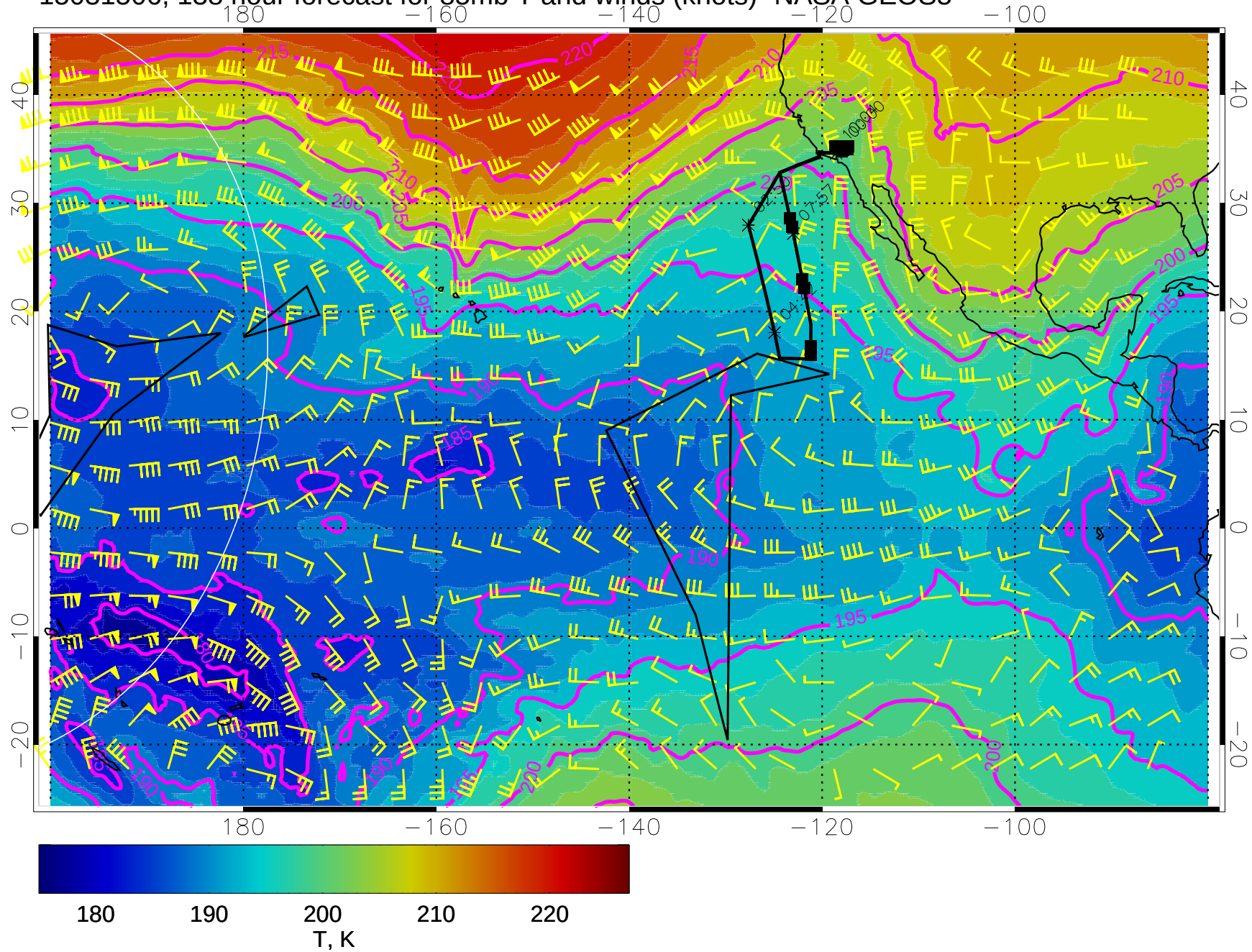
15031506, 138 hour forecast for 85mb T and winds (knots)- NASA GEOS5
