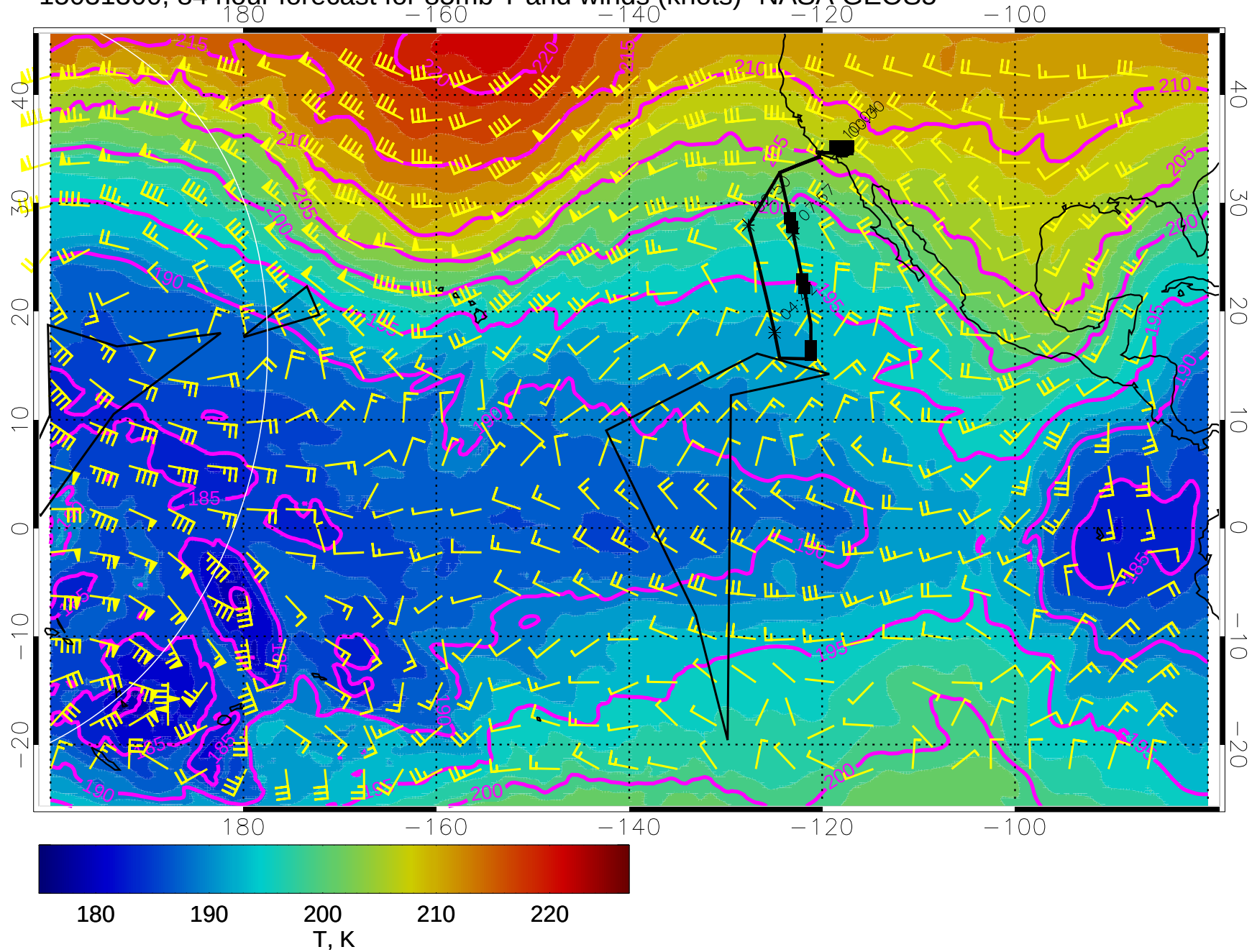
15031300, 84 hour forecast for 85mb T and winds (knots)- NASA GEOS5
