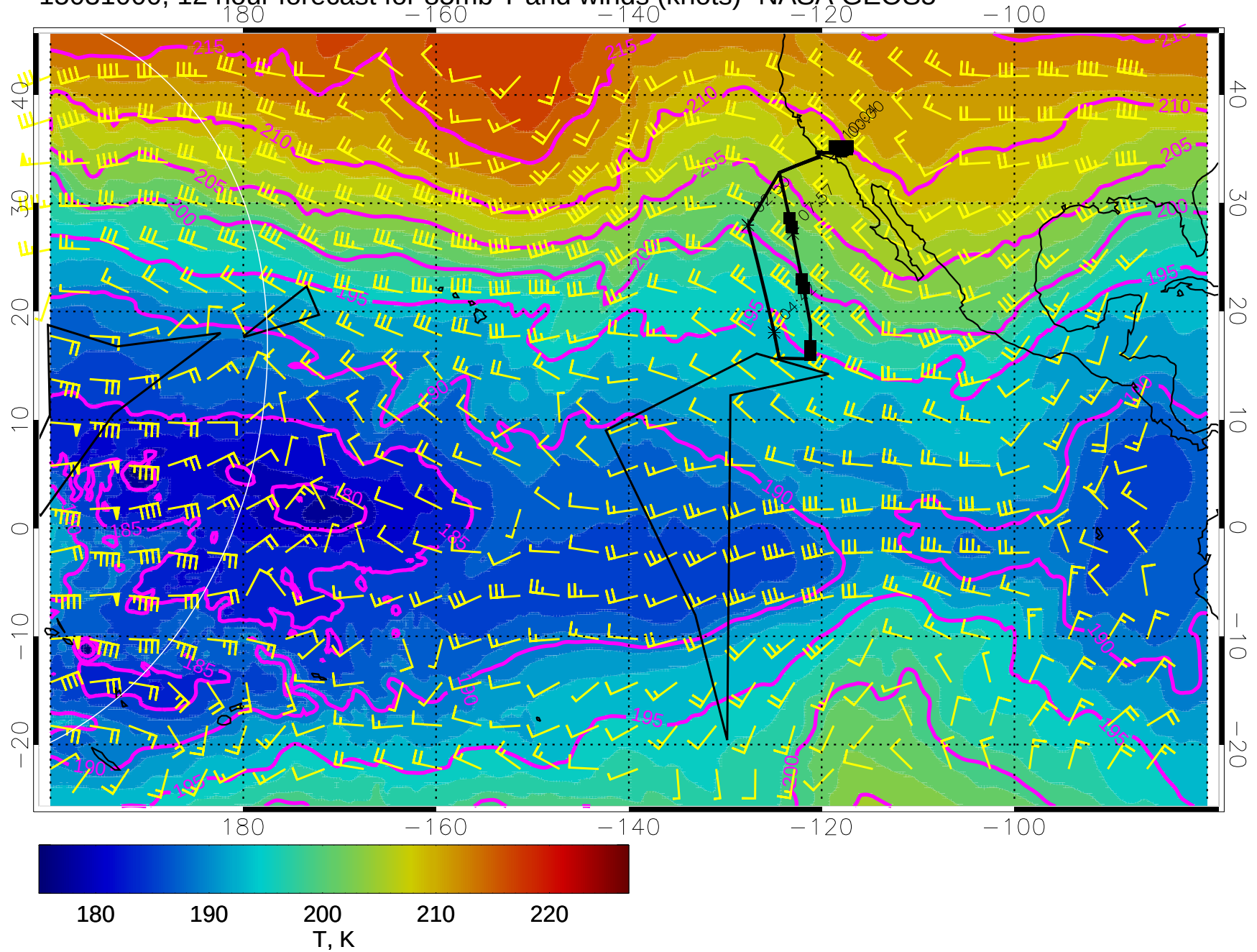
15031000, 12 hour forecast for 85mb T and winds (knots)- NASA GEOS5
