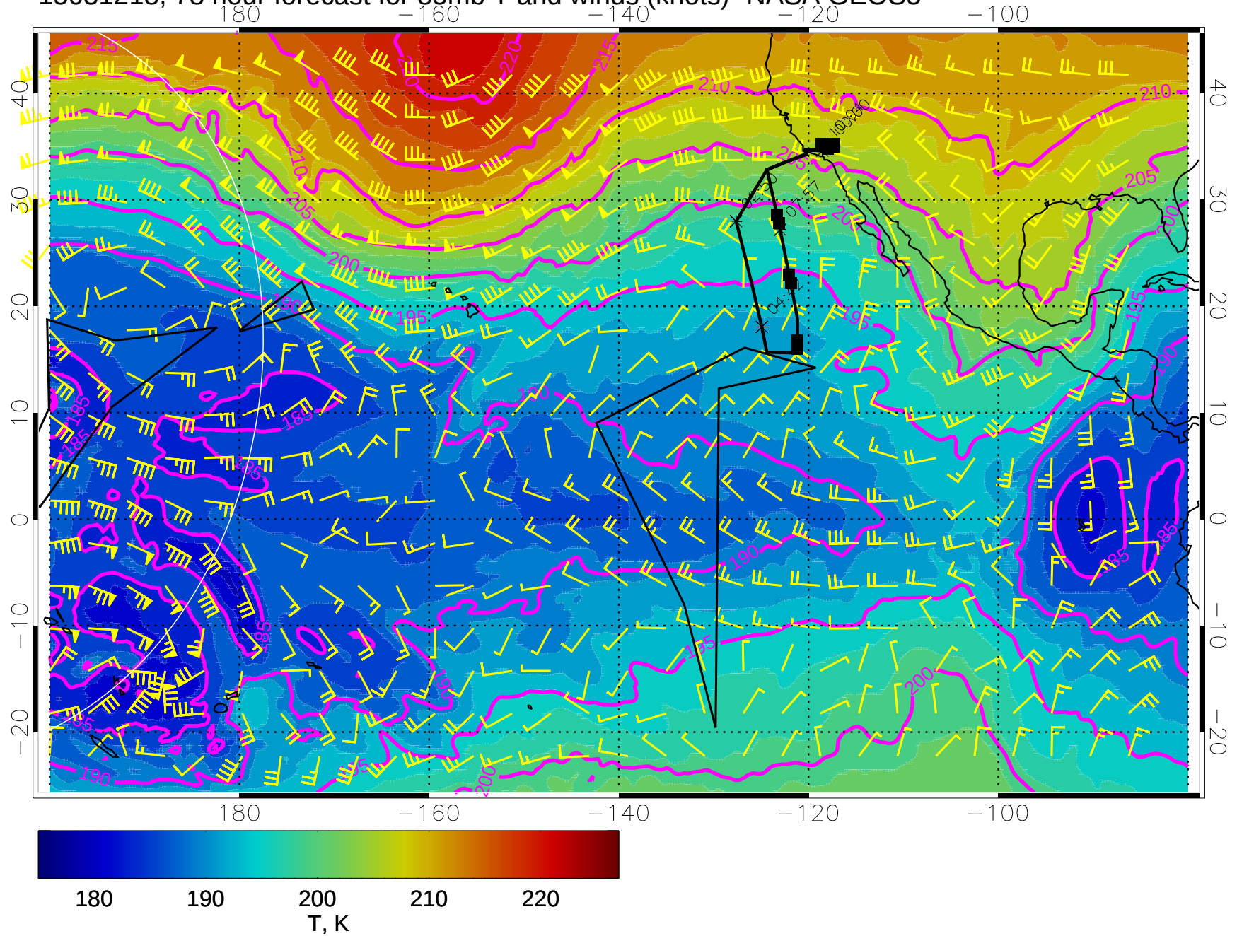
15031218, 78 hour forecast for 85mb T and winds (knots)- NASA GEOS5
