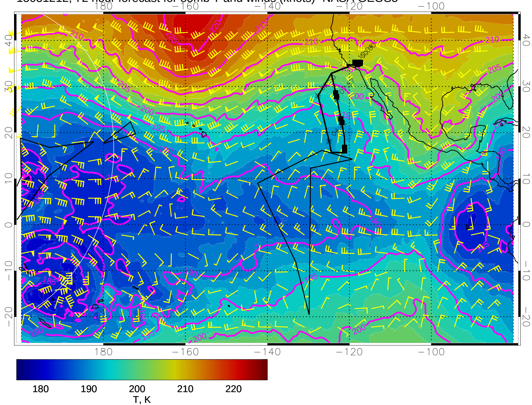
15031212, 72 hour forecast for 85mb T and winds (knots)- NASA GEOS5
