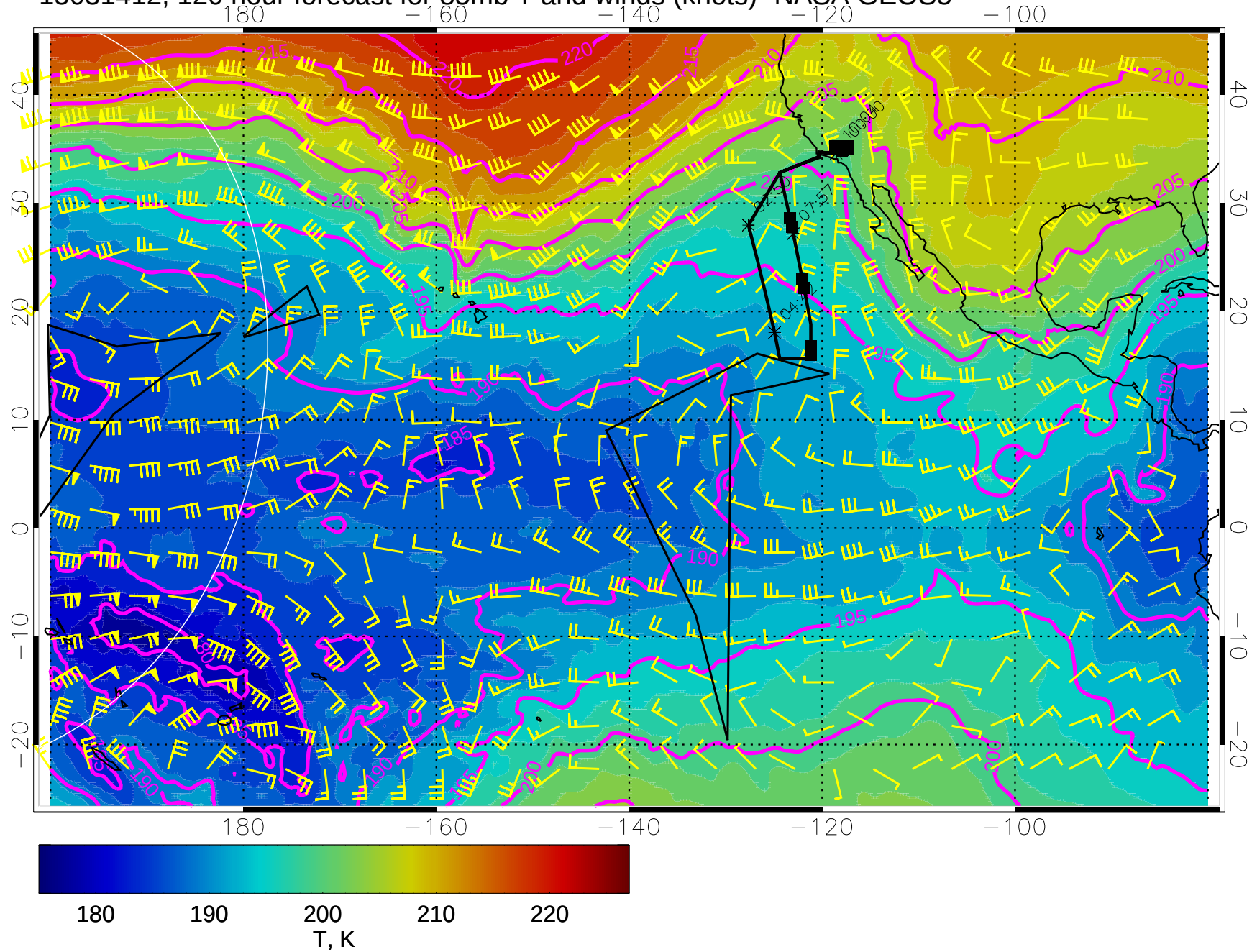
15031412, 120 hour forecast for 85mb T and winds (knots)- NASA GEOS5
