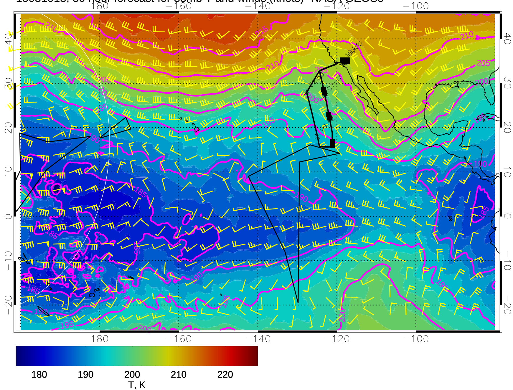
15031018, 30 hour forecast for 85mb T and winds (knots)- NASA GEOS5
