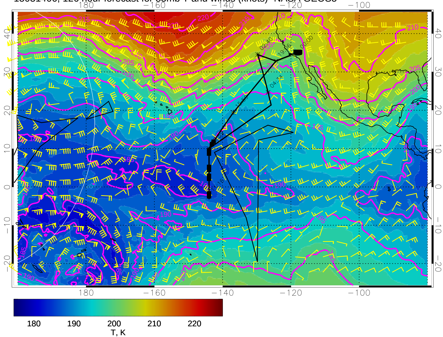
15031406, 126 hour forecast for 85mb T and winds (knots)- NASA GEOS5
