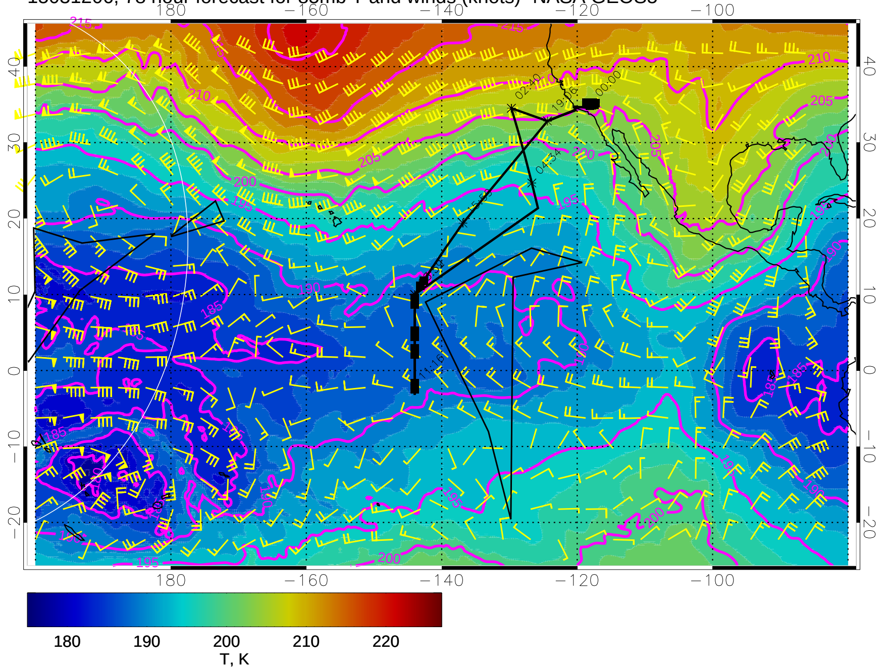
15031206, 78 hour forecast for 85mb T and winds (knots)- NASA GEOS5
