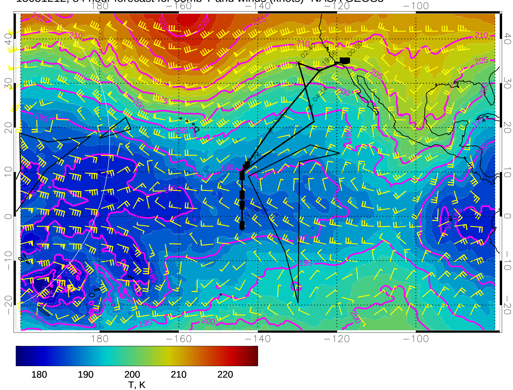
15031212, 84 hour forecast for 85mb T and winds (knots)- NASA GEOS5
