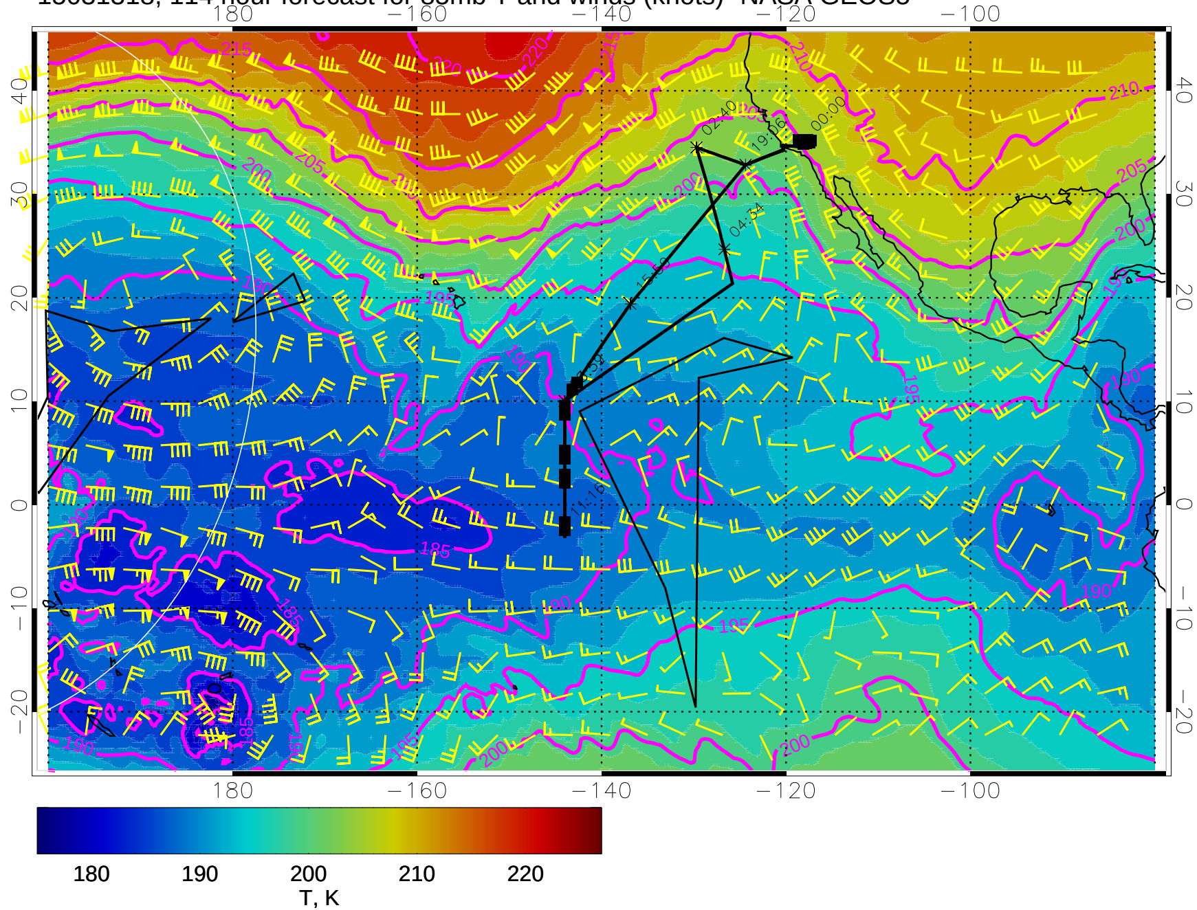
15031318, 114 hour forecast for 85mb T and winds (knots)- NASA GEOS5
