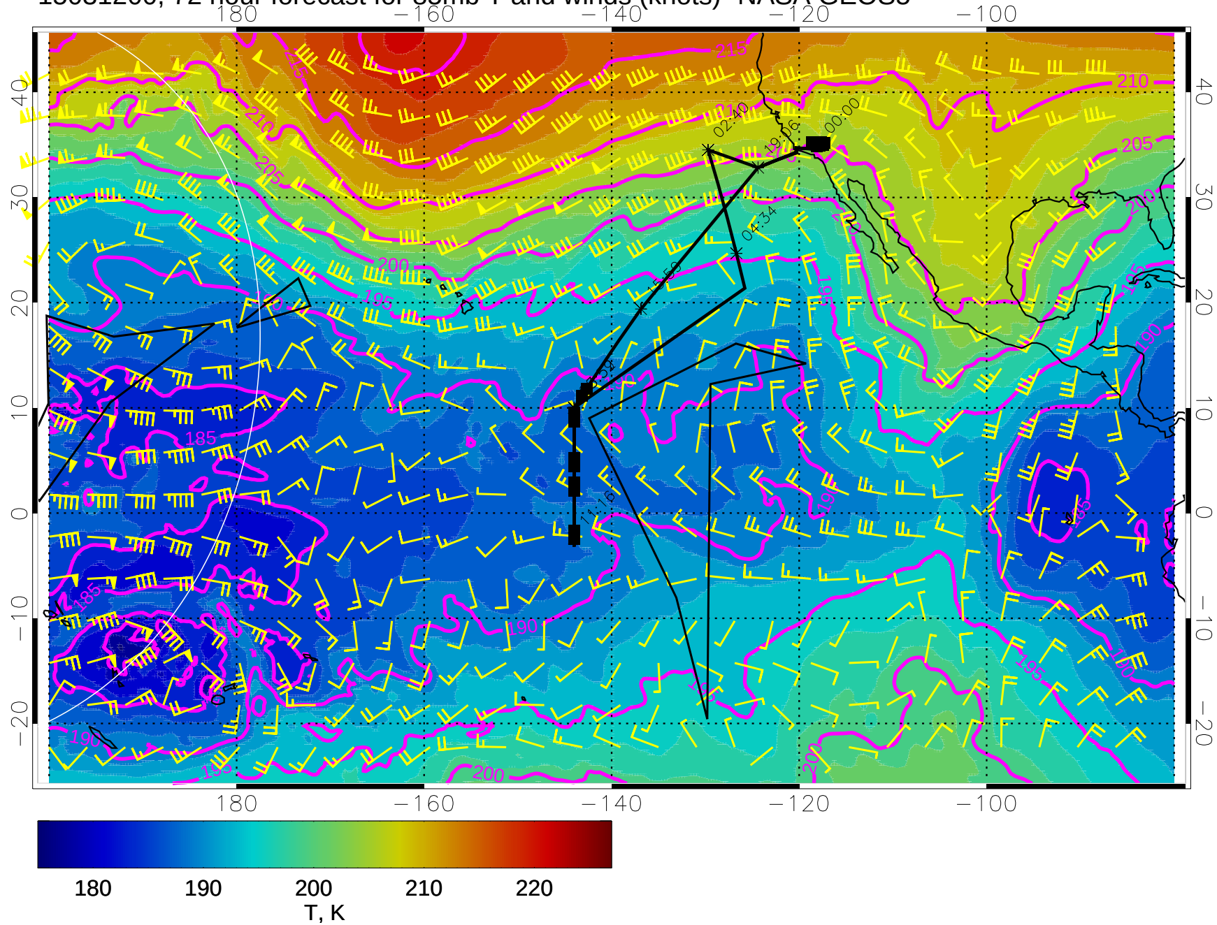
15031200, 72 hour forecast for 85mb T and winds (knots)- NASA GEOS5
