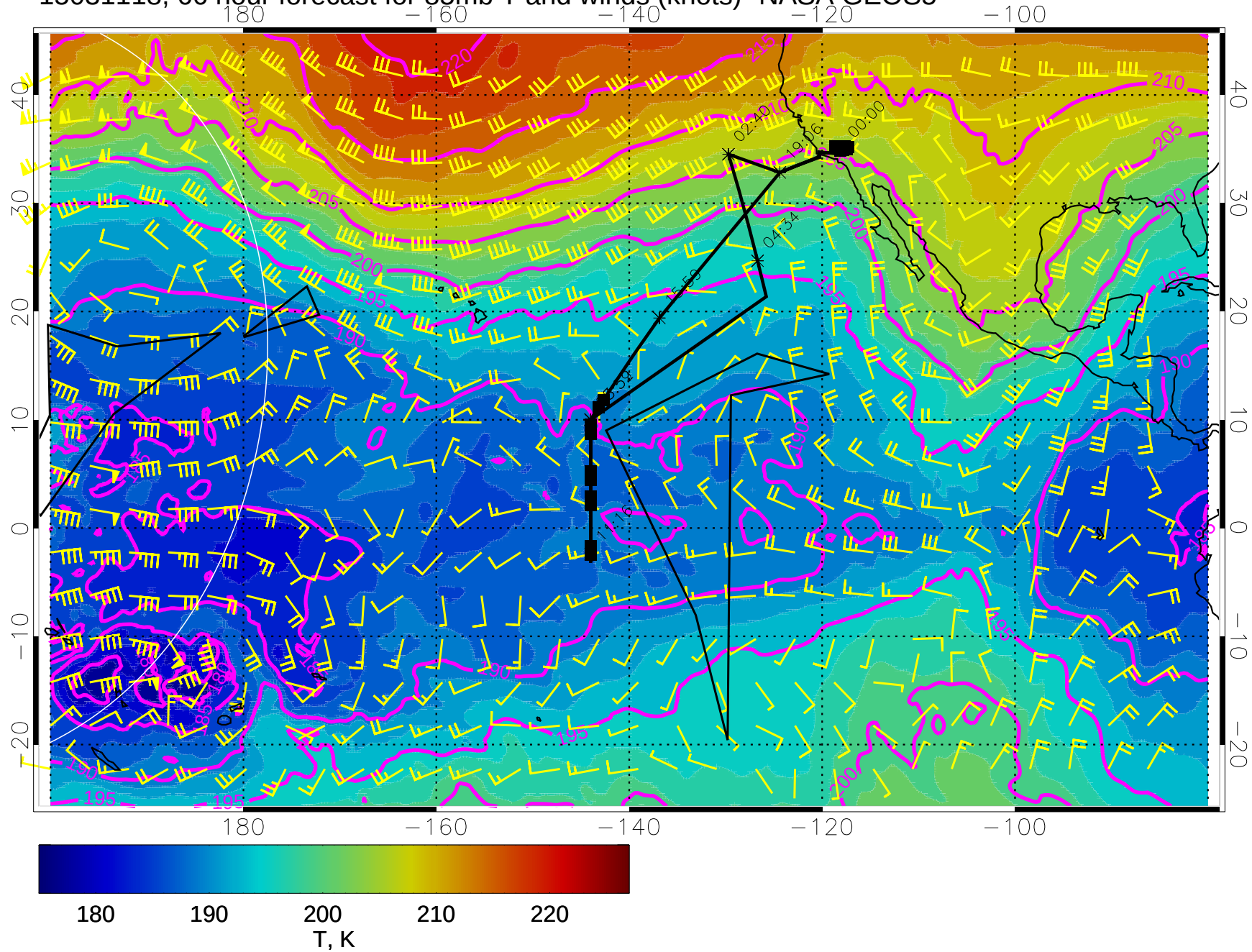
15031118, 66 hour forecast for 85mb T and winds (knots)- NASA GEOS5
