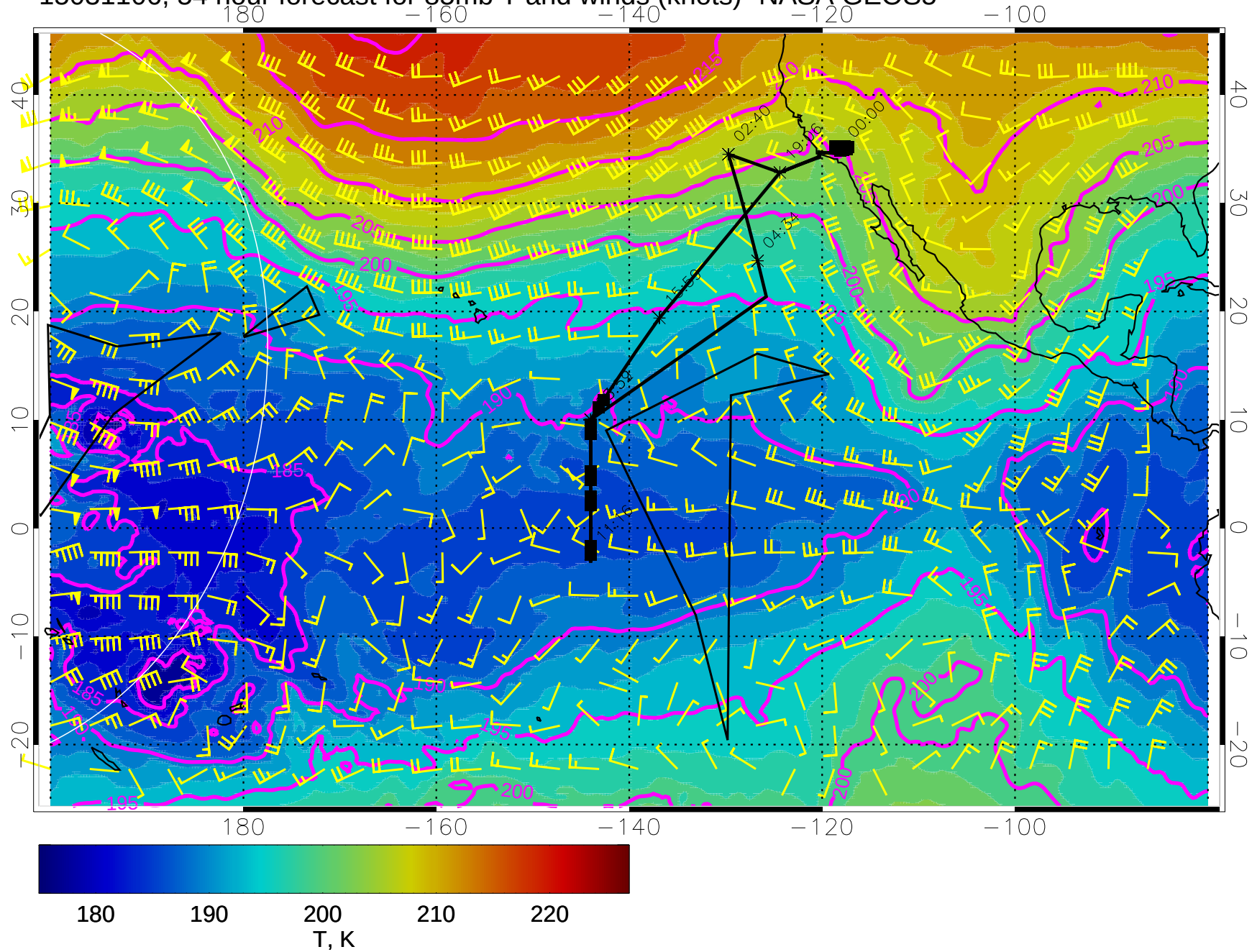
15031106, 54 hour forecast for 85mb T and winds (knots)- NASA GEOS5
