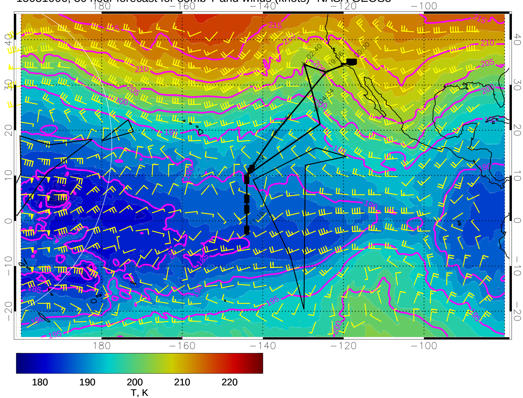
15031006, 30 hour forecast for 85mb T and winds (knots)- NASA GEOS5
