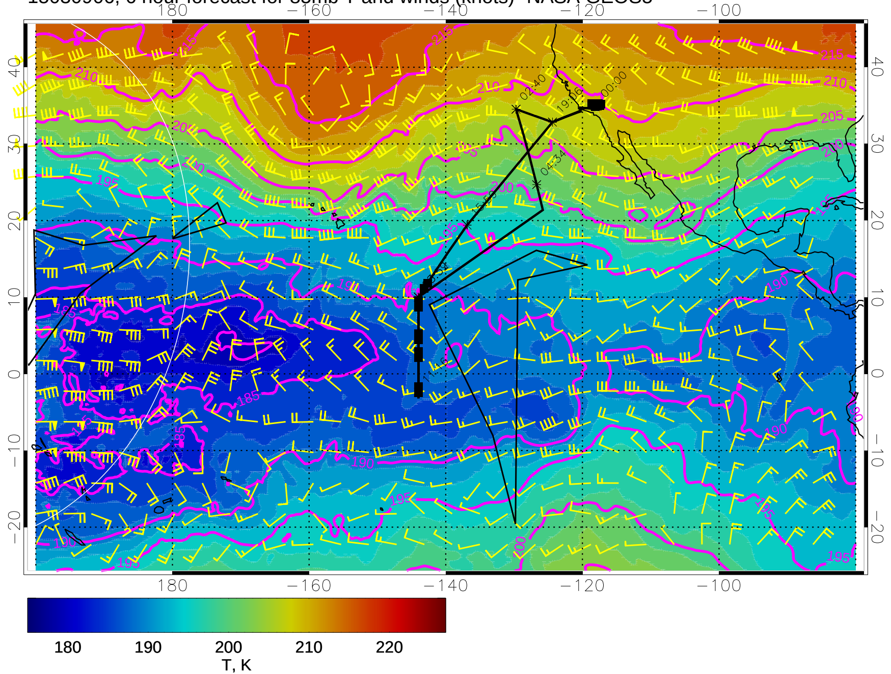
15030906, 6 hour forecast for 85mb T and winds (knots)- NASA GEOS5
