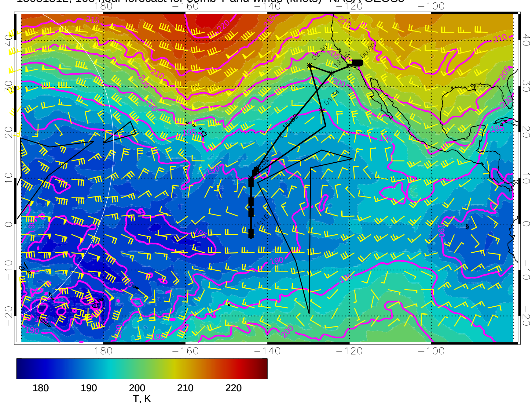
15031312, 108 hour forecast for 85mb T and winds (knots)- NASA GEOS5
