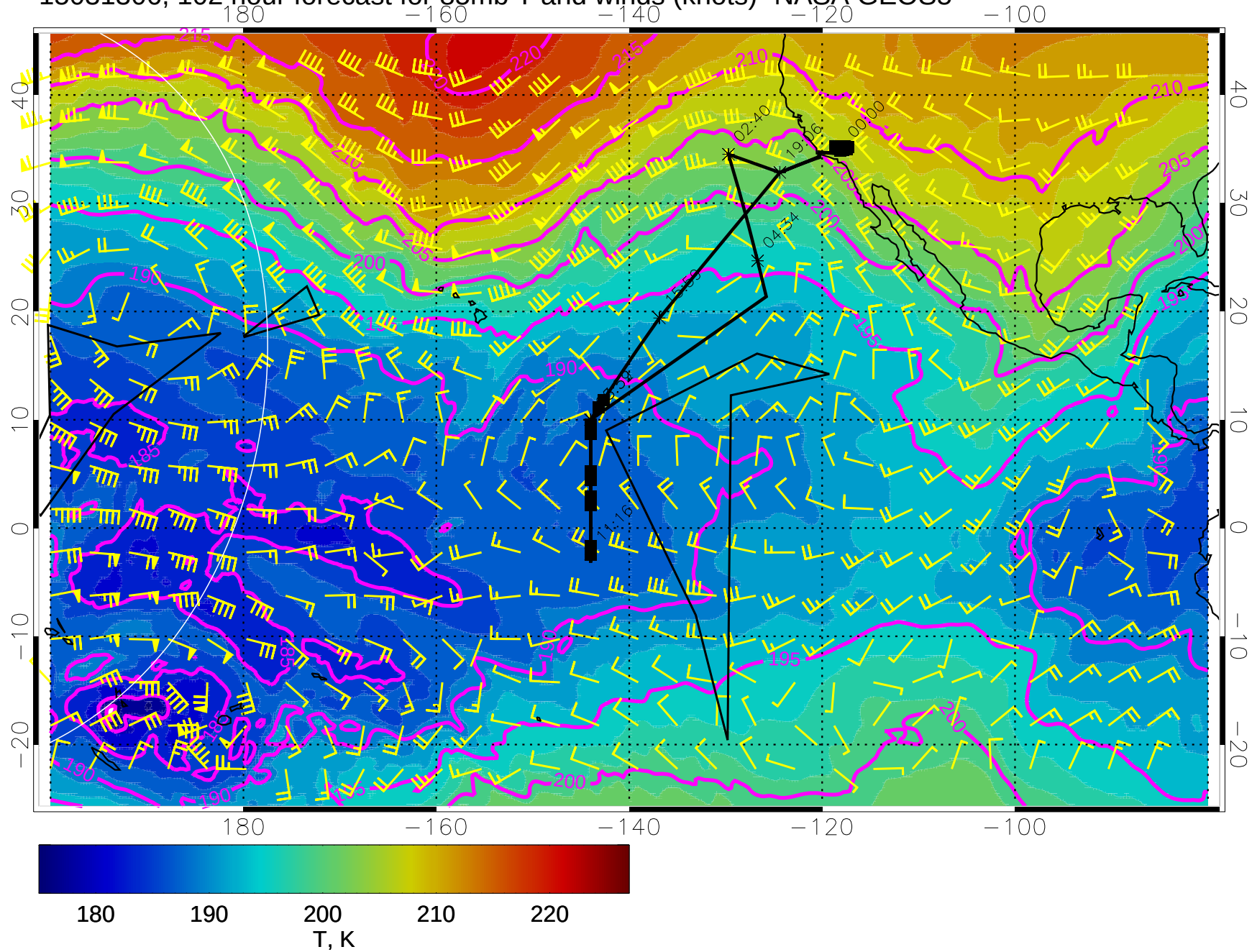
15031306, 102 hour forecast for 85mb T and winds (knots)- NASA GEOS5
