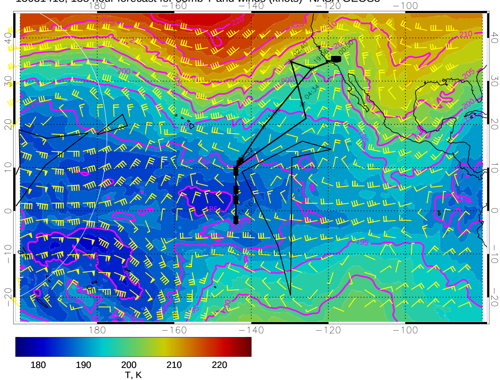
15031418, 138 hour forecast for 85mb T and winds (knots)- NASA GEOS5
