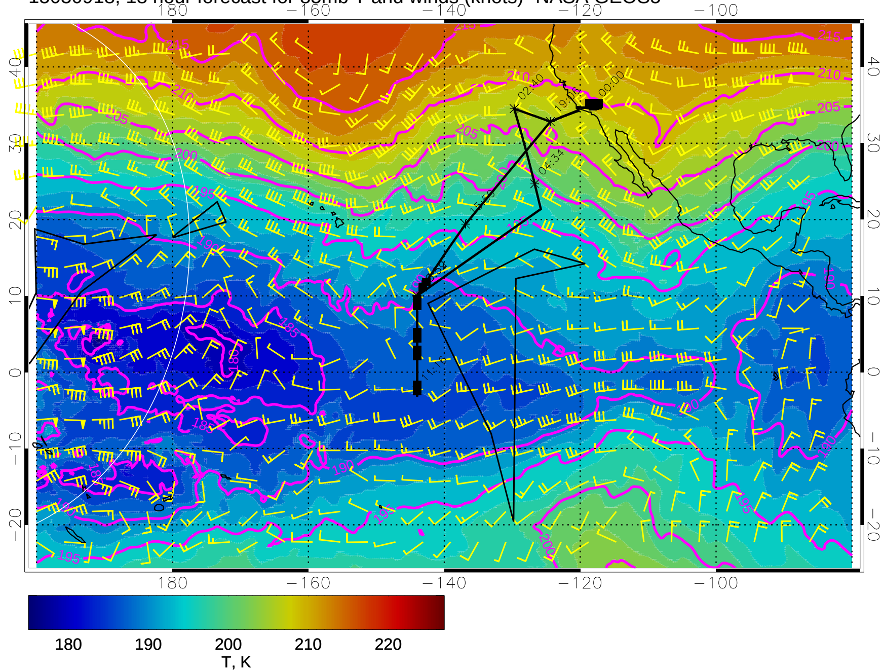
15030918, 18 hour forecast for 85mb T and winds (knots)- NASA GEOS5
