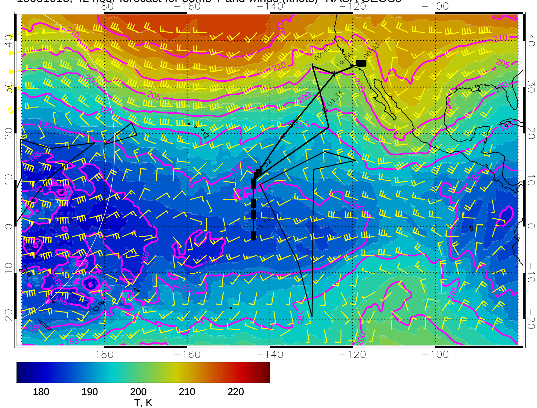
15031018, 42 hour forecast for 85mb T and winds (knots)- NASA GEOS5
