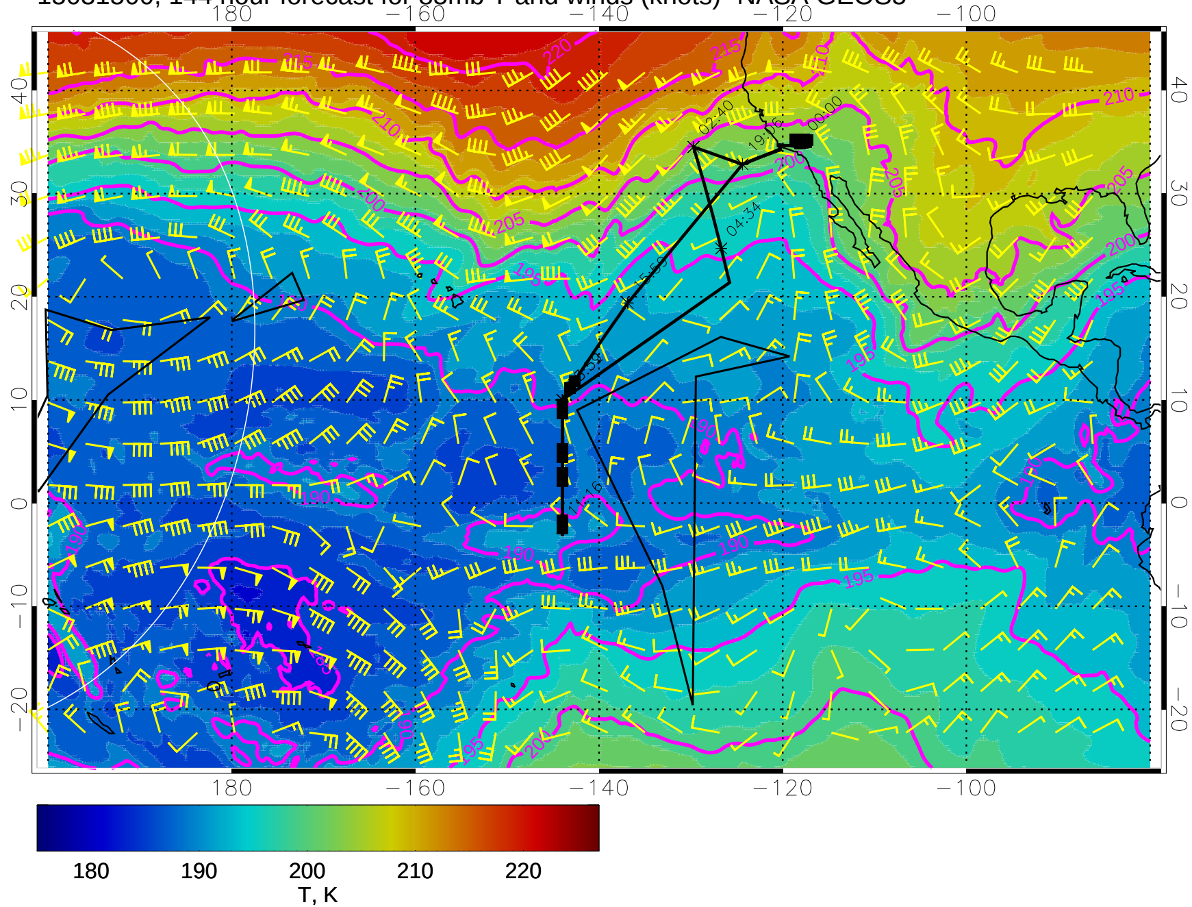
15031500, 144 hour forecast for 85mb T and winds (knots)- NASA GEOS5
