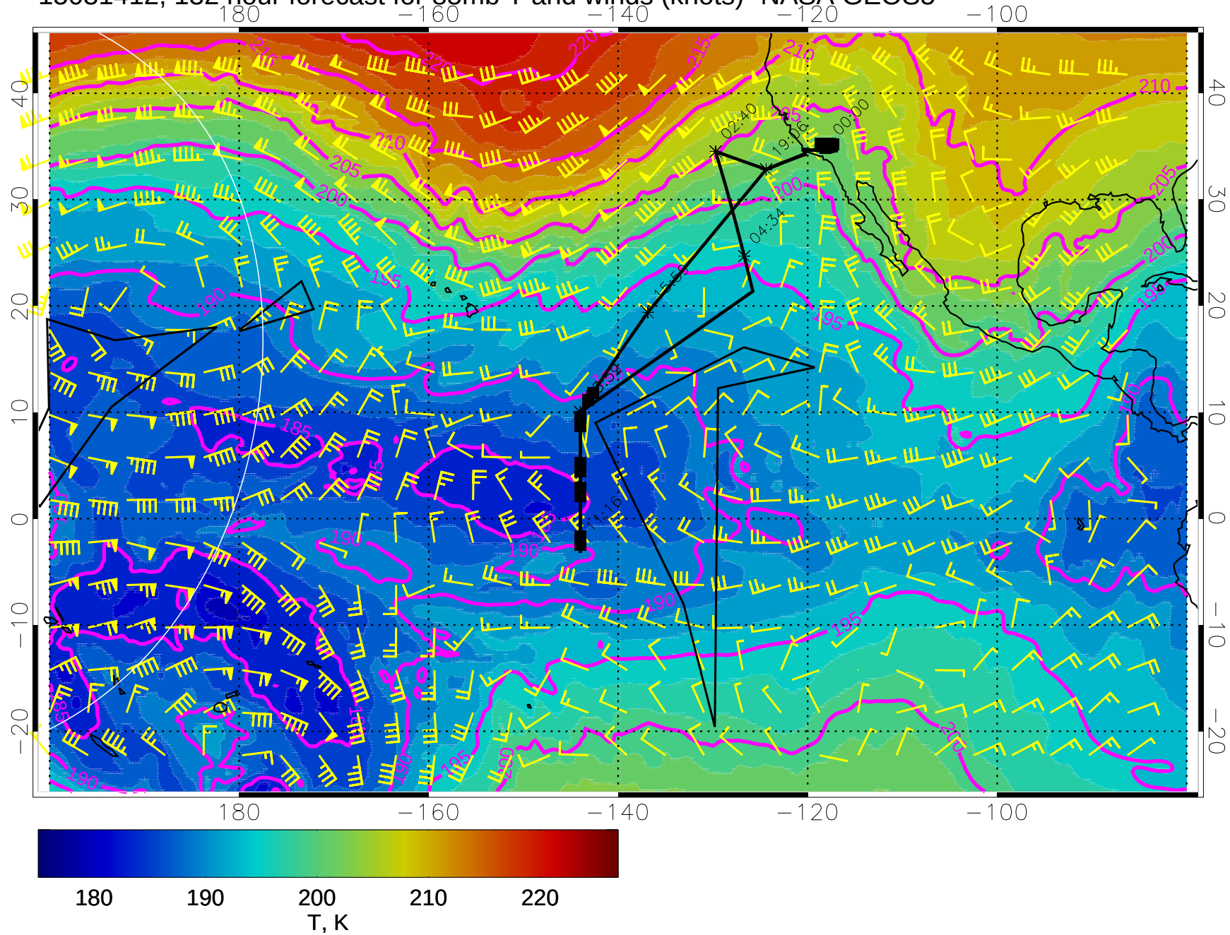
15031412, 132 hour forecast for 85mb T and winds (knots)- NASA GEOS5
