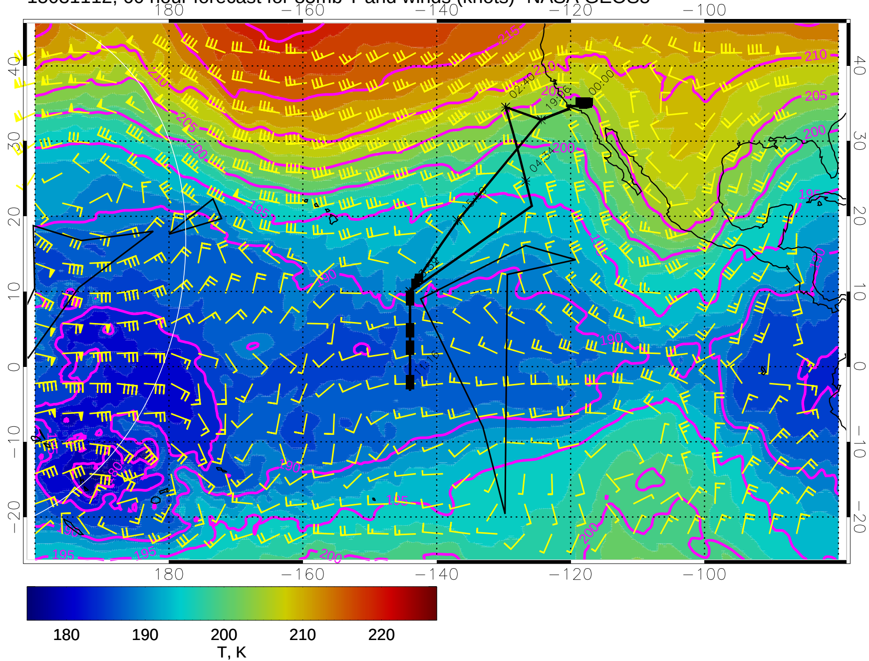
15031112, 60 hour forecast for 85mb T and winds (knots)- NASA GEOS5
