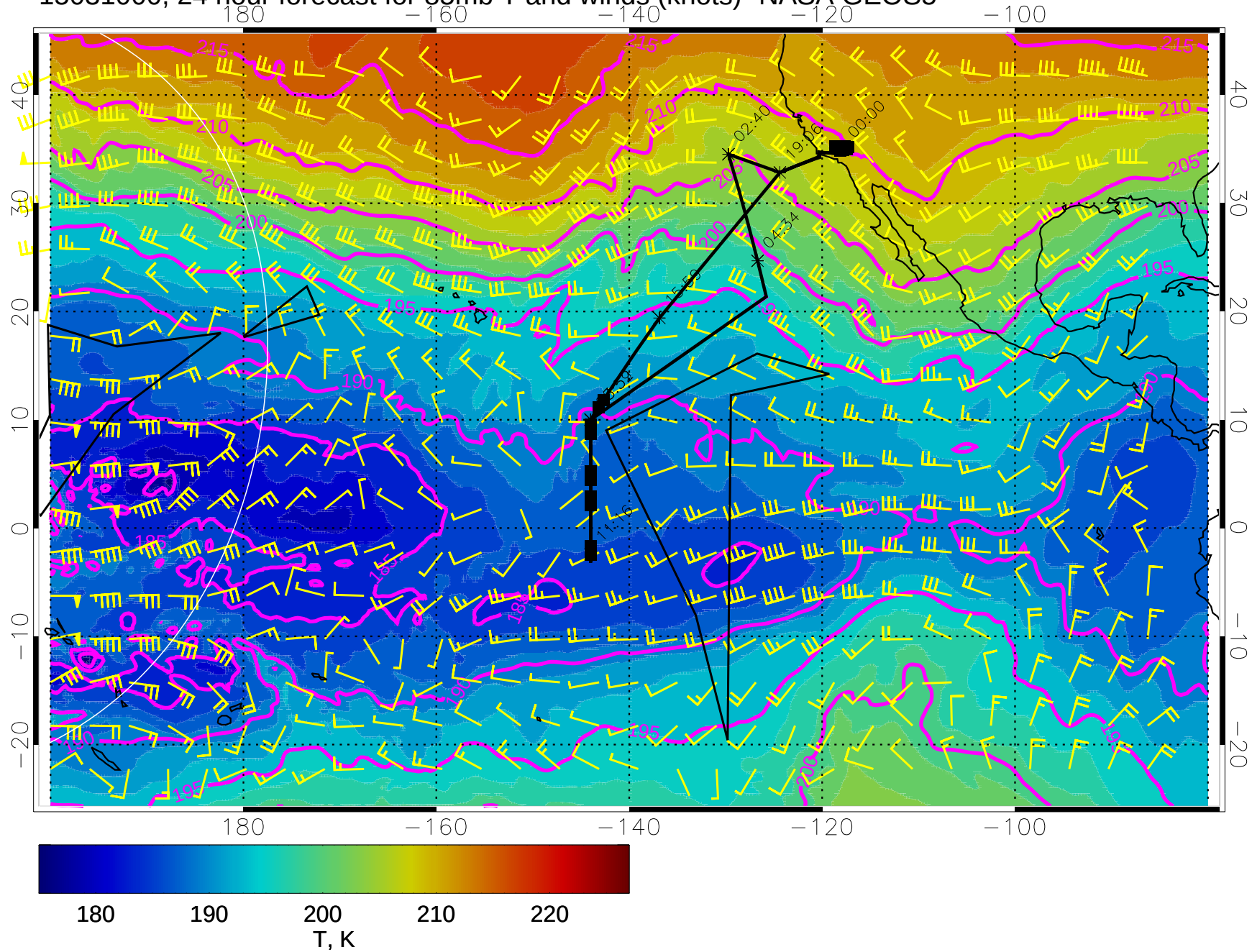
15031000, 24 hour forecast for 85mb T and winds (knots)- NASA GEOS5
