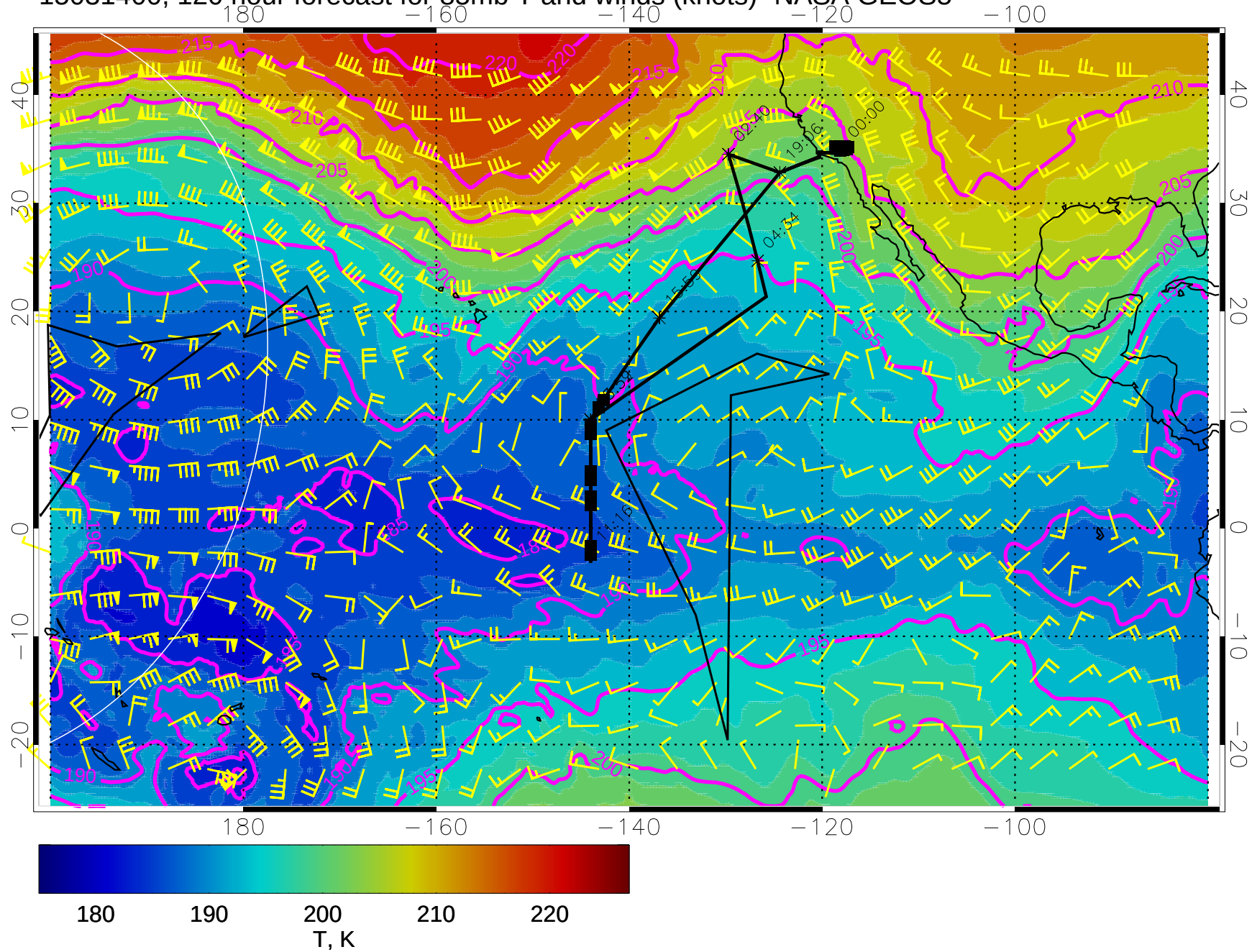
15031400, 120 hour forecast for 85mb T and winds (knots)- NASA GEOS5
