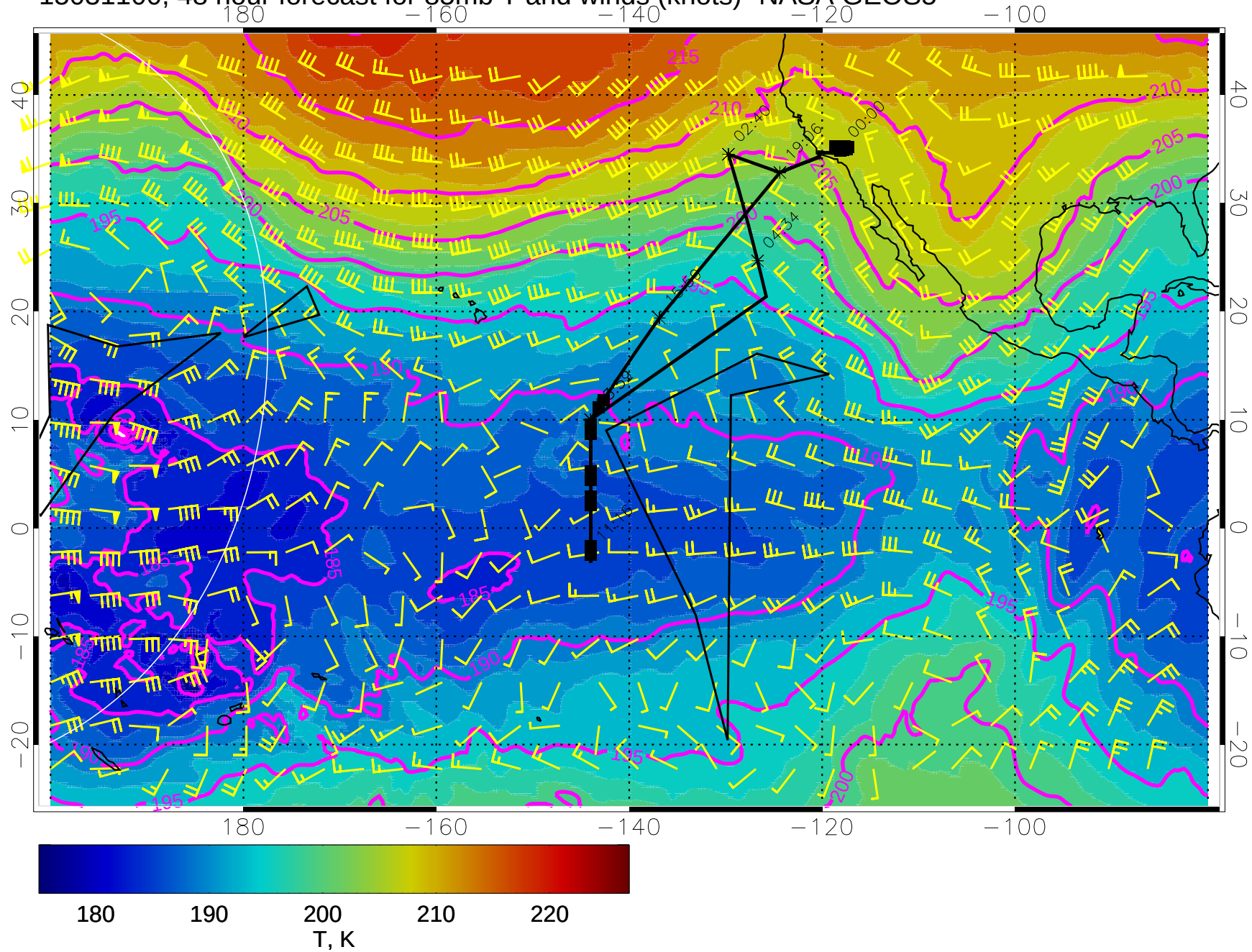
15031100, 48 hour forecast for 85mb T and winds (knots)- NASA GEOS5
