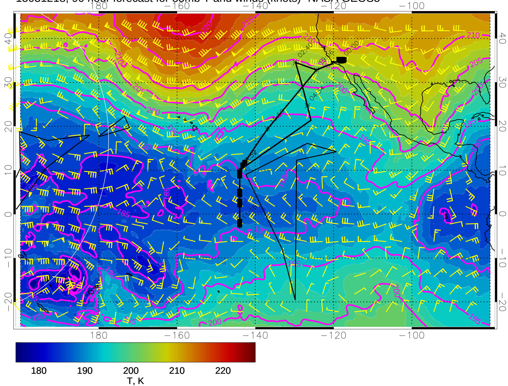
15031218, 90 hour forecast for 85mb T and winds (knots)- NASA GEOS5
