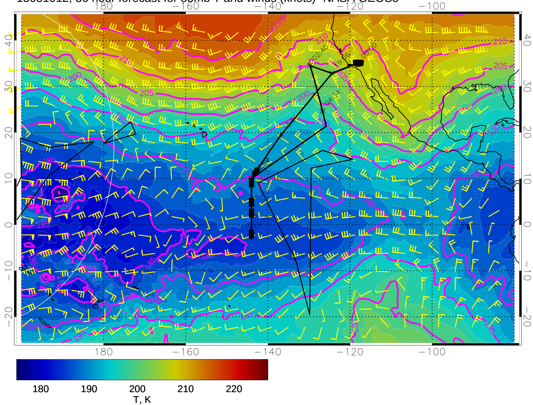
15031012, 36 hour forecast for 85mb T and winds (knots)- NASA GEOS5
