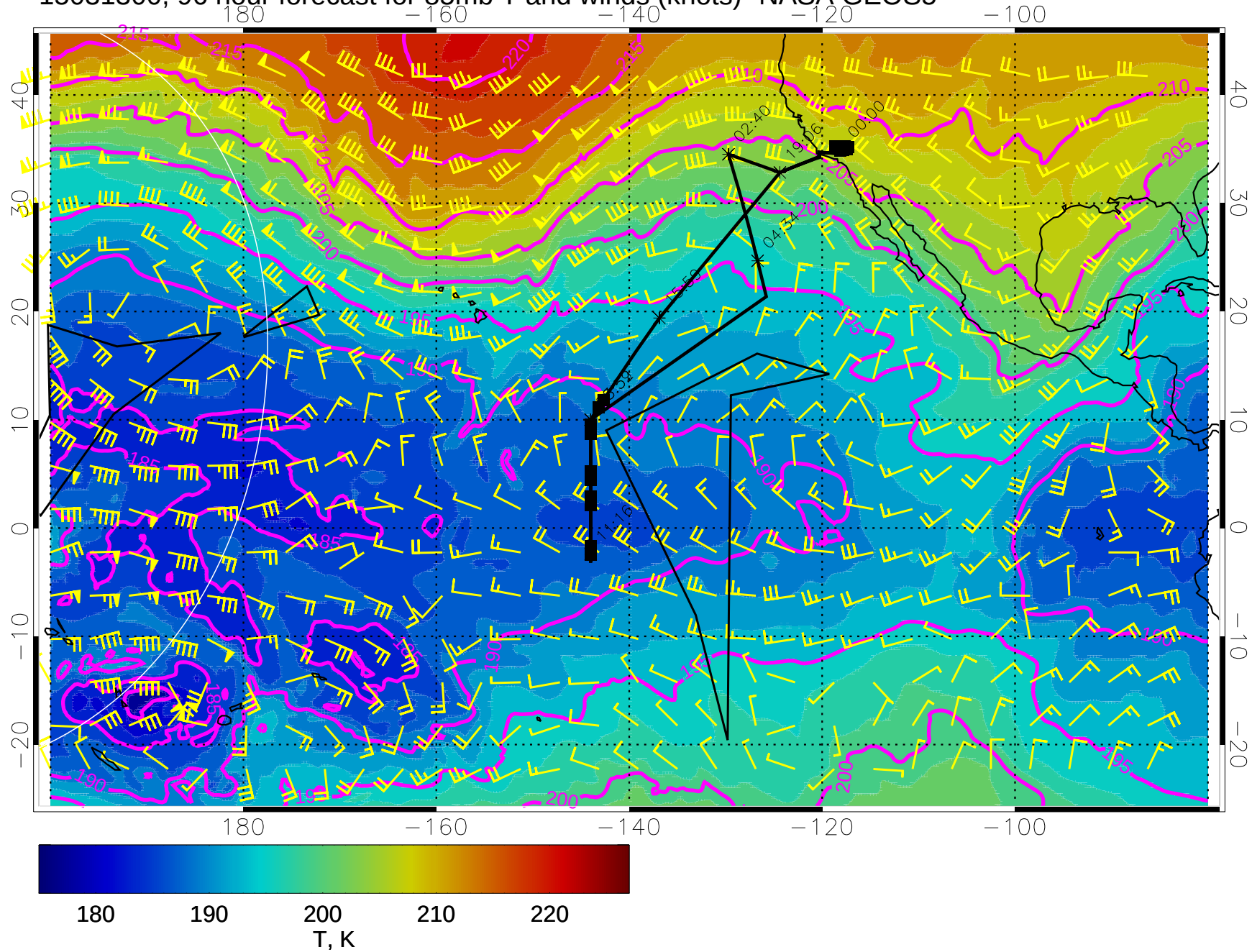
15031300, 96 hour forecast for 85mb T and winds (knots)- NASA GEOS5
