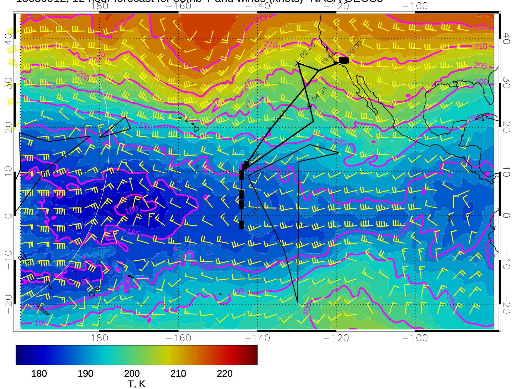
15030912, 12 hour forecast for 85mb T and winds (knots)- NASA GEOS5
