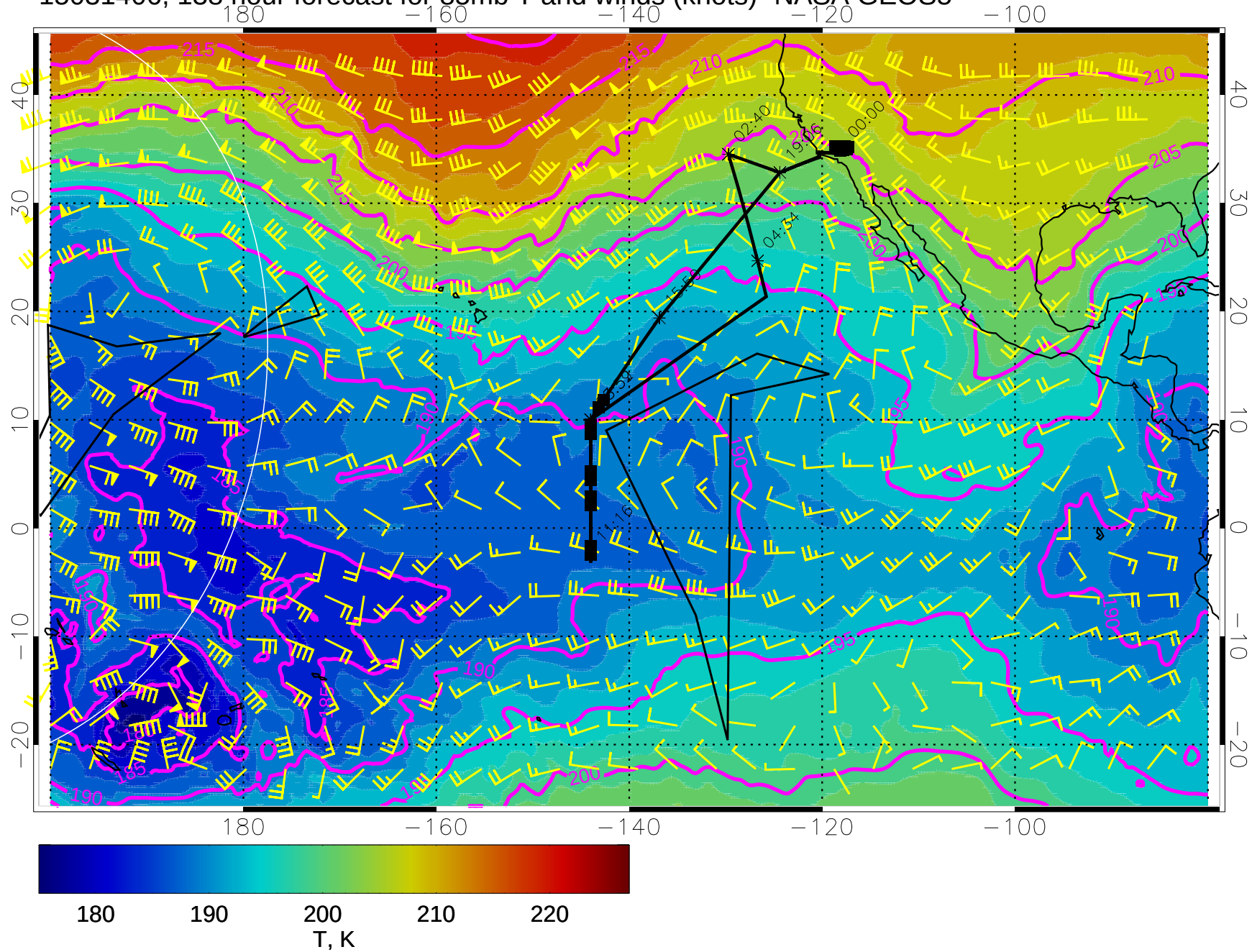
15031406, 138 hour forecast for 85mb T and winds (knots)- NASA GEOS5
