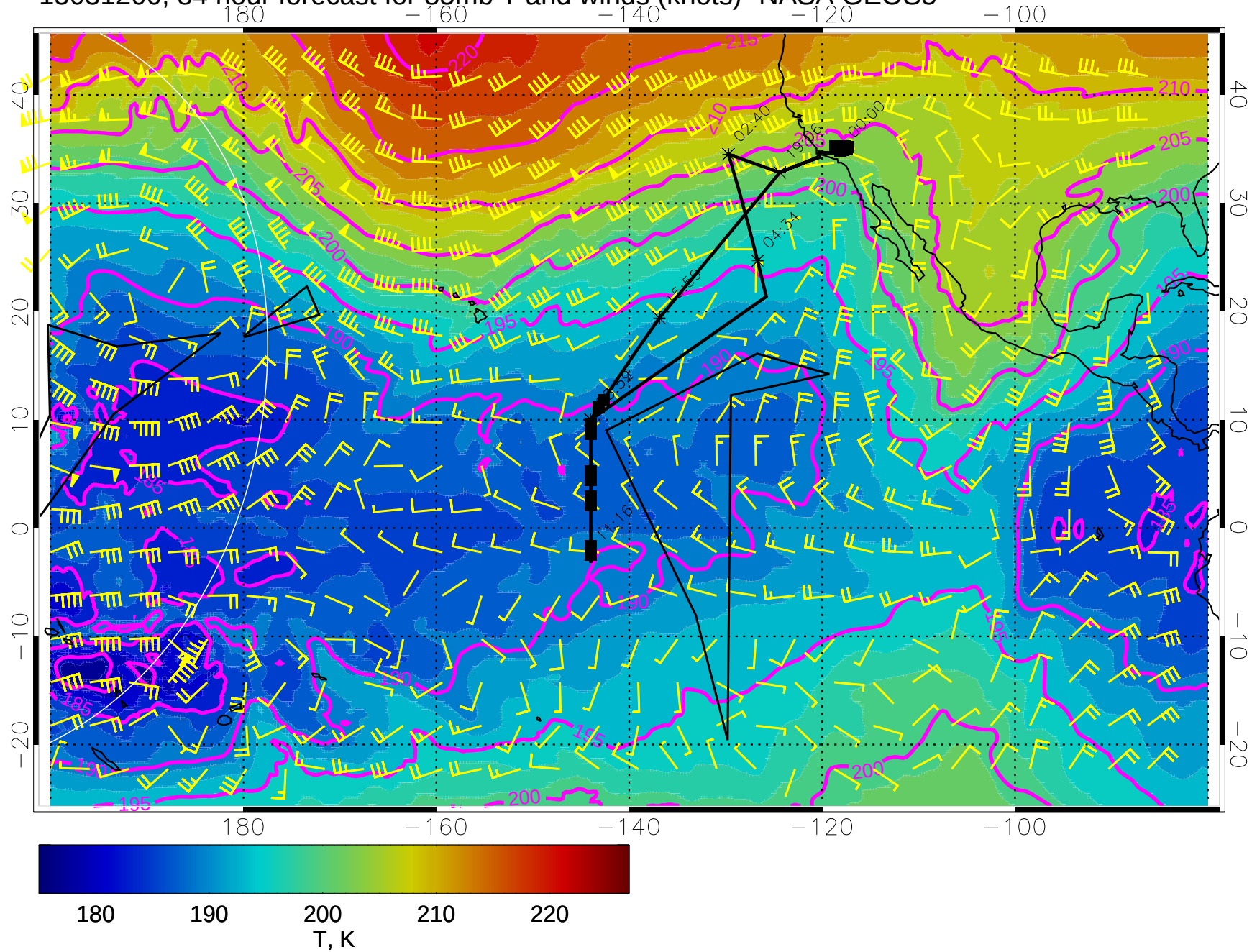
15031200, 84 hour forecast for 85mb T and winds (knots)- NASA GEOS5
