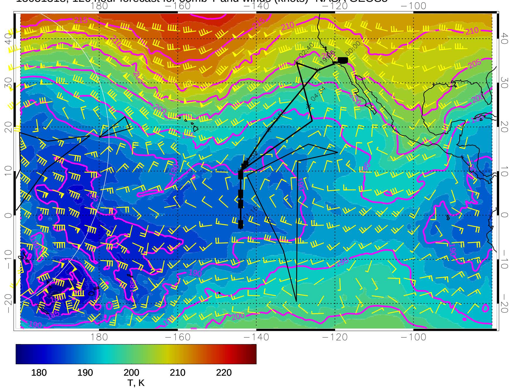
15031318, 126 hour forecast for 85mb T and winds (knots)- NASA GEOS5
