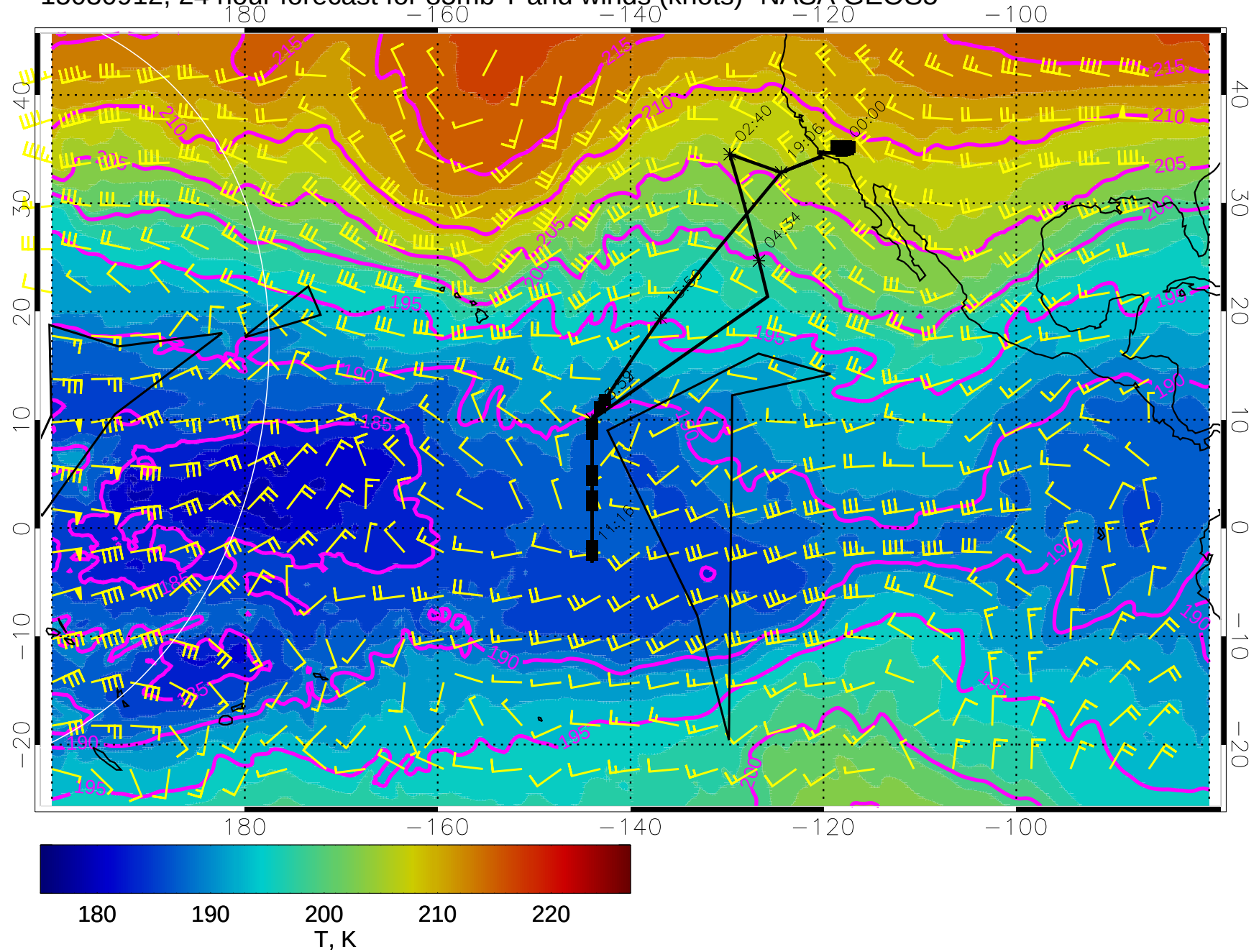
15030912, 24 hour forecast for 85mb T and winds (knots)- NASA GEOS5
