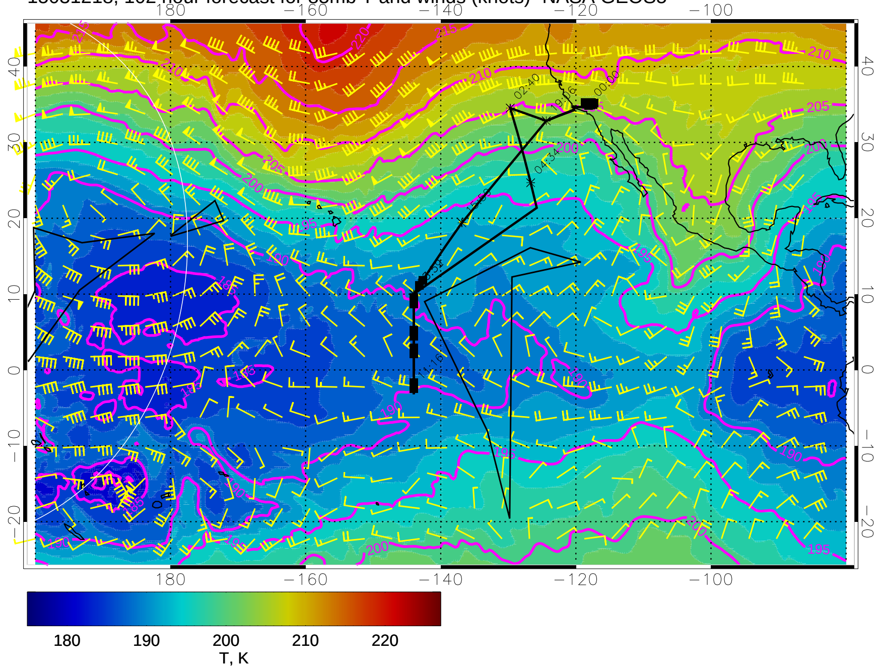
15031218, 102 hour forecast for 85mb T and winds (knots)- NASA GEOS5
