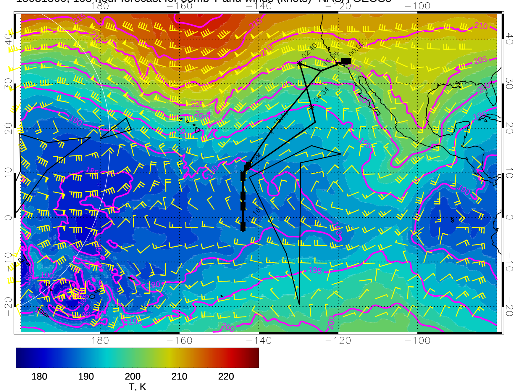
15031300, 108 hour forecast for 85mb T and winds (knots)- NASA GEOS5
