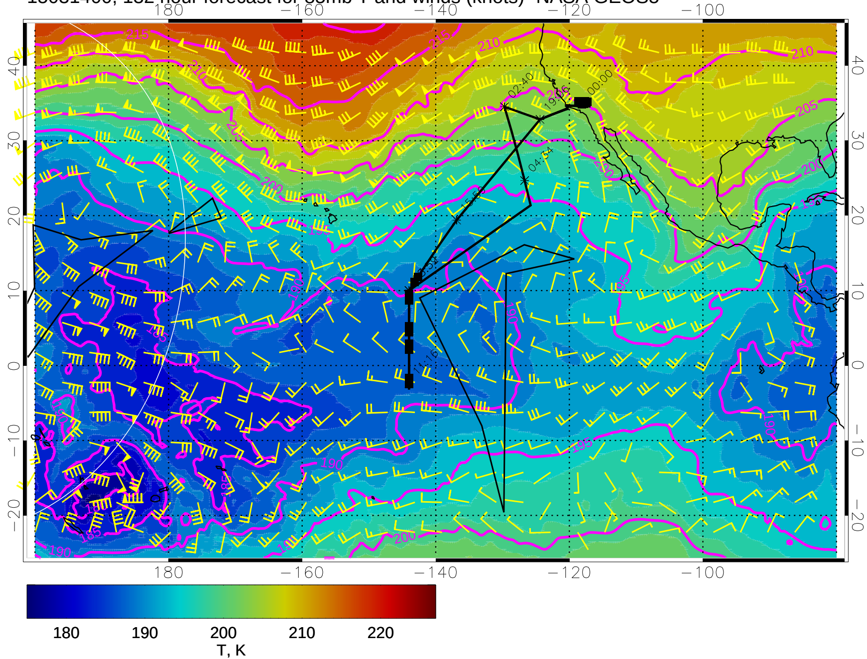
15031400, 132 hour forecast for 85mb T and winds (knots)- NASA GEOS5
