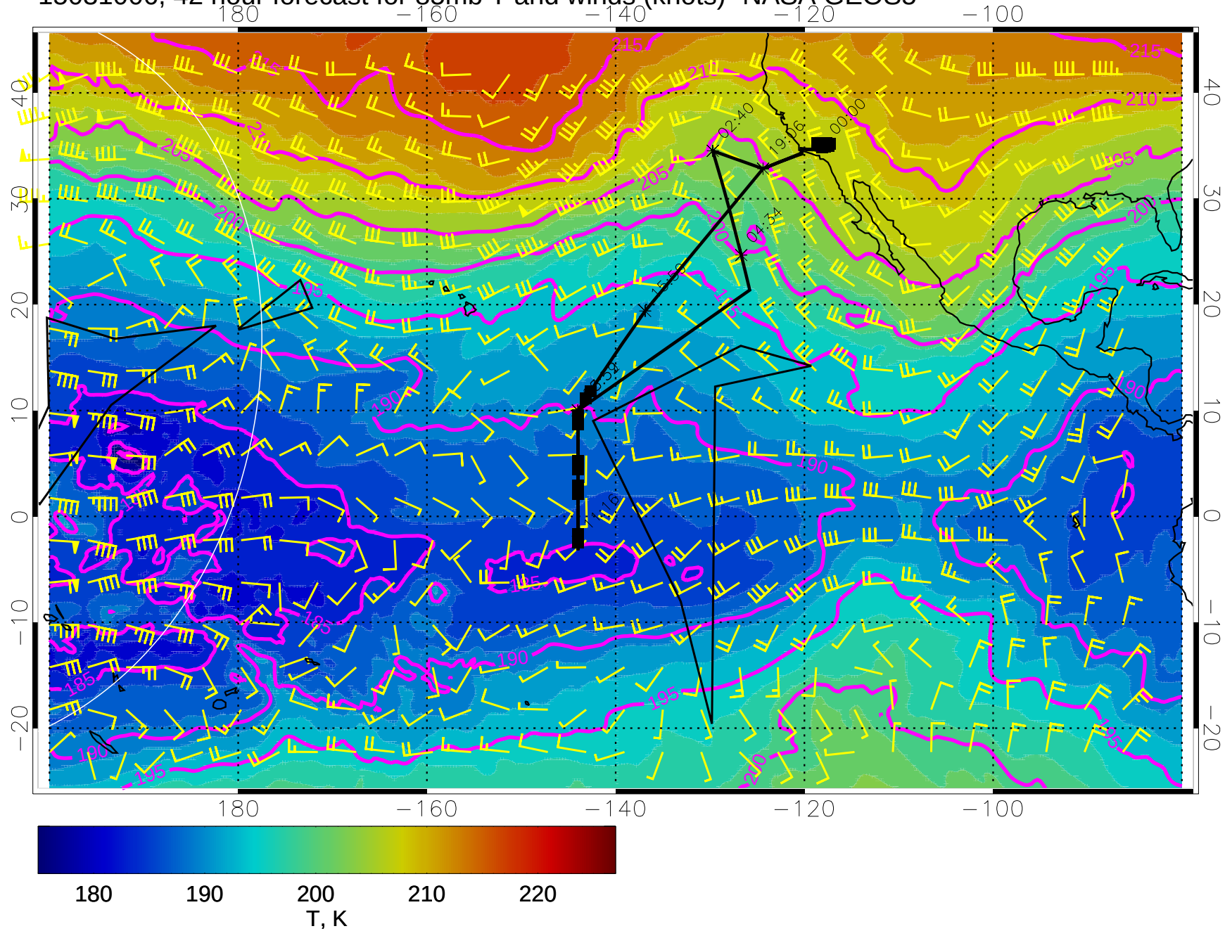
15031006, 42 hour forecast for 85mb T and winds (knots)- NASA GEOS5
