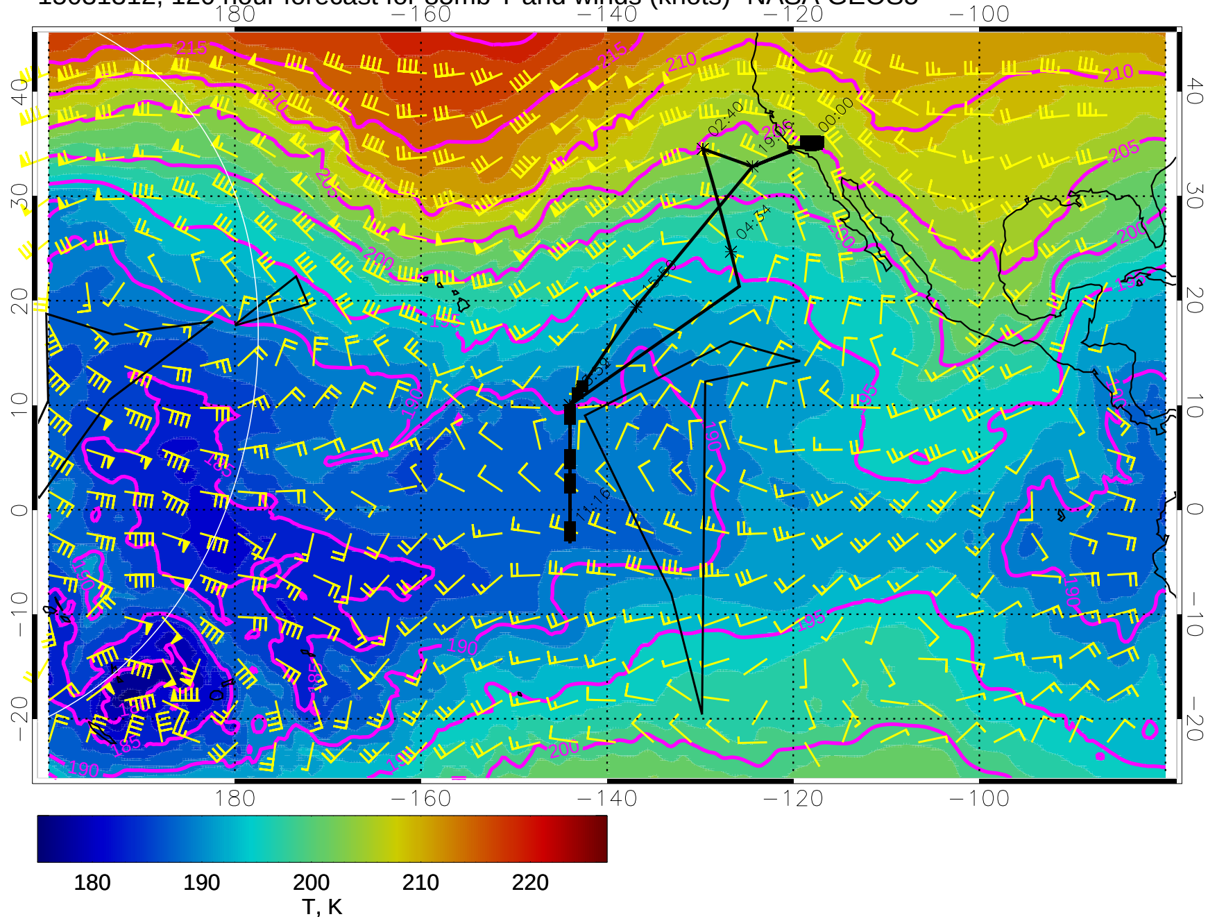
15031312, 120 hour forecast for 85mb T and winds (knots)- NASA GEOS5
