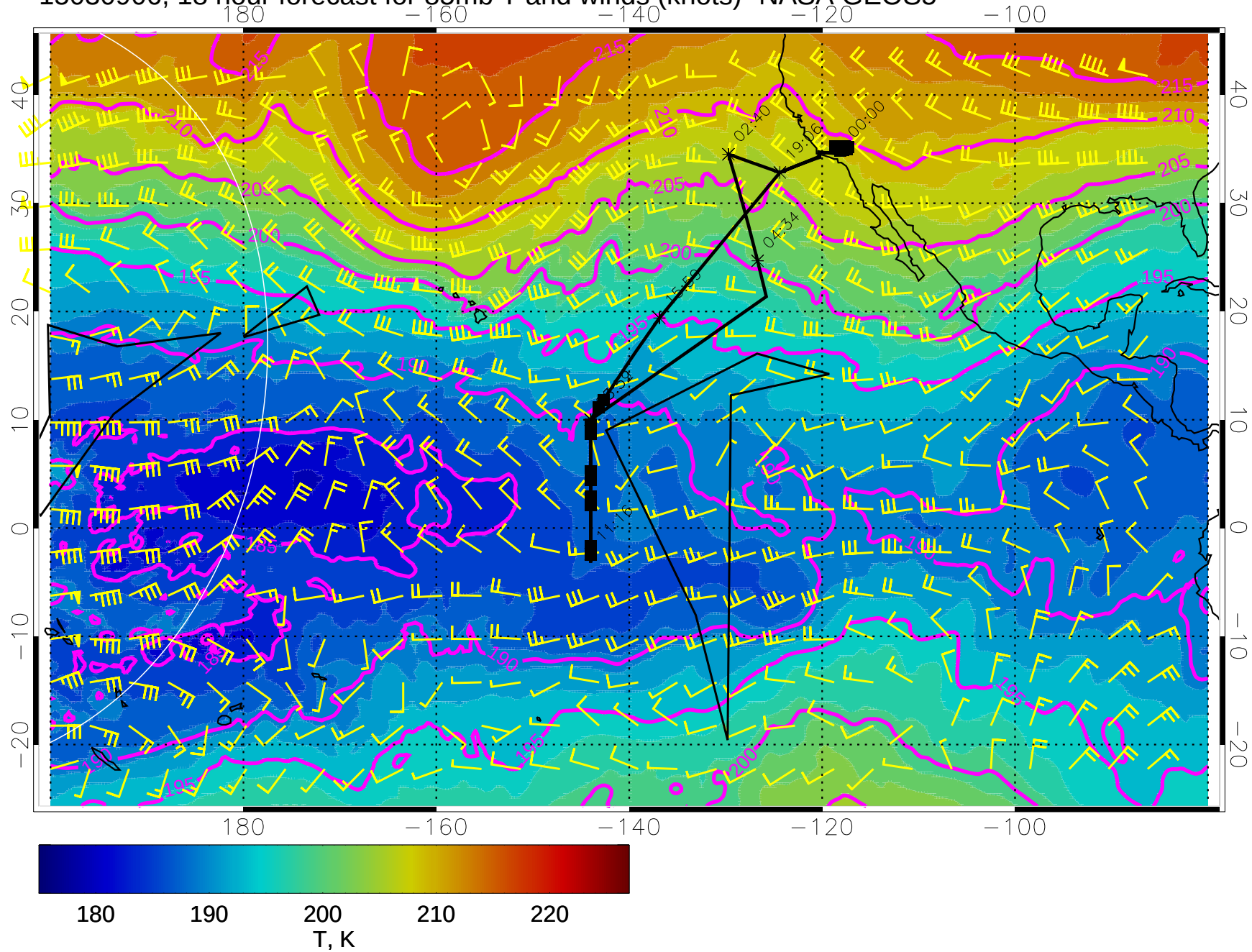
15030906, 18 hour forecast for 85mb T and winds (knots)- NASA GEOS5
