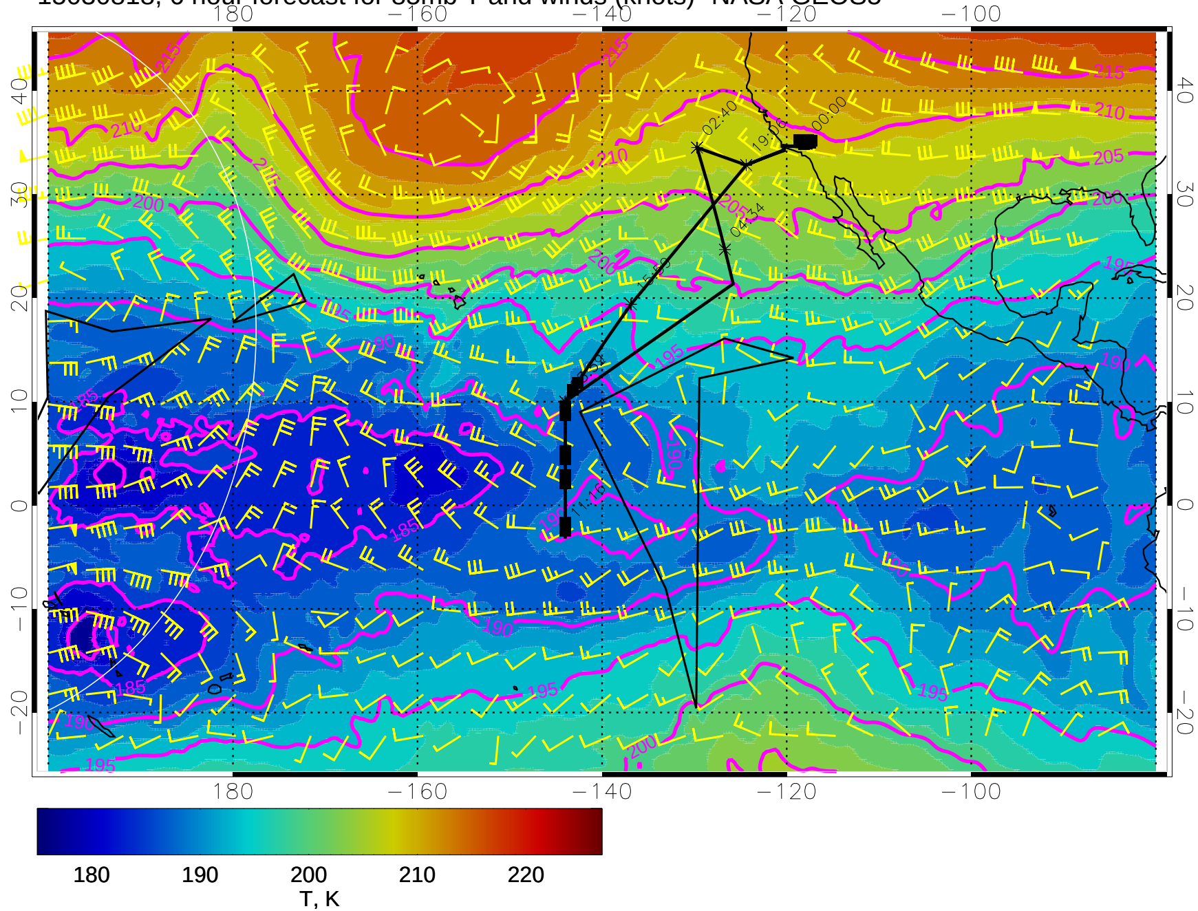
15030818, 6 hour forecast for 85mb T and winds (knots)- NASA GEOS5
