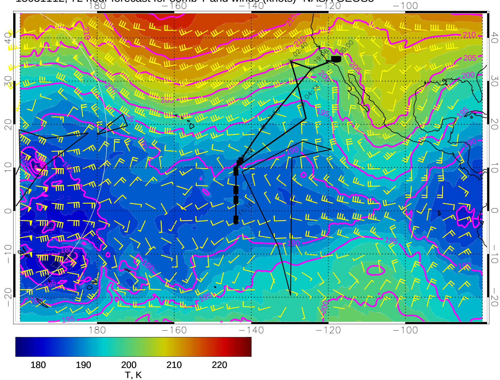
15031112, 72 hour forecast for 85mb T and winds (knots)- NASA GEOS5
