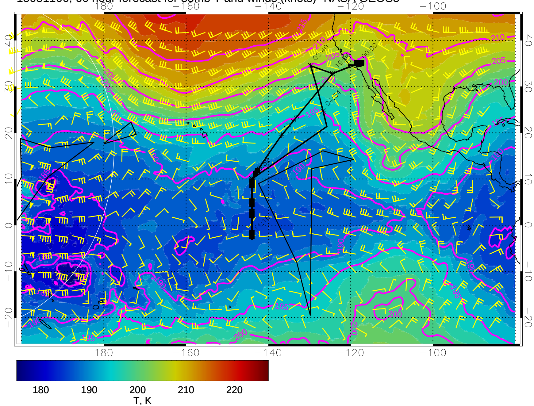
15031106, 66 hour forecast for 85mb T and winds (knots)- NASA GEOS5
