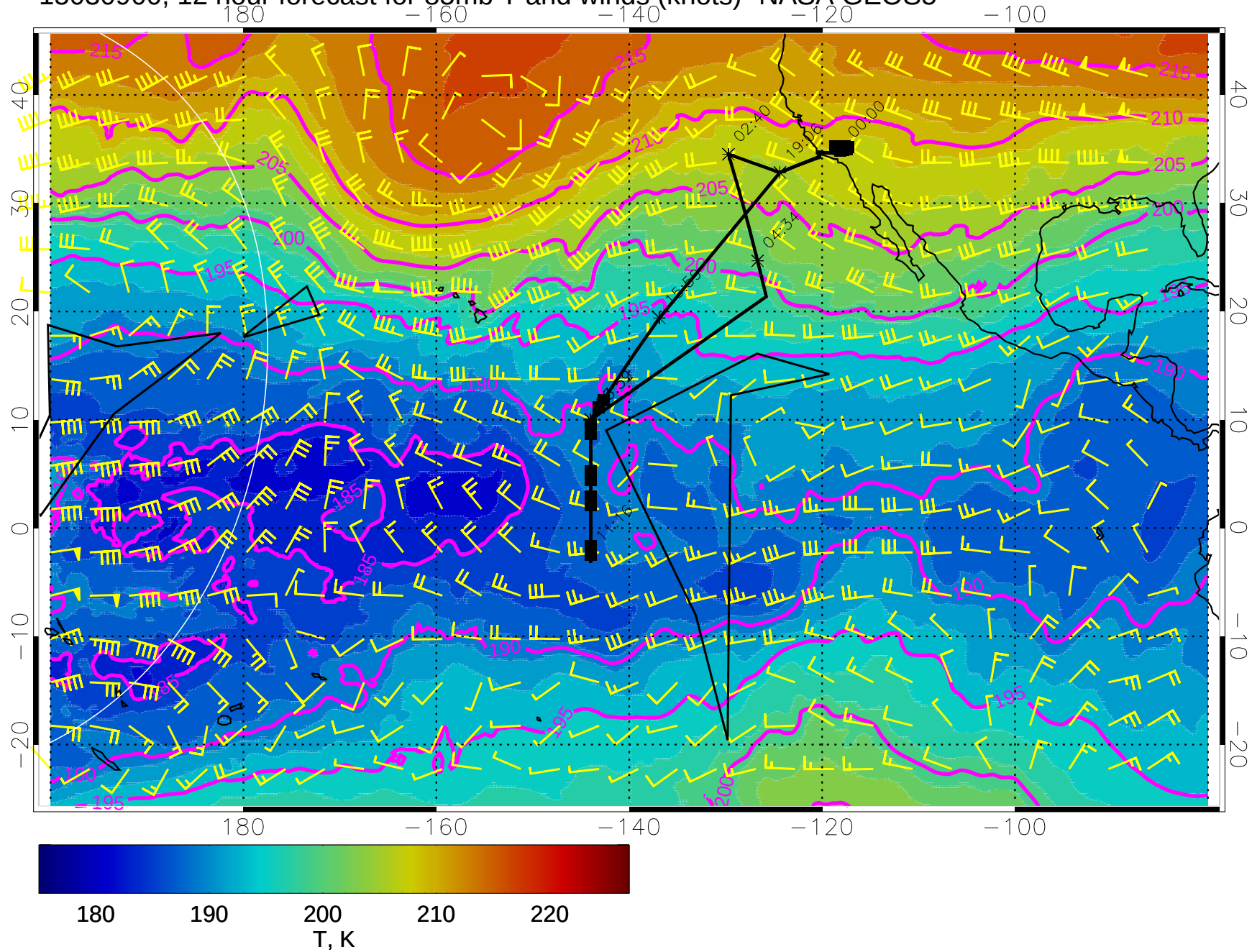
15030900, 12 hour forecast for 85mb T and winds (knots)- NASA GEOS5
