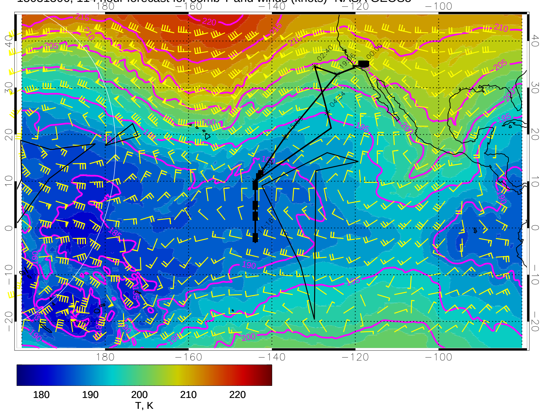
15031306, 114 hour forecast for 85mb T and winds (knots)- NASA GEOS5
