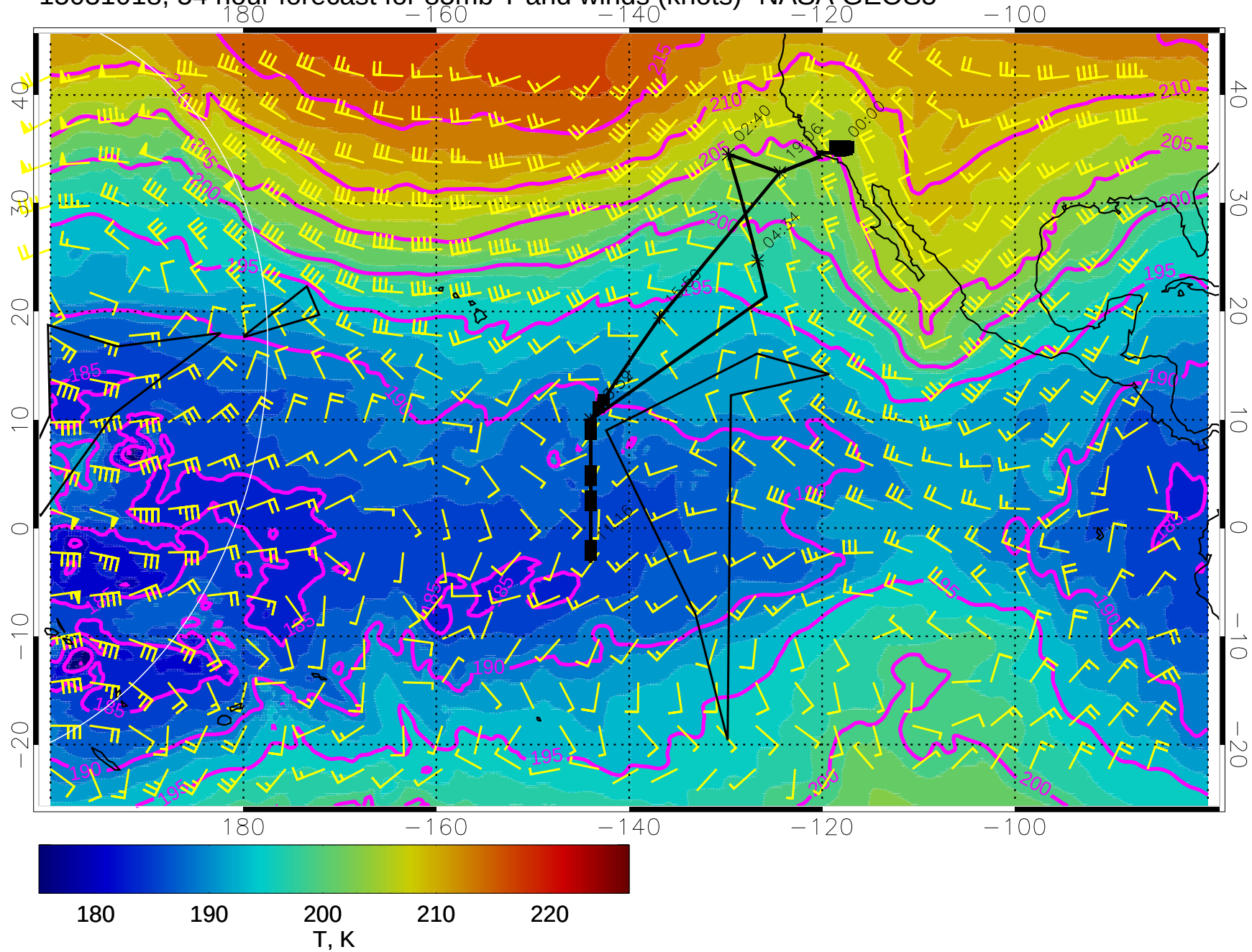
15031018, 54 hour forecast for 85mb T and winds (knots)- NASA GEOS5
