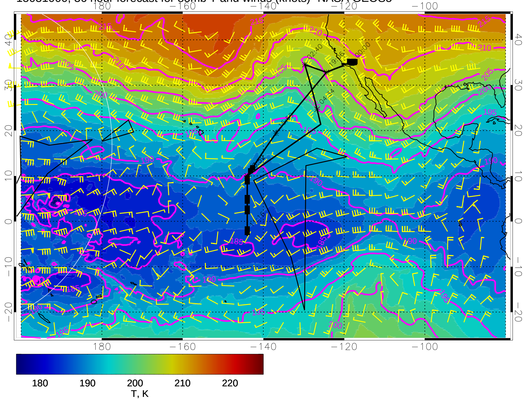
15031000, 36 hour forecast for 85mb T and winds (knots)- NASA GEOS5
