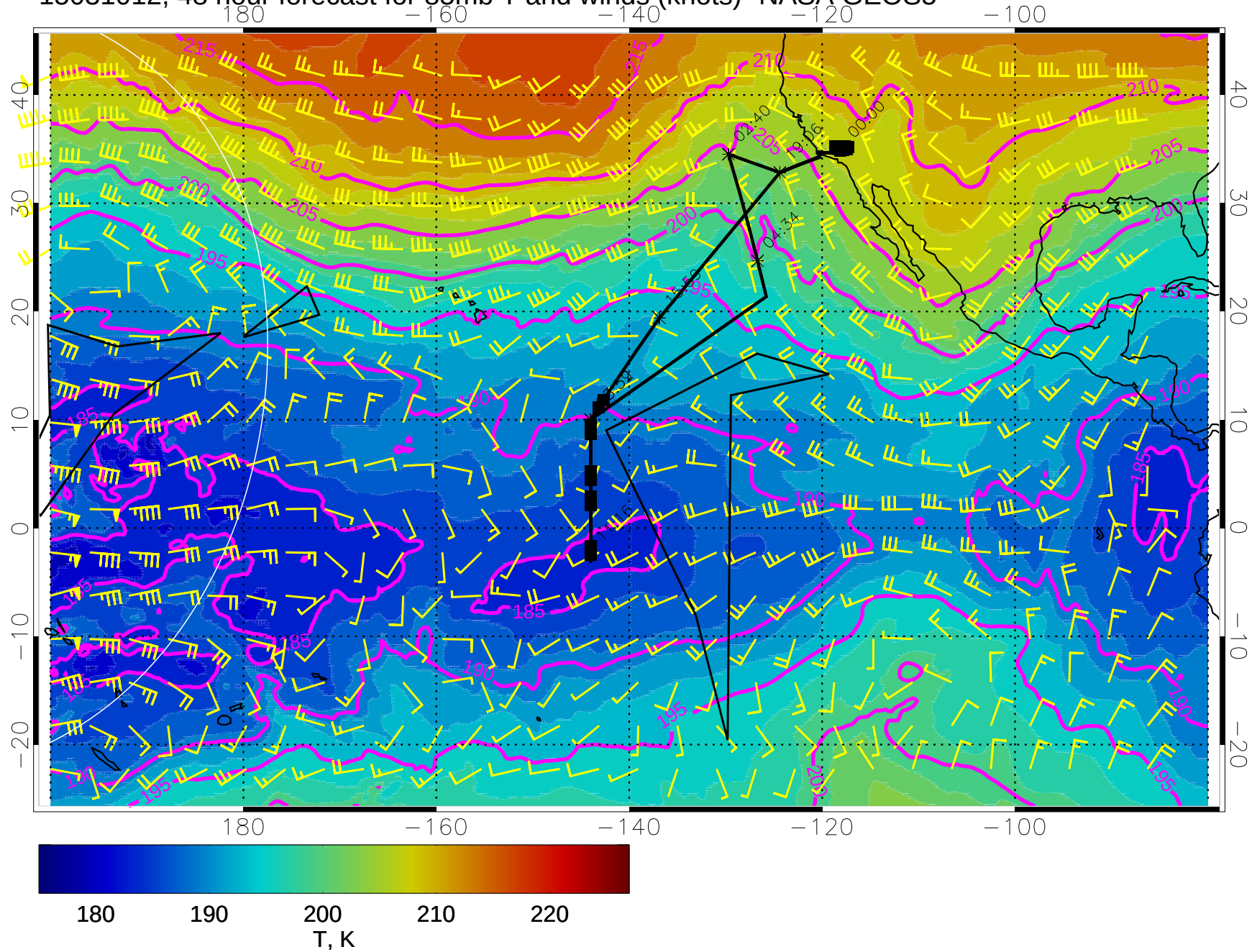
15031012, 48 hour forecast for 85mb T and winds (knots)- NASA GEOS5
