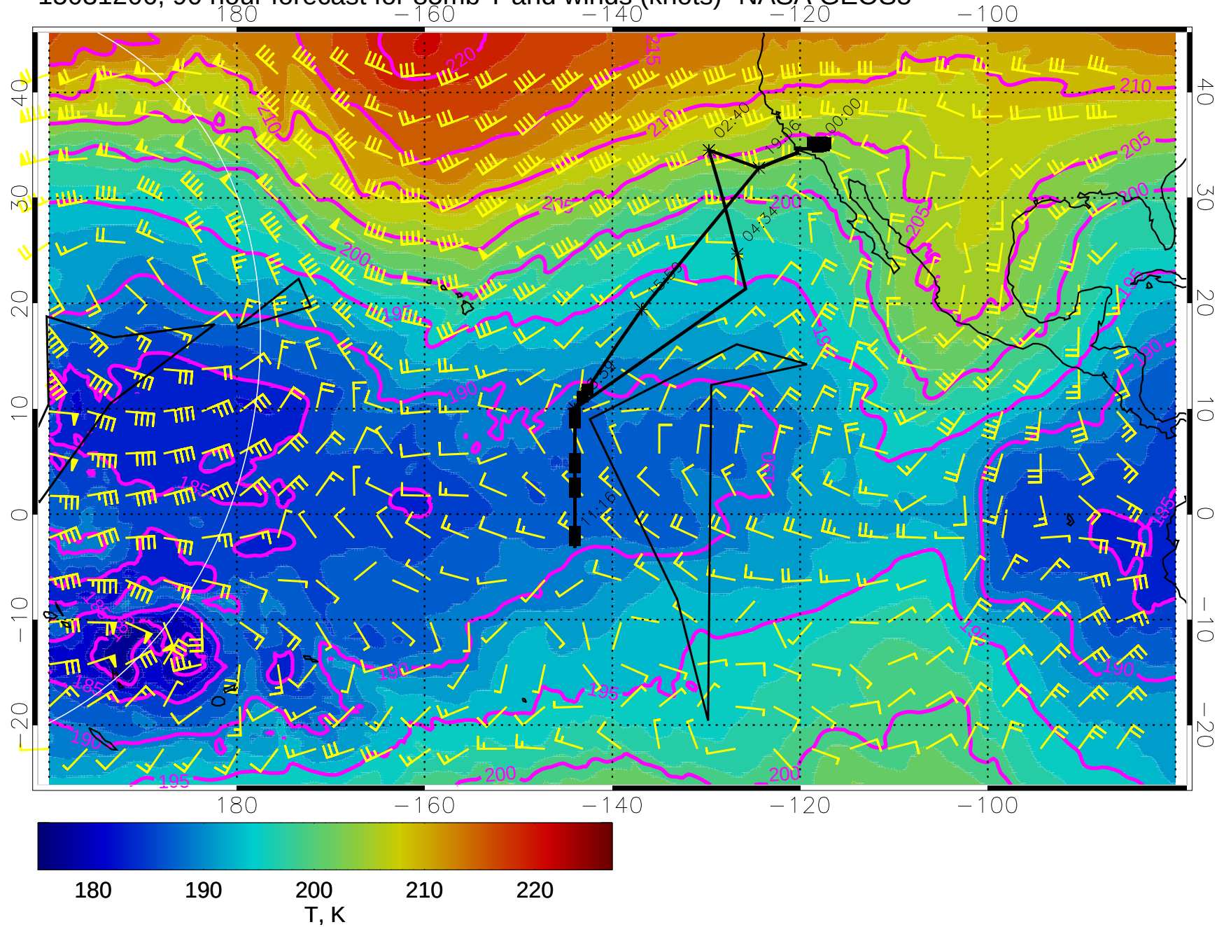
15031206, 90 hour forecast for 85mb T and winds (knots)- NASA GEOS5
