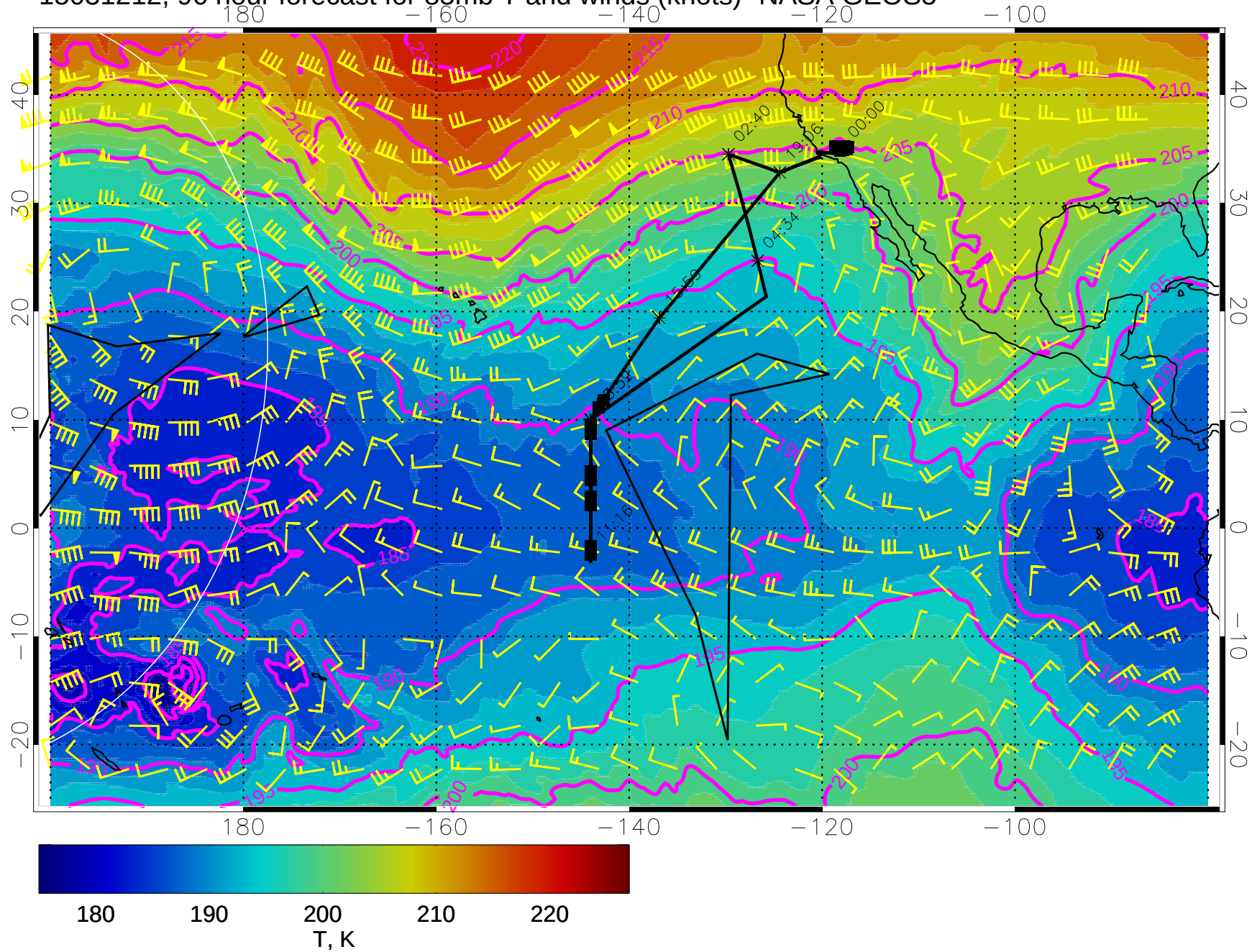
15031212, 96 hour forecast for 85mb T and winds (knots)- NASA GEOS5
