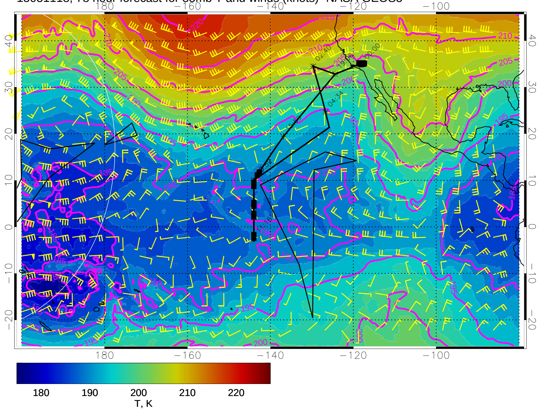
15031118, 78 hour forecast for 85mb T and winds (knots)- NASA GEOS5
