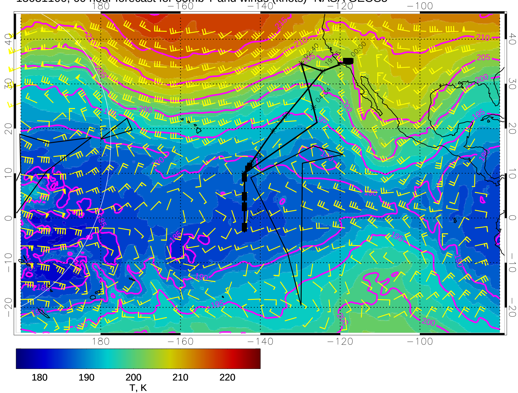
15031100, 60 hour forecast for 85mb T and winds (knots)- NASA GEOS5
