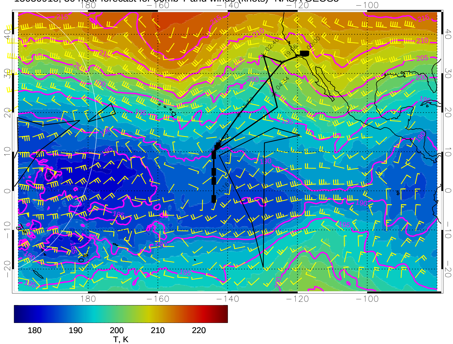
15030918, 30 hour forecast for 85mb T and winds (knots)- NASA GEOS5
